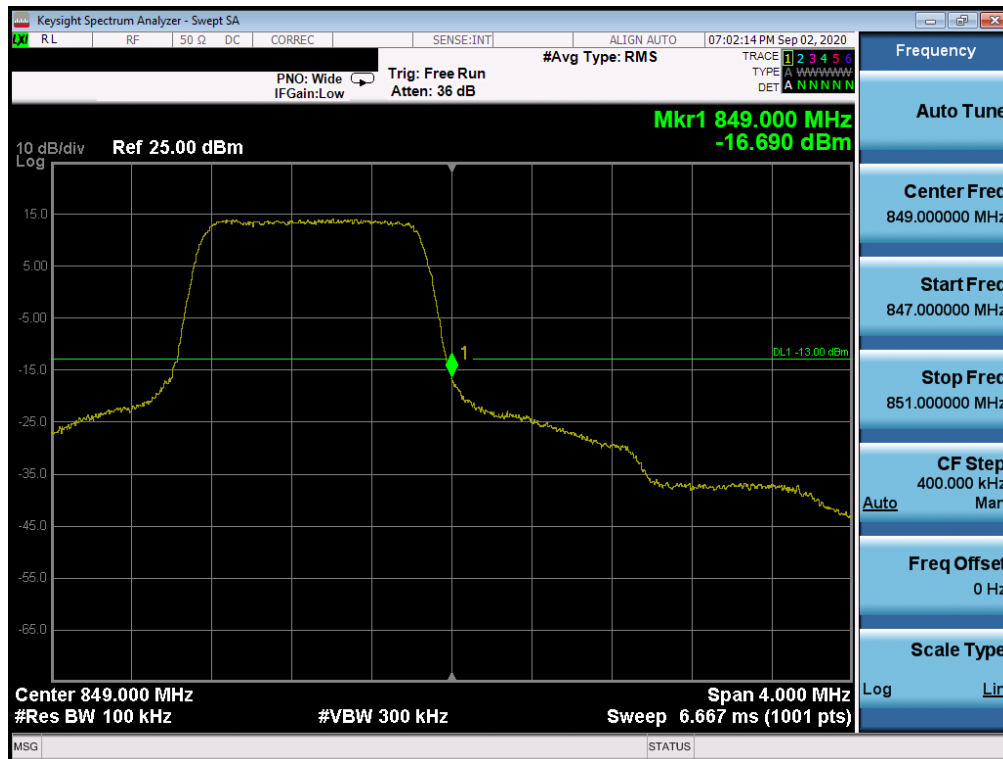
Plot 7-60. Upper Band Edge Plot (LTE Band 5 – 1.4MHz QPSK – Full RB Configuration)
