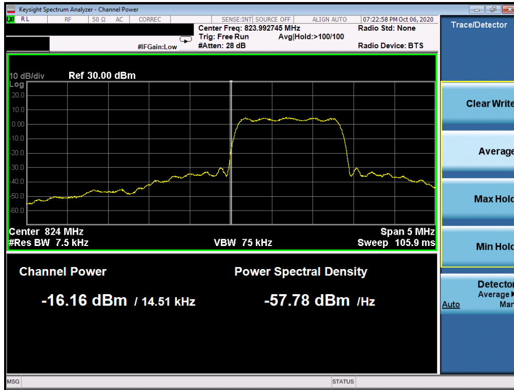
Plot 7-65. Lower Band Edge Plot (CDMA Cell – Ch. 1013)
