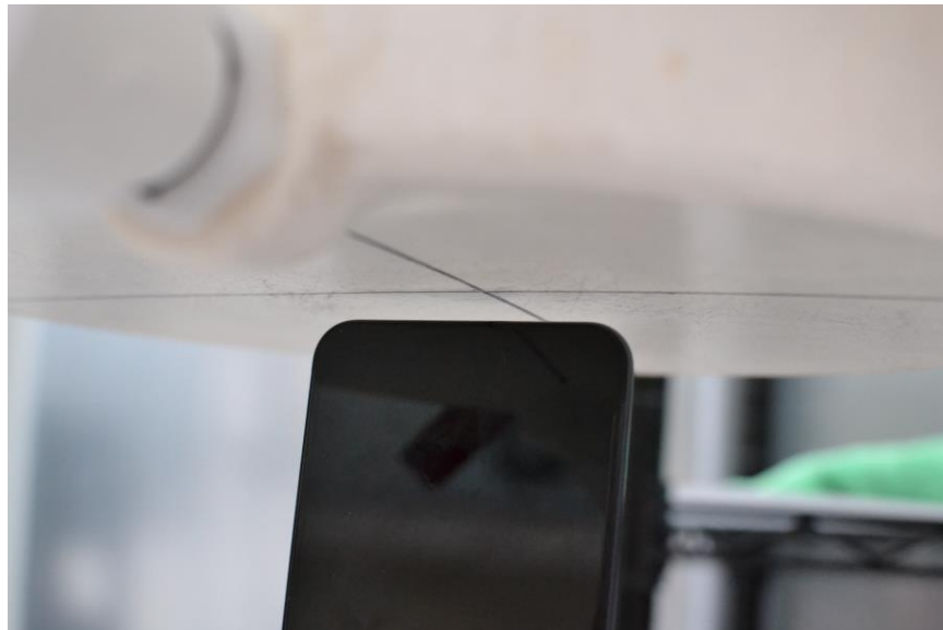
SAR Test Setup Photo 10 Bottom Edge 10 mm
