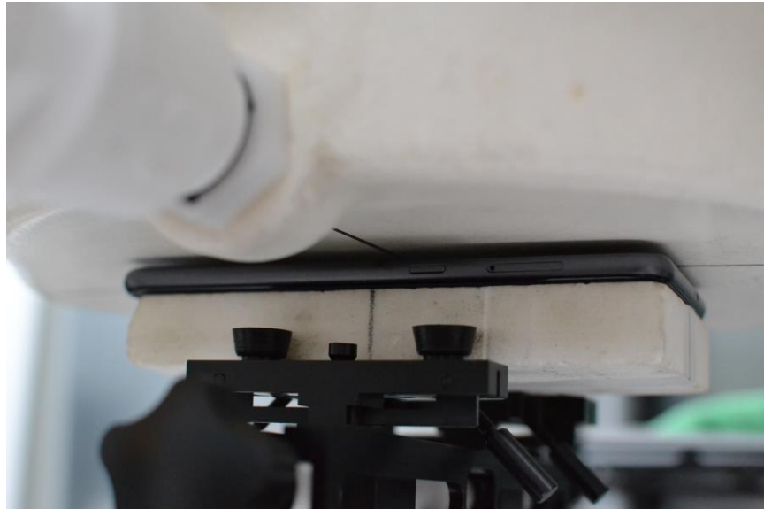
SAR Test Setup Photo 6 Back Side 2 mm
