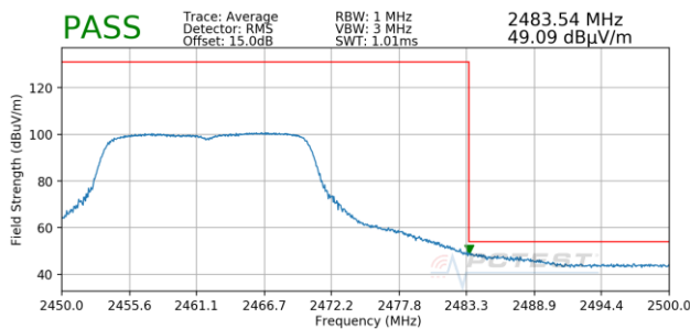
Plot 7-41. Radiated Restricted Upper Band Edge Measurement (Average)
