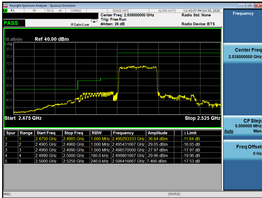
Plot 7-26. Lower ACP Plot (LTE Band 7 - 10MHz QPSK – Full RB Configuration)
