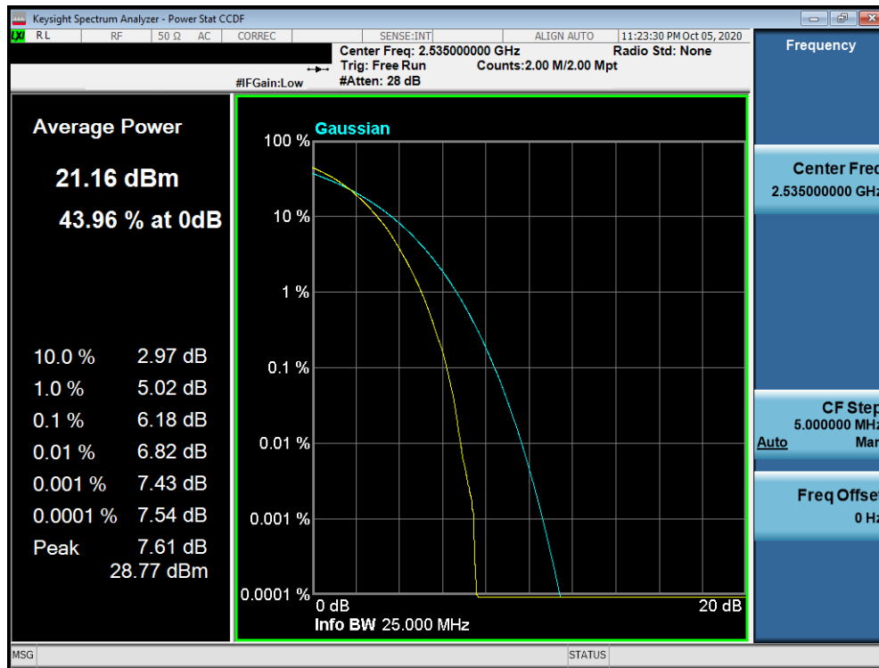
Plot 7-32. PAR Plot (LTE Band 7 - 20MHz 64-QAM - Full RB Configuration)
