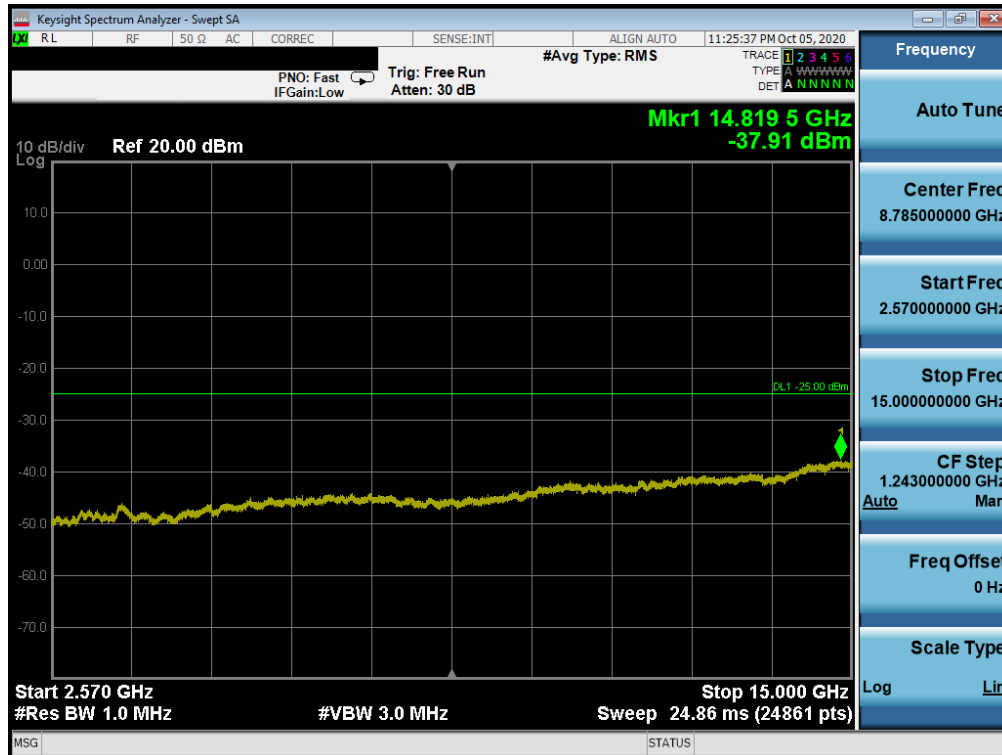
Plot 7-17. Conducted Spurious Plot (LTE Band 7 - 20MHz QPSK - RB Size 1, RB Offset 0 - Mid Channel)
