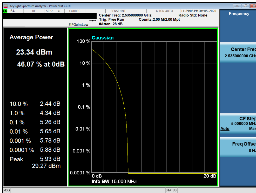
Plot 7-33. PAR Plot (LTE Band 7 - 15MHz QPSK - Full RB Configuration)
