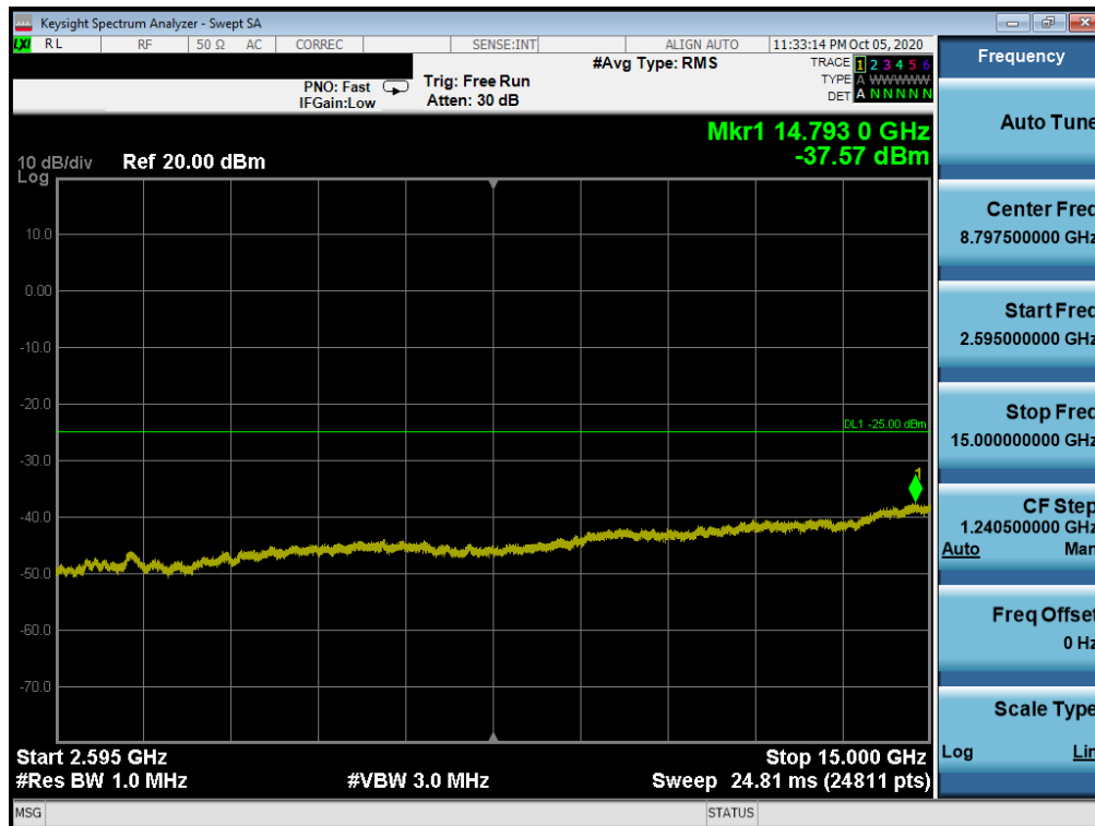
Plot 7-20. Conducted Spurious Plot (LTE Band 7 - 20MHz QPSK - RB Size 1, RB Offset 0 - High Channel)
