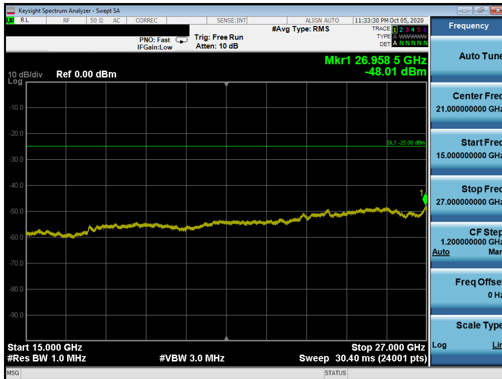
Plot 7-21. Conducted Spurious Plot (LTE Band 7 - 20MHz QPSK - RB Size 1, RB Offset 0 - High Channel)
