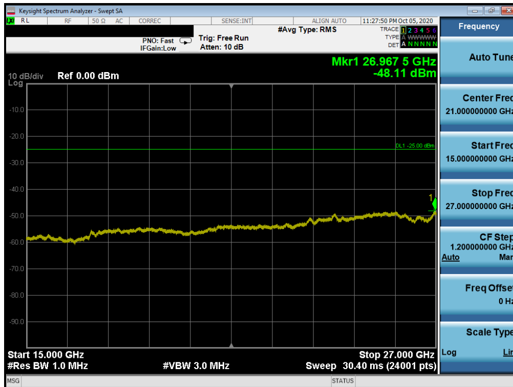
Plot 7-15. Conducted Spurious Plot (LTE Band 7 - 20MHz QPSK - RB Size 1, RB Offset 0 - Low Channel)
