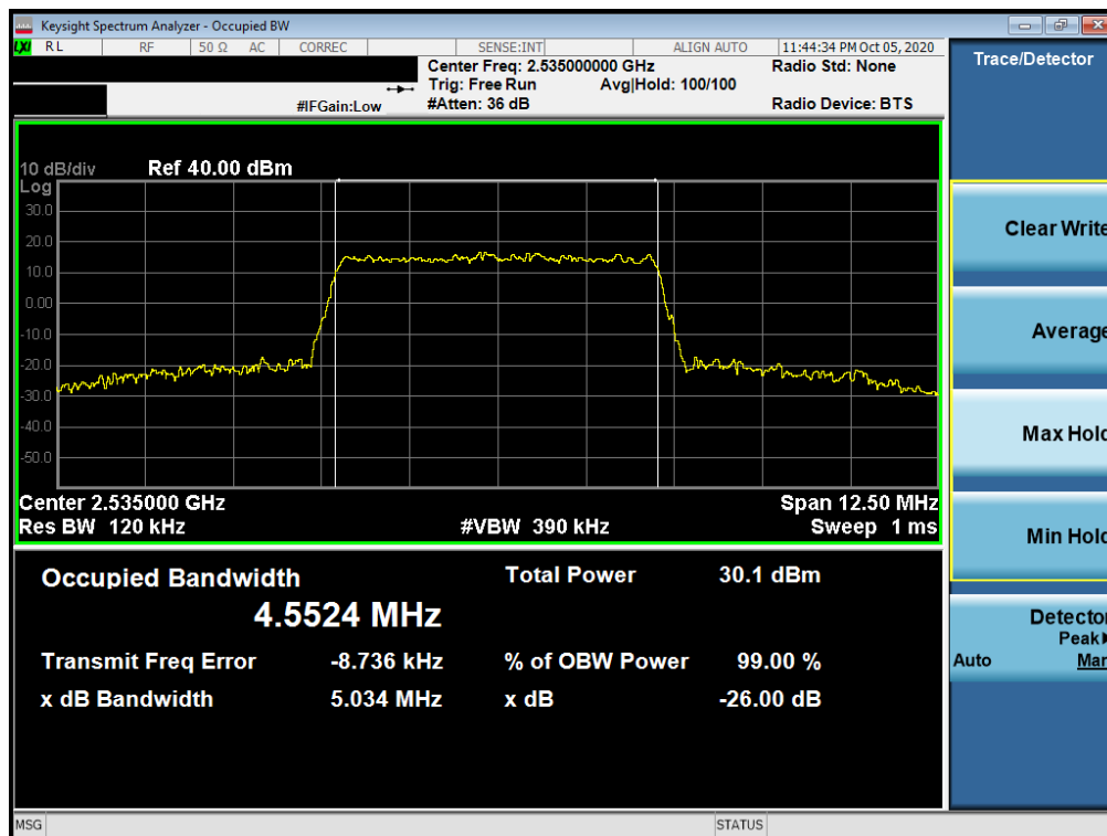
Plot 7-12. Occupied Bandwidth Plot (LTE Band 7 - 5MHz 64-QAM - Full RB Configuration)
