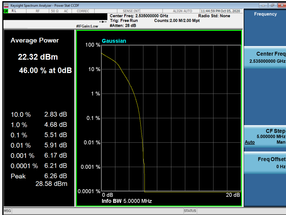
Plot 7-38. PAR Plot (LTE Band 7 - 5MHz 16-QAM - Full RB Configuration)
