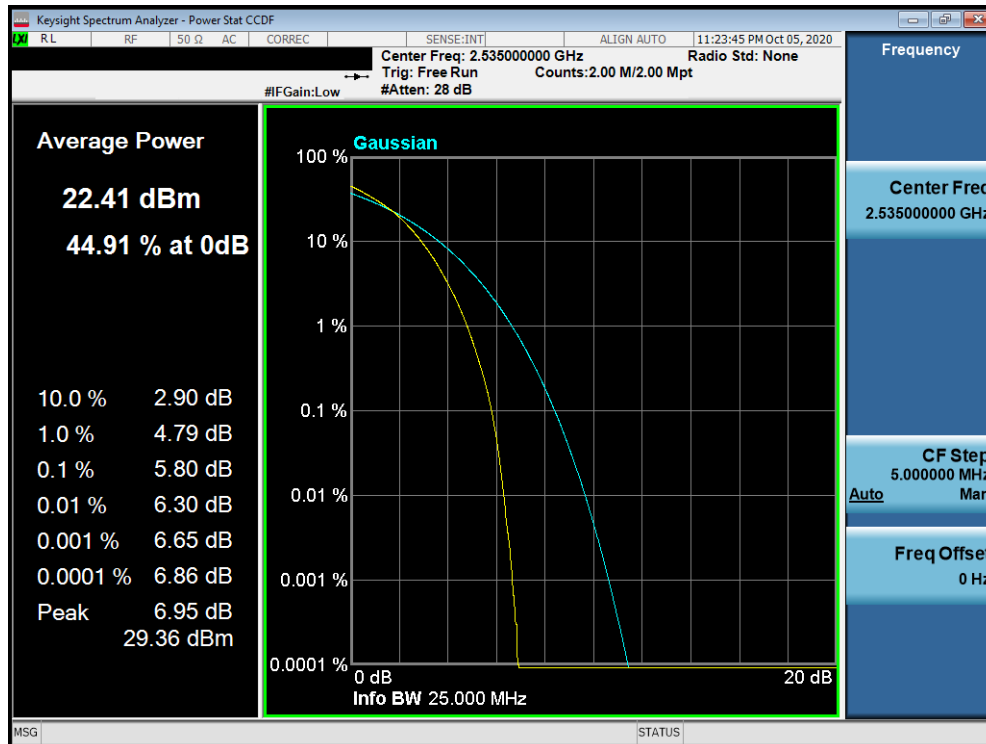
Plot 7-31. PAR Plot (LTE Band 7 - 20MHz 16-QAM - Full RB Configuration)
