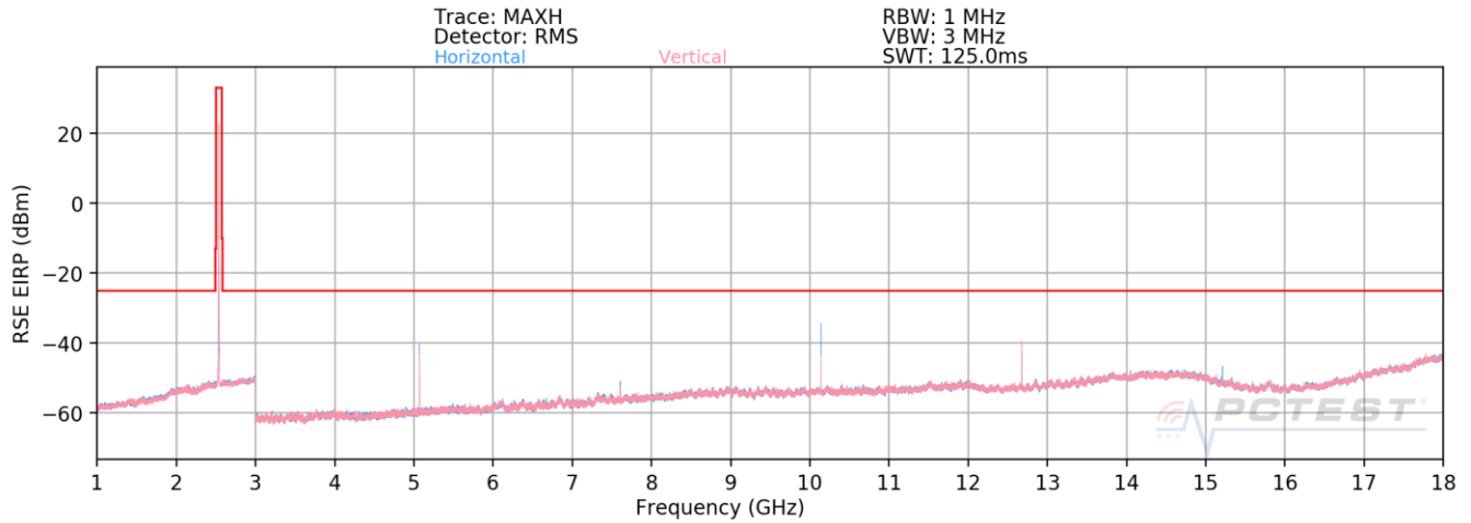
Plot 7-41. Radiated Spurious Plot (LTE Band 7)
