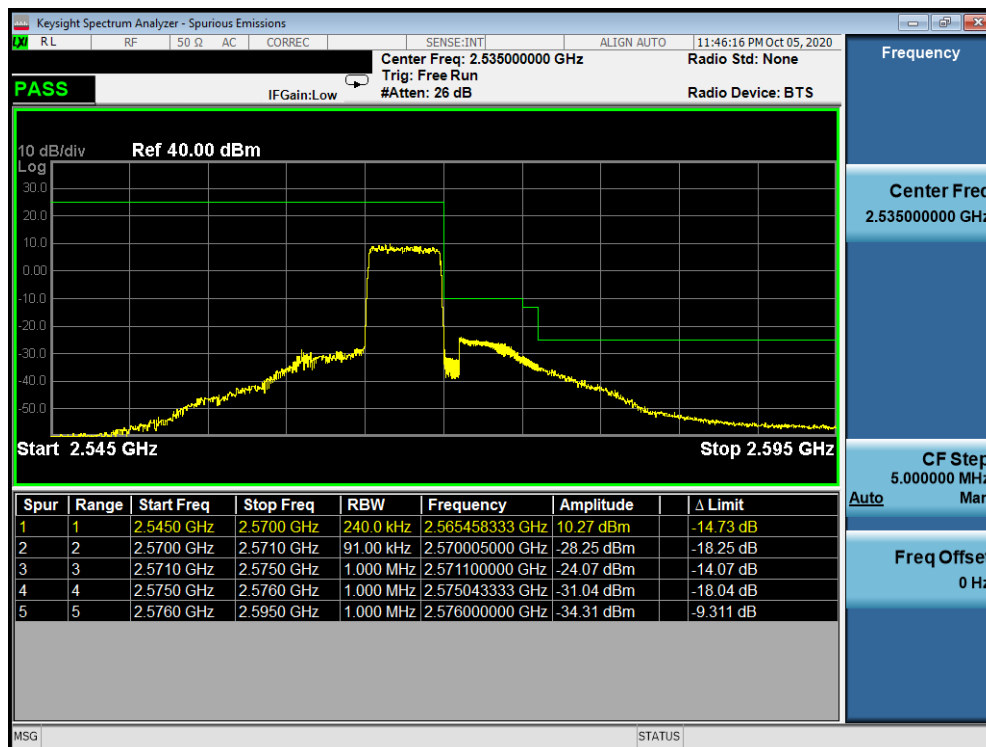
Plot 7-29. Upper ACP Plot (LTE Band 7 - 5MHz QPSK - Full RB Configuration)
