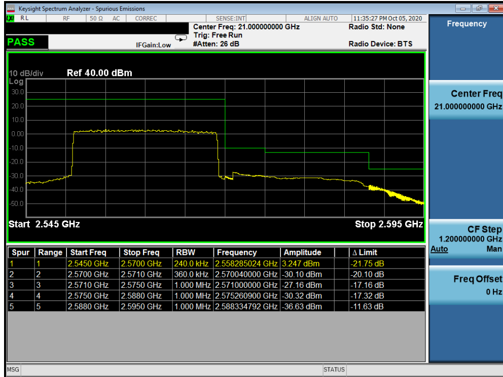
Plot 7-23. Upper ACP Plot (LTE Band 7 - 20MHz QPSK – Full RB Configuration)
