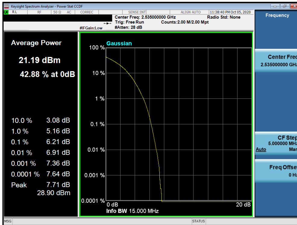
Plot 7 29. PAR Plot (LTE Band 7 - 15MHz 64-QAM - Full RB Configuration)
