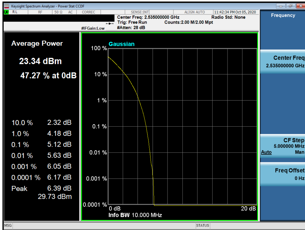
Plot 7-35. PAR Plot (LTE Band 7 - 10MHz QPSK - Full RB Configuration)
