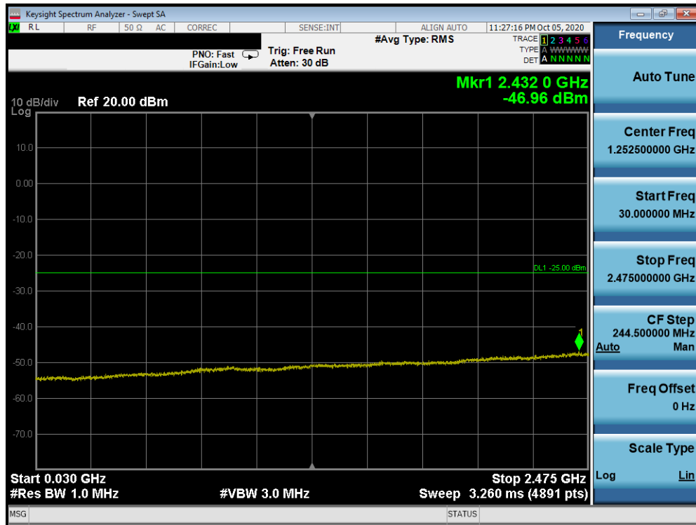
Plot 7-13. Conducted Spurious Plot (LTE Band 7 - 20MHz QPSK - RB Size 1, RB Offset 0 - Low Channel)
