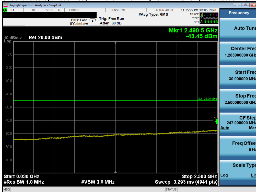
Plot 7-16. Conducted Spurious Plot (LTE Band 7 - 20MHz QPSK - RB Size 1, RB Offset 0 - Mid Channel)
