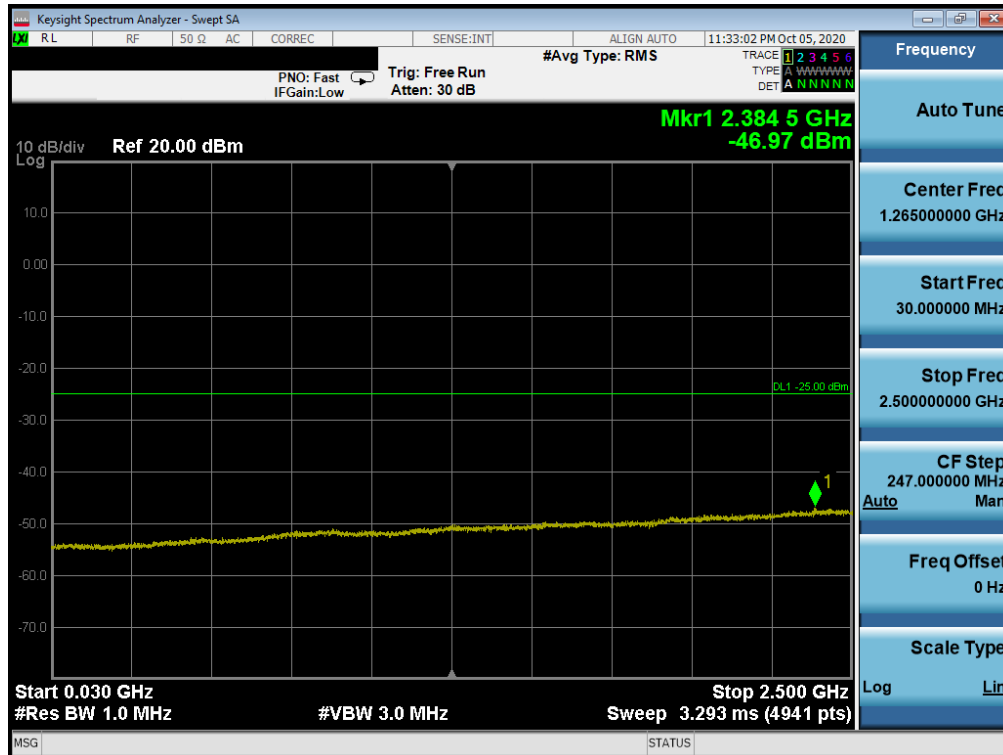
Plot 7-19. Conducted Spurious Plot (LTE Band 7 - 20MHz QPSK - RB Size 1, RB Offset 0 - High Channel)
