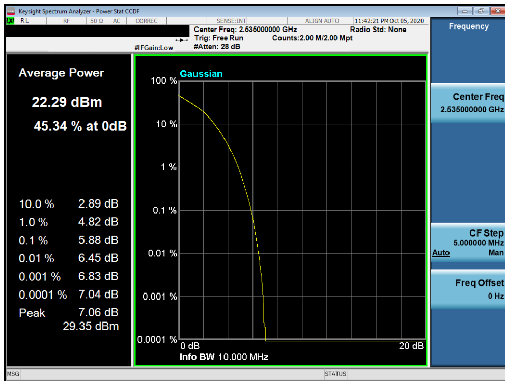
Plot 7-36. PAR Plot (LTE Band 7 - 10MHz 16-QAM - Full RB Configuration)
