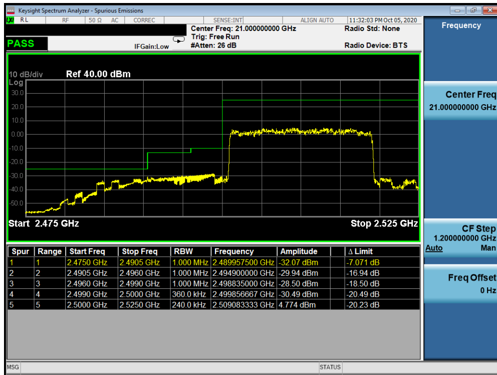
Plot 7-22. Lower ACP Plot (LTE Band 7 - 20MHz QPSK – Full RB Configuration)
