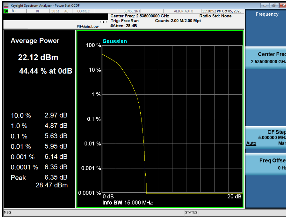
Plot 7-34. PAR Plot (LTE Band 7 - 15MHz 16-QAM - Full RB Configuration)
