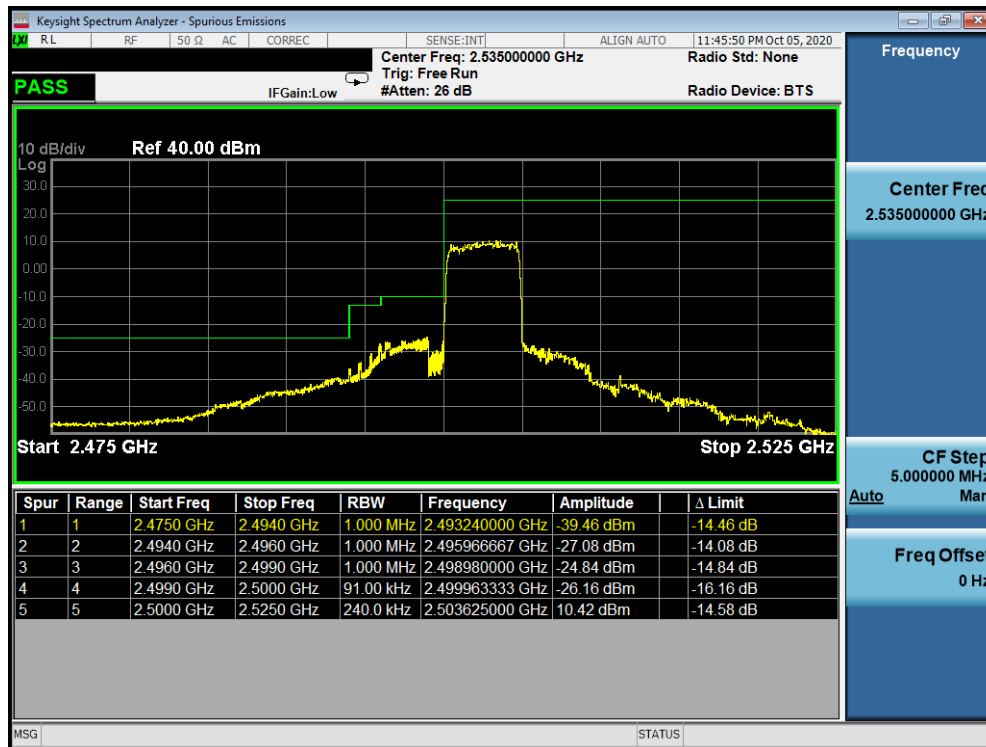
Plot 7-28. Lower ACP Plot (LTE Band 7 - 5MHz QPSK - Full RB Configuration)
