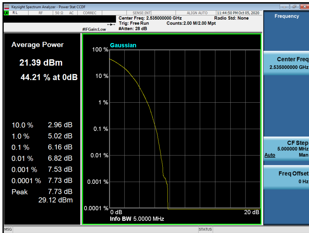
Plot 7-39. PAR Plot (LTE Band 7 - 5MHz 16-QAM - Full RB Configuration)
