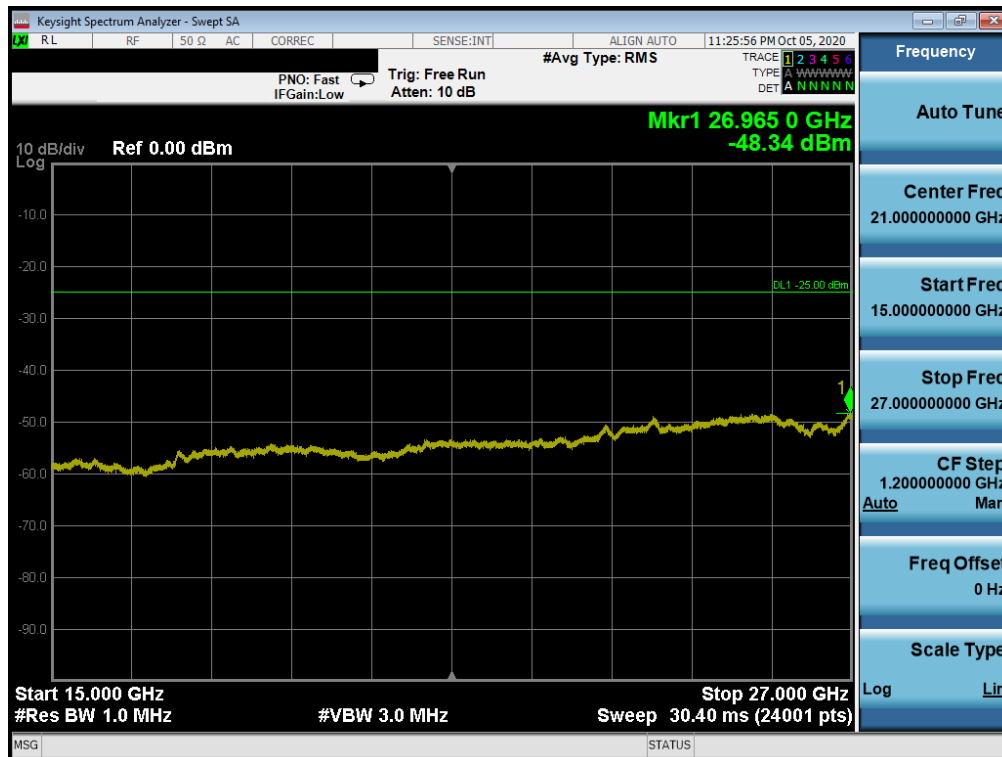
Plot 7-18. Conducted Spurious Plot (LTE Band 7 - 20MHz QPSK - RB Size 1, RB Offset 0 - Mid Channel)
