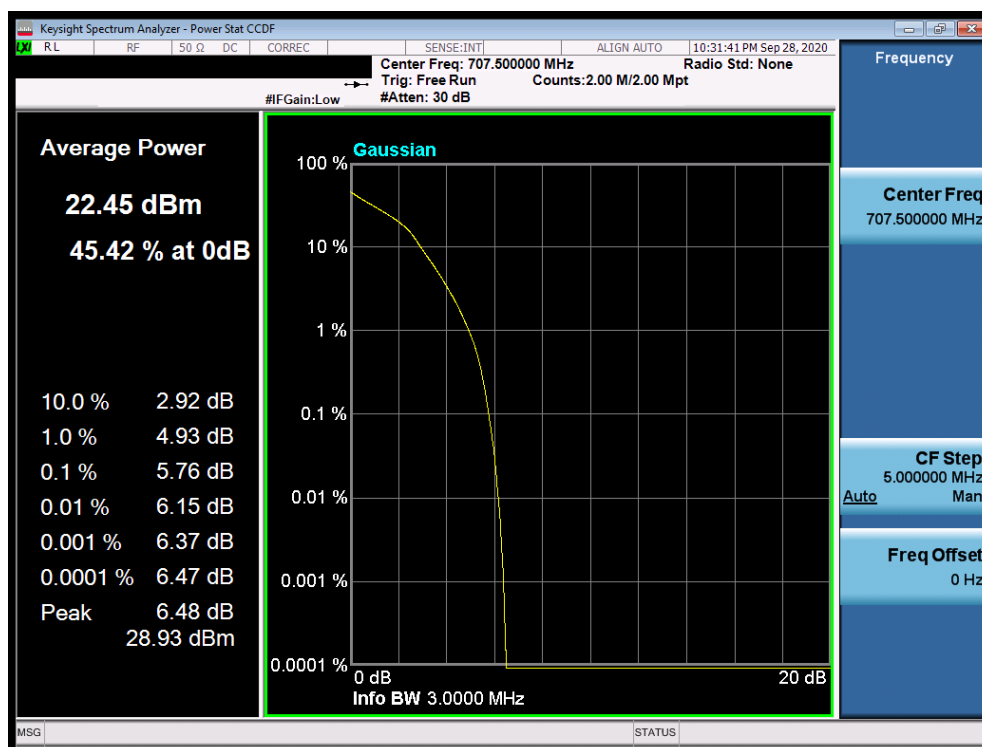
Plot 7-133. PAR Plot (LTE Band 12 - 3MHz 16-QAM - Full RB Configuration)
