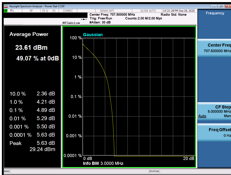
Plot 7-132. PAR Plot (LTE Band 12 - 3MHz QPSK - Full RB Configuration)
