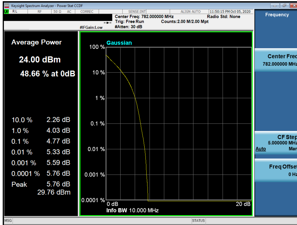
Plot 7-138. PAR Plot (LTE Band 13 – 10MHz QPSK - Full RB Configuration)
