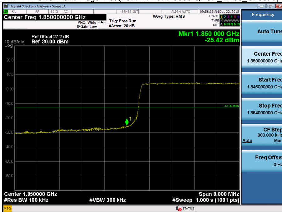
BAND 2. Lower Band Edge Plot (10M BW Ch.18650 QPSK_RB50_Offset 0) -2
