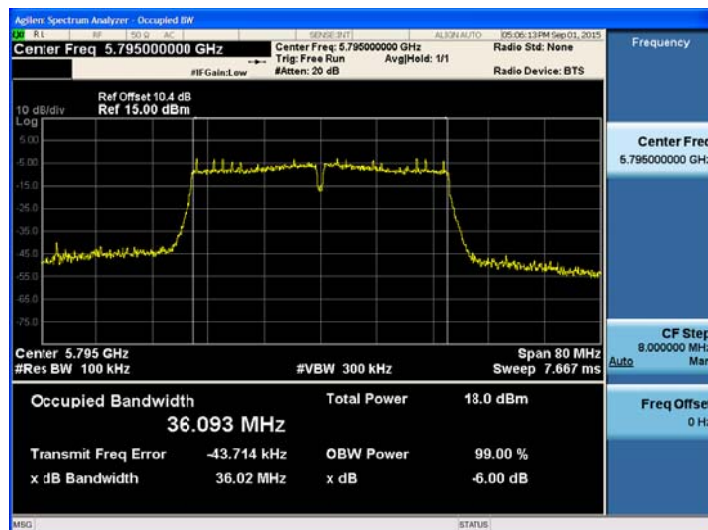
802.11ac_40 MHz BW UNII 3 BAND 6dB Bandwidth(CH.159)
