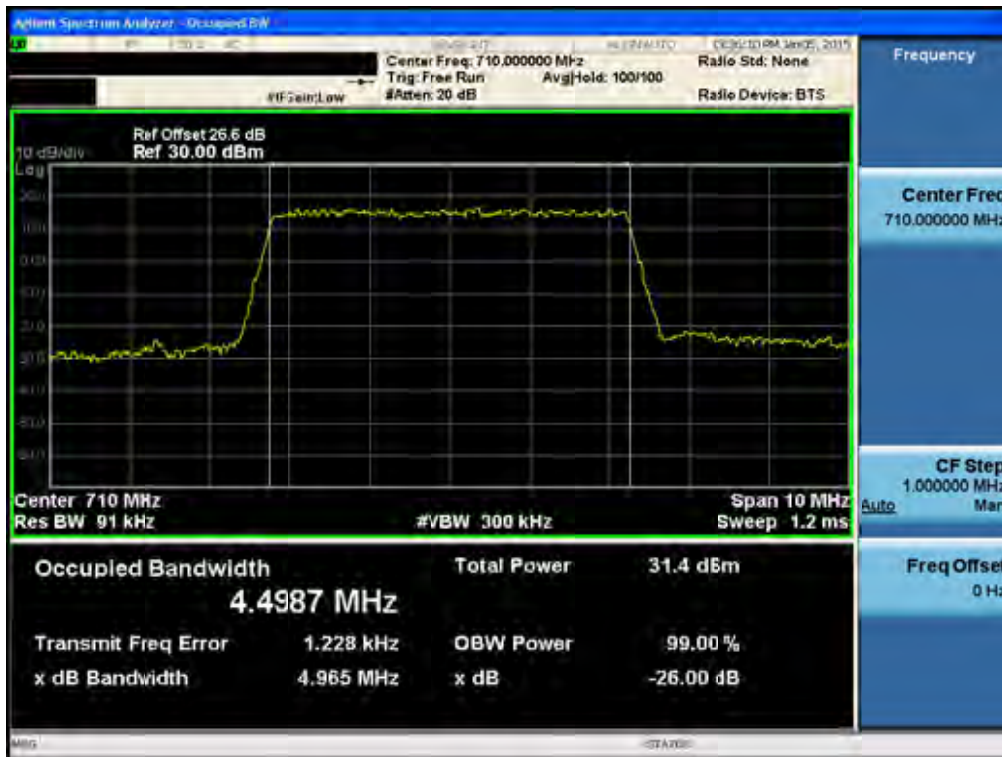
BAND 17. Occupied Bandwidth Plot (5M BW Ch.23790 QPSK RB 25)
