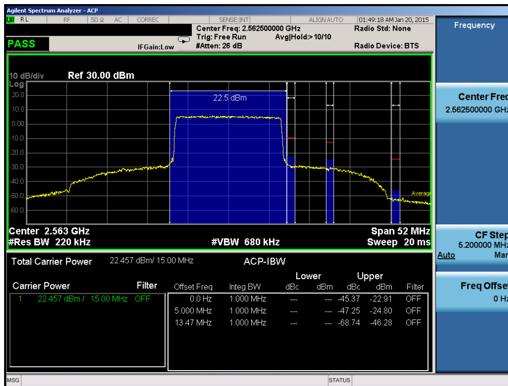
Plot 6-163. Upper ACP Plot (Band 7 – 15.0MHz QPSK – RB Size 75)
