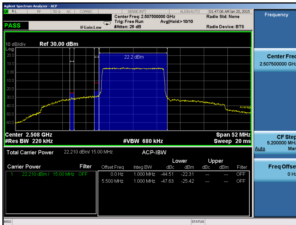
Plot 6-162. Lower ACP Plot (Band 7 – 15.0MHz QPSK – RB Size 75)
