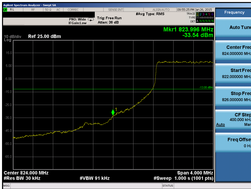
Plot 6-100. Lower Band Edge Plot (Band 5 - 3.0MHz QPSK - RB Size 15)
