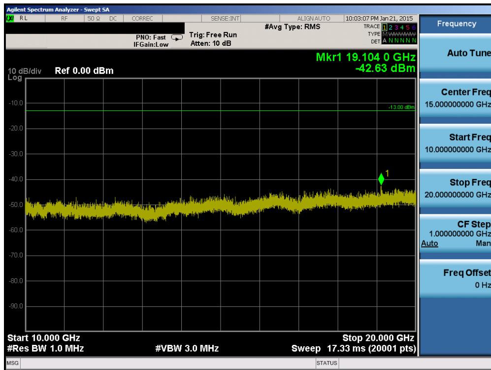
Plot 6-36. Conducted Spurious Plot (PCS WCDMA Mode – Ch. 9538)
