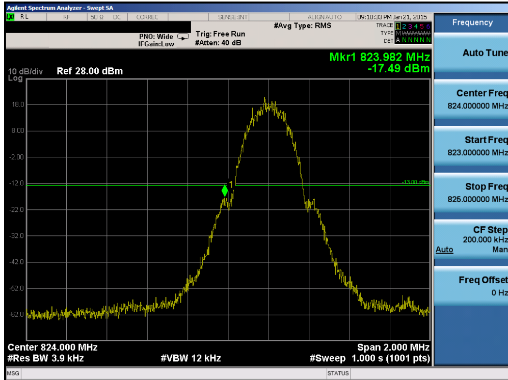
Plot 6-37. Band Edge Plot (Cellular GSM Mode – Ch. 128)
