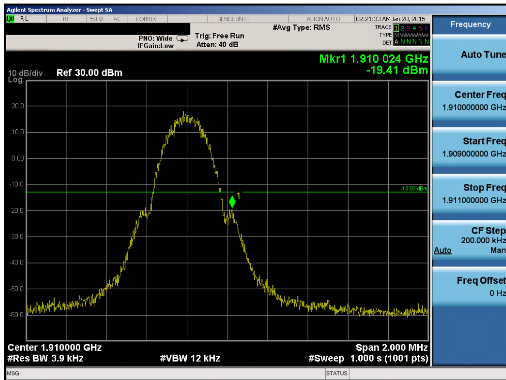
Plot 6-40. Band Edge Plot (PCS GSM Mode – Ch. 810)
