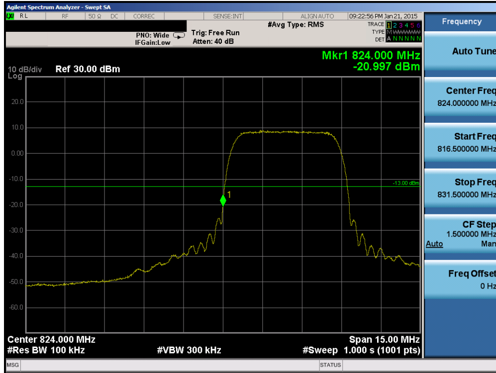
Plot 6-41. Band Edge Plot (Cellular WCDMA Mode – Ch. 4132)
