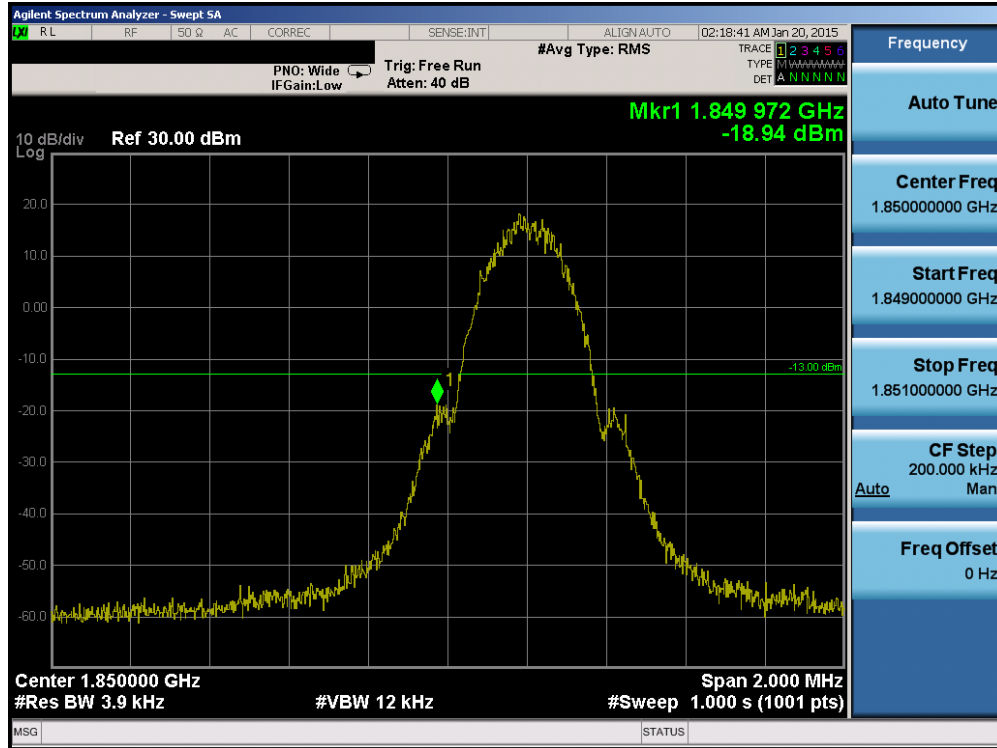
Plot 6-39. Band Edge Plot (PCS GSM Mode – Ch. 512)
