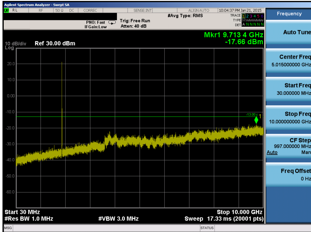
Plot 6-33. Conducted Spurious Plot (PCS WCDMA Mode – Ch. 9400)
