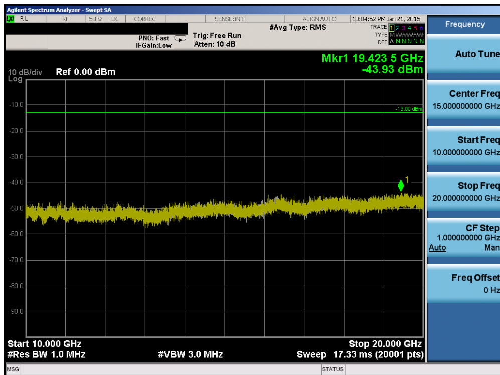
Plot 6-34. Conducted Spurious Plot (PCS WCDMA Mode – Ch. 9400)
