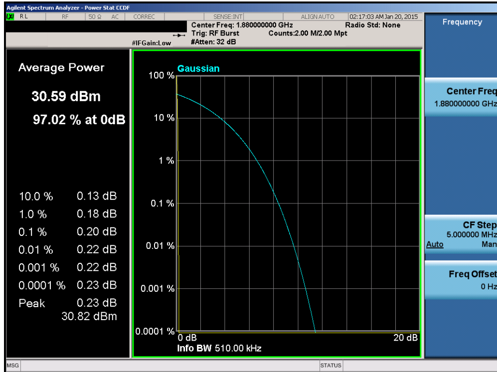
Plot 6-45. Peak-Average Ratio Plot (PCS GSM Mode – Ch. 661)
