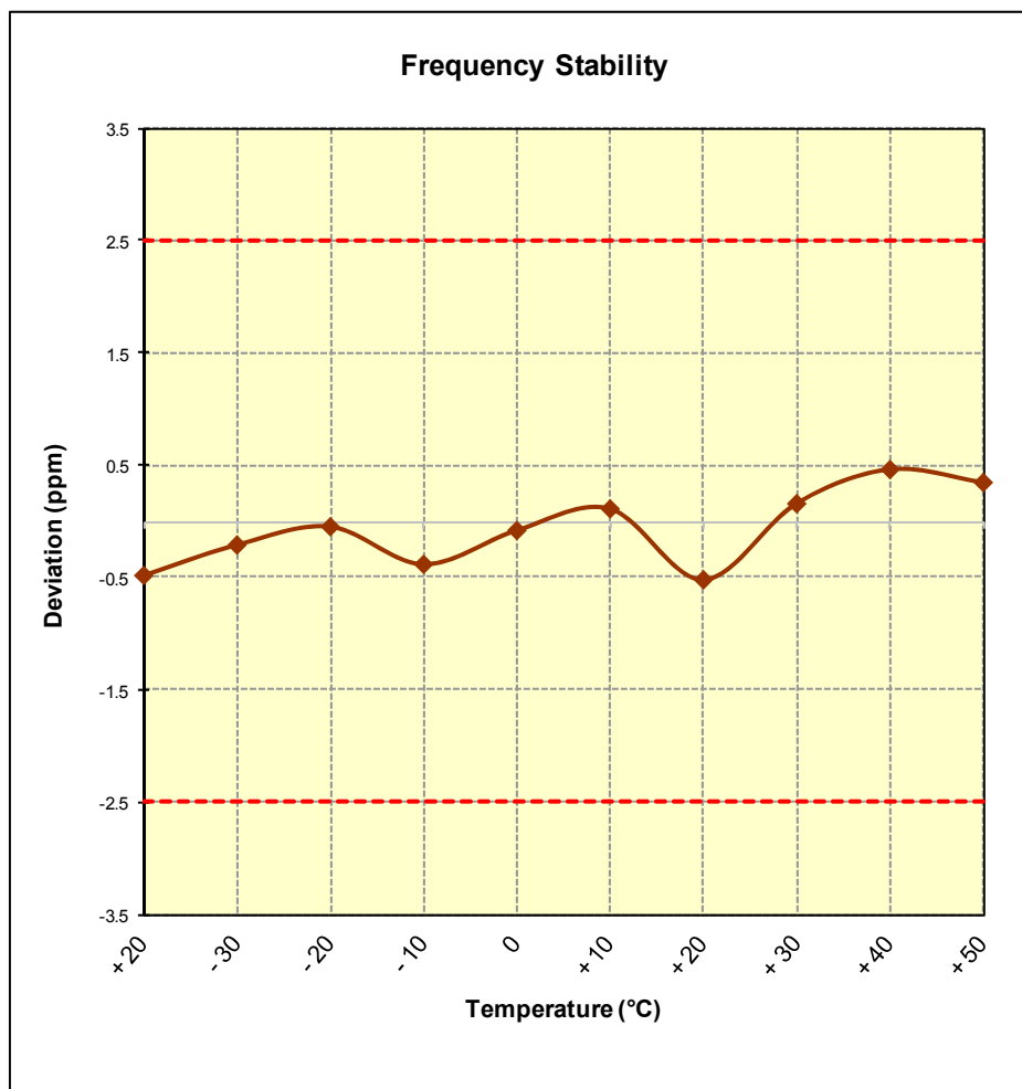
Figure 6-7. Frequency Stability Graph (Cellular GSM Mode – Ch. 190)
