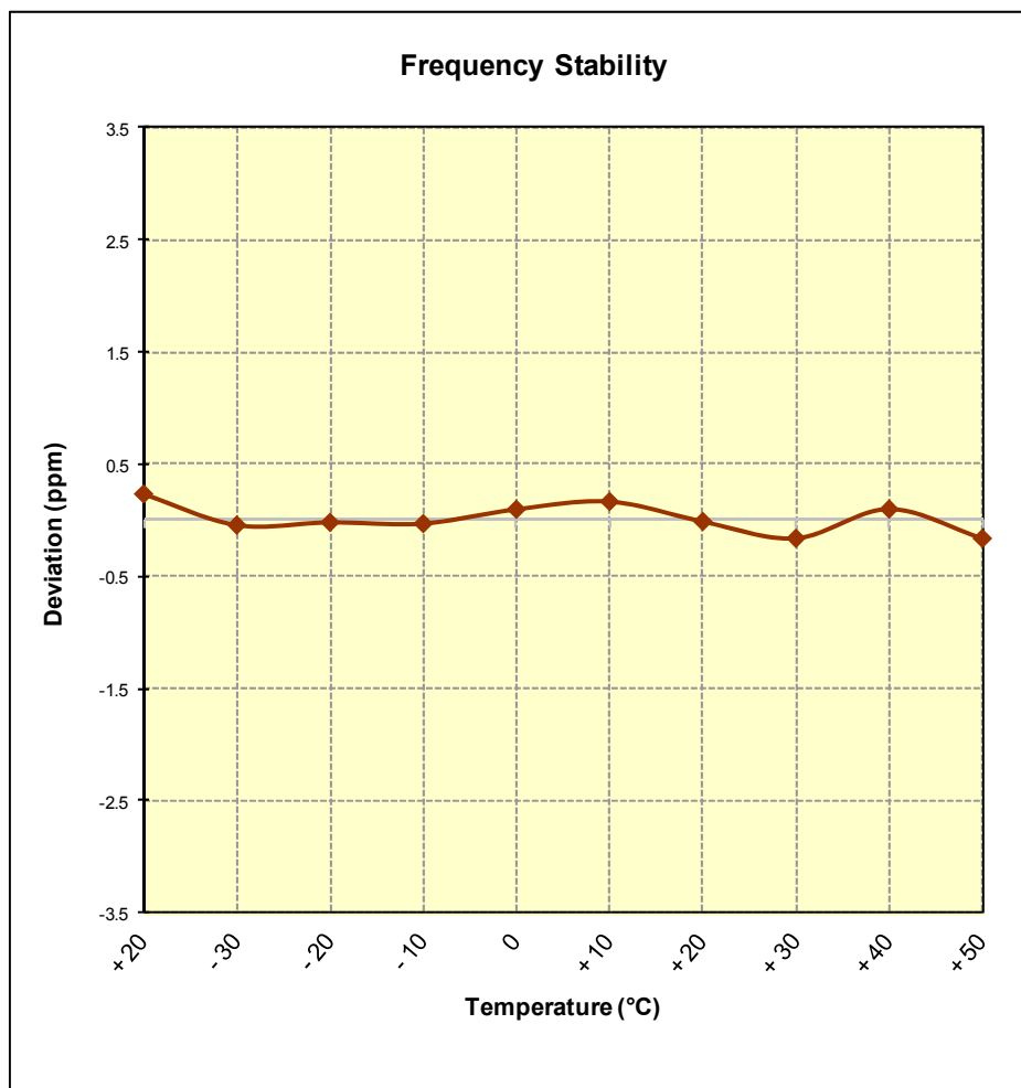
Figure 6-10. Frequency Stability Graph (PCS WCDMA Mode – Ch. 9400)
