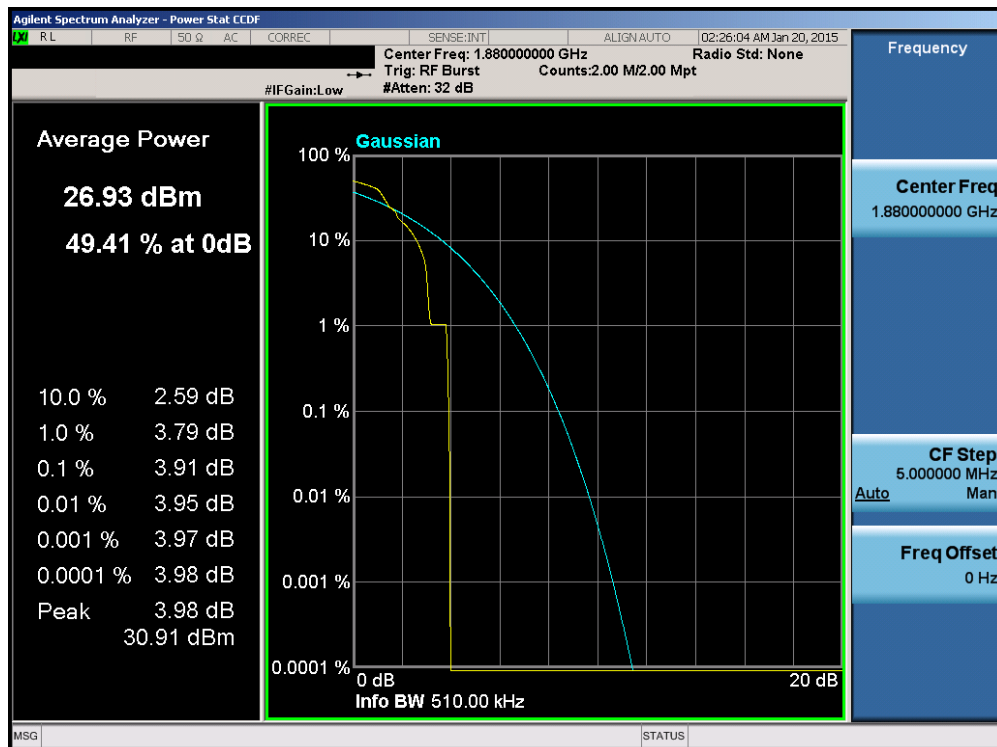
Plot 6-46. Peak-Average Ratio Plot (EDGE1900 Mode – Ch. 661)
