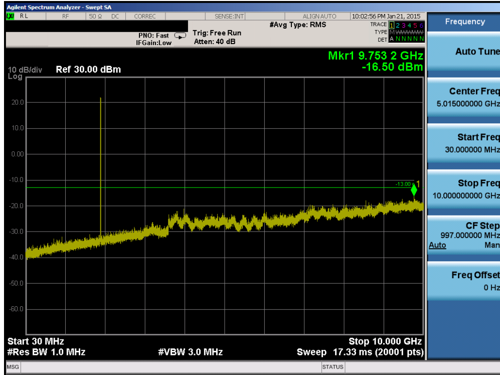
Plot 6-35. Conducted Spurious Plot (PCS WCDMA Mode – Ch. 9538)
