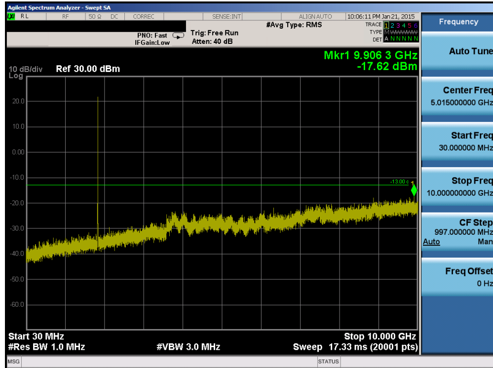
Plot 6-31. Conducted Spurious Plot (PCS WCDMA Mode – Ch. 9262)
