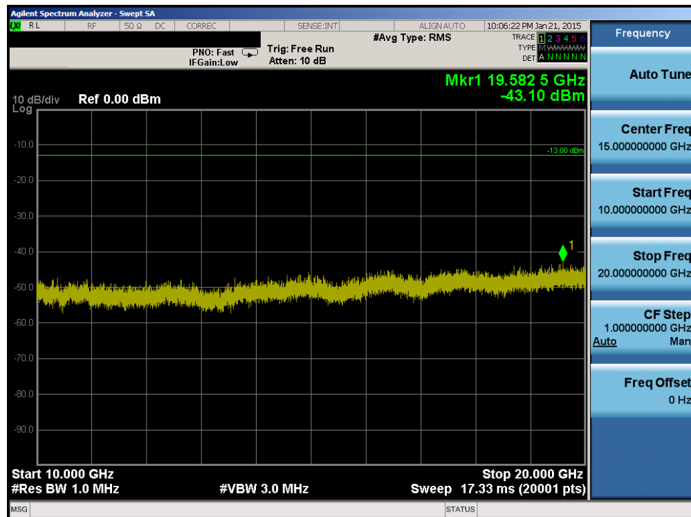
Plot 6-32. Conducted Spurious Plot (PCS WCDMA Mode – Ch. 9262)
