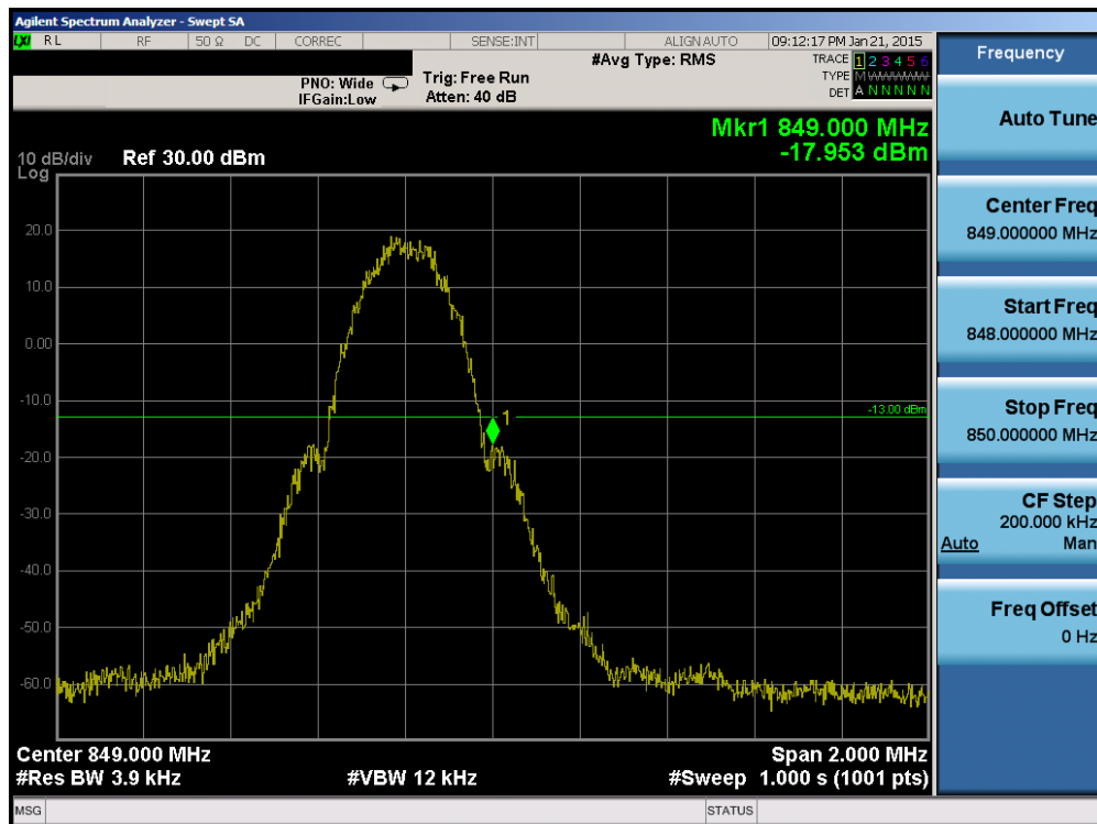
Plot 6-38. Band Edge Plot (Cellular GSM Mode – Ch. 251)
