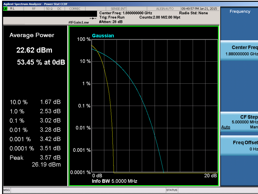
Plot 6-47. Peak-Average Ratio Plot (PCS WCDMA Mode – Ch. 9400)
