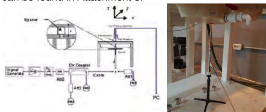
Figure 11.1 Dipole Verification Test Setup Diagram &amp; Photo
