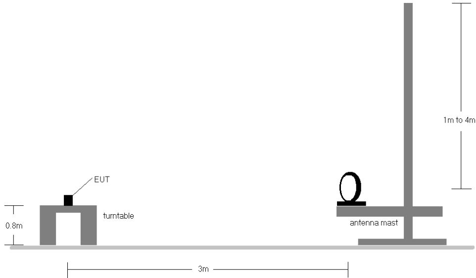
Figure 8-1. Radiated Test Setup
