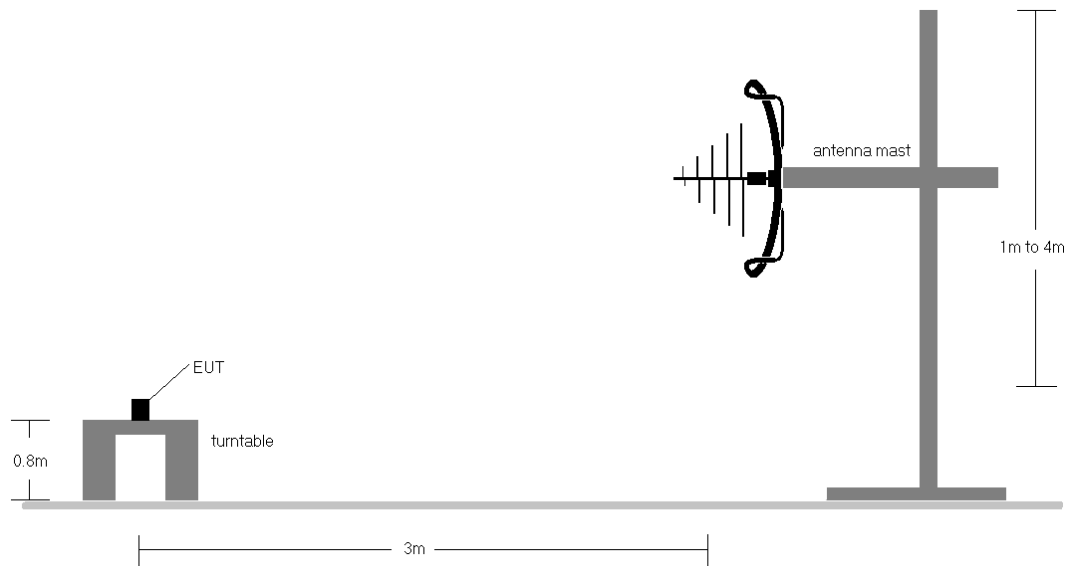
Figure 8-3. Radiated Test Setup > 30MHz
