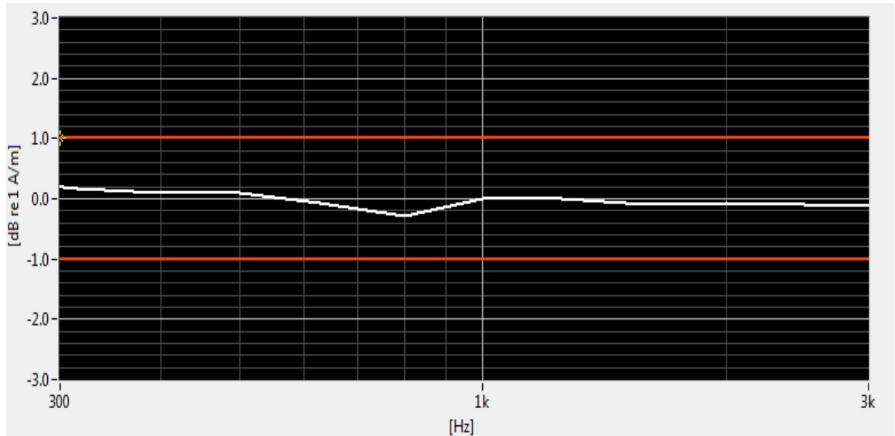
Figure 7-4 Helmholtz Coil Validation for Frequency Response
