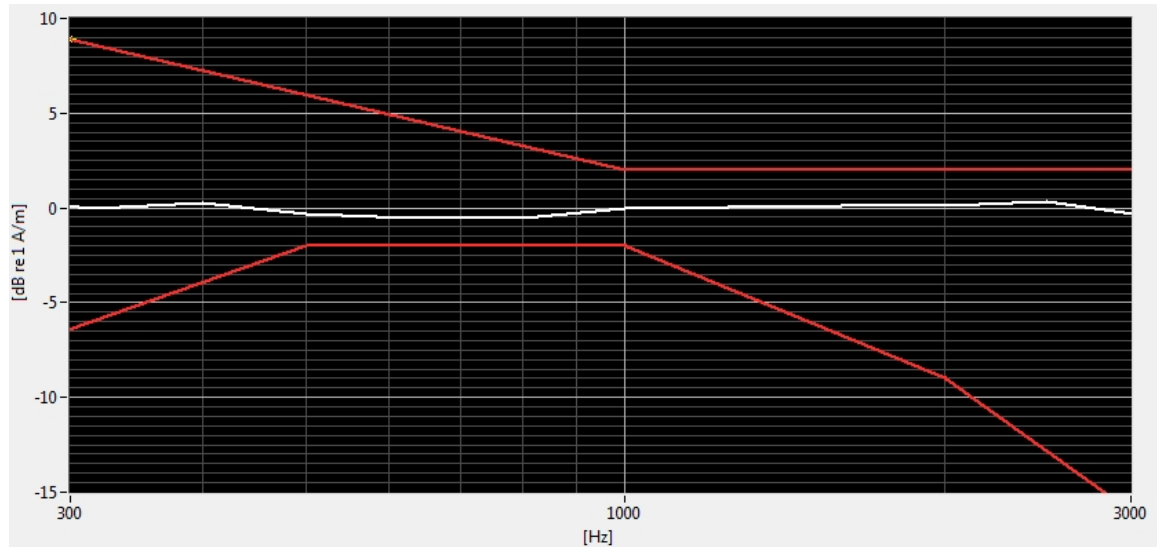
Figure 7-1 Axial Frequency Response
