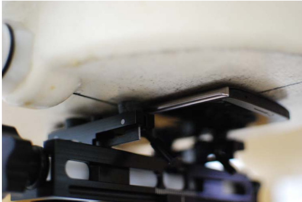
SAR Test Setup Photo 10: Back Side at 0.0 cm with Wireless Charging Cover
