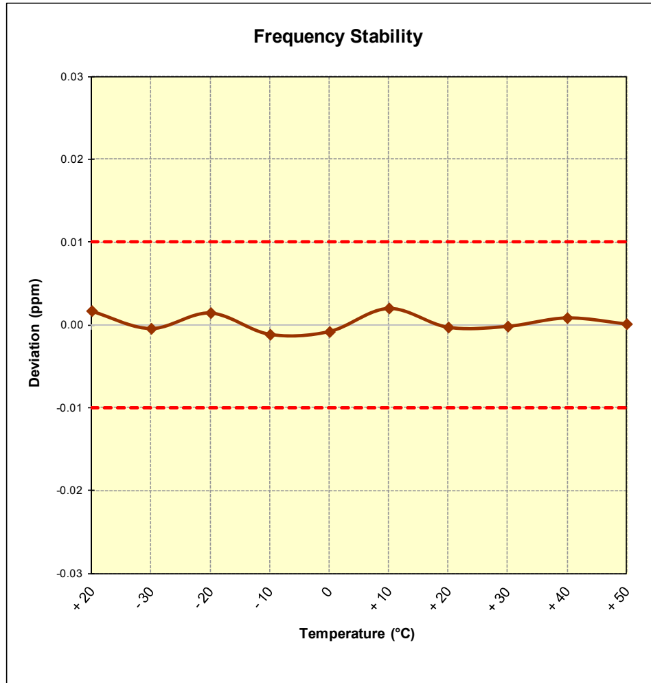
Figure 7-5. Frequency Stability Plot
