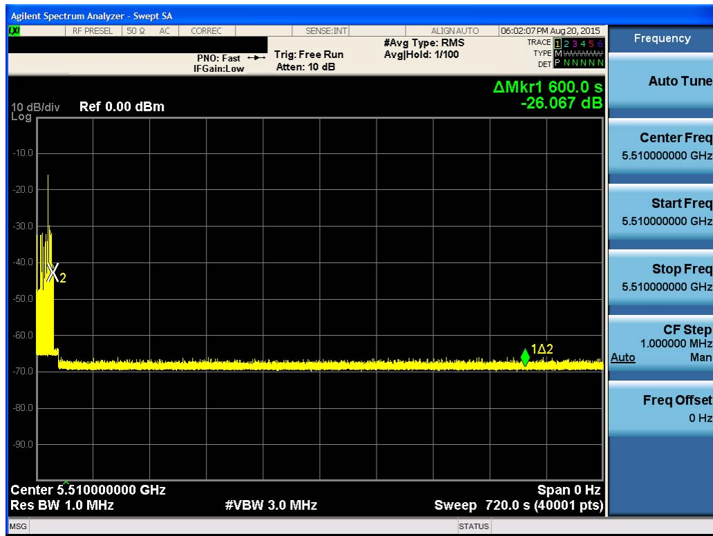
Figure 5-8. Band 2C Client Beacon Test – Monitoring live spectrum – Elapsed time 10 minutes
