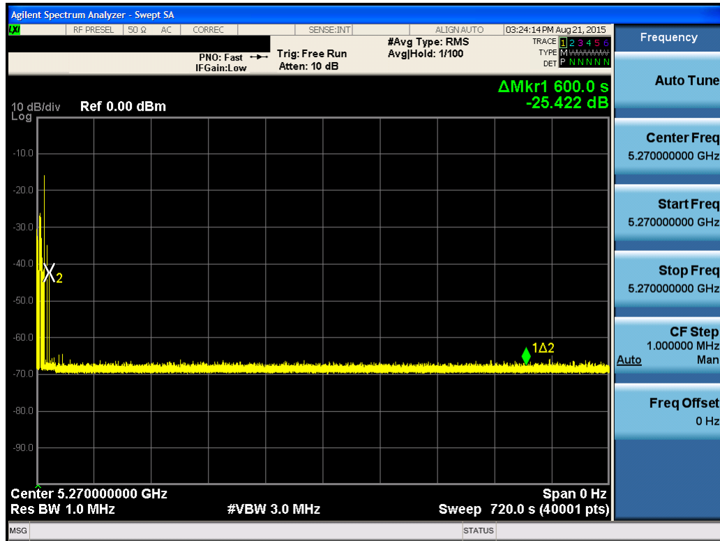
Figure 5-7. Band 2A Client Beacon Test – Monitoring live spectrum – Elapsed time 10 minutes
