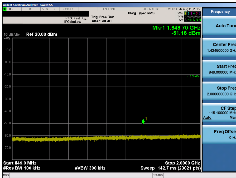
Plot 6-55. Conducted Spurious Plot (Band 5 – 5.0MHz QPSK – RB Size 1, RB Offset 0 – Low Channel)
