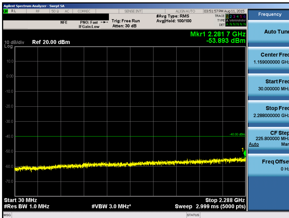
Plot 6-78. Conducted Spurious Plot (Band 30 – 10.0MHz QPSK – RB Size 1, RB Offset 0 – Mid Channel)
