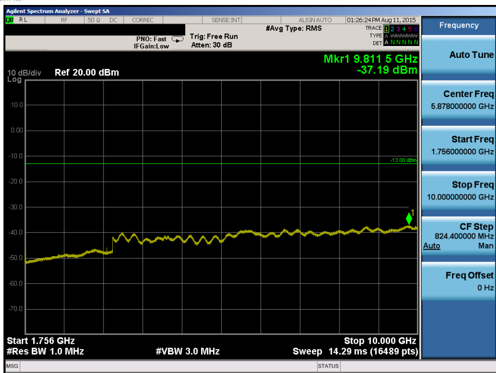
Plot 6-67. Conducted Spurious Plot (Band 4 – 20.0MHz QPSK – RB Size 1, RB Offset 0 – High Channel)
