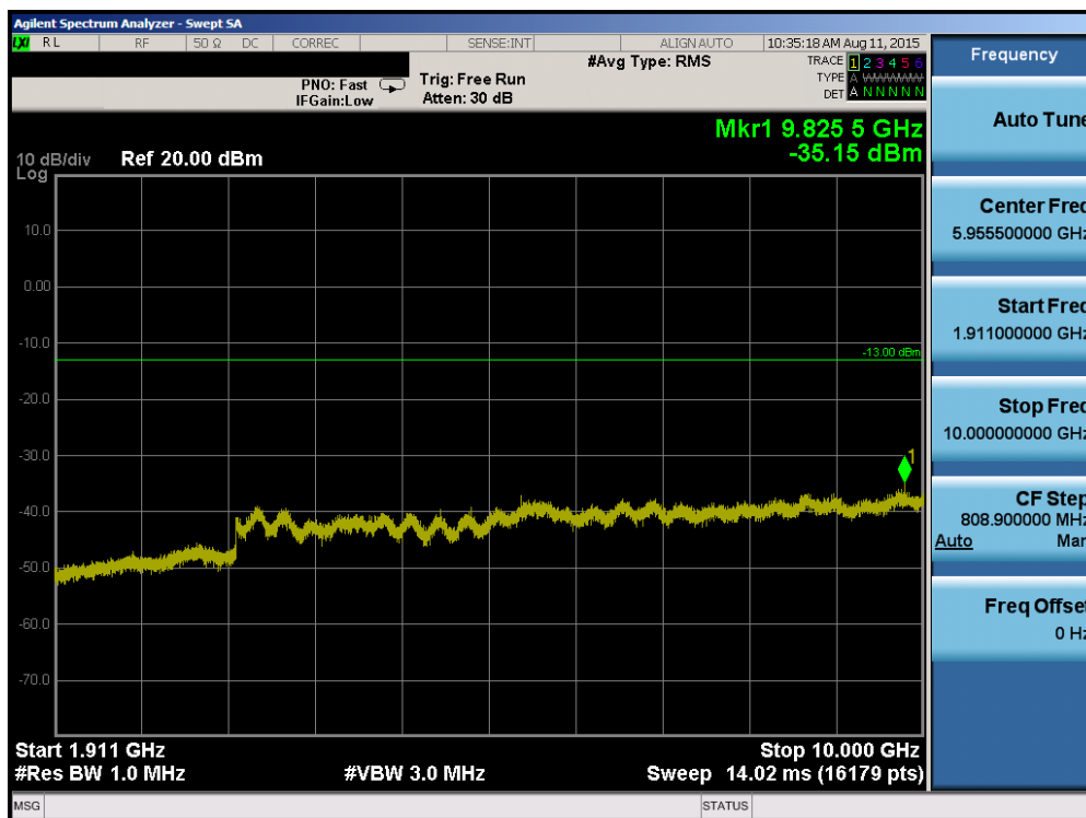
Plot 6-76. Conducted Spurious Plot (Band 2 – 20.0MHz QPSK – RB Size 1, RB Offset 0 – High Channel)
