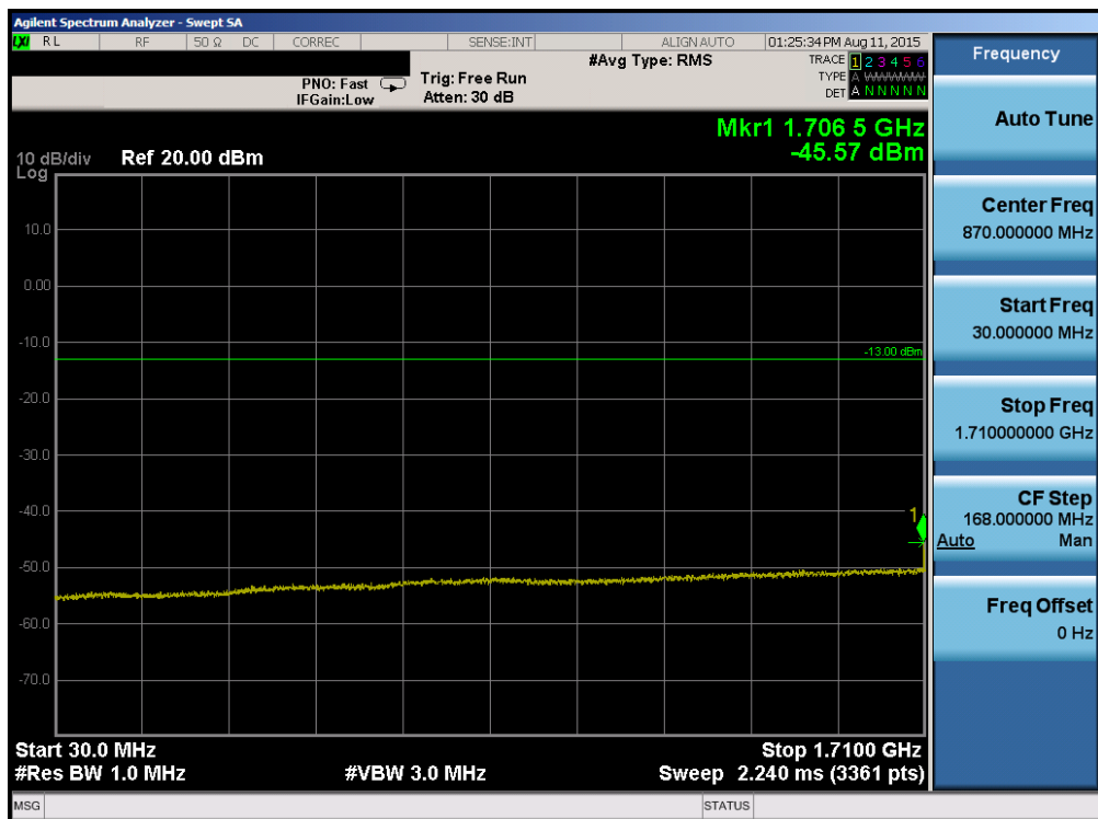
Plot 6-66. Conducted Spurious Plot (Band 4 – 20.0MHz QPSK – RB Size 1, RB Offset 0 – High Channel)
