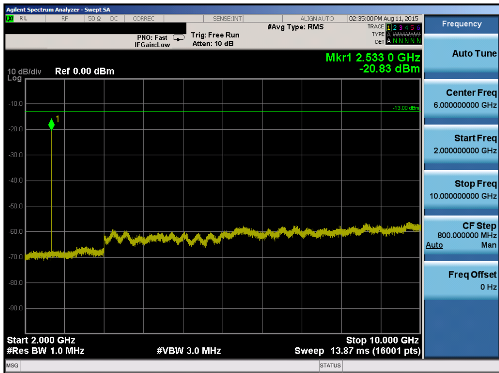
Plot 6-62. Conducted Spurious Plot (Band 5 – 5.0MHz QPSK – RB Size 1, RB Offset 0 – High Channel)
