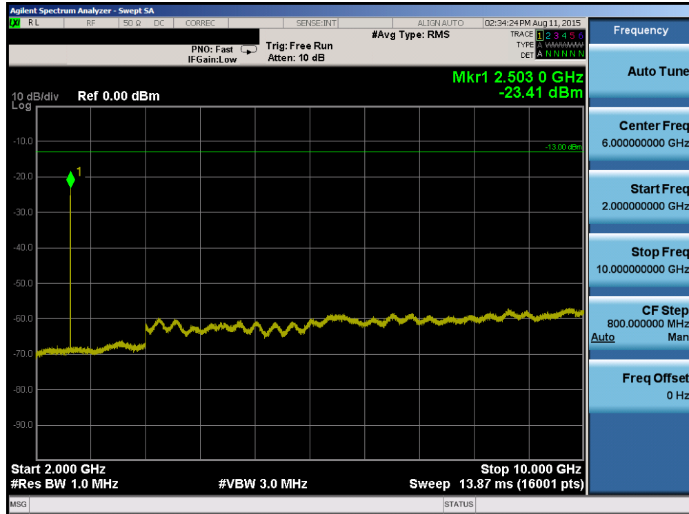
Plot 6-59. Conducted Spurious Plot (Band 5 – 5.0MHz QPSK – RB Size 1, RB Offset 0 – Mid Channel)
