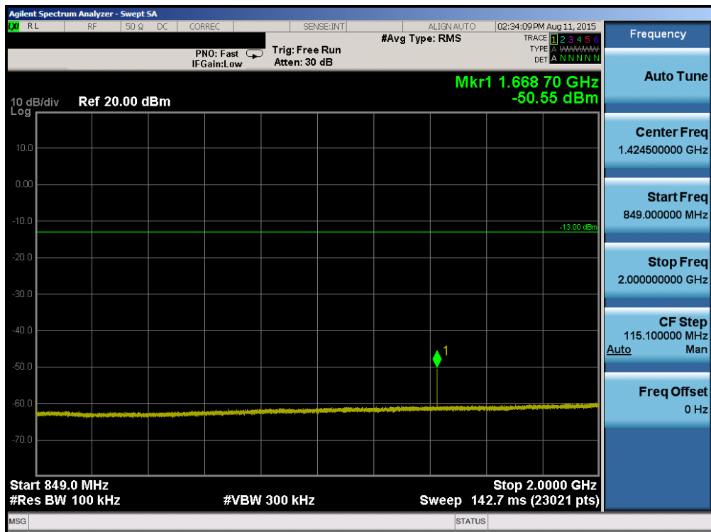
Plot 6-58. Conducted Spurious Plot (Band 5 – 5.0MHz QPSK – RB Size 1, RB Offset 0 – Mid Channel)
