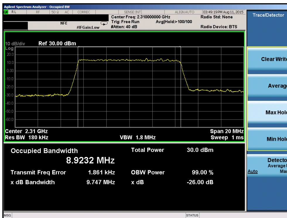
Plot 6-44. Occupied Bandwidth Plot (Band 30 – 10.0MHz 16-QAM – RB Size 50)
