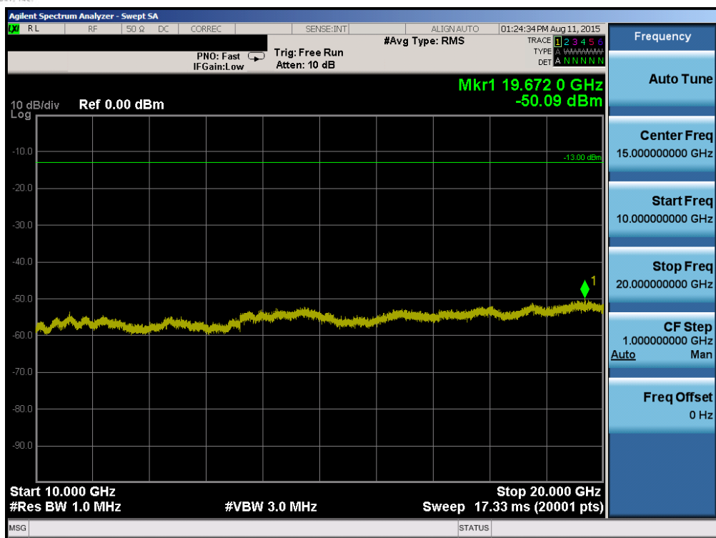
Plot 6-65. Conducted Spurious Plot (Band 4 – 20.0MHz QPSK – RB Size 1, RB Offset 0 – Low Channel)
