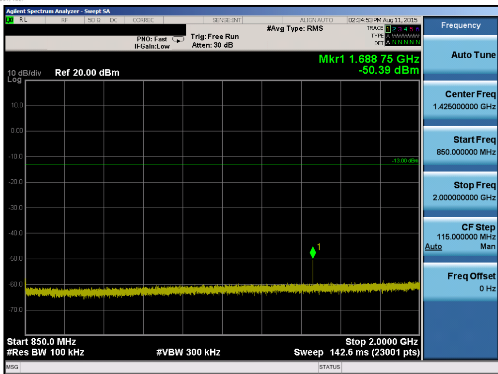
Plot 6-61. Conducted Spurious Plot (Band 5 – 5.0MHz QPSK – RB Size 1, RB Offset 0 – High Channel)
