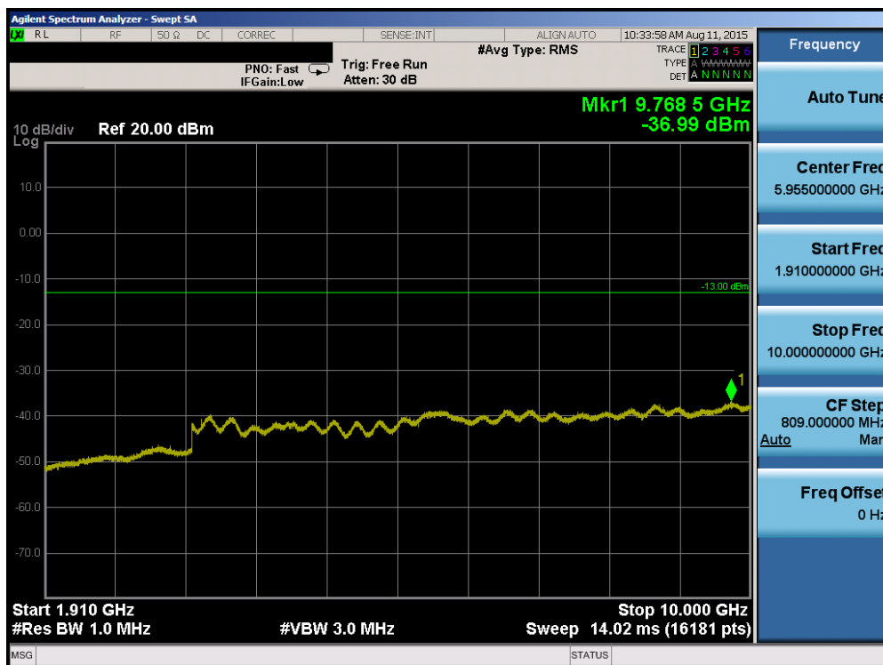
Plot 6-70. Conducted Spurious Plot (Band 2 – 20.0MHz QPSK – RB Size 1, RB Offset 0 – Low Channel)
