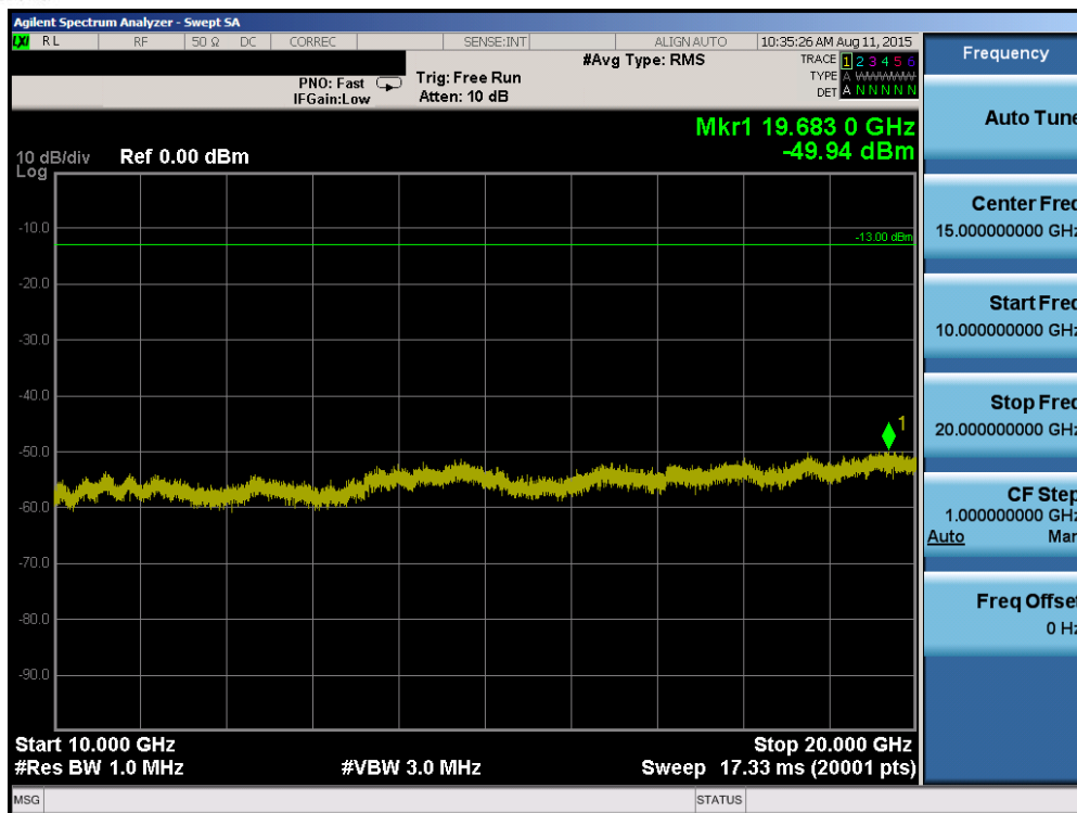
Plot 6-77. Conducted Spurious Plot (Band 2 – 20.0MHz QPSK – RB Size 1, RB Offset 0 – High Channel)
