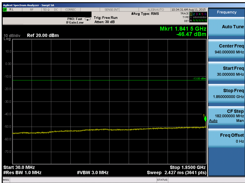
Plot 6-72. Conducted Spurious Plot (Band 2 – 20.0MHz QPSK – RB Size 1, RB Offset 0 – Mid Channel)
