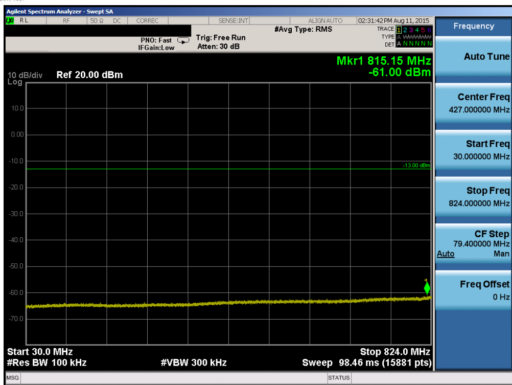
Plot 6-57. Conducted Spurious Plot (Band 5 – 5.0MHz QPSK – RB Size 1, RB Offset 0 – Mid Channel)
