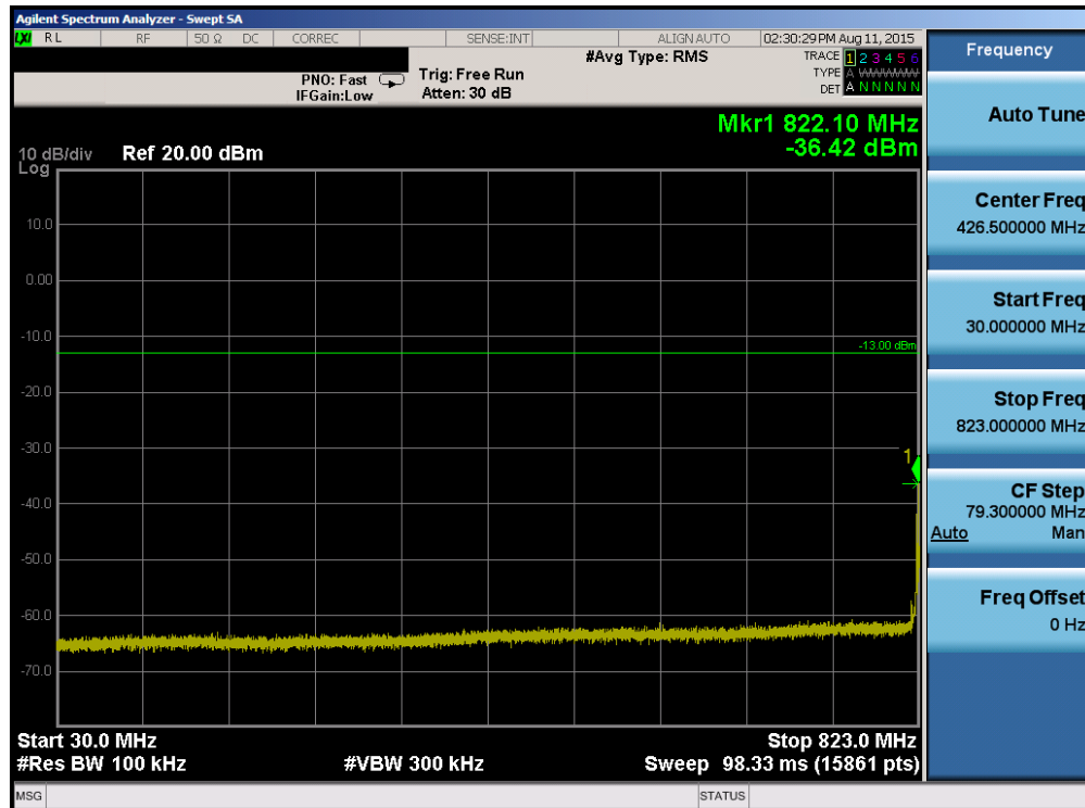
Plot 6-54. Conducted Spurious Plot (Band 5 – 5.0MHz QPSK – RB Size 1, RB Offset 0 – Low Channel)
