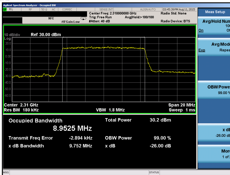
Plot 6-43. Occupied Bandwidth Plot (Band 30 – 10.0MHz QPSK – RB Size 50)
