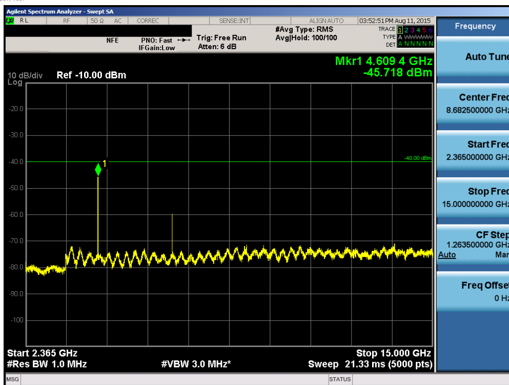
Plot 6-79. Conducted Spurious Plot (Band 30 – 10.0MHz QPSK – RB Size 1, RB Offset 0 – Mid Channel)
