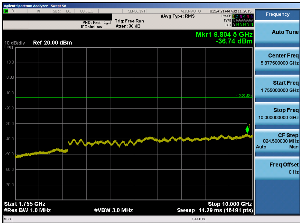
Plot 6-64. Conducted Spurious Plot (Band 4 – 20.0MHz QPSK – RB Size 1, RB Offset 0 – Low Channel)
