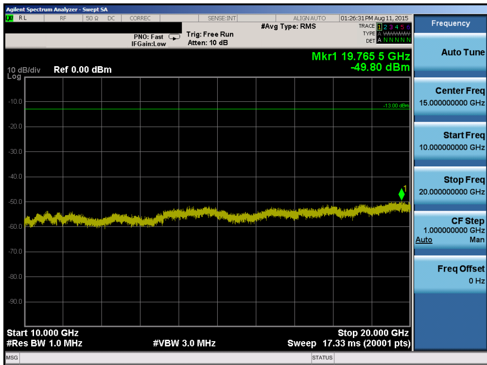
Plot 6-68. Conducted Spurious Plot (Band 4 – 20.0MHz QPSK – RB Size 1, RB Offset 0 – High Channel)
