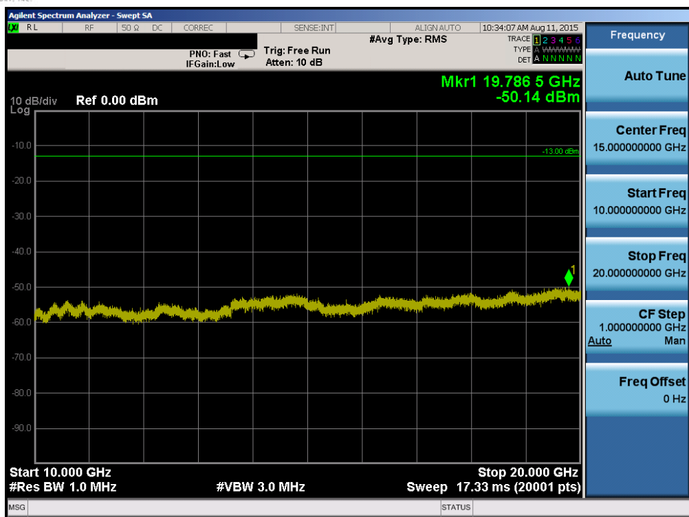
Plot 6-71. Conducted Spurious Plot (Band 2 – 20.0MHz QPSK – RB Size 1, RB Offset 0 – Low Channel)
