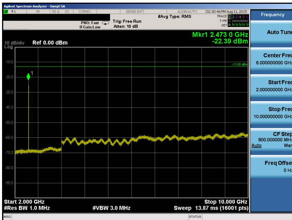
Plot 6-56. Conducted Spurious Plot (Band 5 – 5.0MHz QPSK – RB Size 1, RB Offset 0 – Low Channel)
