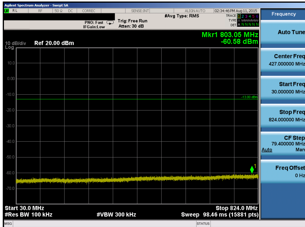
Plot 6-60. Conducted Spurious Plot (Band 5 – 5.0MHz QPSK – RB Size 1, RB Offset 0 – High Channel)
