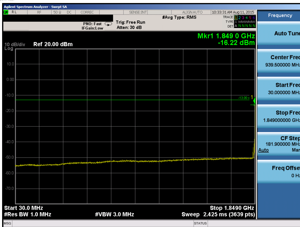
Plot 6-69. Conducted Spurious Plot (Band 2 – 20.0MHz QPSK – RB Size 1, RB Offset 0– Low Channel)
