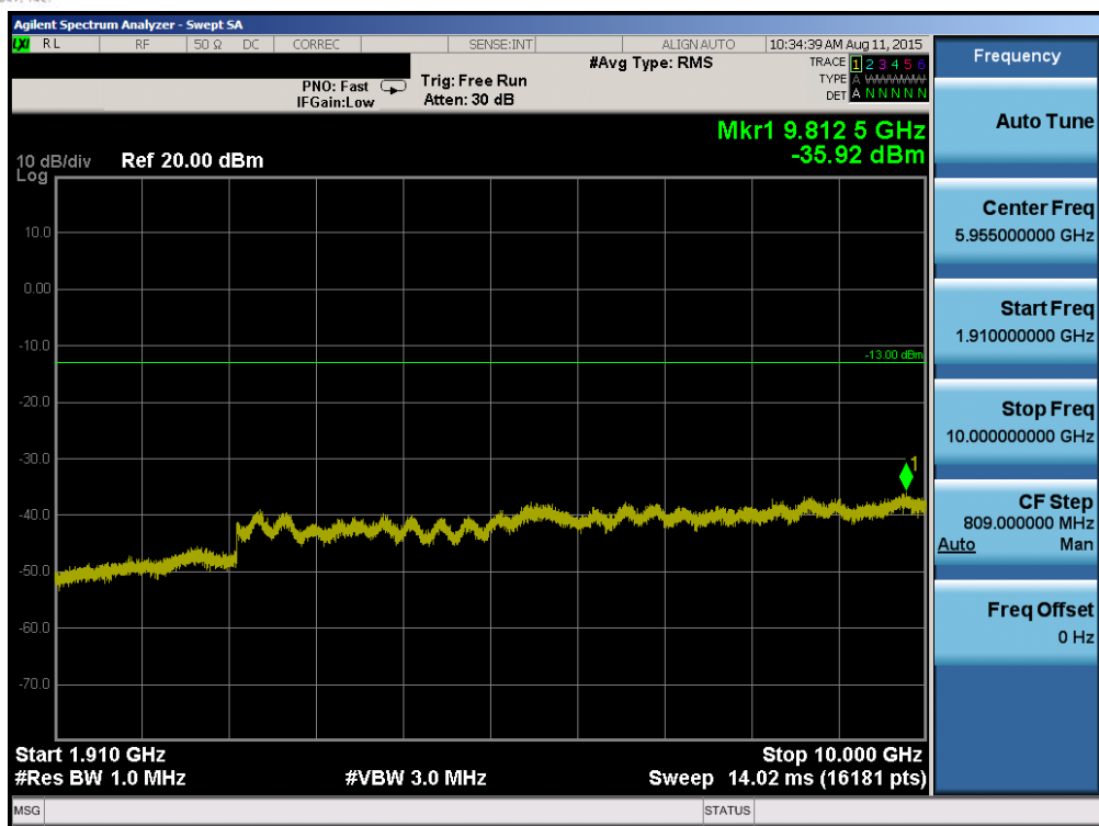
Plot 6-73. Conducted Spurious Plot (Band 2 – 20.0MHz QPSK – RB Size 1, RB Offset 0 – Mid Channel)
