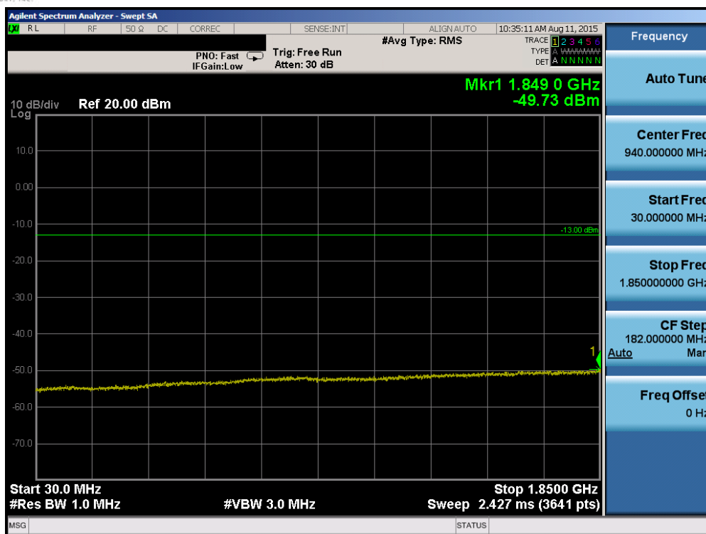
Plot 6-75. Conducted Spurious Plot (Band 2 – 20.0MHz QPSK – RB Size 1, RB Offset 0 – High Channel)
