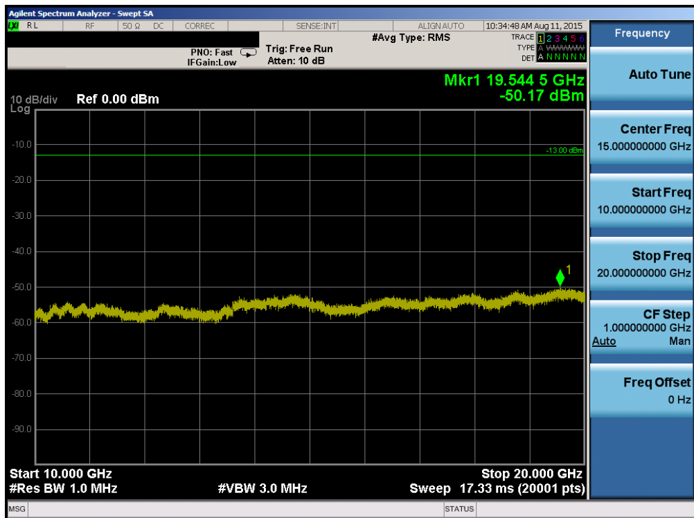
Plot 6-74. Conducted Spurious Plot (Band 2 – 20.0MHz QPSK – RB Size 1, RB Offset 0 – Mid Channel)
