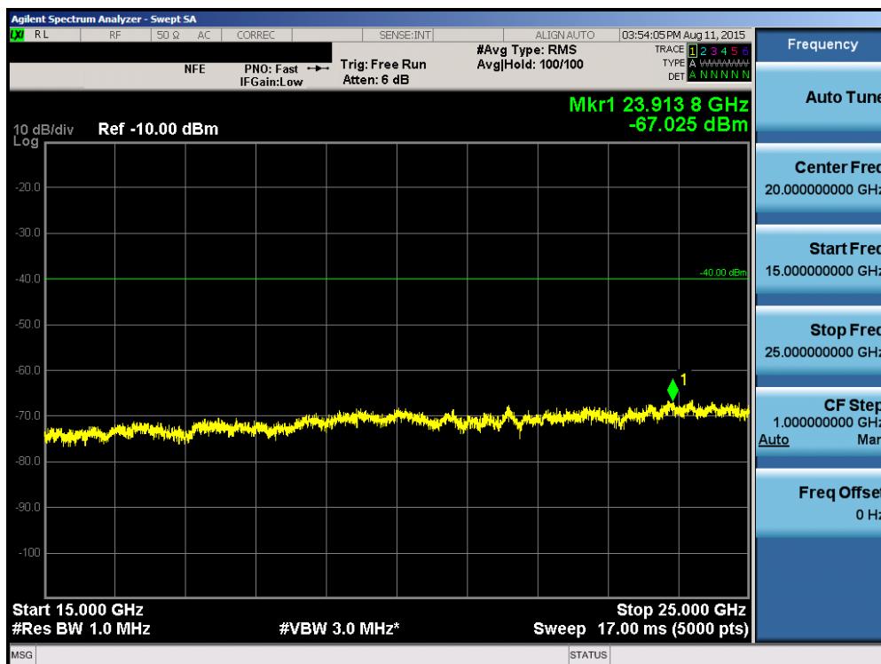
Plot 6-80. Conducted Spurious Plot (Band 30 – 10.0MHz QPSK – RB Size 1, RB Offset 0 – Mid Channel)
