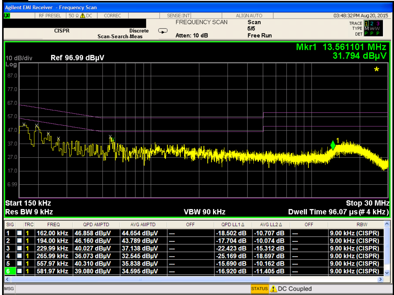
Plot 6-126. Line Conducted Plot with 802.11a UNII Band 1 (N)
