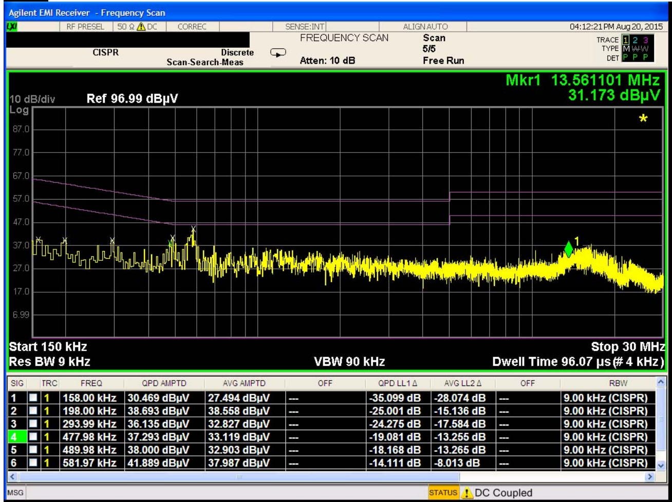
Plot 6-132. Line Conducted Plot with 802.11a UNII Band 3 (N)
