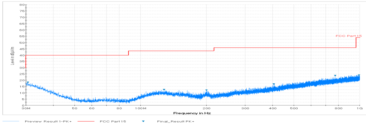
Plot 6-123. Radiated Spurious Plot below 1GHz (802.11a – U3 Ch. 157, Ant. Pol. H)
