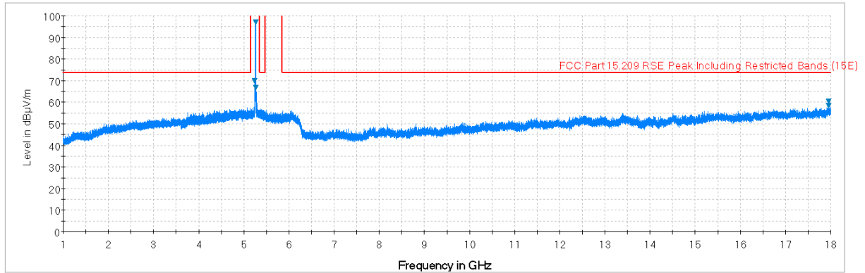
Plot 6-80. Radiated Spurious Plot above 1GHz (802.11a – U2A Ch. 56, Ant. Pol. V)
