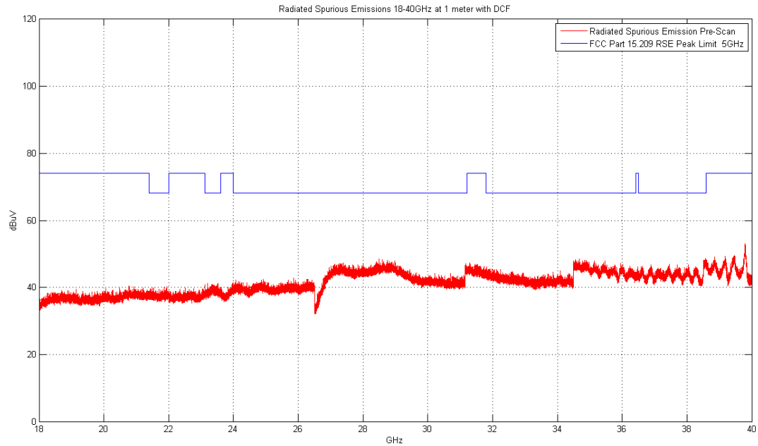
Plot 6-85. Radiated Spurious Plot above 18GHz (802.11a – Ant. Pol. H)
