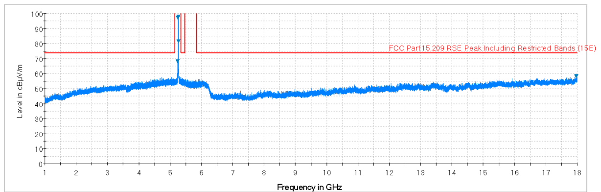
Plot 6-79. Radiated Spurious Plot above 1GHz (802.11a – U2A Ch. 56, Ant. Pol. H)
