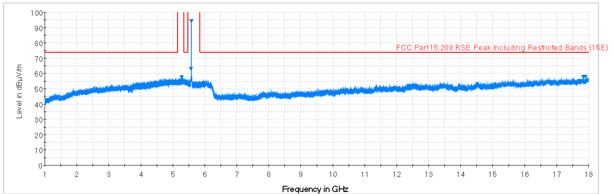
Plot 6-82. Radiated Spurious Plot above 1GHz (802.11a – U2C Ch. 116, Ant. Pol. V)
