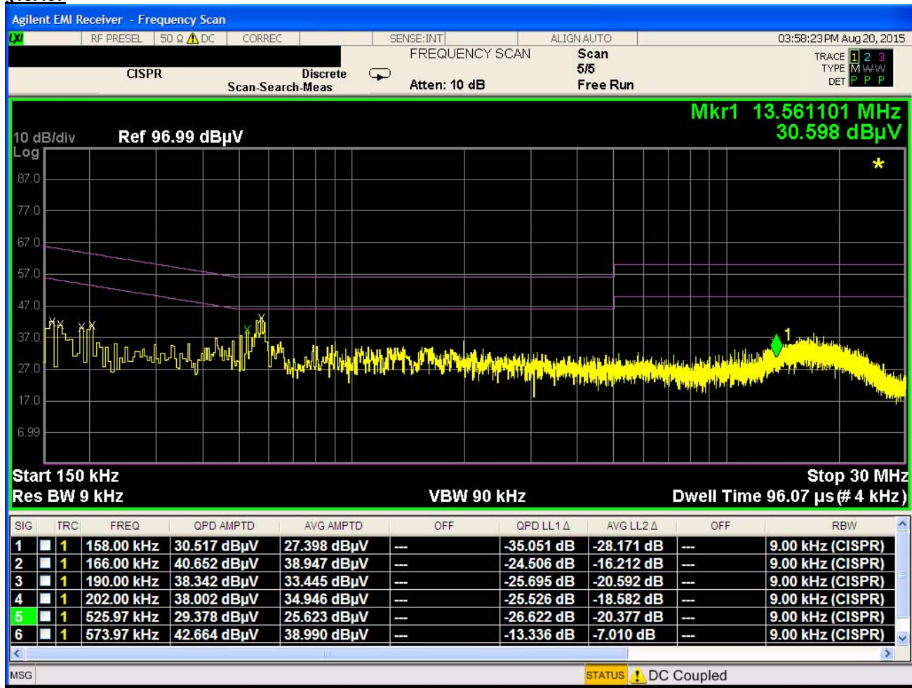
Plot 6-128. Line Conducted Plot with 802.11a UNII Band 2A (N)
