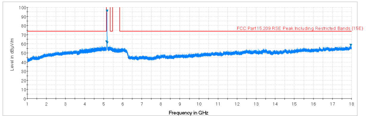
Plot 6-77. Radiated Spurious Plot above 1GHz (802.11a – U1 Ch. 40, Ant. Pol. H)
