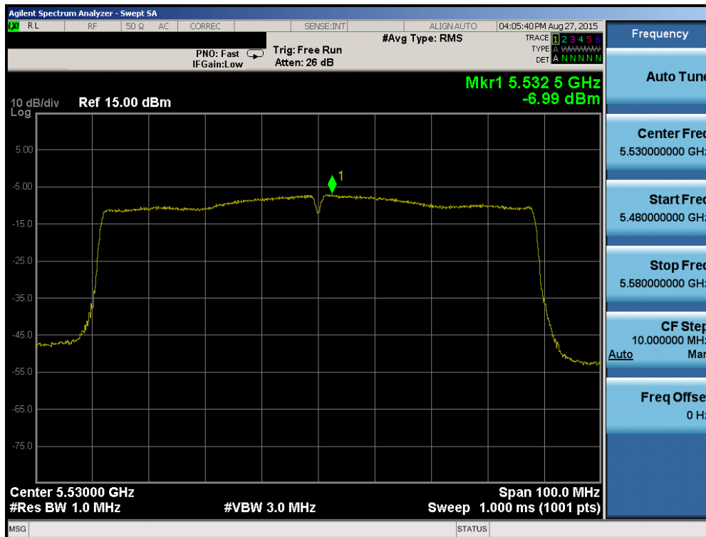
Plot 6-66. Power Spectral Density Plot (80MHz BW 802.11ac (UNII Band 2C) – Ch. 106)
