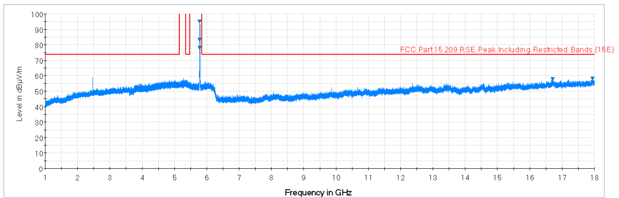
Plot 6-84. Radiated Spurious Plot above 1GHz (802.11a – U3 Ch. 157, Ant. Pol. V)
