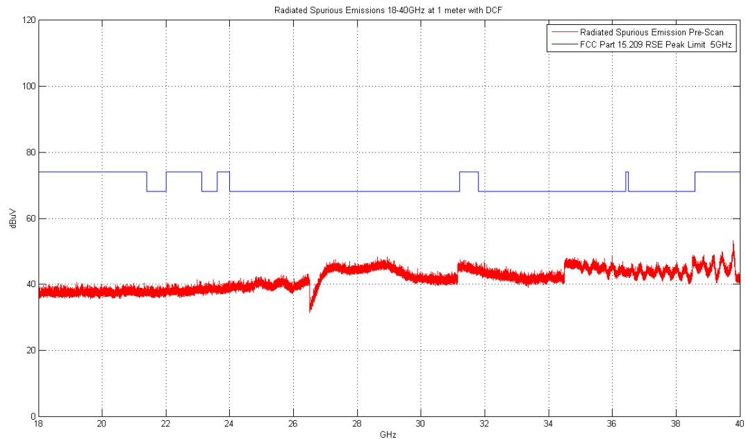
Plot 6-86. Radiated Spurious Plot above 18GHz (802.11a – Ant. Pol. V)
