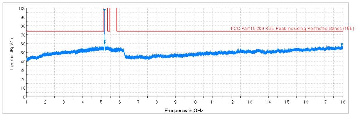
Plot 6-78. Radiated Spurious Plot above 1GHz (802.11a – U1 Ch. 40, Ant. Pol. V)
