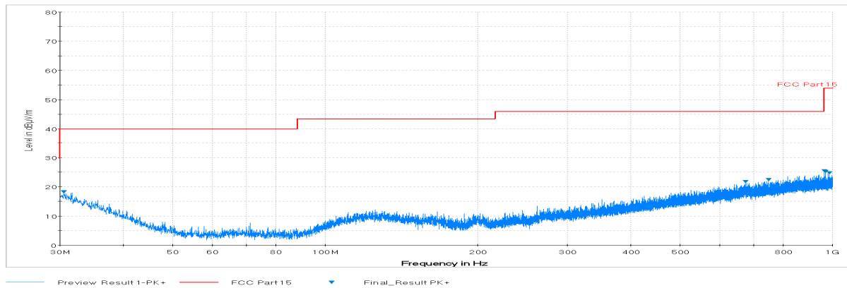
Plot 6-124. Radiated Spurious Plot below 1GHz (802.11a – U3 Ch. 157, Ant. Pol. V)
