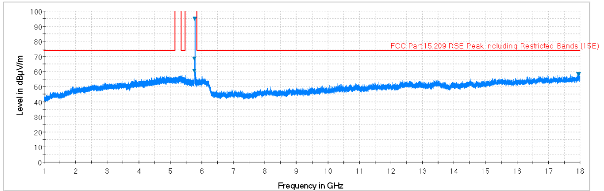
Plot 6-83. Radiated Spurious Plot above 1GHz (802.11a – U3 Ch. 157, Ant. Pol. H)
