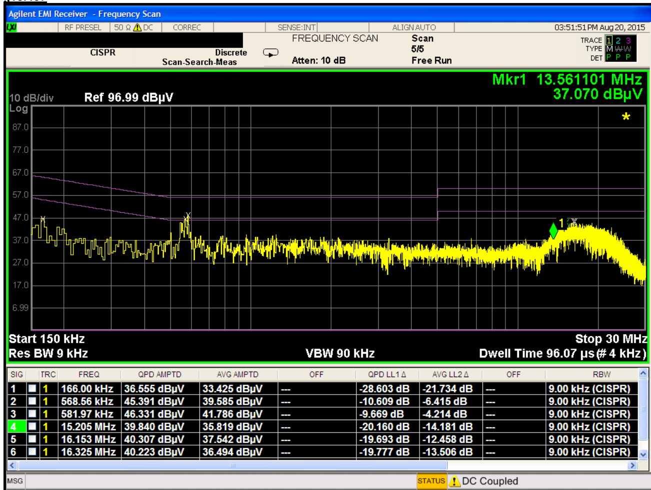
Plot 6-125. Line Conducted Plot with 802.11a UNII Band 1 (L1)
