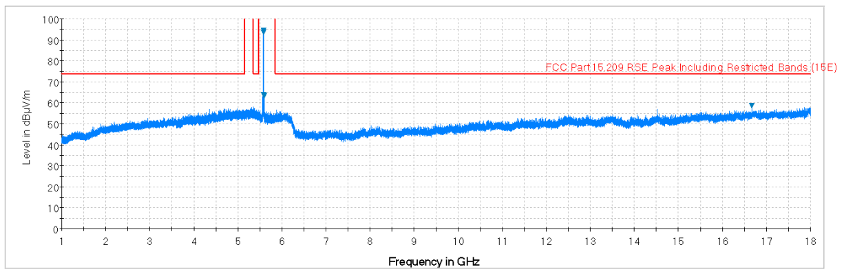
Plot 6-81. Radiated Spurious Plot above 1GHz (802.11a – U2C Ch. 116, Ant. Pol. H)
