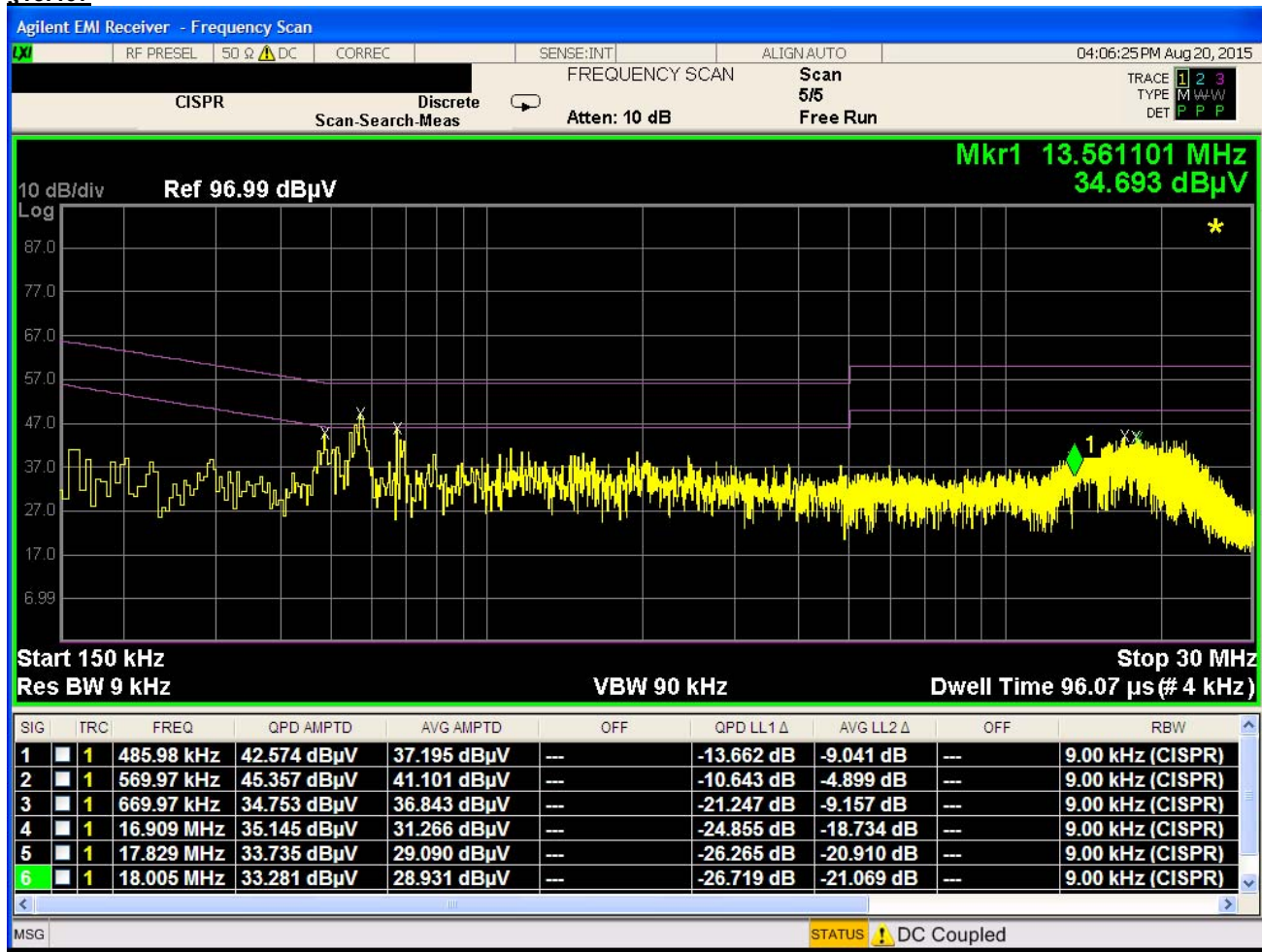
Plot 6-129. Line Conducted Plot with 802.11a UNII Band 2C (L1)
