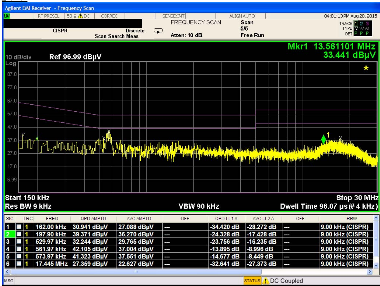
Plot 6-130. Line Conducted Plot with 802.11a UNII Band 2C (N)
