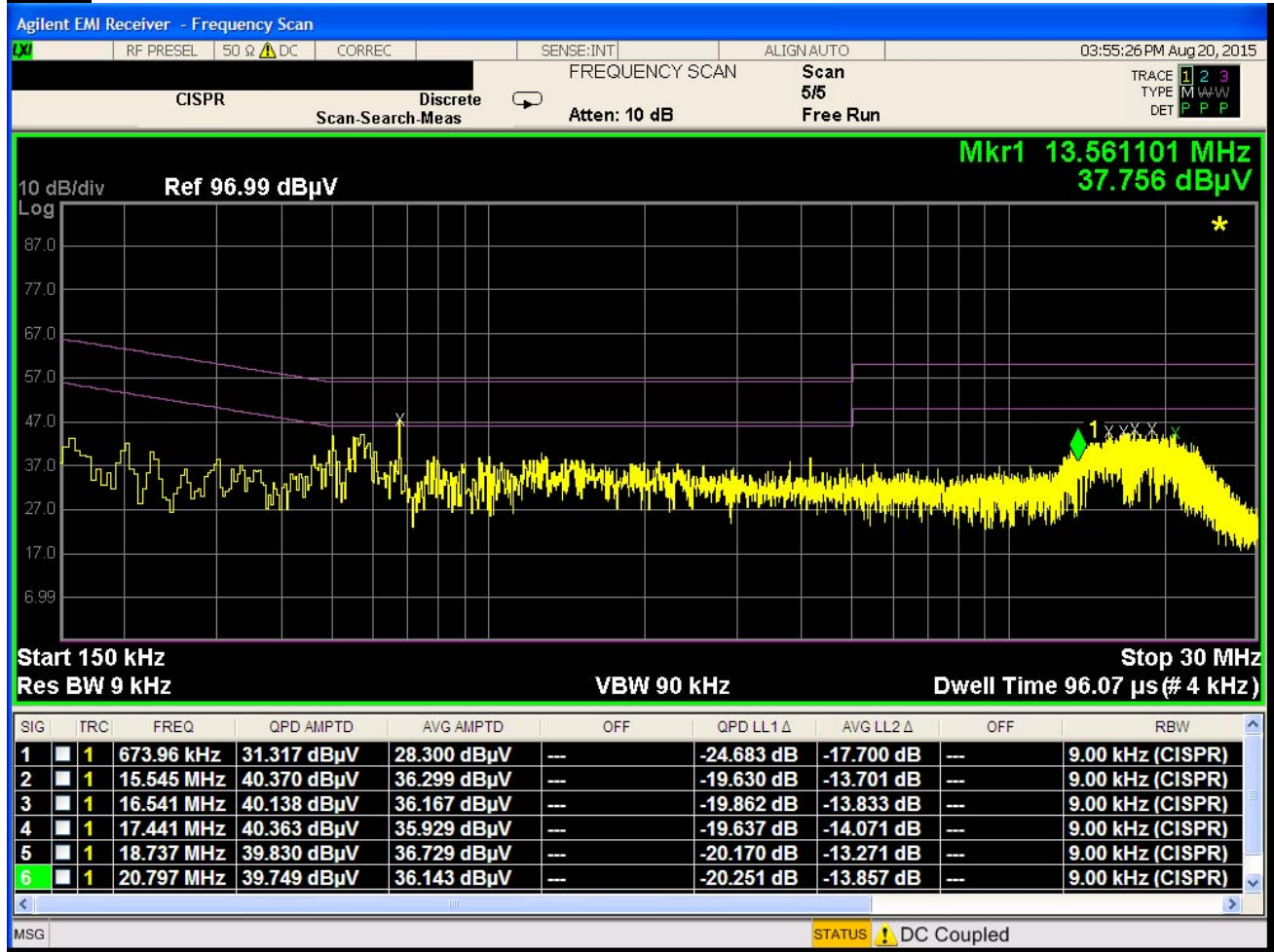
Plot 6-127. Line Conducted Plot with 802.11a UNII Band 2A (L1)
