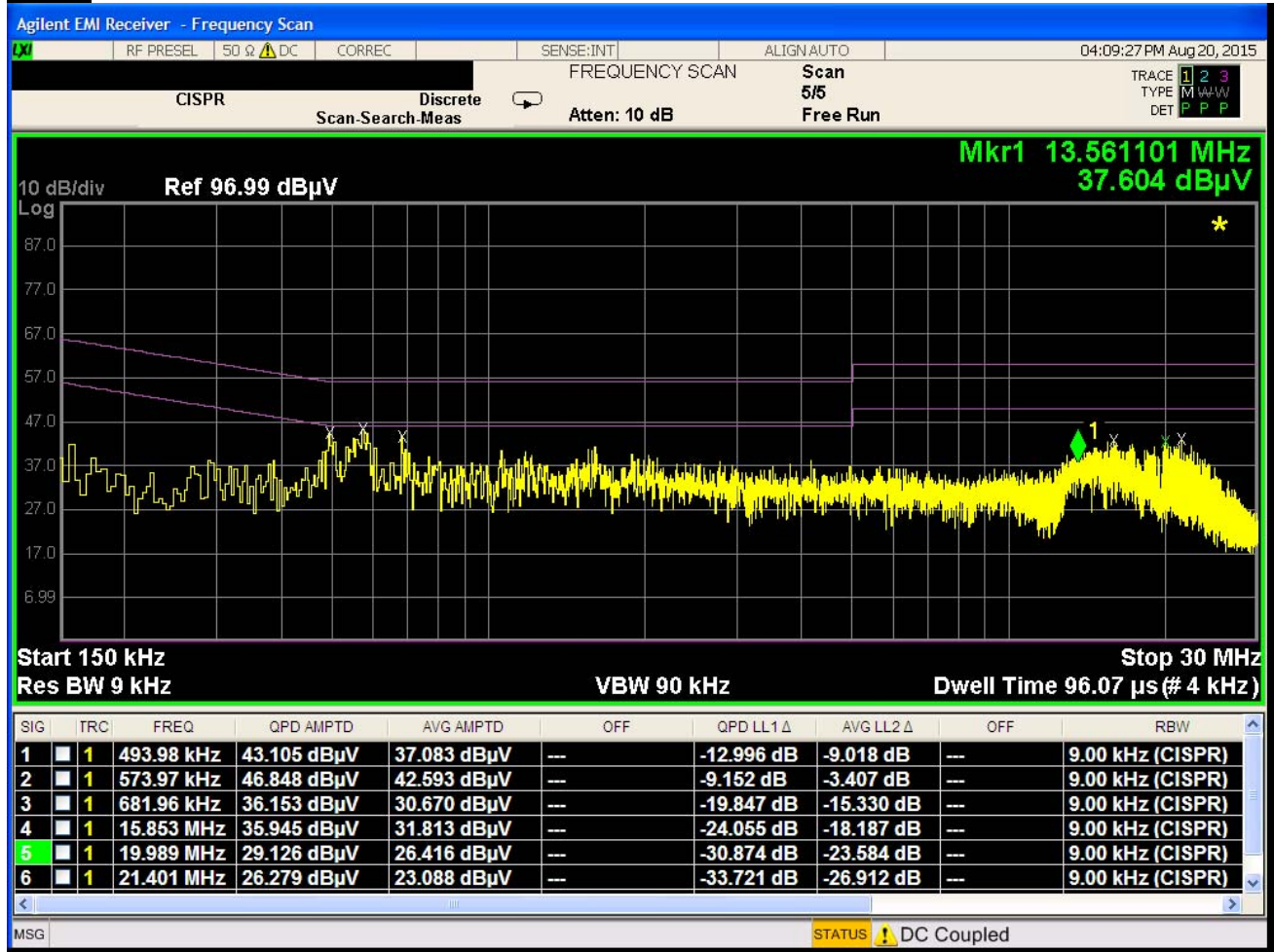
Plot 6-131. Line Conducted Plot with 802.11a UNII Band 3 (L1)
