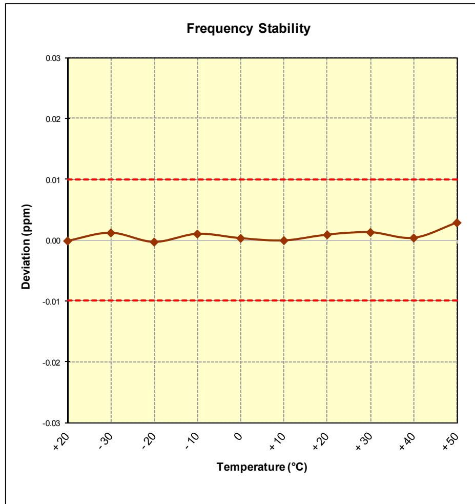
Figure 7-5. Frequency Stability Plot
