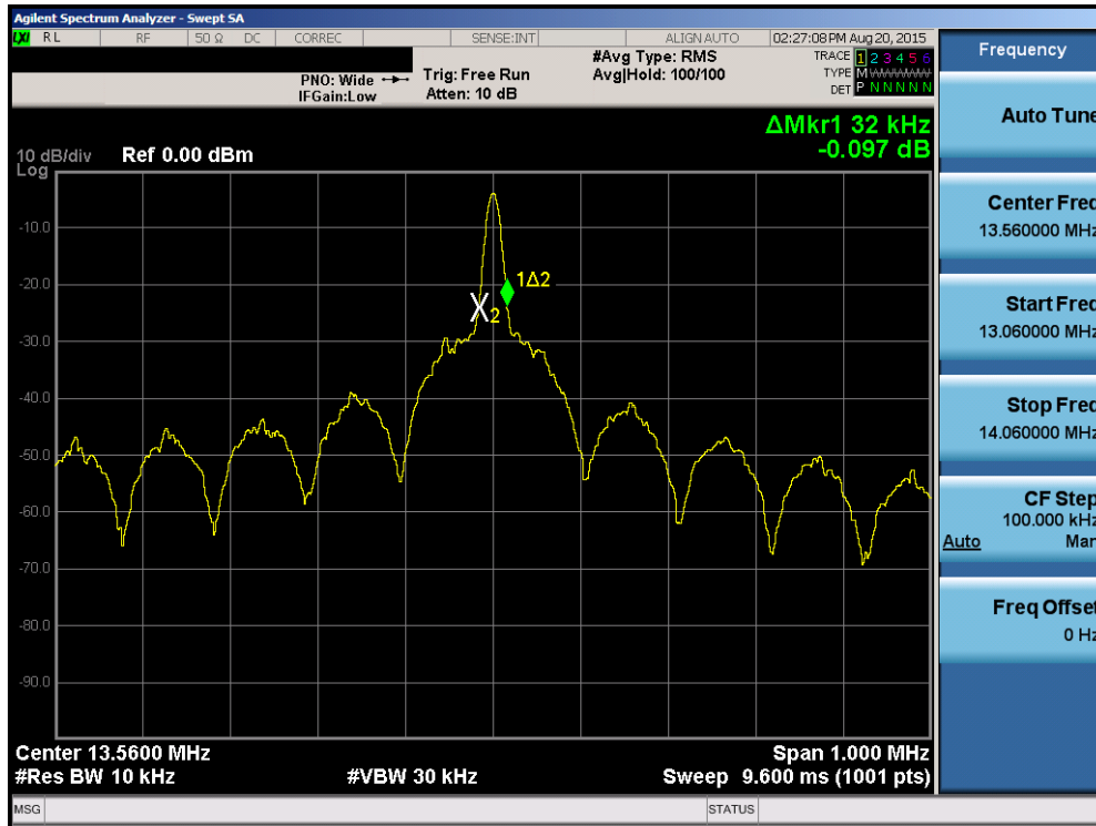
Figure 7-3. 20dB Bandwidth Plot with WCC
