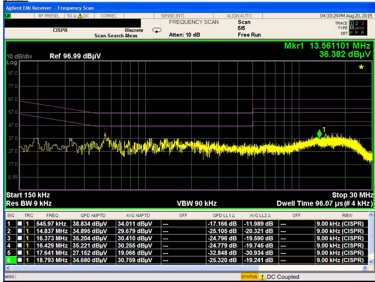
Plot 7-4. Line-Conducted Test Plot (N)
