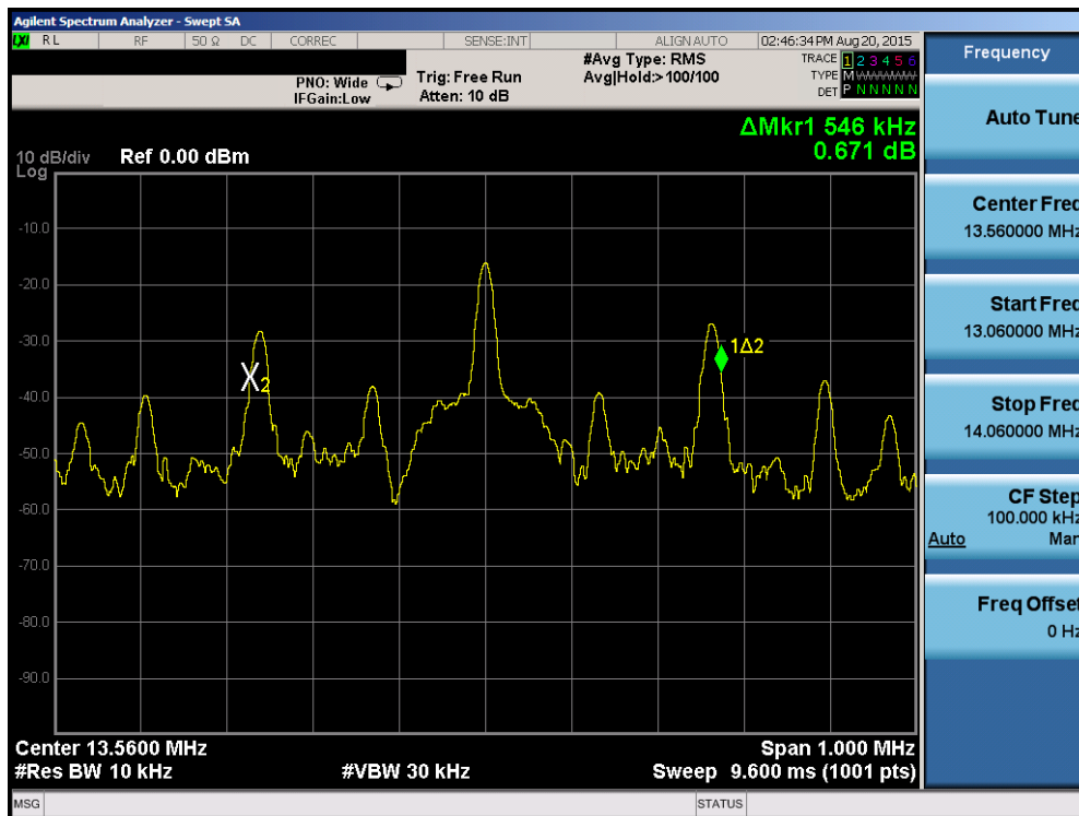
Figure 7-4. 20dB Bandwidth Plot with WCP
