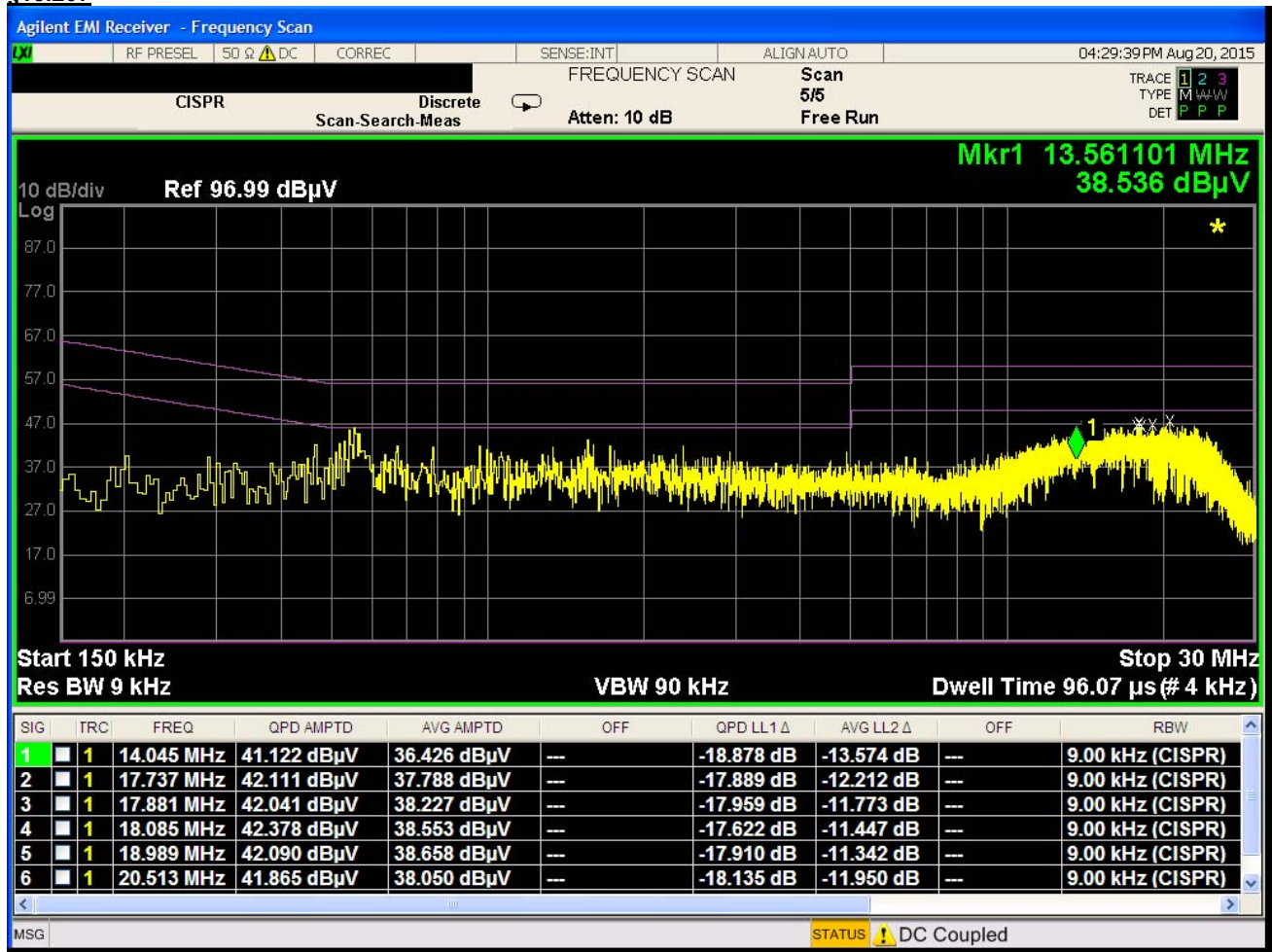
Plot 7-3. Line-Conducted Test Plot (L1)
