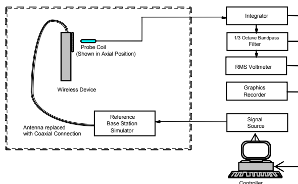
Figure 4-14 Audio Magnetic Field Test Setup
