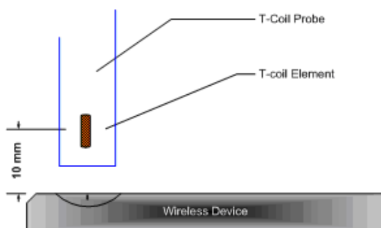
Figure 4-11 Measurement Distance
