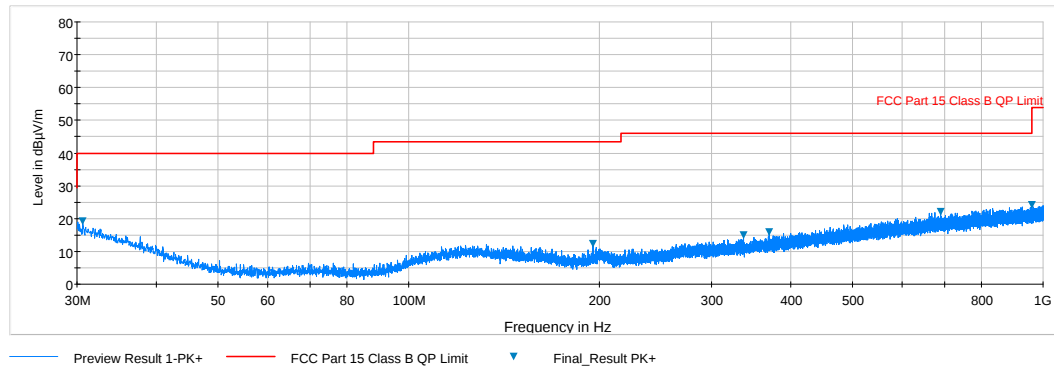
Plot 6-15. Radiated Spurious Plot below 1GHz (Pol. H)
