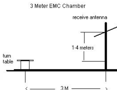
Figure 6-1. Test Instrument & Measurement Setup
