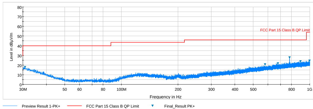
Plot 6-16. Radiated Spurious Plot below 1GHz (Pol. V)
