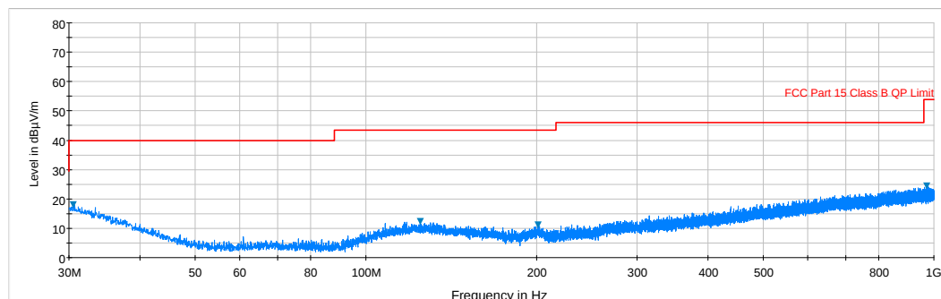
Plot 6-8. Radiated Spurious Plot below 1GHz (Pol. V)
