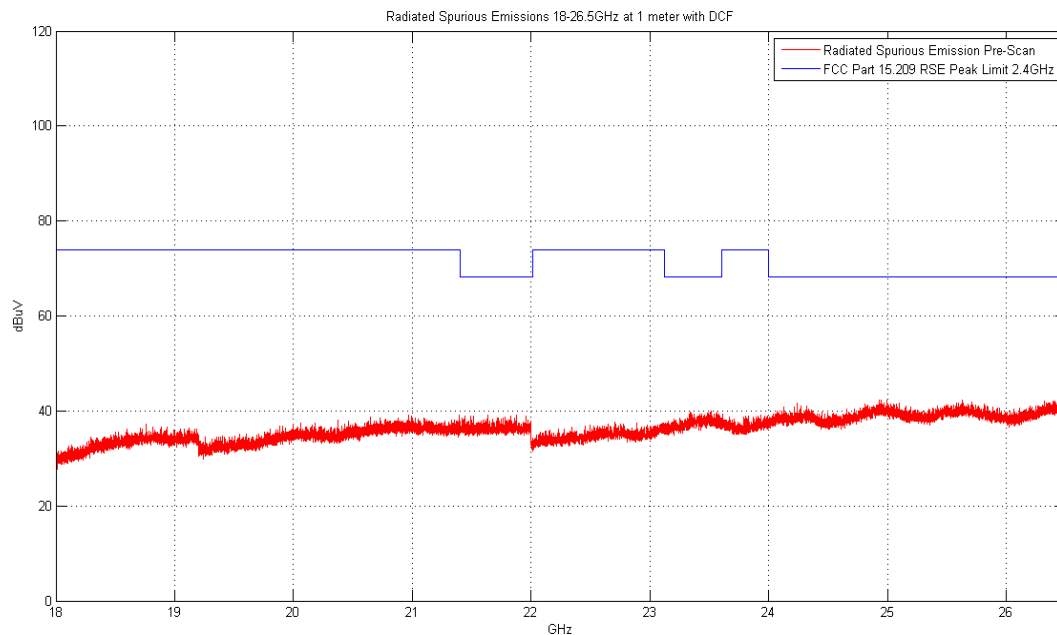
Plot 6-2. Radiated Spurious Plot above 18GHz (Pol. V)
