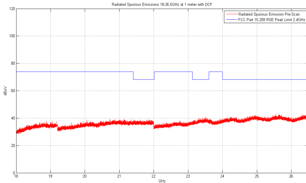
Plot 6-1. Radiated Spurious Plot above 18GHz (Pol. H)
