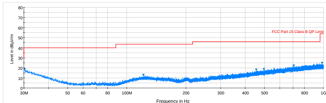
Plot 6-7. Radiated Spurious Plot below 1GHz (Pol. H)
