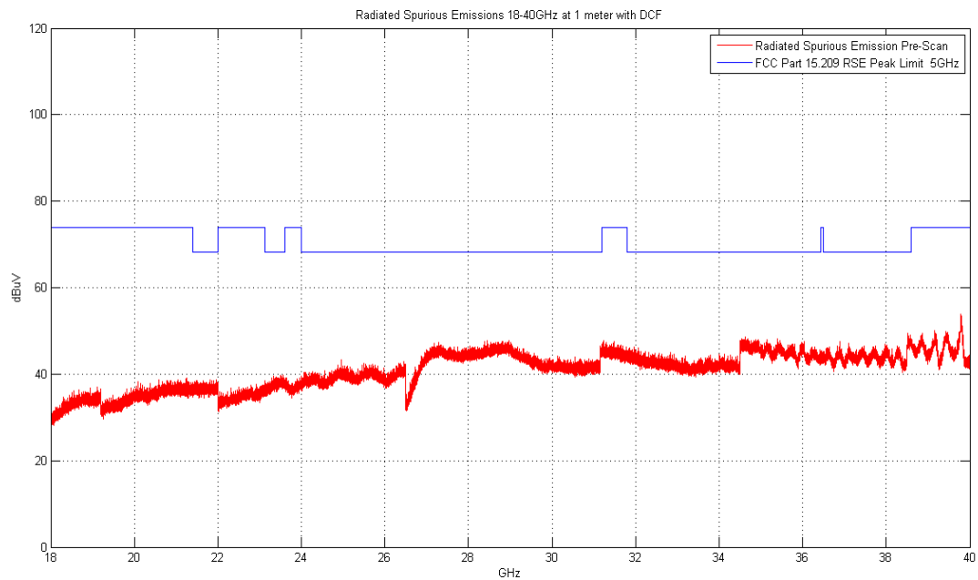
Plot 6-10. Radiated Spurious Plot above 18GHz (802.11a – Ant. Pol. V)
