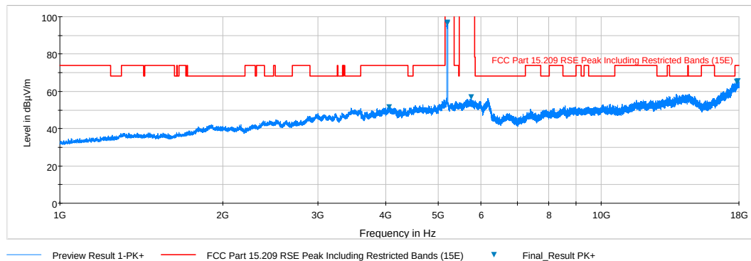
Plot 6-2. Radiated Spurious Plot above 1GHz (802.11a – U1 Ch. 40, Ant. Pol. V)
