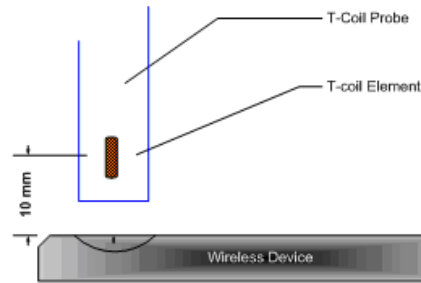
Figure 4-11 Measurement Distance
