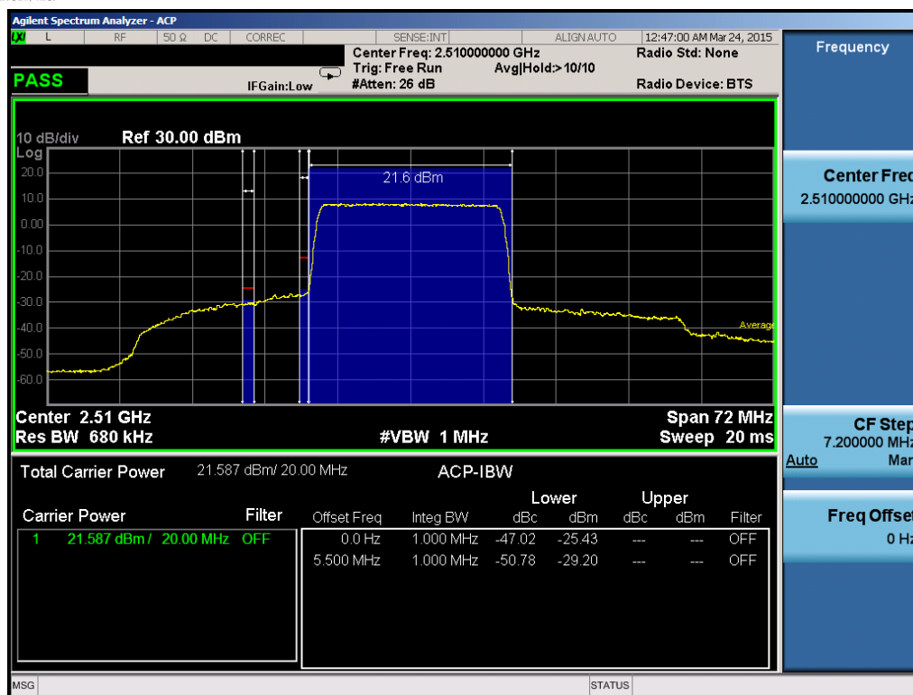
Plot 6-177. Lower ACP Plot (Band 7 – 20.0MHz QPSK – RB Size 100)
