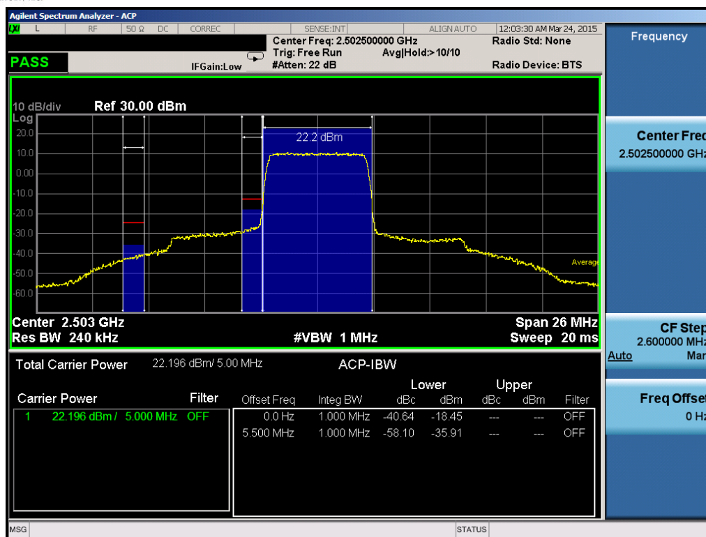
Plot 6-171. Lower ACP Plot (Band 7 – 5.0MHz QPSK – RB Size 25)
