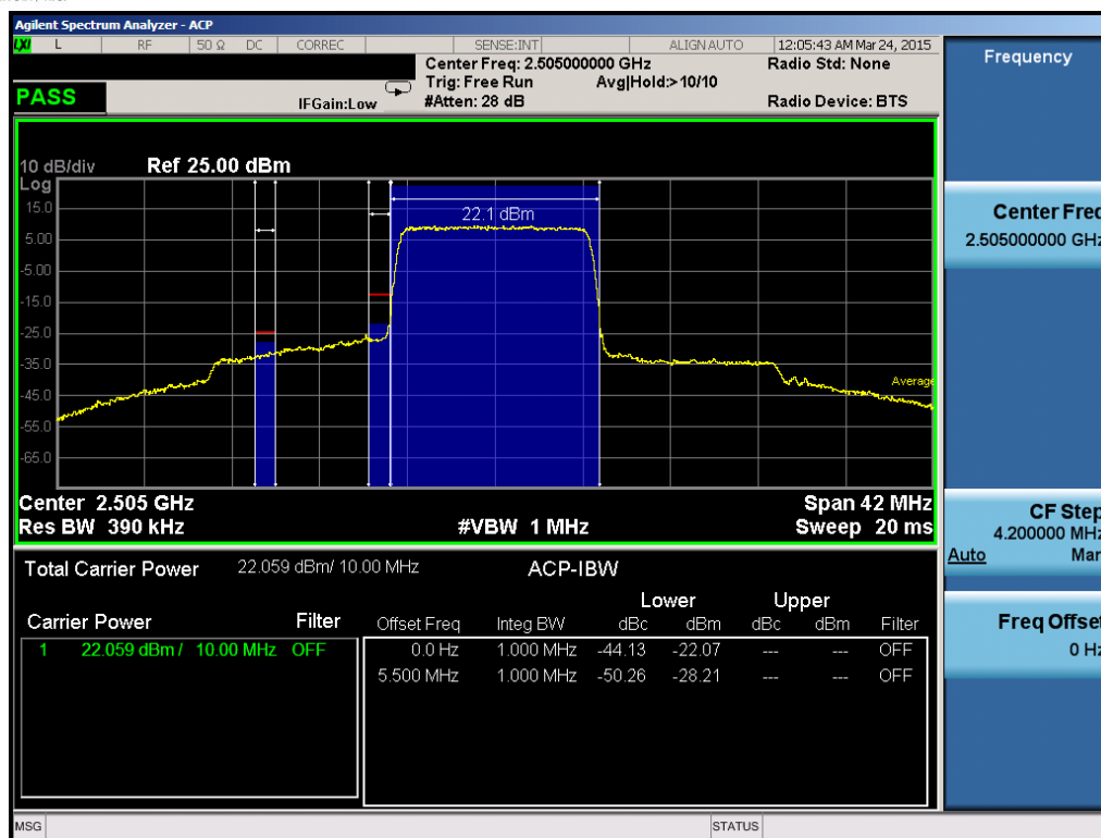
Plot 6-173. Lower ACP Plot (Band 7 – 10.0MHz QPSK – RB Size 50)
