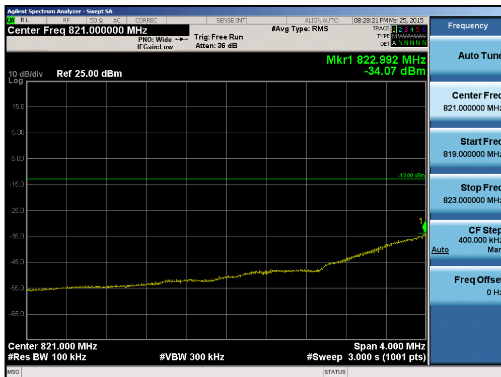
Plot 6-110. Lower Extended Band Edge Plot (Band 5 – 1.4MHz QPSK – RB Size 6)
