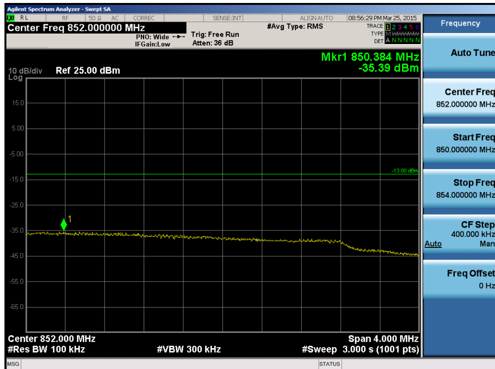
Plot 6-120. Upper Extended Band Edge Plot (Band 5 - 5.0MHz QPSK - RB Size 25)
