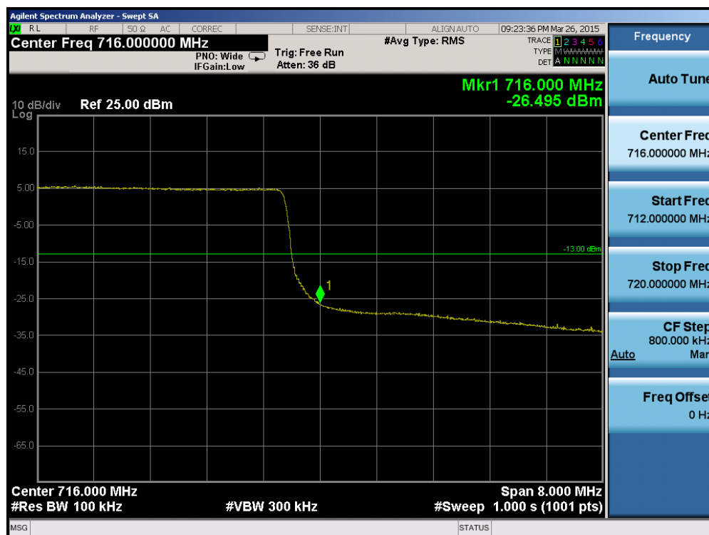
Plot 6-108. Upper Band Edge Plot (Band 12 – 10.0MHz QPSK – RB Size 50)
