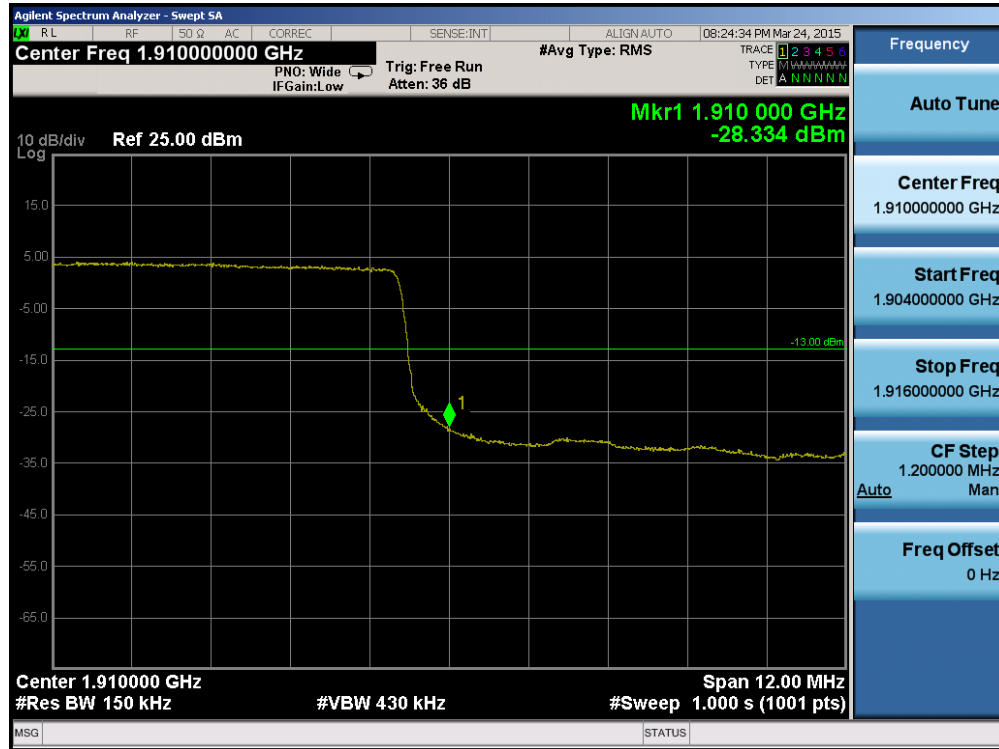
Plot 6-165. Upper Band Edge Plot (Band 2 – 15.0MHz QPSK – RB Size 75)
