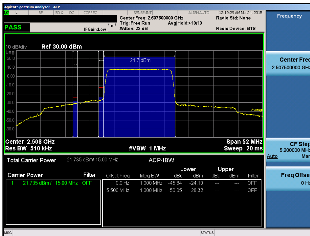
Plot 6-175. Lower ACP Plot (Band 7 – 15.0MHz QPSK – RB Size 75)
