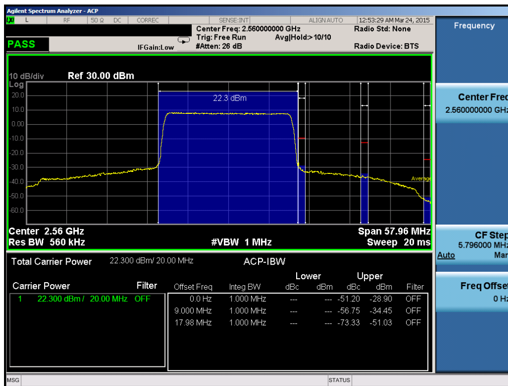
Plot 6-178. Upper ACP Plot (Band 7 – 20.0MHz QPSK – RB Size 100)
