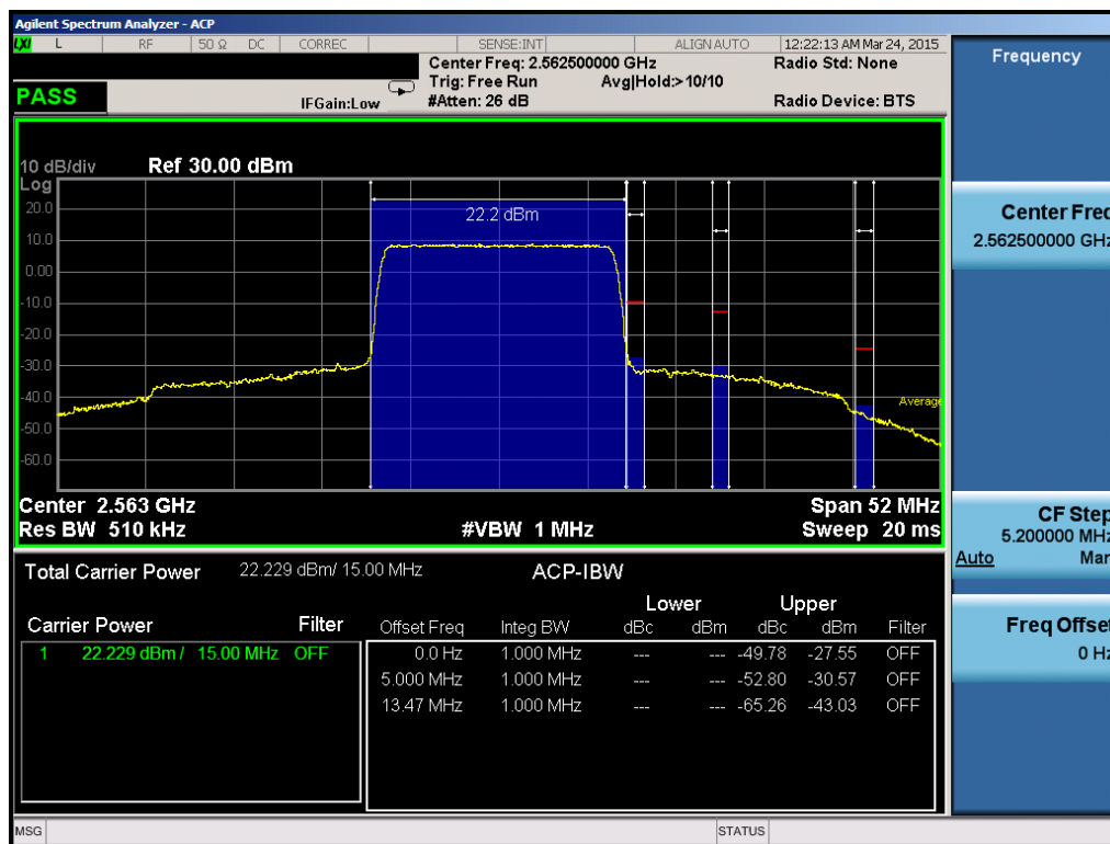
Plot 6-176. Upper ACP Plot (Band 7 – 15.0MHz QPSK – RB Size 75)
