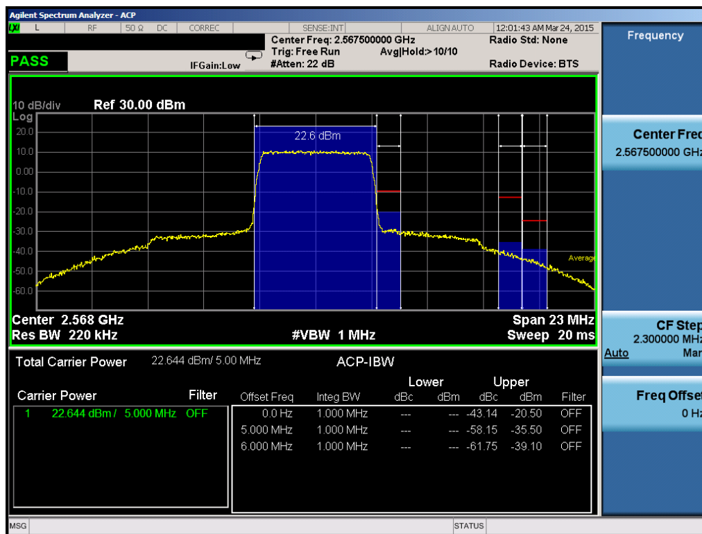
Plot 6-172. Upper ACP Plot (Band 7 – 5.0MHz QPSK – RB Size 25)
