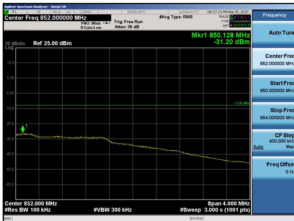
Plot 6-116. Upper Extended Band Edge Plot (Band 5 - Band 5 - 3.0MHz QPSK - RB Size 15)
