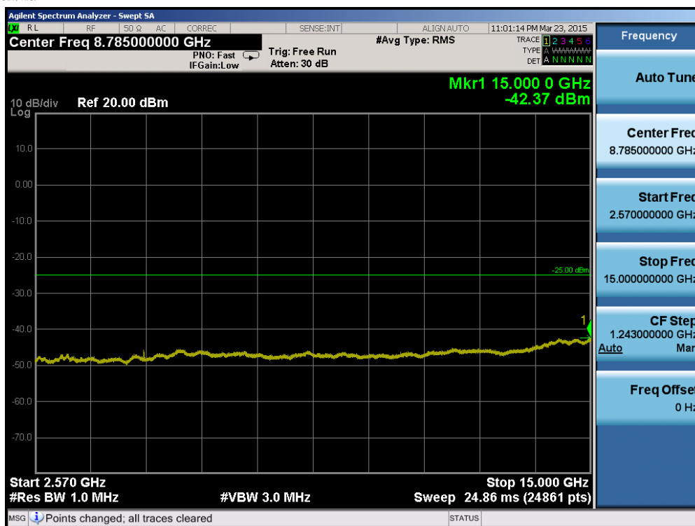
Plot 6-87. Conducted Spurious Plot (Band 7 – 20.0MHz QPSK – RB Size 1, RB Offset 0 – Low Channel)
