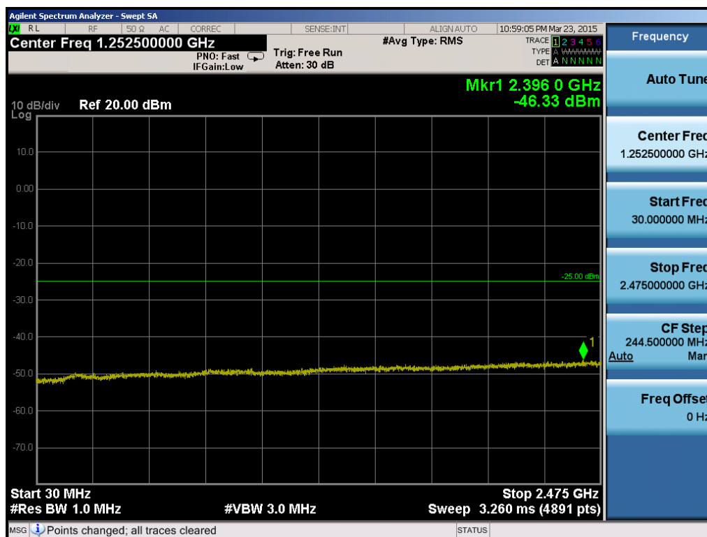
Plot 6-86. Conducted Spurious Plot (Band 7 – 20.0MHz QPSK – RB Size 1, RB Offset 0– Low Channel)
