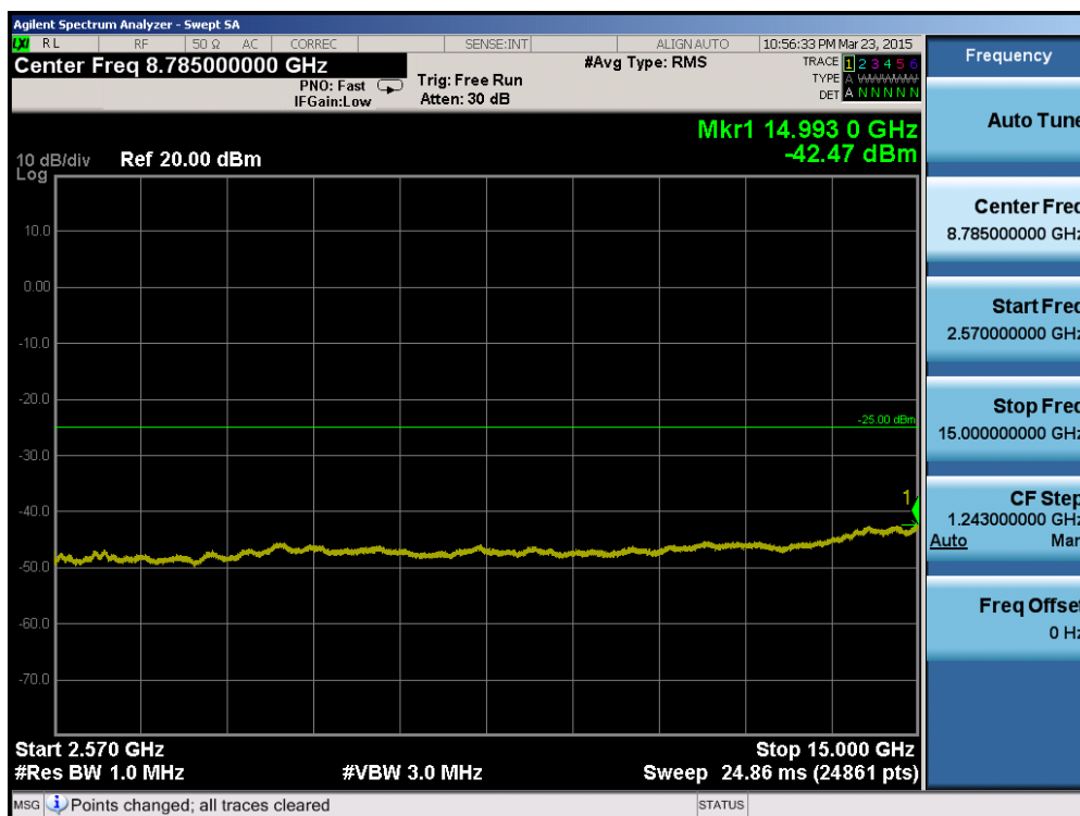
Plot 6-90. Conducted Spurious Plot (Band 7 – 20.0MHz QPSK – RB Size 1, RB Offset 0 – Mid Channel)
