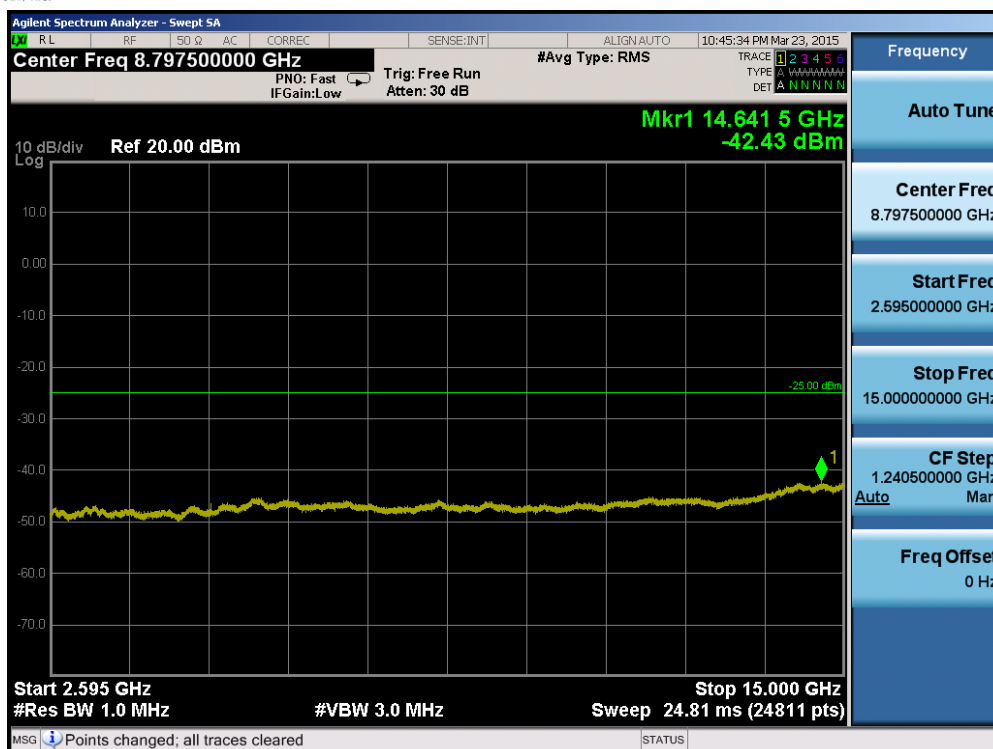
Plot 6-93. Conducted Spurious Plot (Band 7 – 20.0MHz QPSK – RB Size 1, RB Offset 0 – High Channel)
