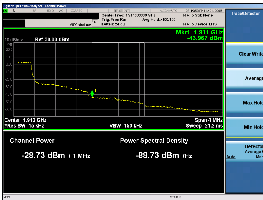
Plot 6-83. Conducted Spurious Plot (Band 2 – 1.4MHz QPSK – RB Size 1, RB Offset 0 – High Channel)
