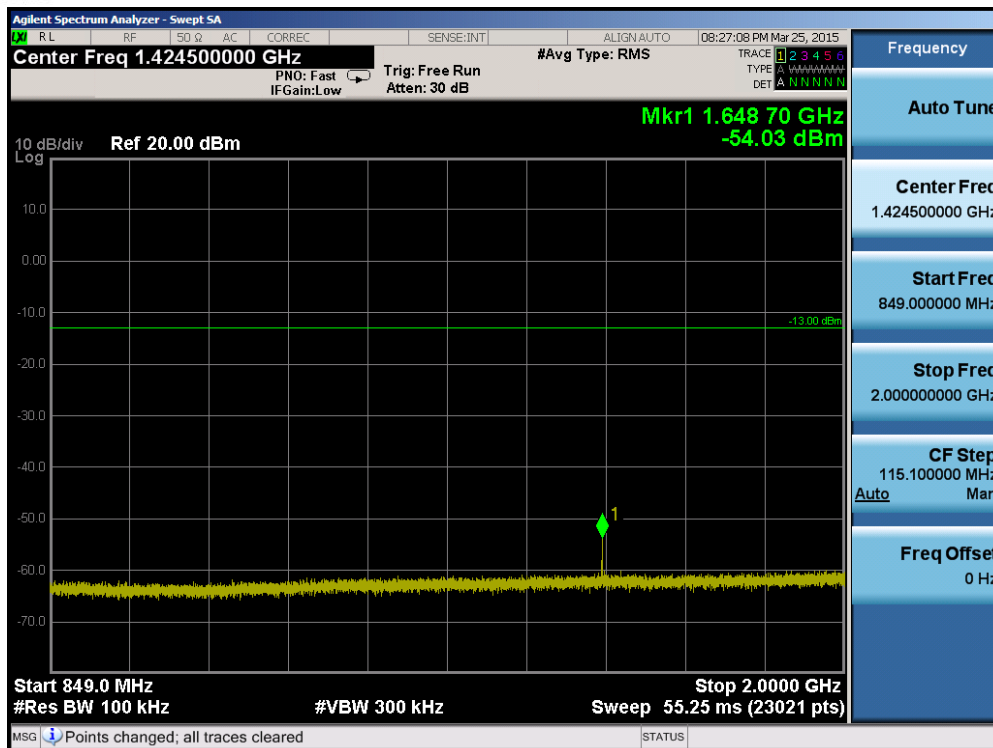
Plot 6-59. Conducted Spurious Plot (Band 5 – 1.4MHz QPSK – RB Size 1, RB Offset 0 – Low Channel)
