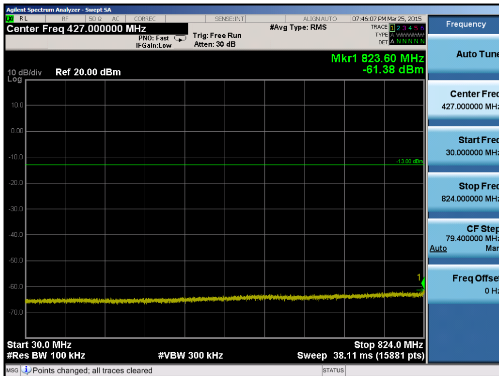
Plot 6-61. Conducted Spurious Plot (Band 5 – 1.4MHz QPSK – RB Size 1, RB Offset 0 – Mid Channel)
