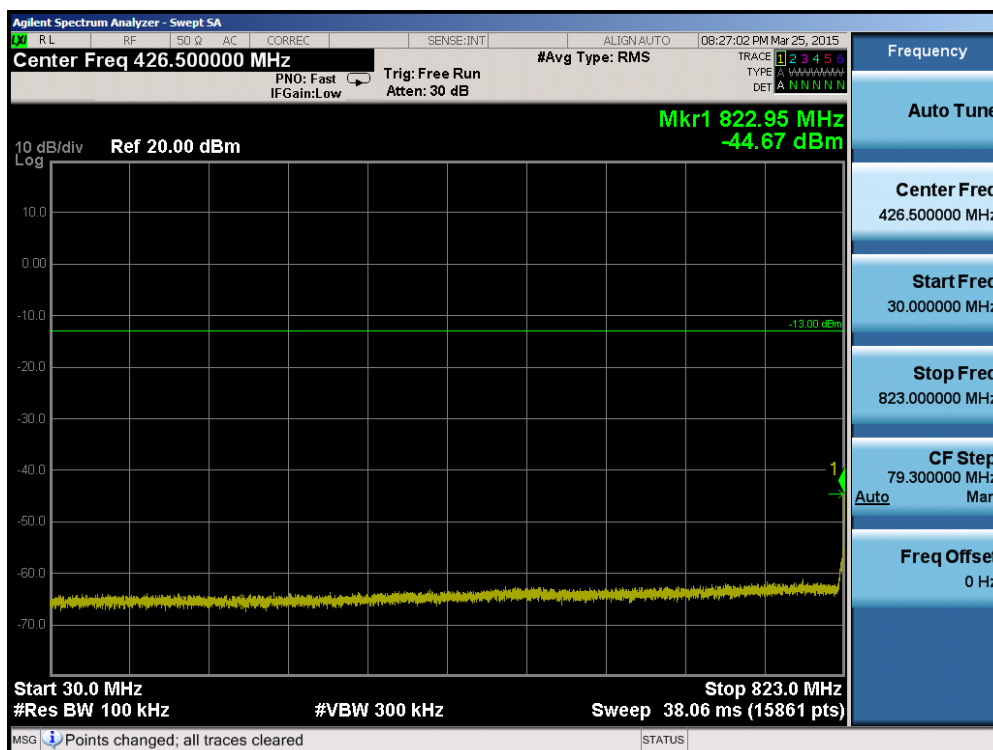
Plot 6-58. Conducted Spurious Plot (Band 5 – 1.4MHz QPSK – RB Size 1, RB Offset 0 – Low Channel)
