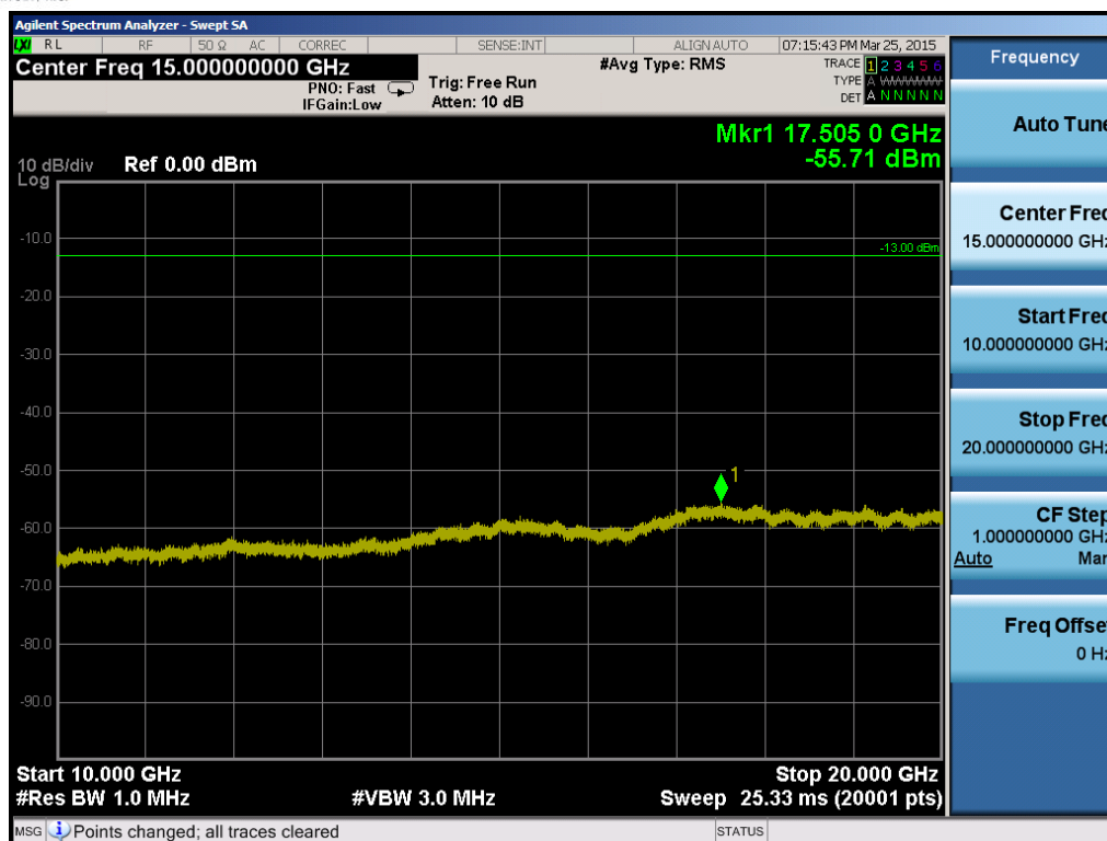
Plot 6-75. Conducted Spurious Plot (Band 4 – 10.0MHz QPSK – RB Size 1, RB Offset 0 – High Channel)
