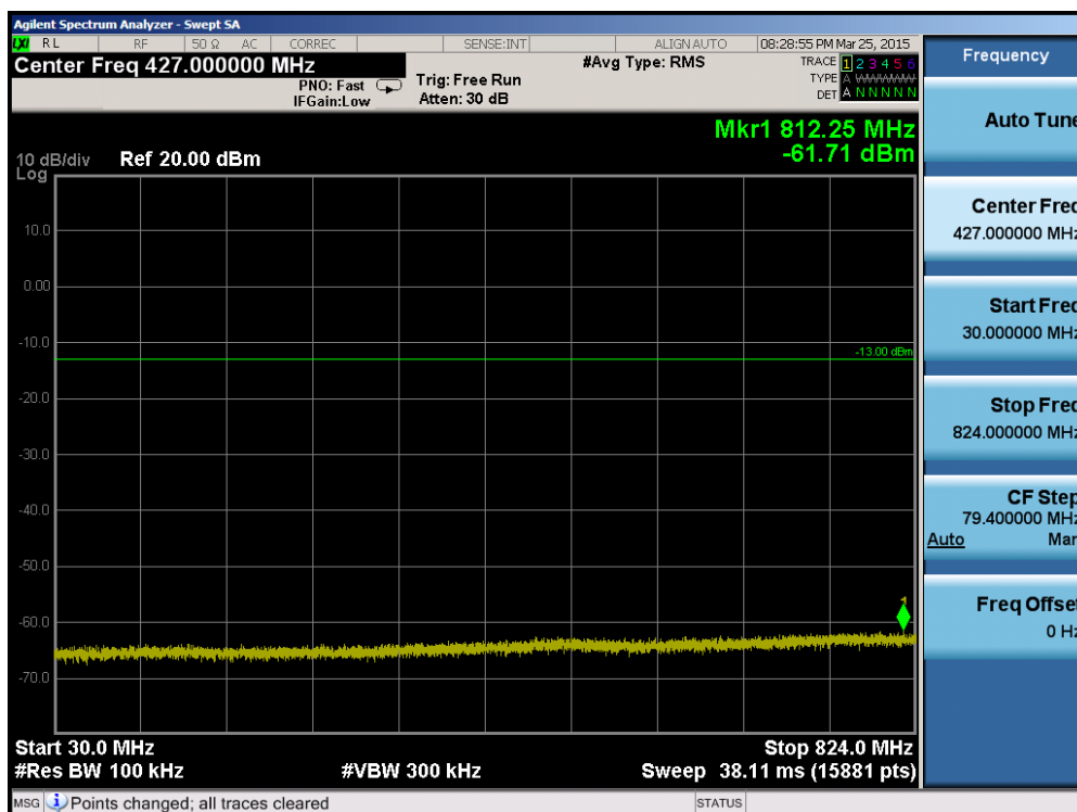
Plot 6-64. Conducted Spurious Plot (Band 5 – 1.4MHz QPSK – RB Size 1, RB Offset 0 – High Channel)
