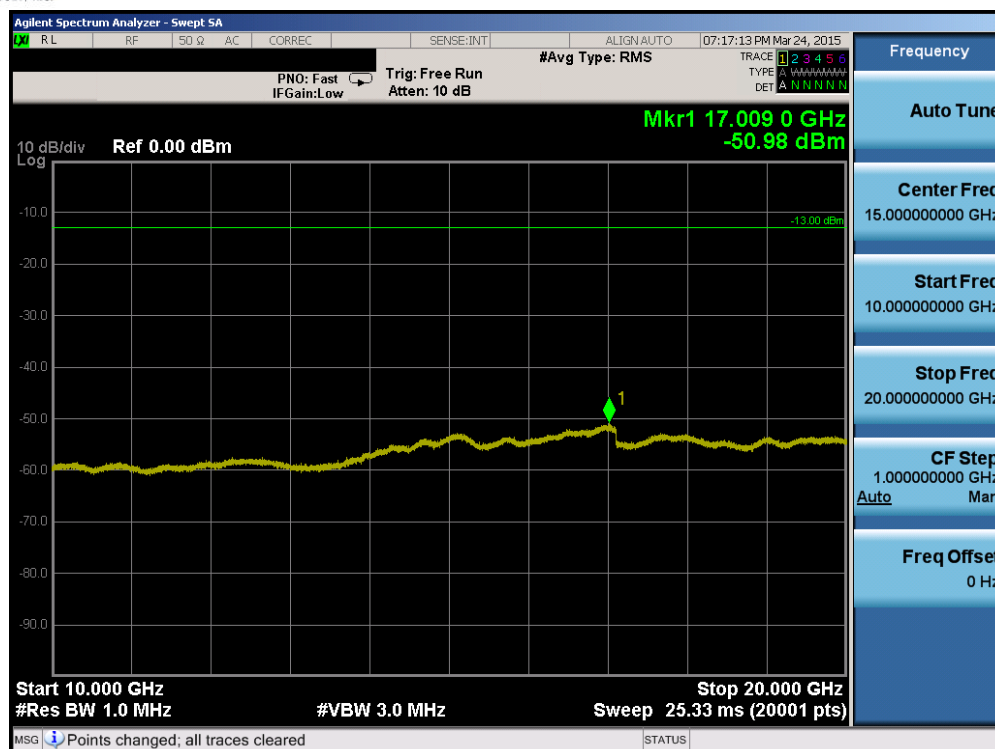
Plot 6-85. Conducted Spurious Plot (Band 2 – 1.4MHz QPSK – RB Size 1, RB Offset 0 – High Channel)
