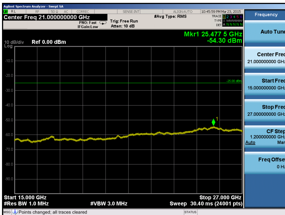
Plot 6-94. Conducted Spurious Plot (Band 7 – 20.0MHz QPSK – RB Size 1, RB Offset 0 – High Channel)
