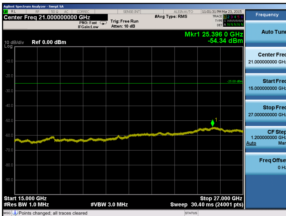
Plot 6-88. Conducted Spurious Plot (Band 7 – 20.0MHz QPSK – RB Size 1, RB Offset 0 – Low Channel)
