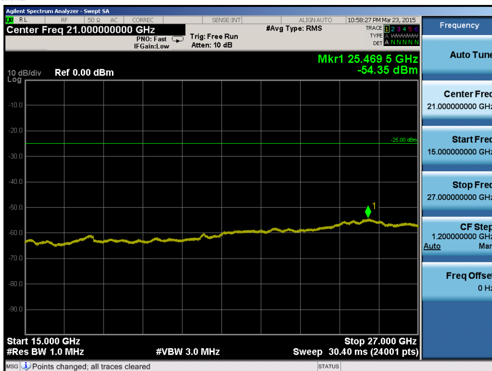
Plot 6-91. Conducted Spurious Plot (Band 7 – 20.0MHz QPSK – RB Size 1, RB Offset 0 – Mid Channel)
