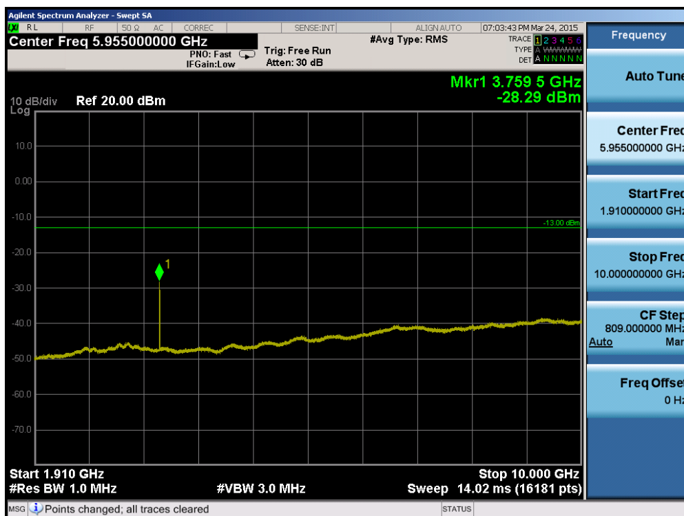
Plot 6-80. Conducted Spurious Plot (Band 2 – 1.4MHz QPSK – RB Size 1, RB Offset 0 – Mid Channel)
