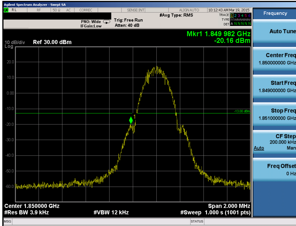
Plot 6-55. Band Edge Plot (PCS GSM Mode – Ch. 512)
