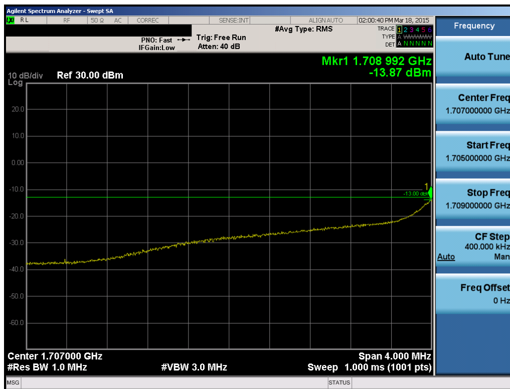
Plot 6-62. 4MHz Span Plot (AWS WCDMA Mode – Ch. 1312)
