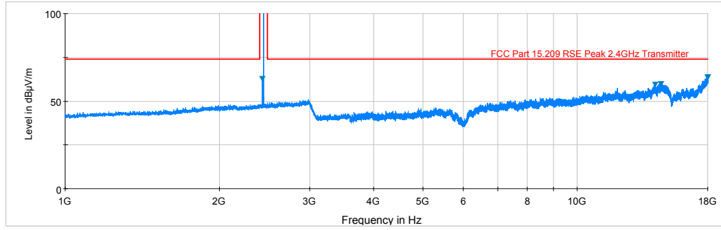
Plot 6-4. Radiated Spurious Plot above 1GHz (BTLE – Ch. 19, Ant. Pol. V)
