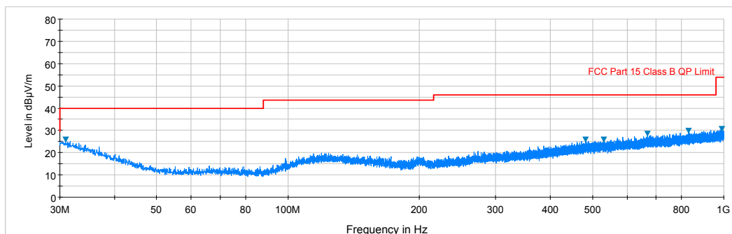
Plot 6-11. Radiated Spurious Plot below 1GHz (Pol. H)
