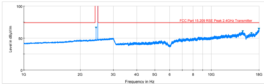
Plot 6-5. Radiated Spurious Plot above 1GHz (BTLE – Ch. 39, Ant. Pol. H)
