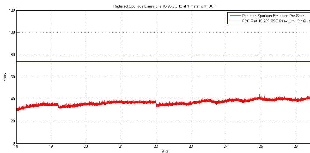
Plot 6-8. Radiated Spurious Plot above 18GHz (Pol. V)
