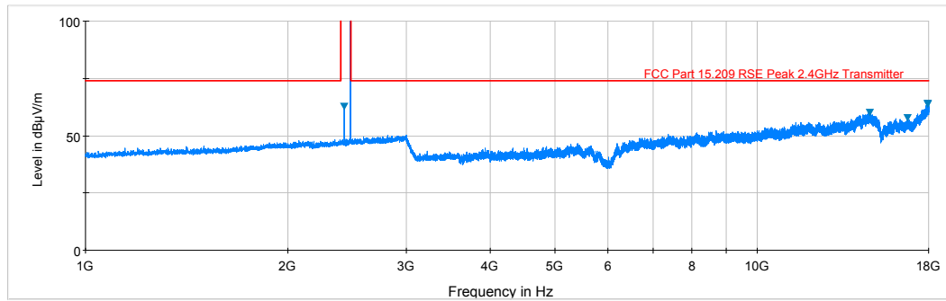
Plot 6-6. Radiated Spurious Plot above 1GHz (BTLE – Ch. 39, Ant. Pol. V)
