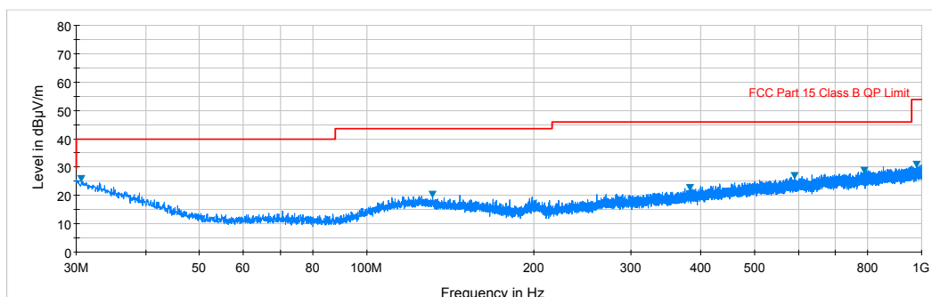
Plot 6-12. Radiated Spurious Plot below 1GHz (Pol. V)
