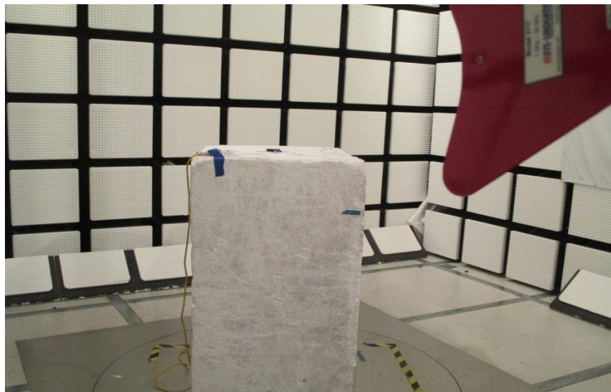
RADIATED FRONT PHOTO (ABOVE 1 GHz)
