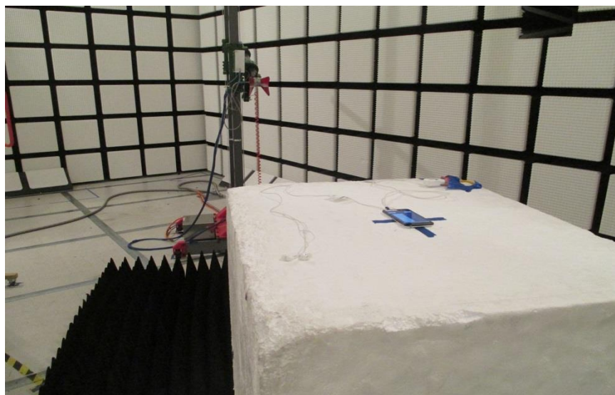
RADIATED BACK PHOTO (ABOVE 1 GHz)
