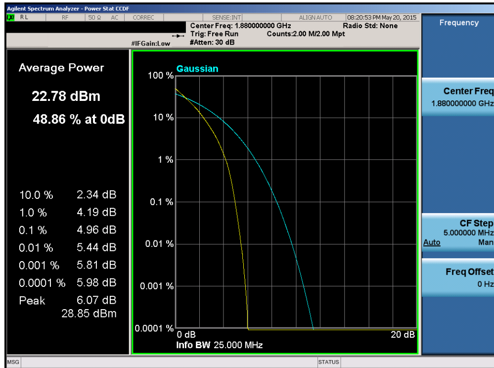
Plot 6-216. PAR Plot (Band 2 – 20.0MHz 16-QAM – RB Size 100)
