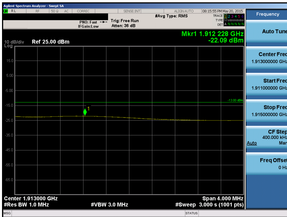
Plot 6-192. Upper Extended Band Edge Plot (Band 2 – 15.0MHz QPSK – RB Size 75)
