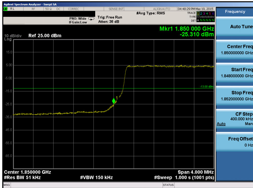
Plot 6-181. Lower Band Edge Plot (Band 2 – 5.0MHz QPSK – RB Size 25)
