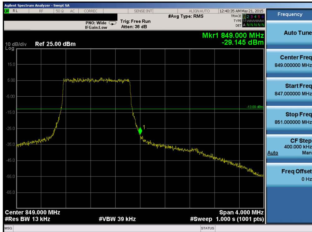
Plot 6-137. Upper Band Edge Plot (Band 5 – 1.4MHz QPSK – RB Size 6)
