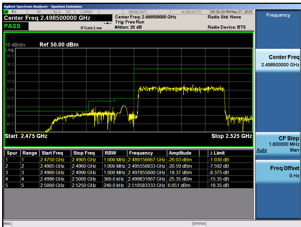
Plot 6-203. Lower ACP Plot (Band 7 – 20.0MHz QPSK – RB Size 100)
