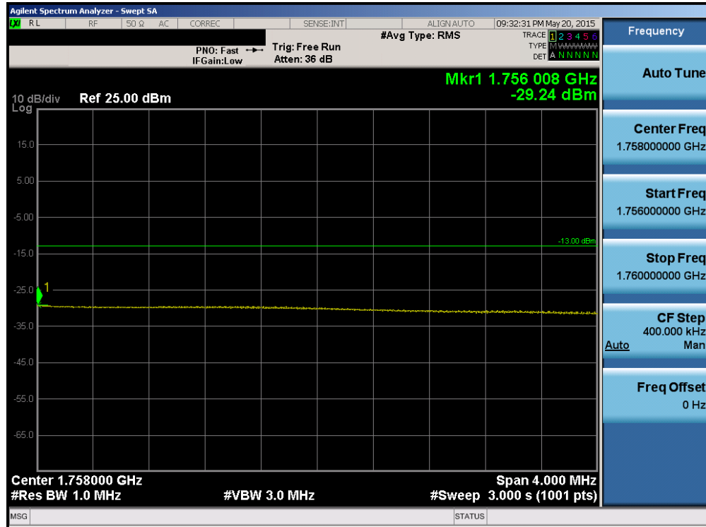
Plot 6-172. Upper Extended Band Edge Plot (Band 4 – 20.0MHz QPSK – RB Size 100)
