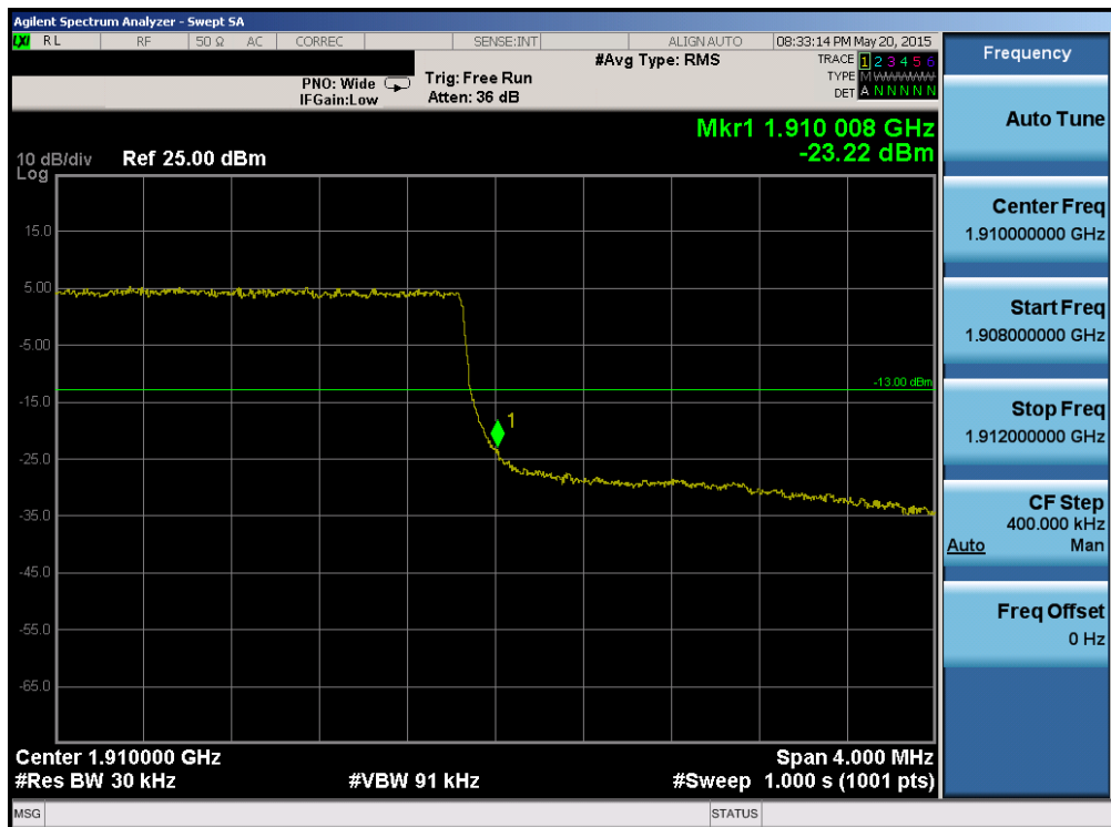
Plot 6-179. Upper Band Edge Plot (Band 2 – 3.0MHz QPSK – RB Size 15)
