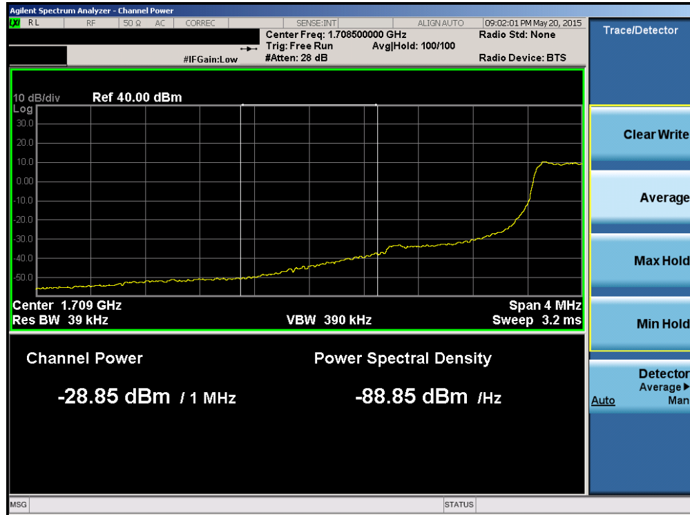
Plot 6-150. Lower Extended Band Edge Plot (Band 4 – 1.4MHz QPSK – RB Size 6)
