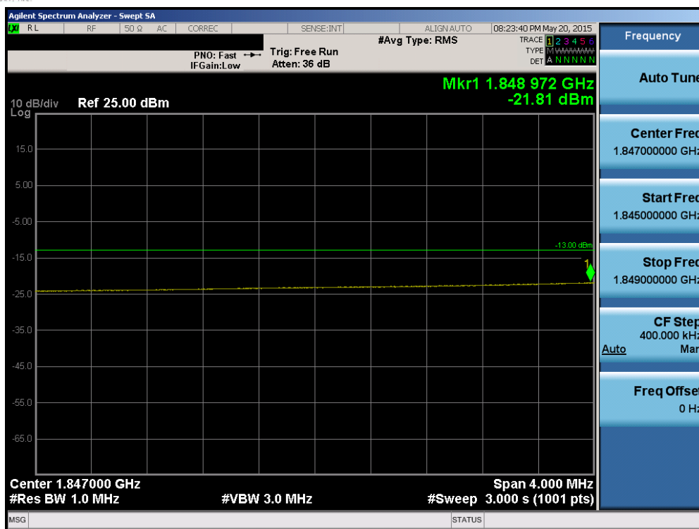
Plot 6-194. Lower Extended Band Edge Plot (Band 2 – 20.0MHz QPSK – RB Size 100)
