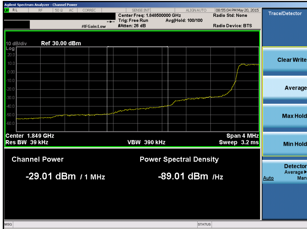
Plot 6-174. Lower Extended Band Edge Plot (Band 2 – 1.4MHz QPSK – RB Size 6)
