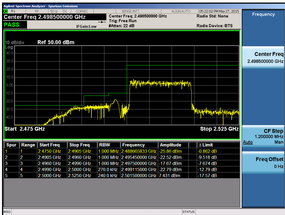
Plot 6-201. Lower ACP Plot (Band 7 – 15.0MHz QPSK – RB Size 75)
