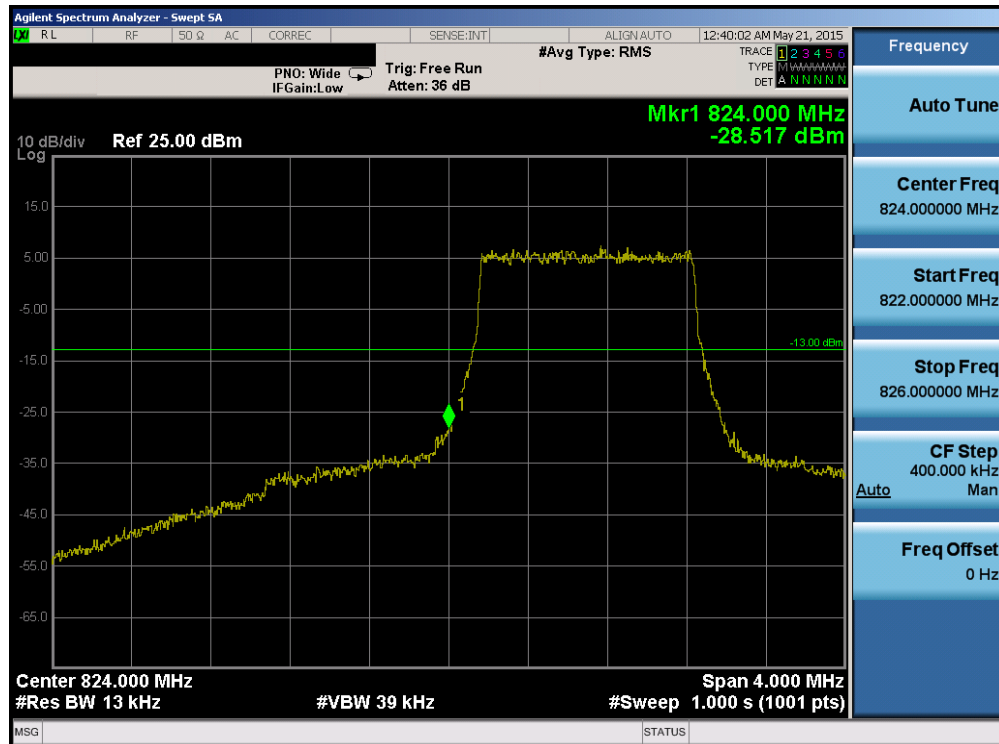
Plot 6-135. Lower Band Edge Plot (Band 5 – 1.4MHz QPSK – RB Size 6)
