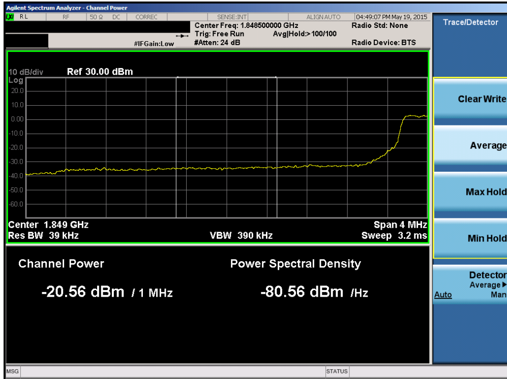
Plot 6-182. Lower Extended Band Edge Plot (Band 2 – 5.0MHz QPSK – RB Size 25)
