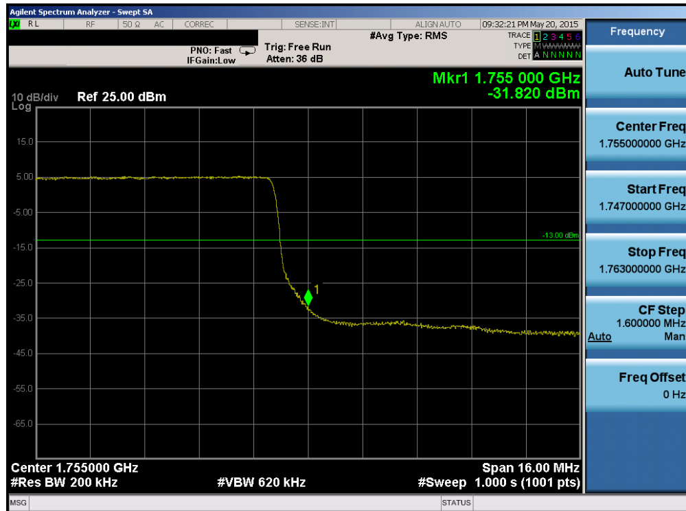
Plot 6-171. Upper Band Edge Plot (Band 4 – 20.0MHz QPSK – RB Size 100)
