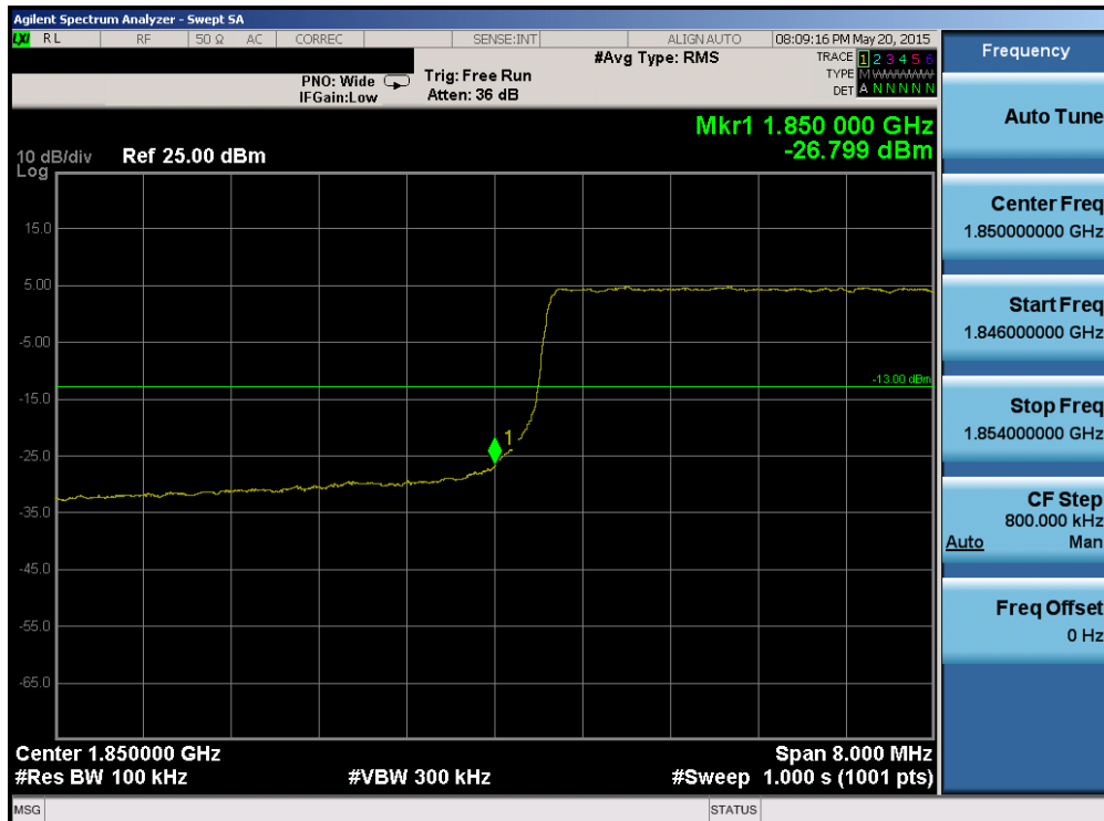
Plot 6-185. Lower Band Edge Plot (Band 2 – 10.0MHz QPSK – RB Size 50)
