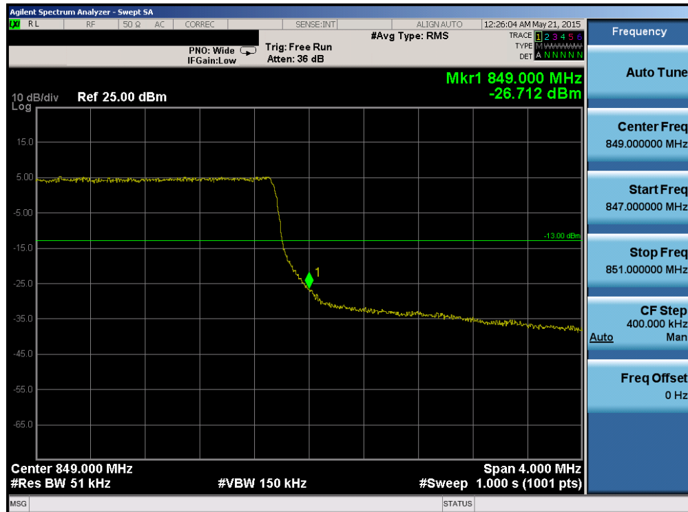
Plot 6-145. Upper Band Edge Plot (Band 5 – 5.0MHz QPSK – RB Size 25)
