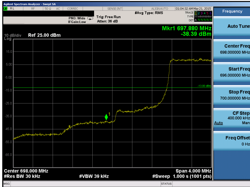
Plot 6-121. Lower Band Edge Plot (Band 12 – 1.4MHz QPSK – RB Size 6)
