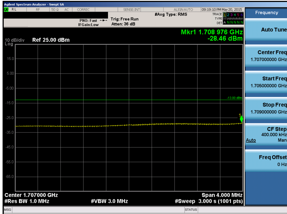
Plot 6-166. Lower Extended Band Edge Plot (Band 4 – 15.0MHz QPSK – RB Size 75)
