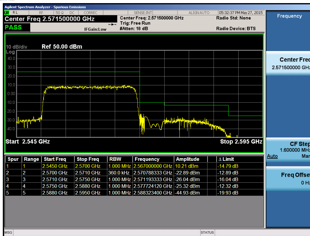
Plot 6-204. Upper ACP Plot (Band 7 – 20.0MHz QPSK – RB Size 100)
