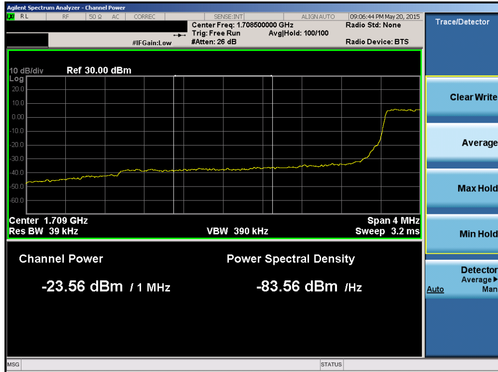
Plot 6-154. Lower Extended Band Edge Plot (Band 4 – 3.0MHz QPSK – RB Size 15)
