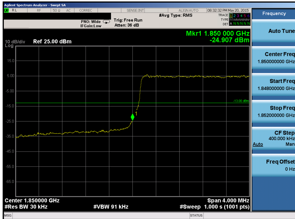
Plot 6-177. Lower Band Edge Plot (Band 2 – 3.0MHz QPSK – RB Size 15)
