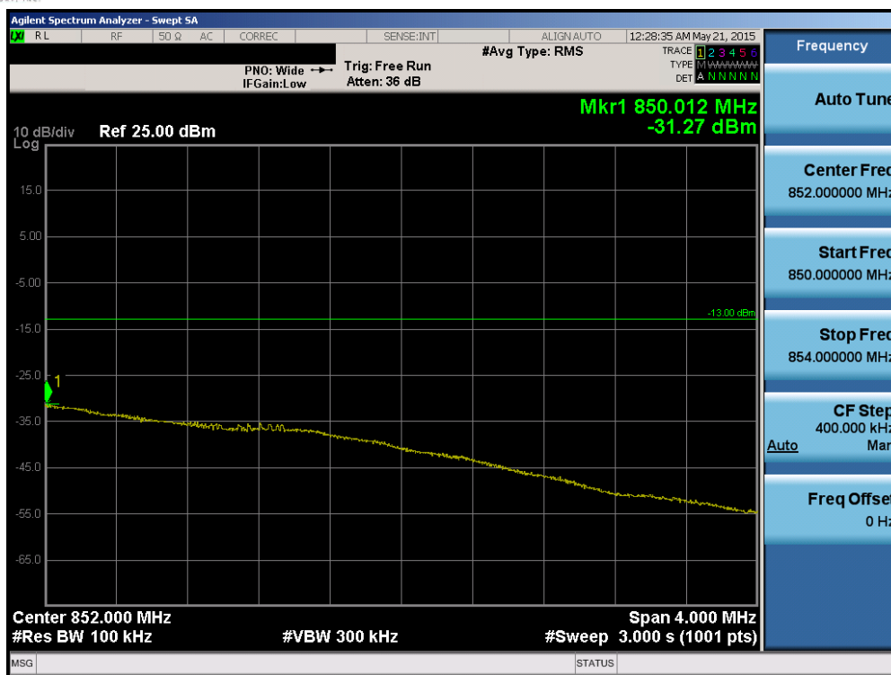
Plot 6-142. Upper Extended Band Edge Plot (Band 5 – Band 5 – 3.0MHz QPSK – RB Size 15)
