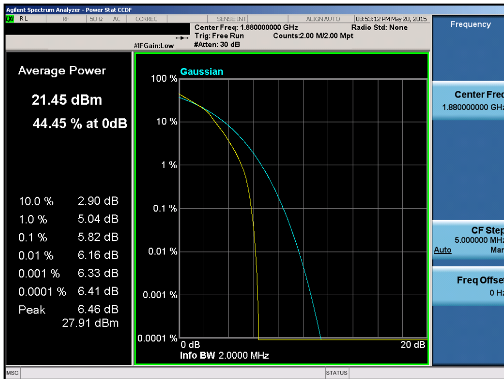
Plot 6-206. PAR Plot (Band 2 – 1.4MHz 16-QAM – RB Size 6)
