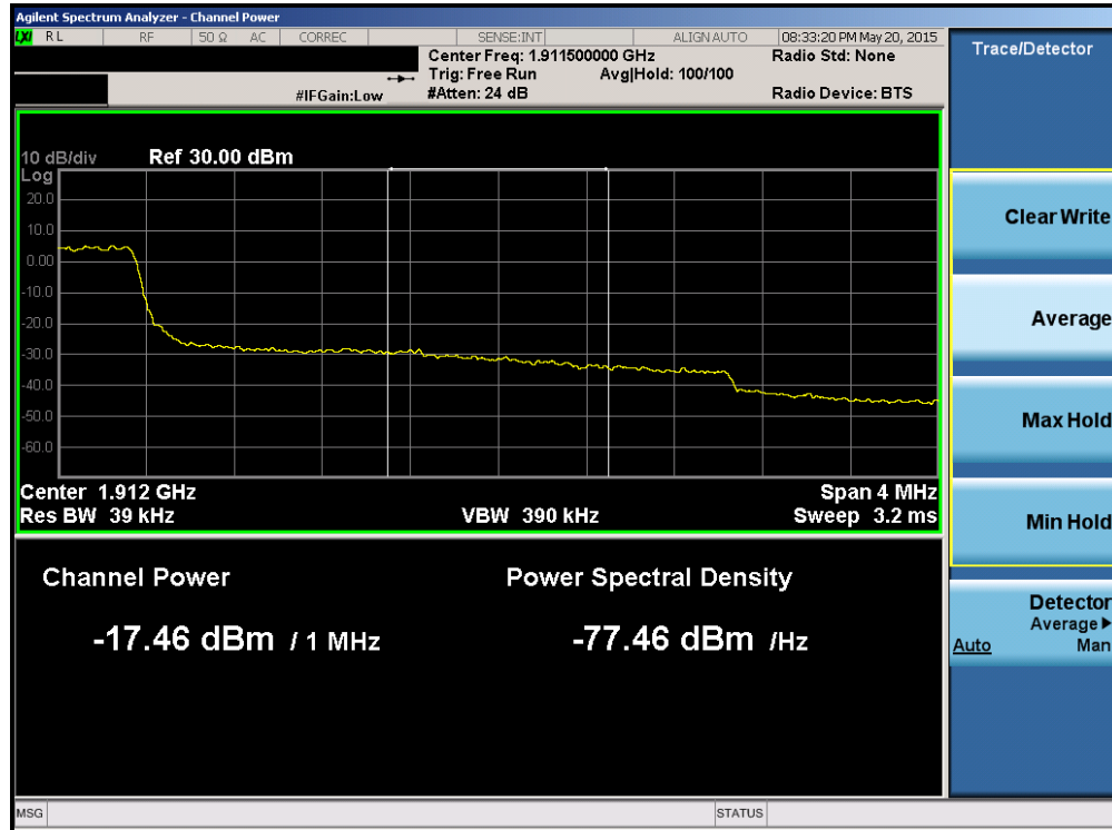
Plot 6-180. Upper Extended Band Edge Plot (Band 2 – 3.0MHz QPSK – RB Size 15)
