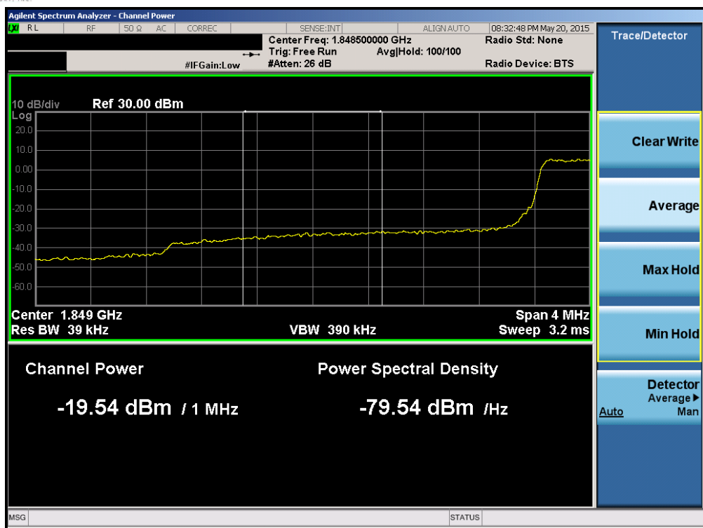
Plot 6-178. Lower Extended Band Edge Plot (Band 2 – 3.0MHz QPSK – RB Size 15)
