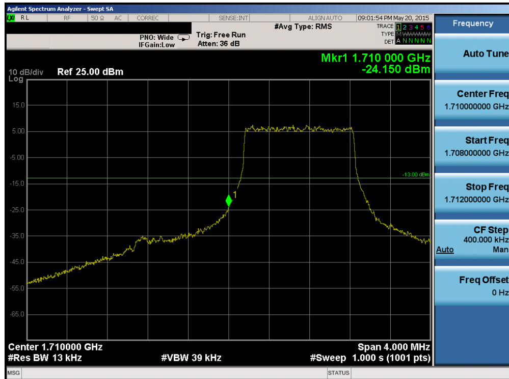
Plot 6-149. Lower Band Edge Plot (Band 4 – 1.4MHz QPSK – RB Size 6)
