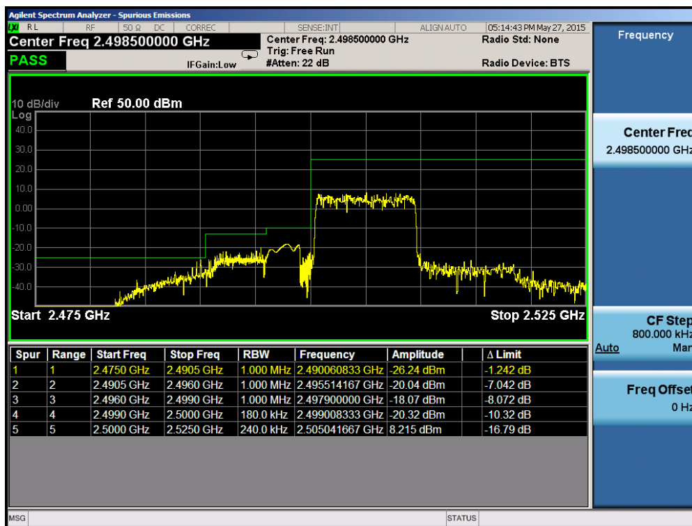
Plot 6-199. Lower ACP Plot (Band 7 – 10.0MHz QPSK – RB Size 50)
