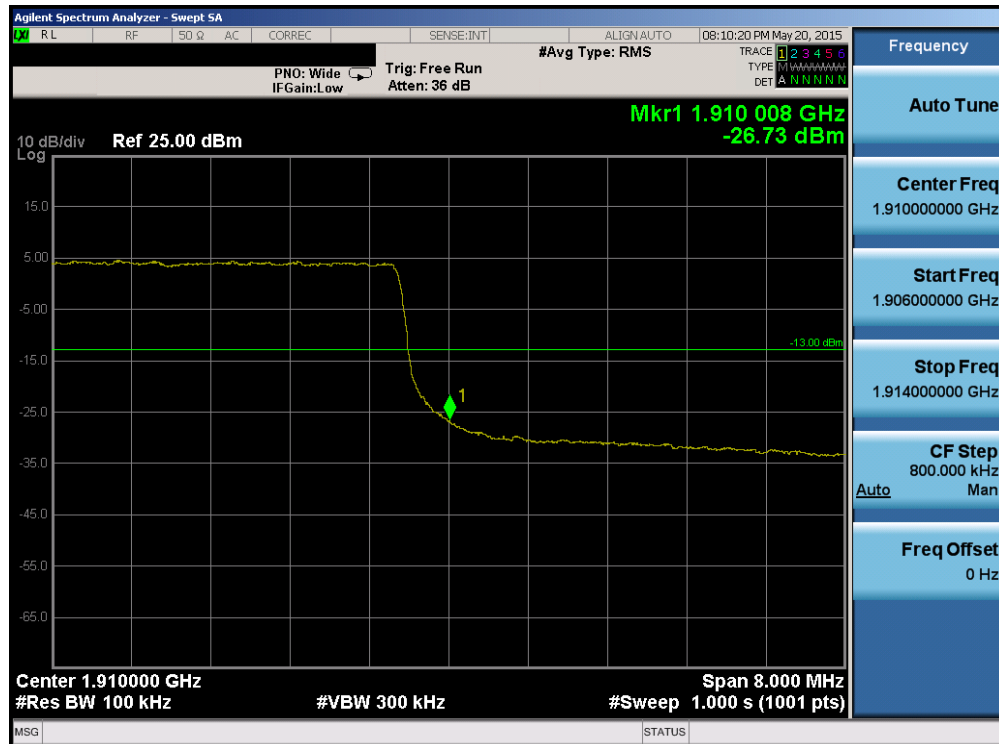
Plot 6-187. Upper Band Edge Plot (Band 2 – 10.0MHz QPSK – RB Size 50)
