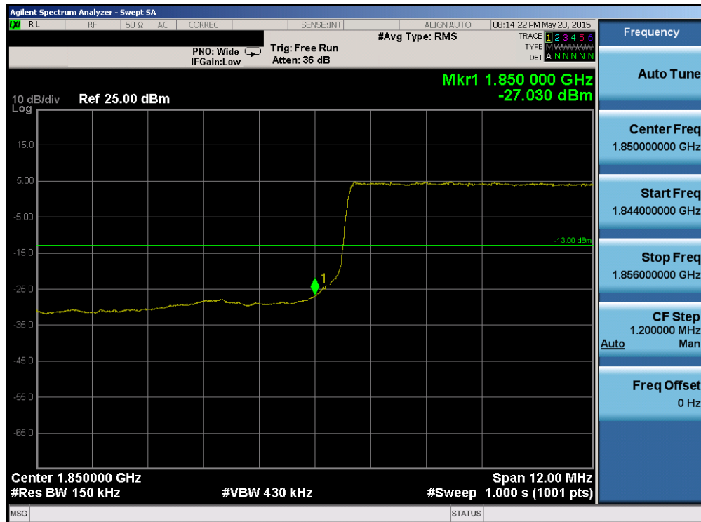
Plot 6-189. Lower Band Edge Plot (Band 2 – 15.0MHz QPSK – RB Size 75)
