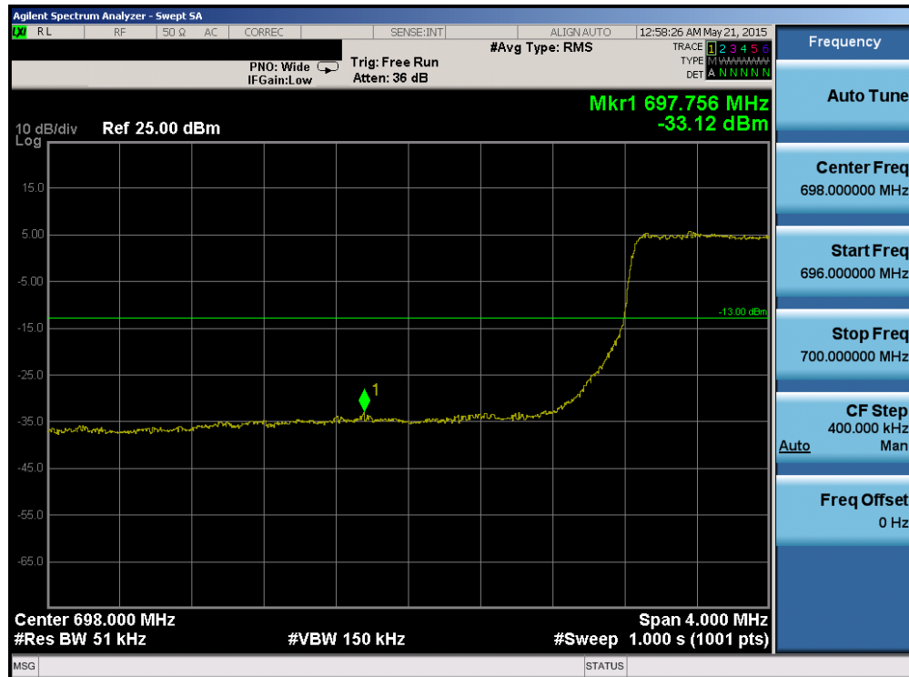
Plot 6-129. Lower Band Edge Plot (Band 12 – 5.0MHz QPSK – RB Size 25)
