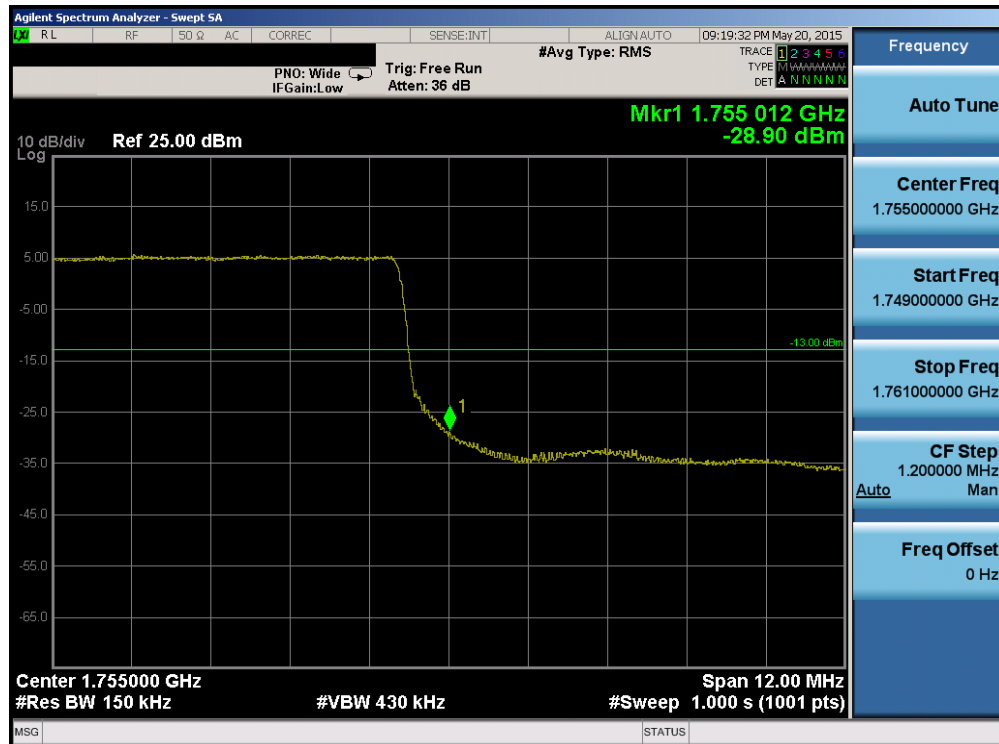
Plot 6-167. Upper Band Edge Plot (Band 4 – 15.0MHz QPSK – RB Size 75)
