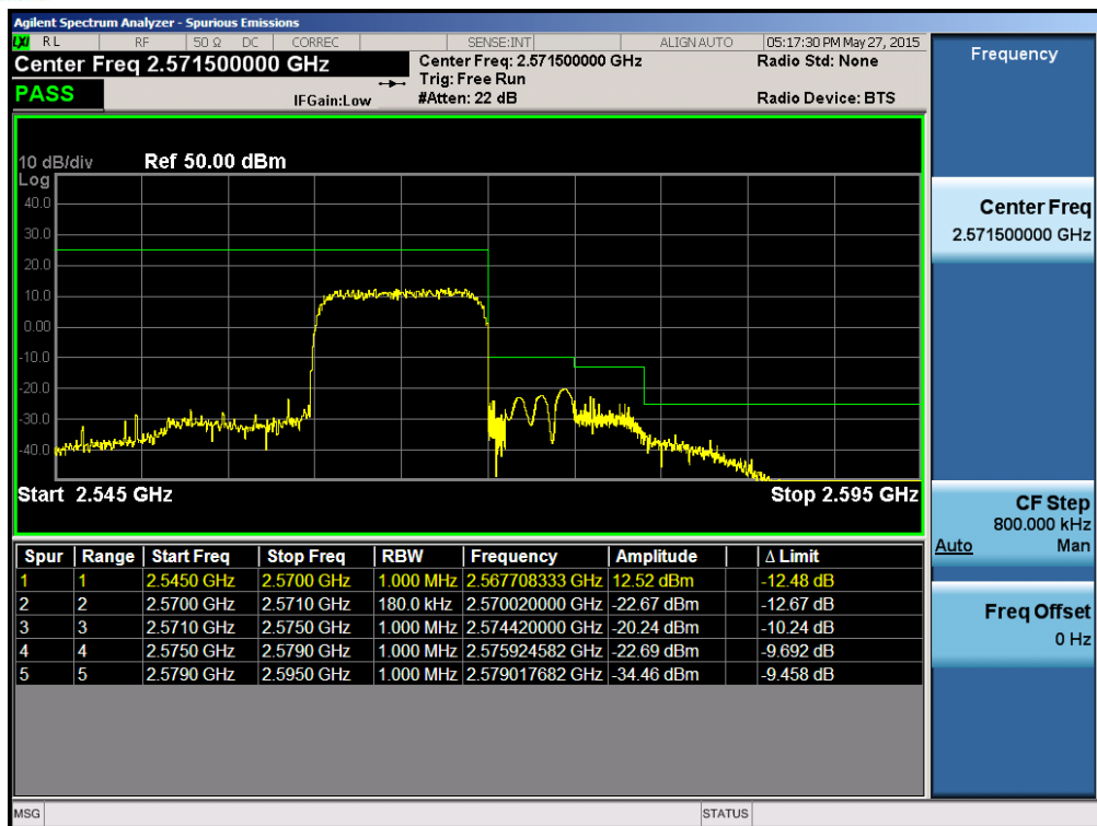
Plot 6-200. Upper ACP Plot (Band 7 – 10.0MHz QPSK – RB Size 50)
