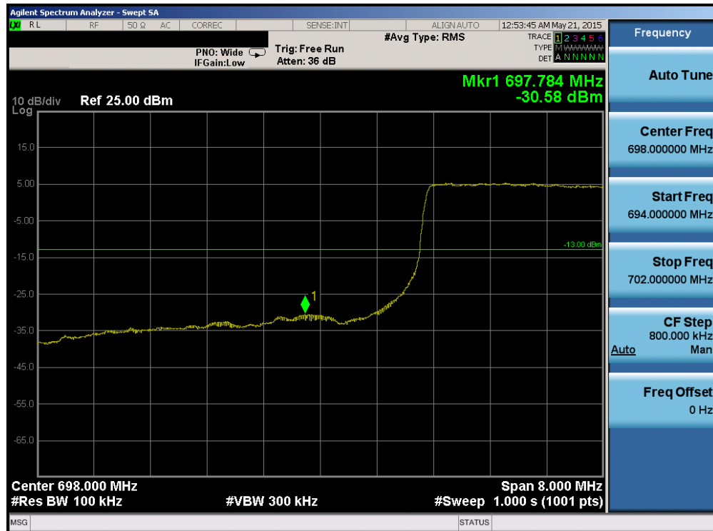
Plot 6-133. Lower Band Edge Plot (Band 12 – 10.0MHz QPSK – RB Size 50)
