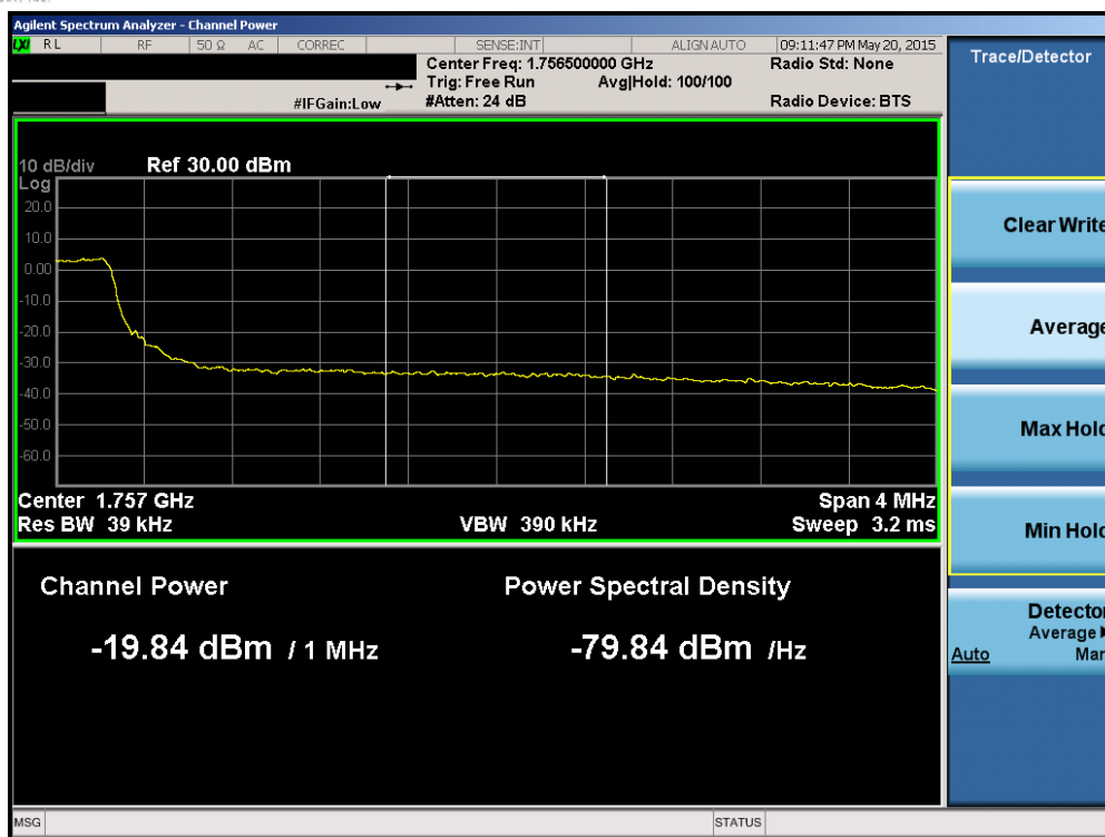
Plot 6-160. Upper Extended Band Edge Plot (Band 4 – 5.0MHz QPSK – RB Size 25)
