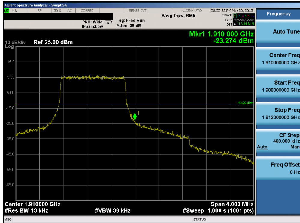
Plot 6-175. Upper Band Edge Plot (Band 2 – 1.4MHz QPSK – RB Size 6)
