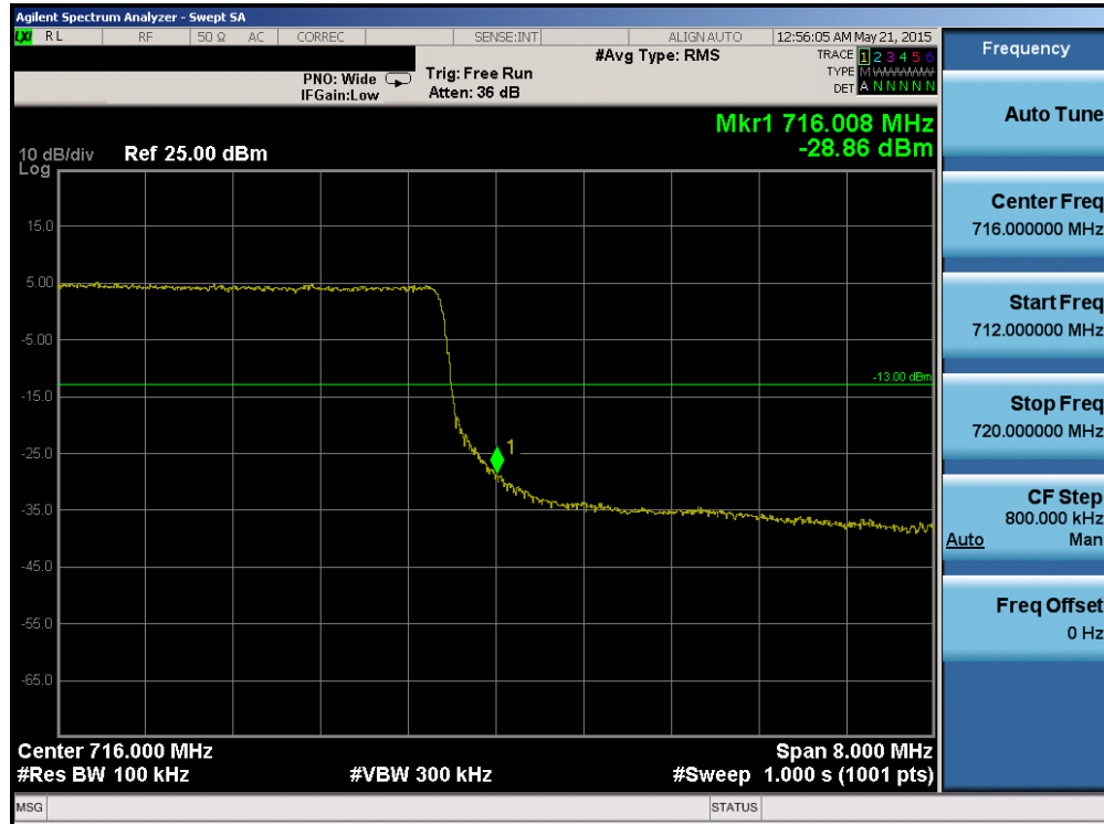
Plot 6-134. Upper Band Edge Plot (Band 12 – 10.0MHz QPSK – RB Size 50)
