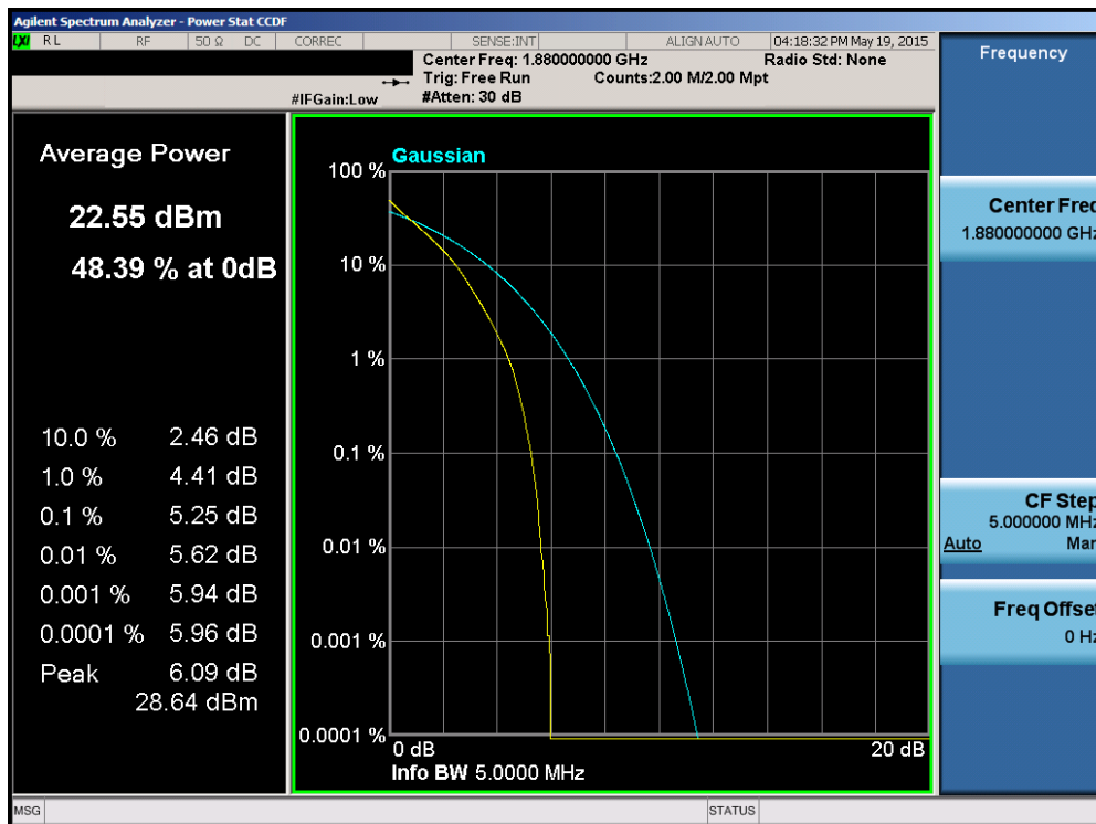
Plot 6-210. PAR Plot (Band 2 – 5.0MHz 16-QAM – RB Size 25)
