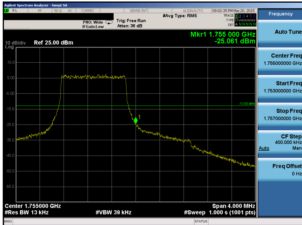
Plot 6-151. Upper Band Edge Plot (Band 4 – 1.4MHz QPSK – RB Size 6)
