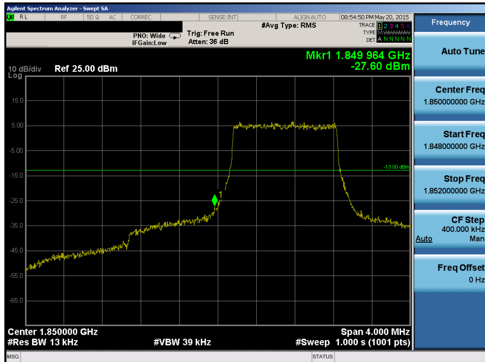
Plot 6-173. Lower Band Edge Plot (Band 2 – 1.4MHz QPSK – RB Size 6)
