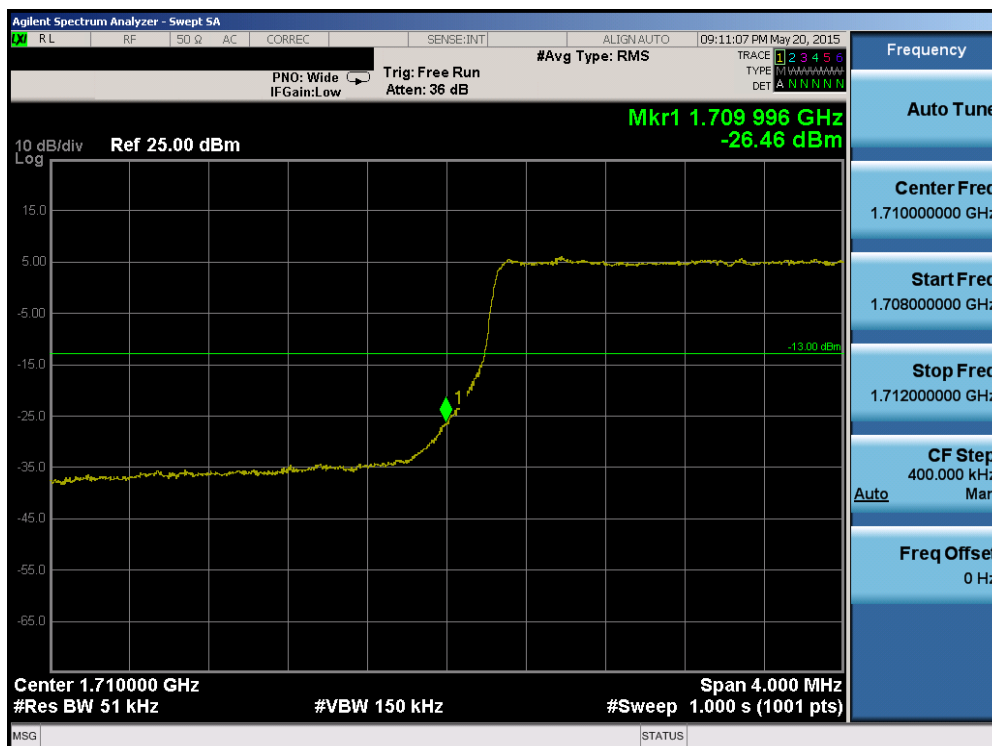
Plot 6-157. Lower Band Edge Plot (Band 4 – 5.0MHz QPSK – RB Size 25)
