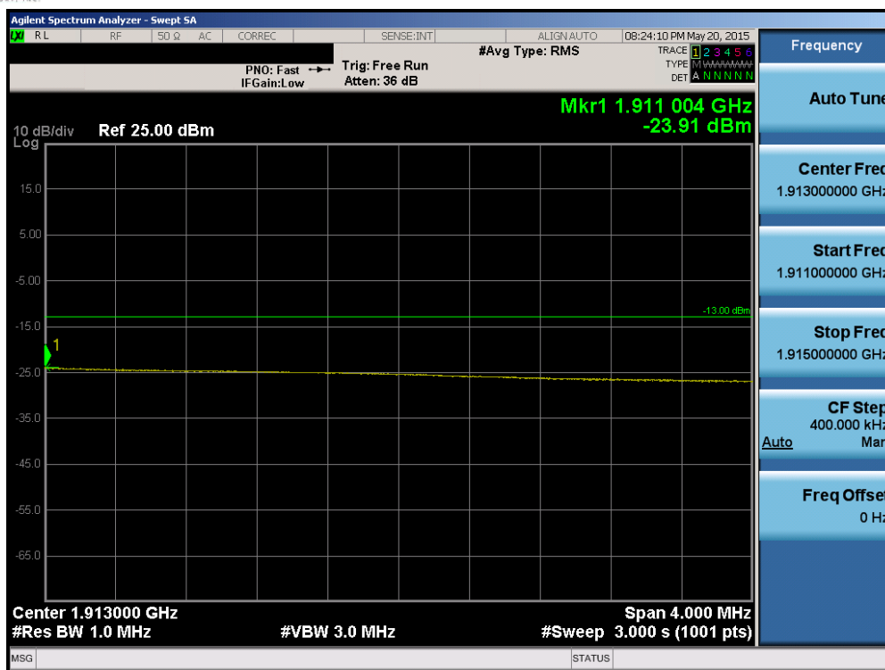
Plot 6-196. Upper Extended Band Edge Plot (Band 2 – 20.0MHz QPSK – RB Size 100)
