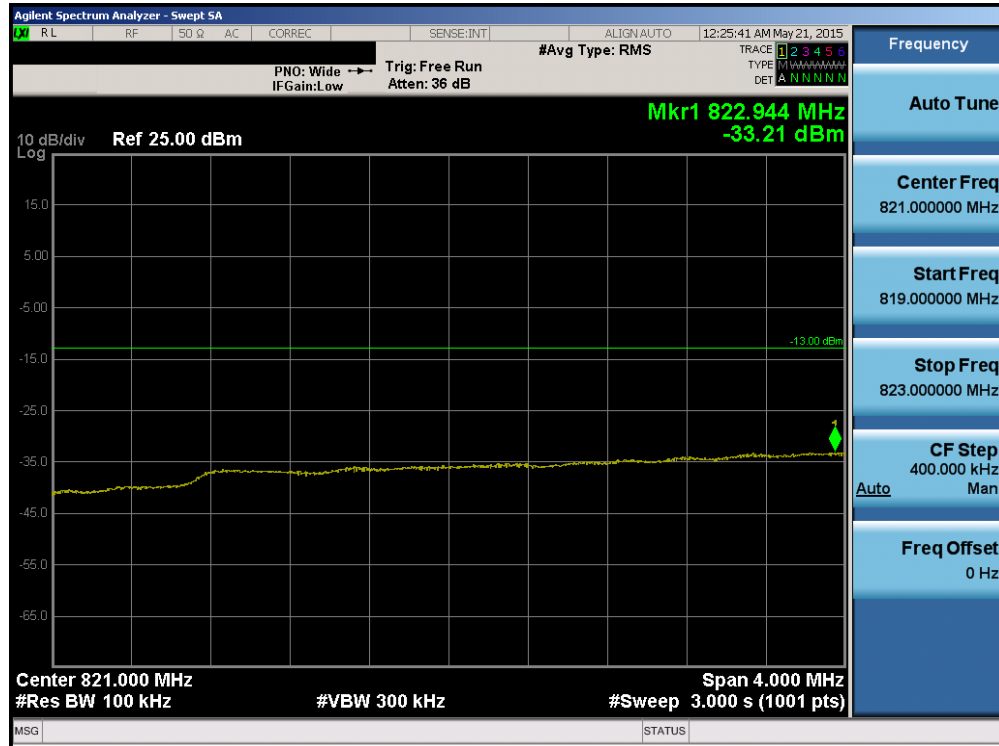
Plot 6-144. Lower Extended Band Edge Plot (Band 5 – 5.0MHz QPSK – RB Size 25)
