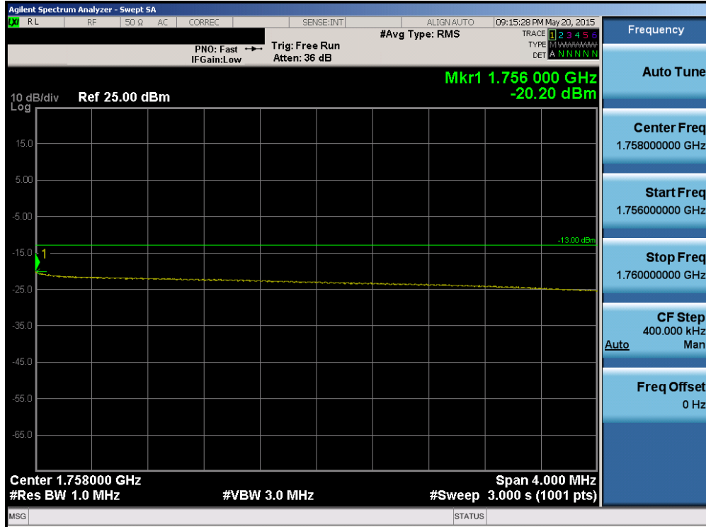
Plot 6-164. Upper Extended Band Edge Plot (Band 4 – 10.0MHz QPSK – RB Size 50)
