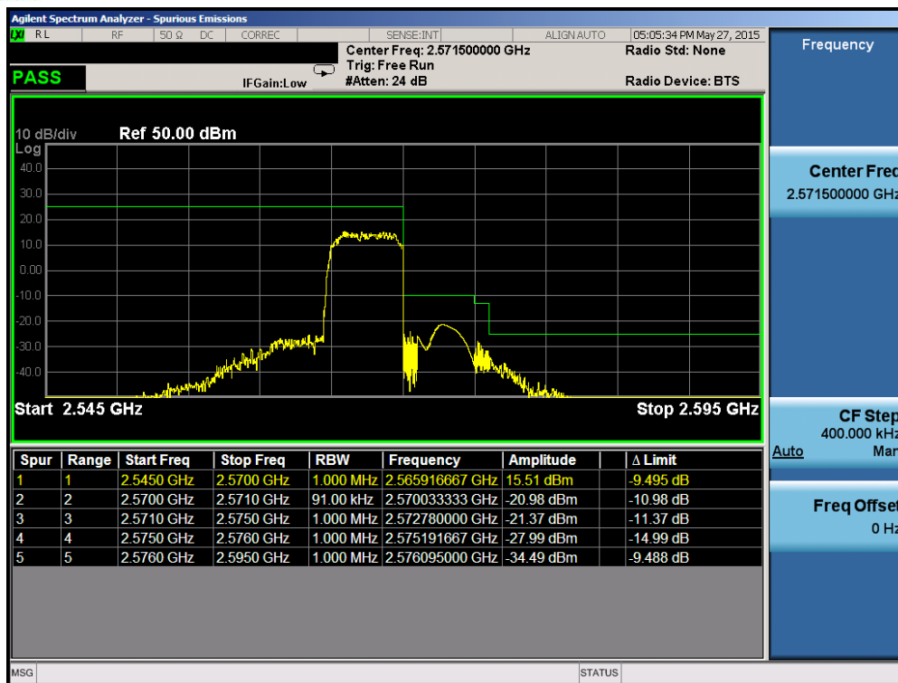
Plot 6-198. Upper ACP Plot (Band 7 – 5.0MHz QPSK – RB Size 25)
