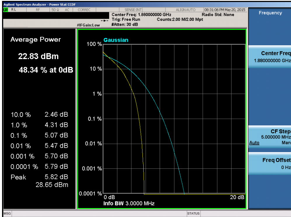
Plot 6-208. PAR Plot (Band 2 – 3.0MHz 16-QAM – RB Size 15)
