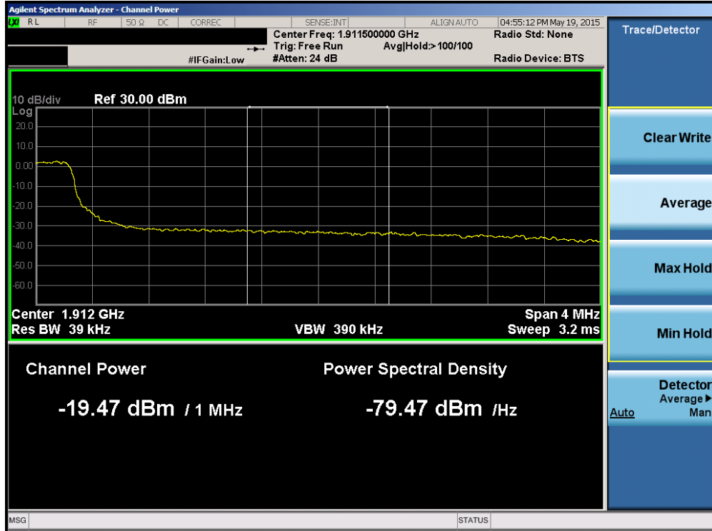
Plot 6-184. Upper Extended Band Edge Plot (Band 2 – 5.0MHz QPSK – RB Size 25)
