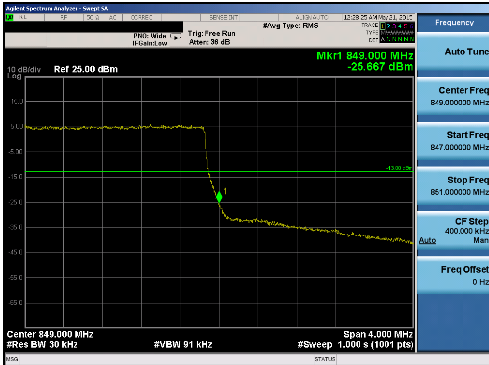
Plot 6-141. Upper Band Edge Plot (Band 5 – 3.0MHz QPSK – RB Size 15)
