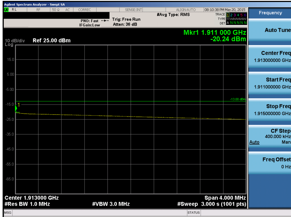
Plot 6-188. Upper Extended Band Edge Plot (Band 2 – 10.0MHz QPSK – RB Size 50)
