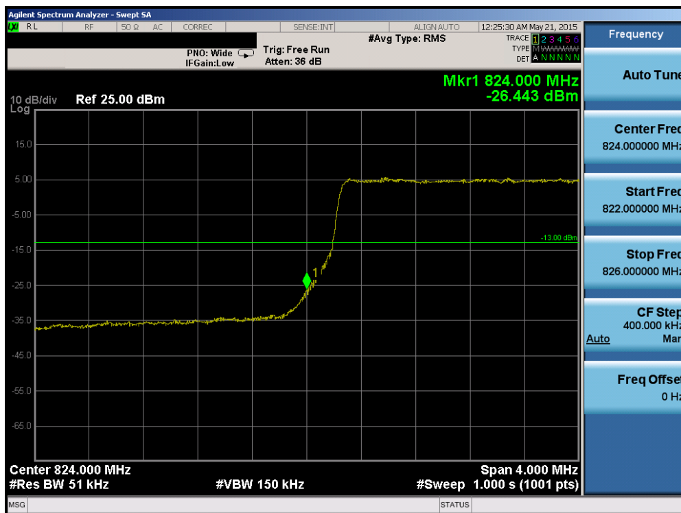
Plot 6-143. Lower Band Edge Plot (Band 5 – 5.0MHz QPSK – RB Size 25)
