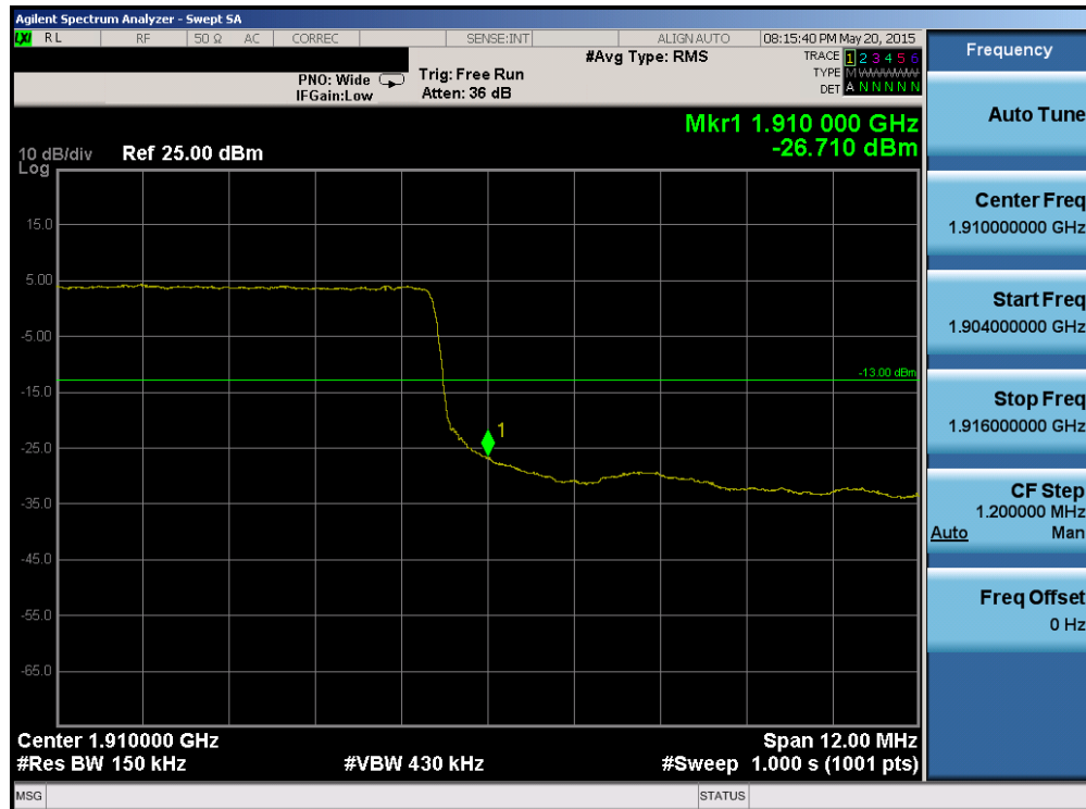
Plot 6-191. Upper Band Edge Plot (Band 2 – 15.0MHz QPSK – RB Size 75)
