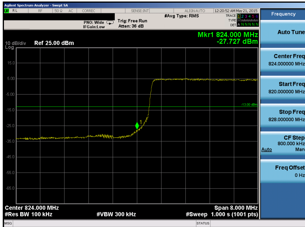
Plot 6-147. Lower Band Edge Plot (Band 5 – 10.0MHz QPSK – RB Size 50)
