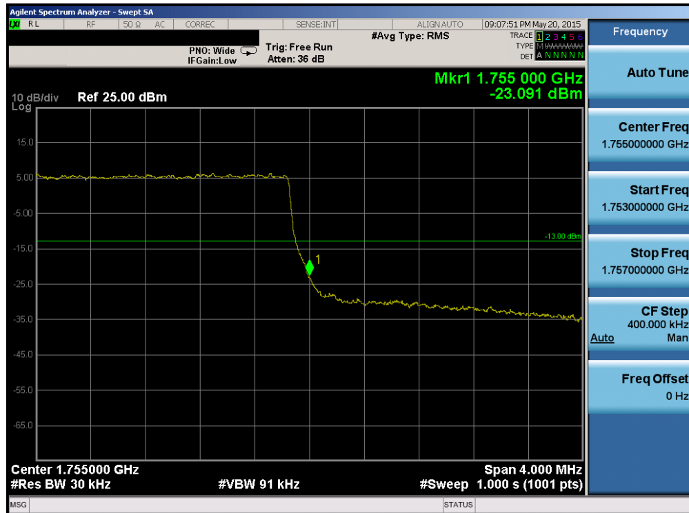
Plot 6-155. Upper Band Edge Plot (Band 4 – 3.0MHz QPSK – RB Size 15)
