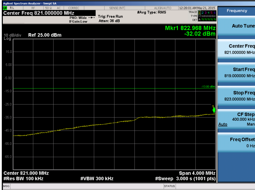
Plot 6-140. Lower Extended Band Edge Plot (Band 5 – 3.0MHz QPSK – RB Size 15)
