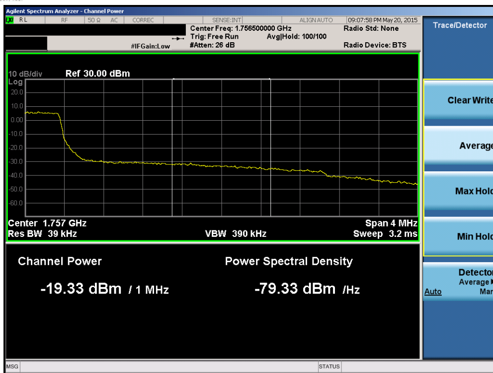
Plot 6-156. Upper Extended Band Edge Plot (Band 4 – 3.0MHz QPSK – RB Size 15)
