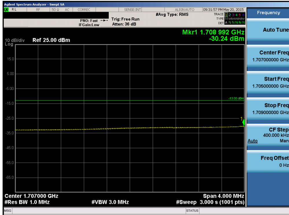
Plot 6-170. Lower Extended Band Edge Plot (Band 4 – 20.0MHz QPSK – RB Size 100)
