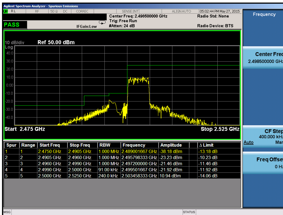
Plot 6-197. Lower ACP Plot (Band 7 – 5.0MHz QPSK – RB Size 25)
