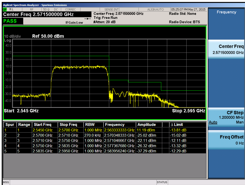
Plot 6-202. Upper ACP Plot (Band 7 – 15.0MHz QPSK – RB Size 75)
