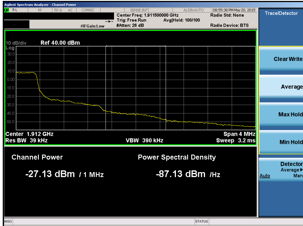
Plot 6-176. Upper Extended Band Edge Plot (Band 2 – 1.4MHz QPSK – RB Size 6)
