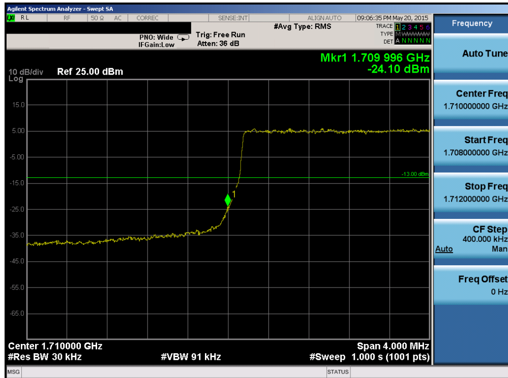
Plot 6-153. Lower Band Edge Plot (Band 4 – 3.0MHz QPSK – RB Size 15)
