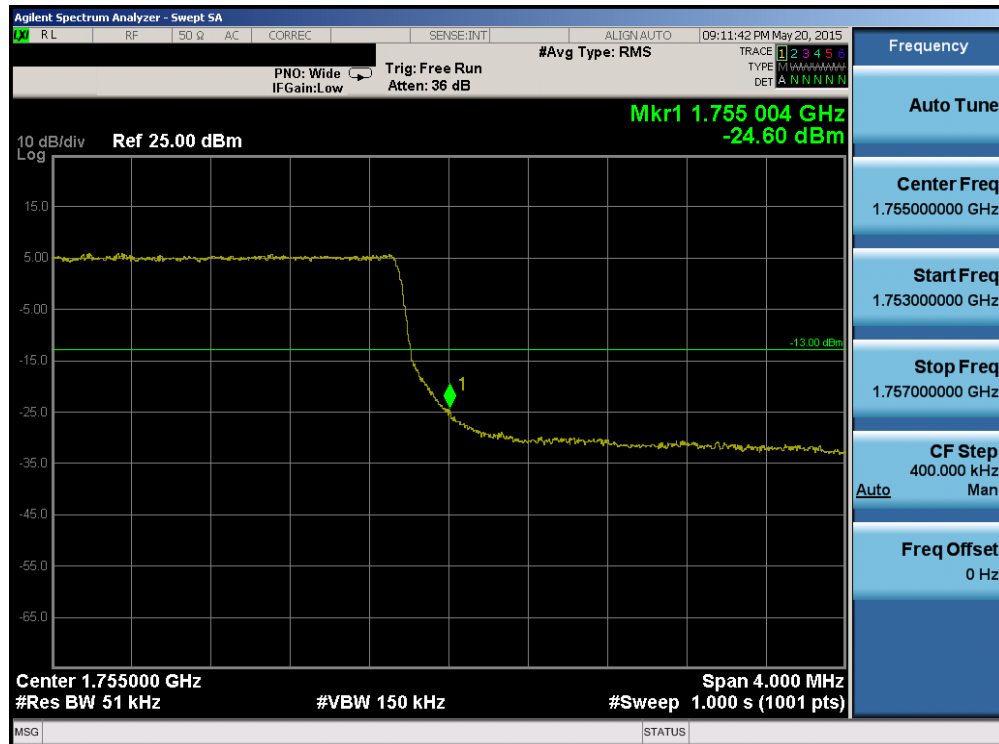
Plot 6-159. Upper Band Edge Plot (Band 4 – 5.0MHz QPSK – RB Size 25)
