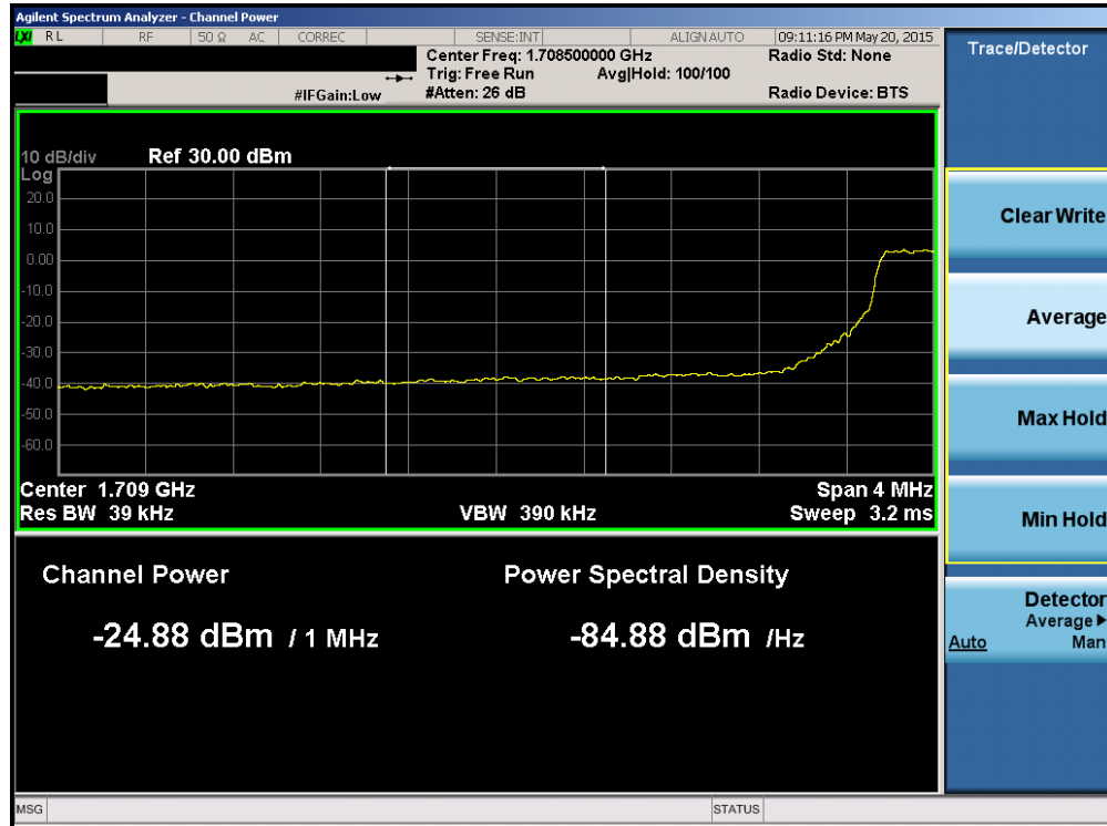
Plot 6-158. Lower Extended Band Edge Plot (Band 4 – 5.0MHz QPSK – RB Size 25)
