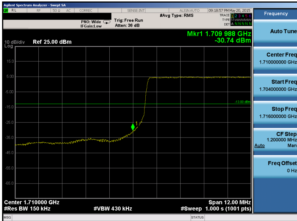
Plot 6-165. Lower Band Edge Plot (Band 4 – 15.0MHz QPSK – RB Size 75)
