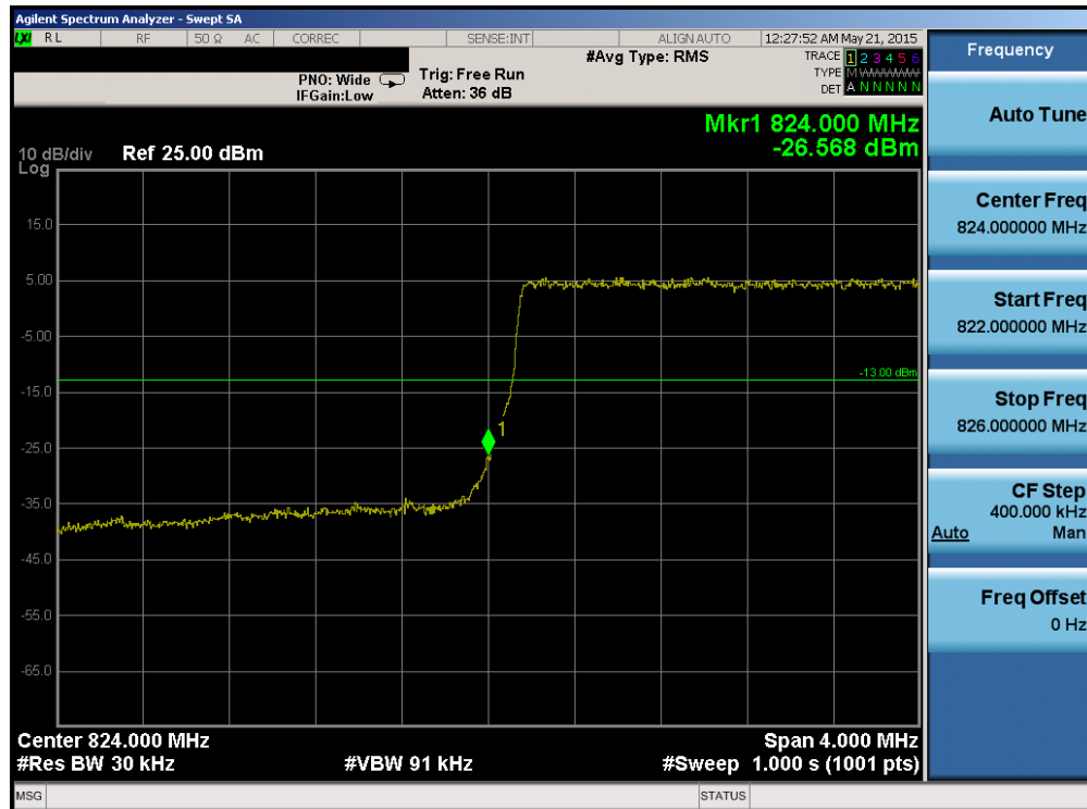
Plot 6-139. Lower Band Edge Plot (Band 5 – 3.0MHz QPSK – RB Size 15)
