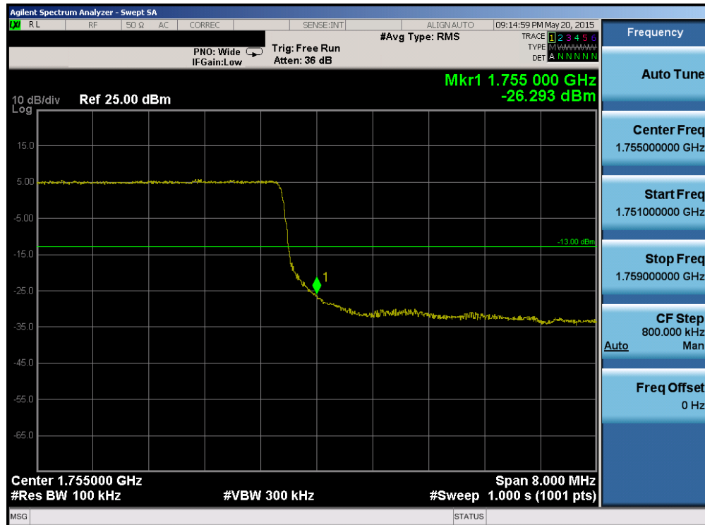
Plot 6-163. Upper Band Edge Plot (Band 4 – 10.0MHz QPSK – RB Size 50)
