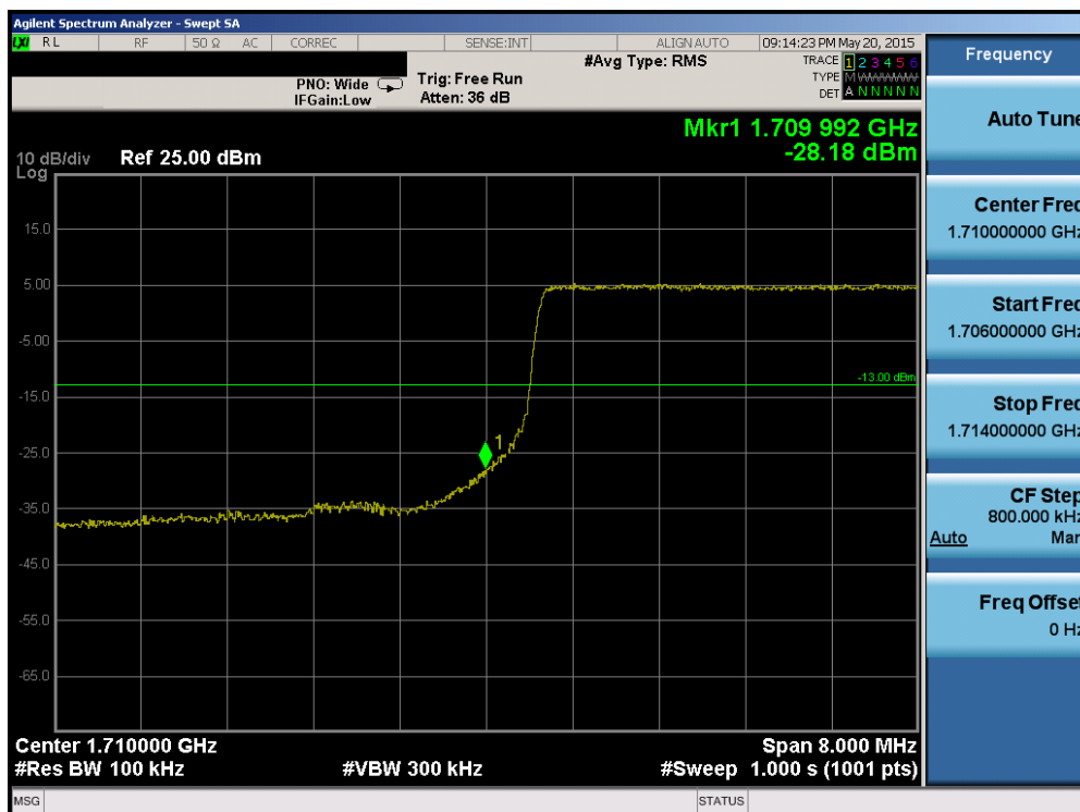
Plot 6-161. Lower Band Edge Plot (Band 4 – 10.0MHz QPSK – RB Size 50)
