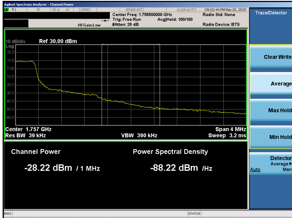
Plot 6-152. Upper Extended Band Edge Plot (Band 4 – 1.4MHz QPSK – RB Size 6)
