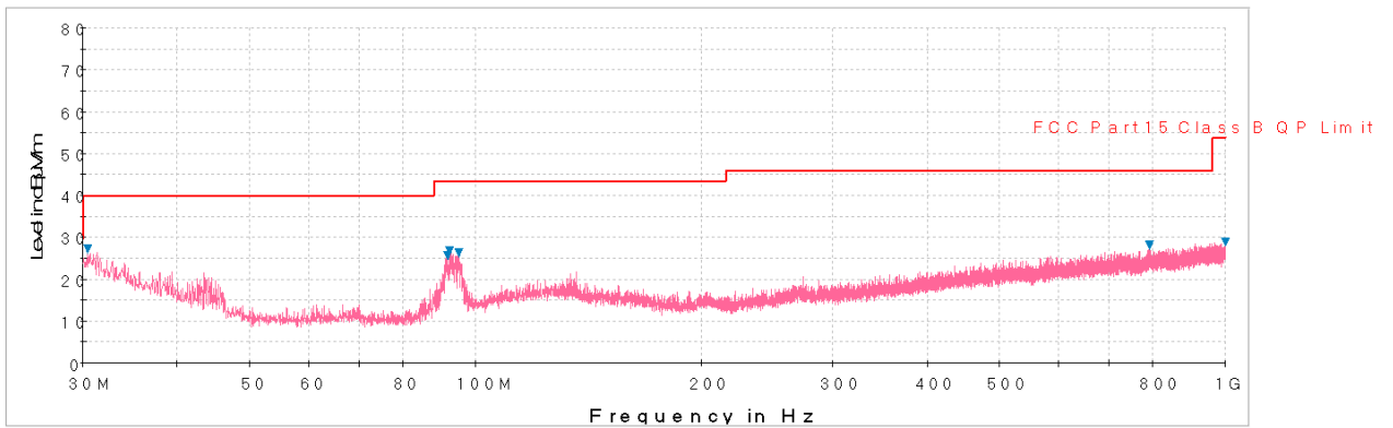
Plot 6-42. Radiated Spurious Plot below 1GHz (Pol. V)
