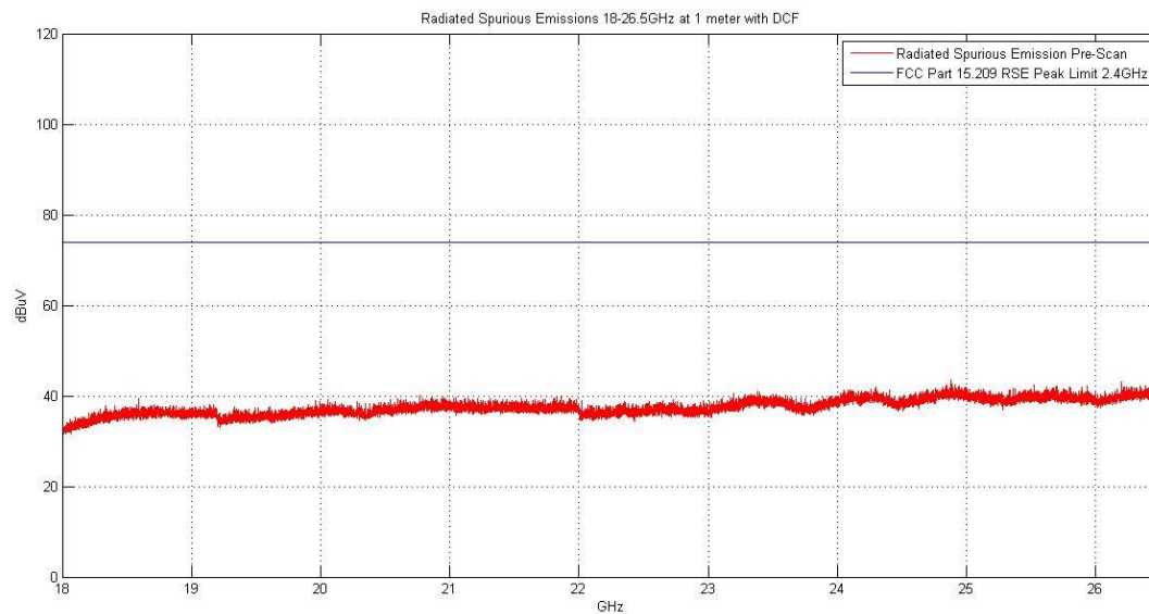
Plot 6-24. Radiated Spurious Plot above 18GHz (Pol. H)
