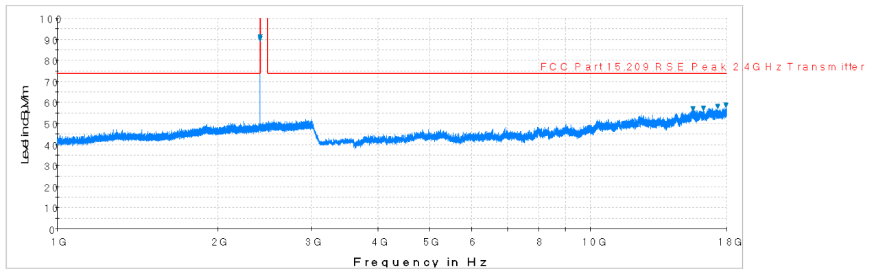
Plot 6-18. Radiated Spurious Plot above 1GHz (BTLE – Ch. 0, Ant. Pol. H)
