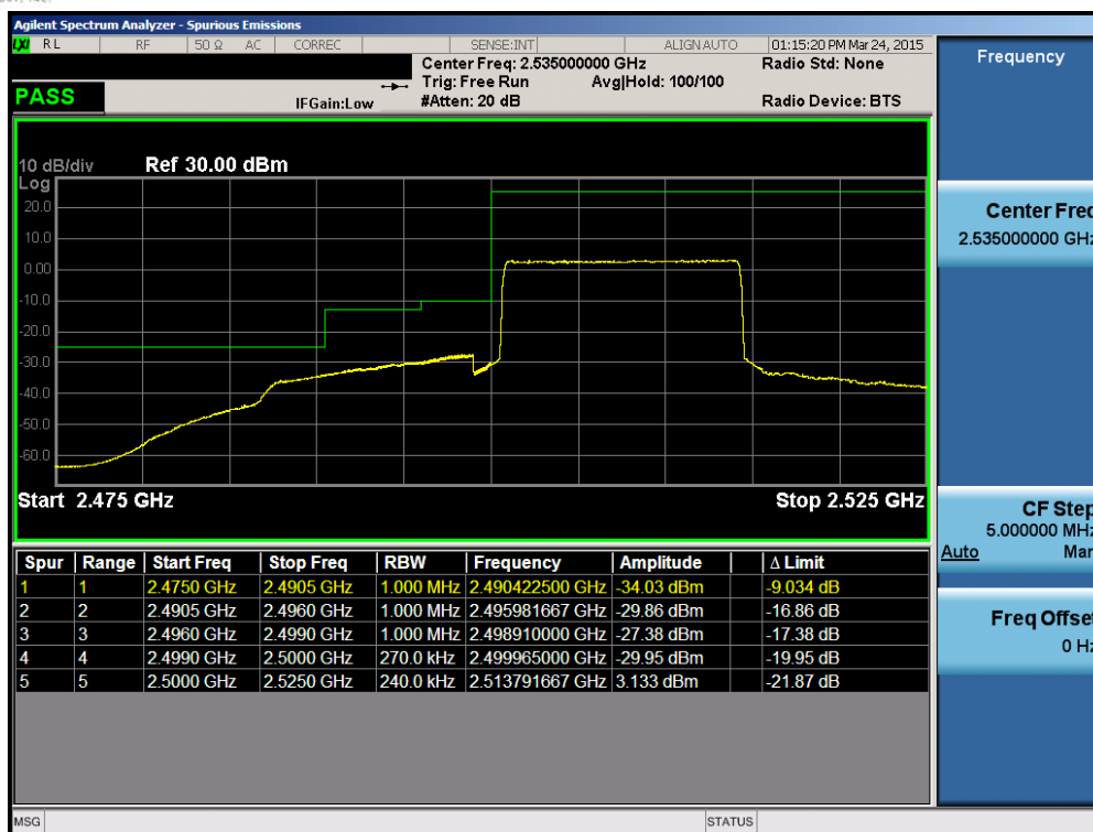
Plot 6-174. Lower ACP Plot (Band 7 – 15.0MHz QPSK – RB Size 75)
