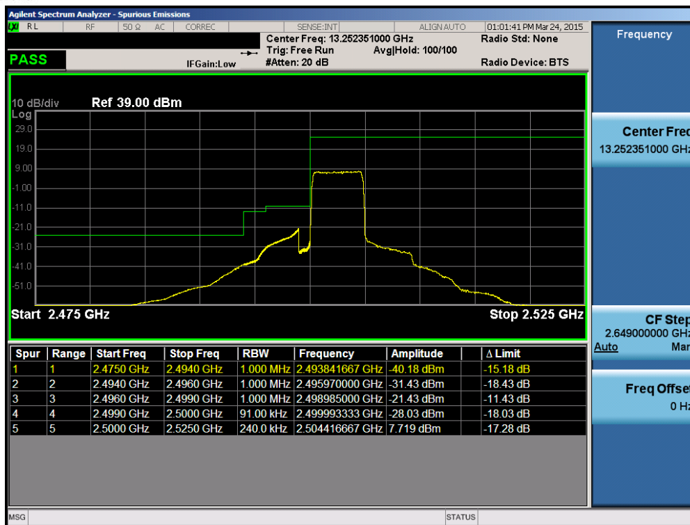
Plot 6-170. Lower ACP Plot (Band 7 – 5.0MHz QPSK – RB Size 25)
