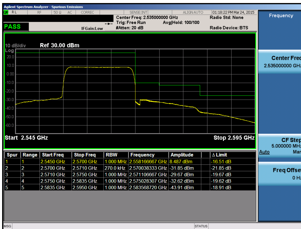
Plot 6-175. Upper ACP Plot (Band 7 – 15.0MHz QPSK – RB Size 75)
