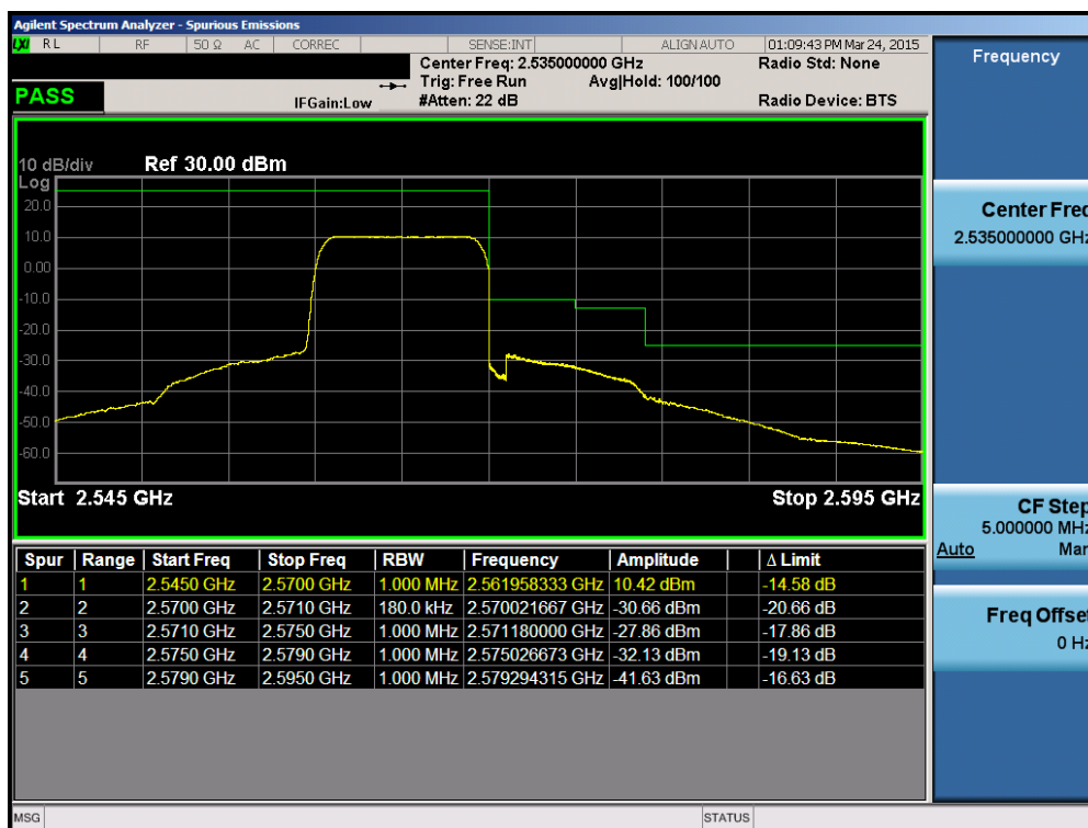
Plot 6-173. Upper ACP Plot (Band 7 – 10.0MHz QPSK – RB Size 50)
