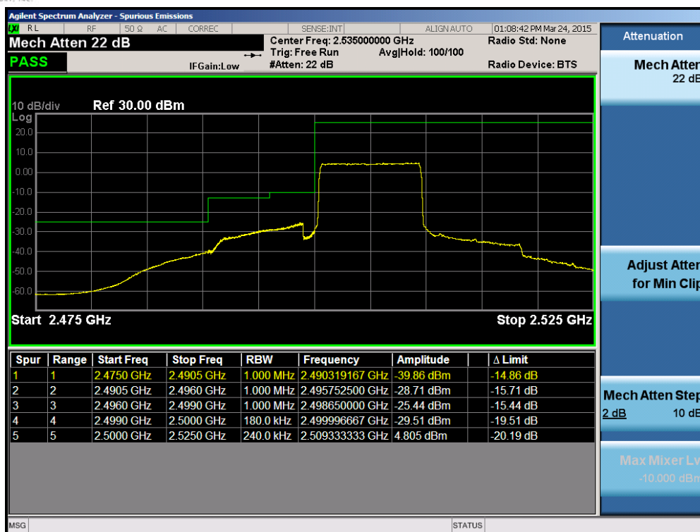
Plot 6-172. Lower ACP Plot (Band 7 – 10.0MHz QPSK – RB Size 50)
