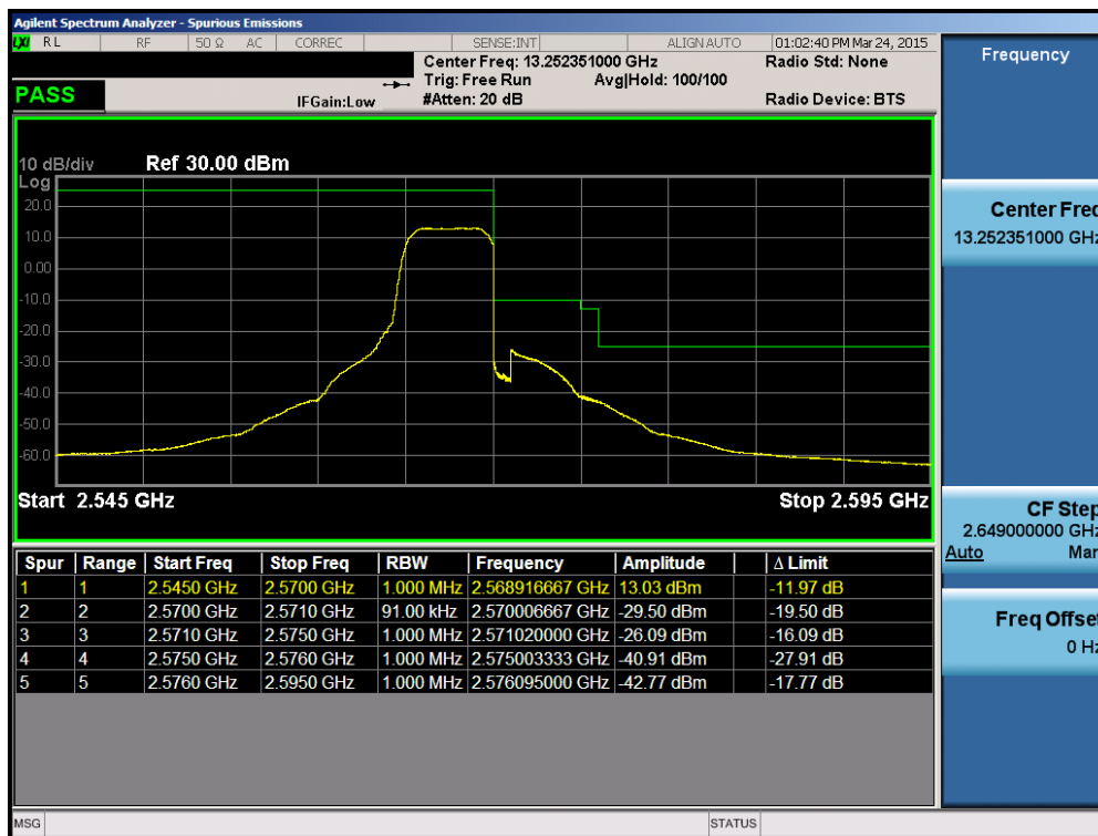
Plot 6-171. Upper ACP Plot (Band 7 – 5.0MHz QPSK – RB Size 25)
