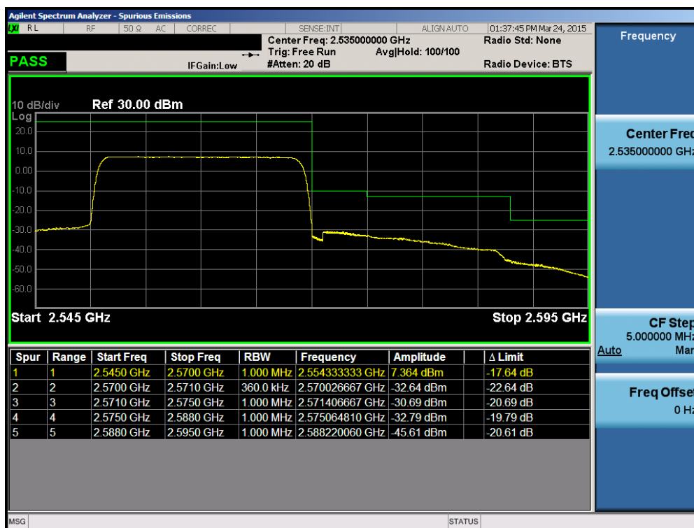
Plot 6-177. Upper ACP Plot (Band 7 – 20.0MHz QPSK – RB Size 100)
