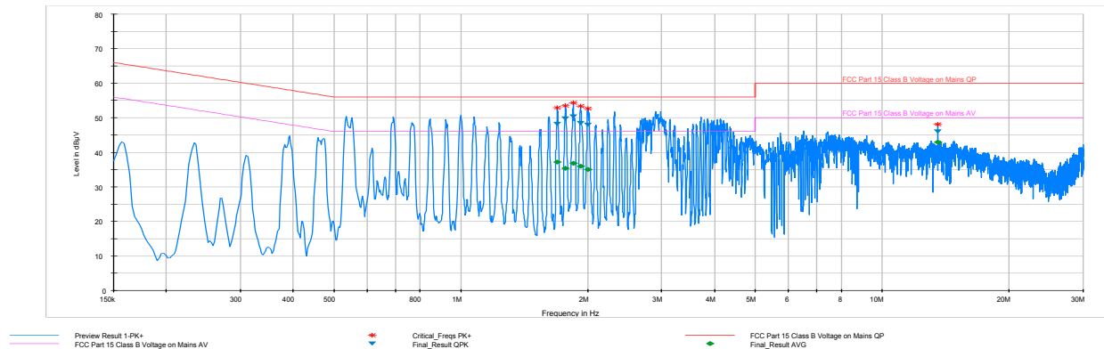
Plot 7-2. Line-Conducted Test Plot (N)
