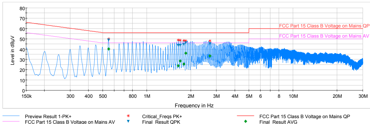
Plot 6-25. Line Conducted Plot with Bluetooth LE (N)
