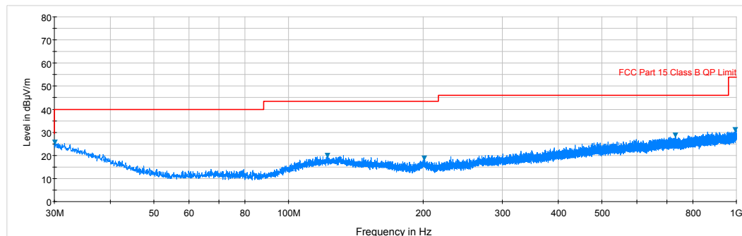
Plot 6-22. Radiated Spurious Plot below 1GHz (Pol. H)
