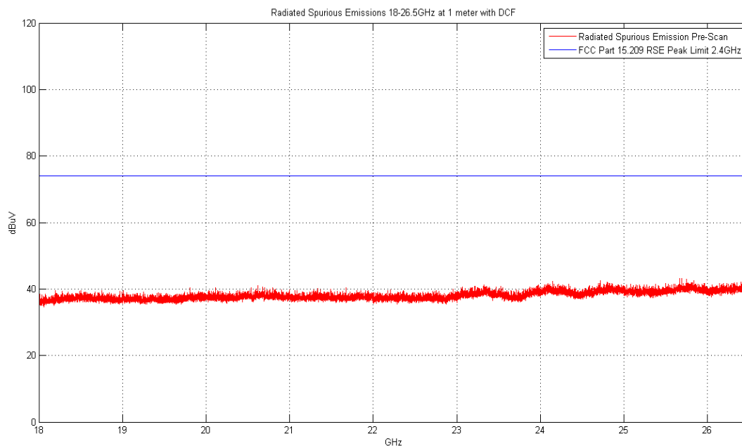
Plot 6-18. Radiated Spurious Plot above 18GHz (Pol. H)
