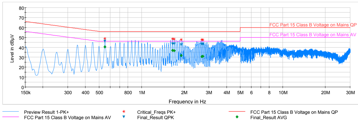
Plot 6-24. Line Conducted Plot with Bluetooth LE (L1)
