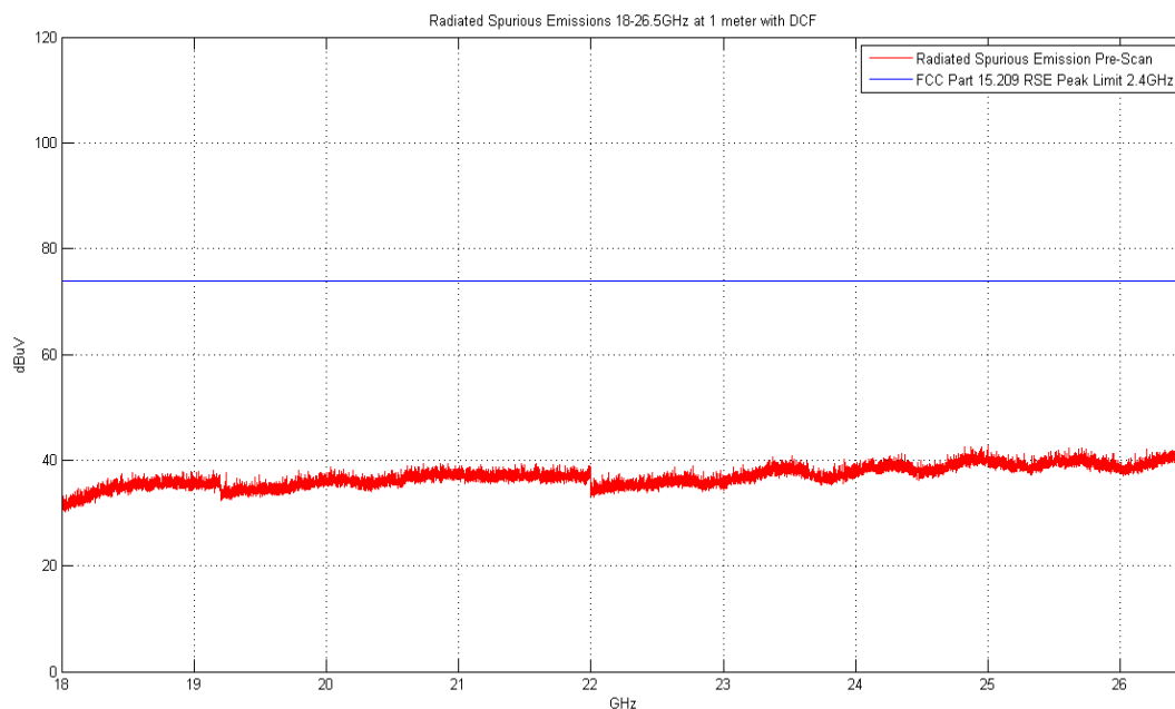
Plot 6-19. Radiated Spurious Plot above 18GHz (Pol. V)
