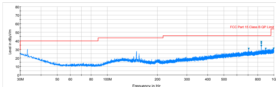
Plot 6-23. Radiated Spurious Plot below 1GHz (Pol. V)
