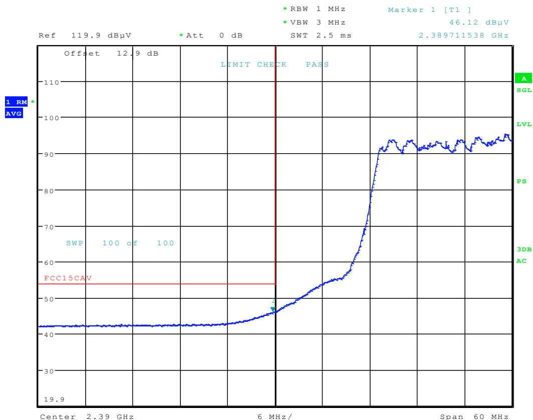
Plot 6-39. Radiated Restricted Lower Band Edge Measurement (Average)
