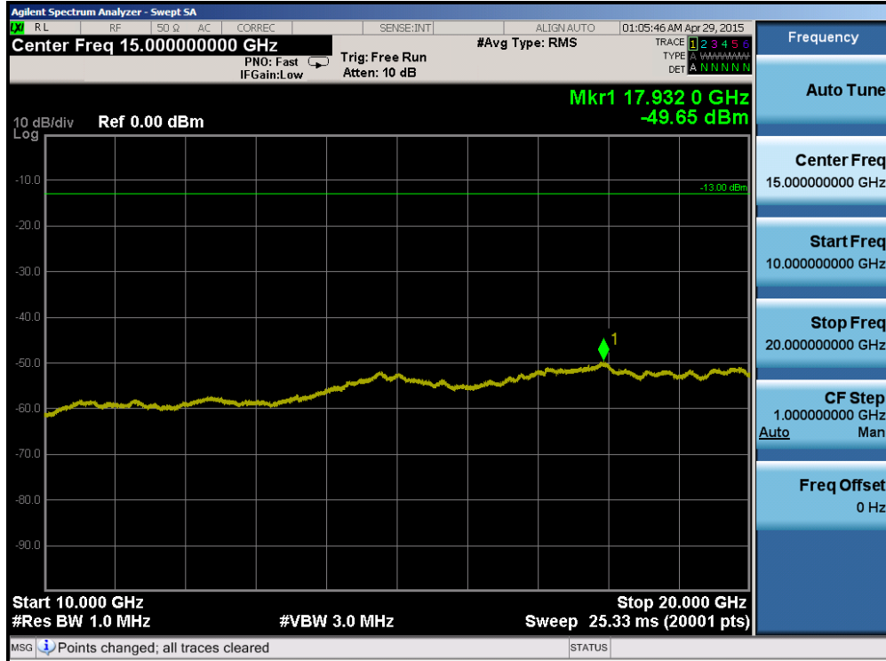
Plot 6-57. Conducted Spurious Plot (Band 4 – 5.0MHz QPSK – RB Size 1, RB Offset 0 – Low Channel)
