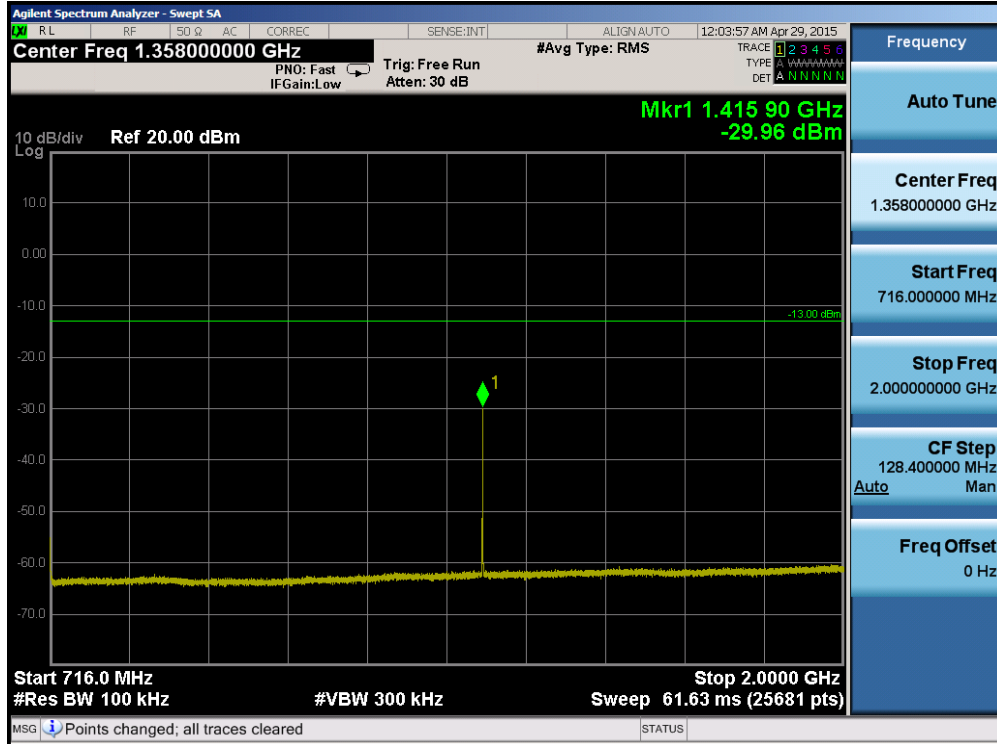
Plot 6-41. Conducted Spurious Plot (Band 17 – 5.0MHz QPSK – RB Size 1, RB Offset 0 – Mid Channel)
