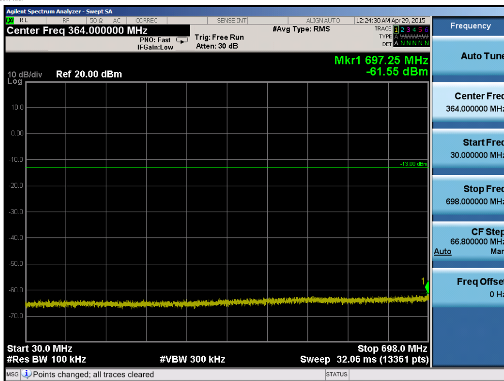
Plot 6-43. Conducted Spurious Plot (Band 17 – 5.0MHz QPSK – RB Size 1, RB Offset 0 – High Channel)
