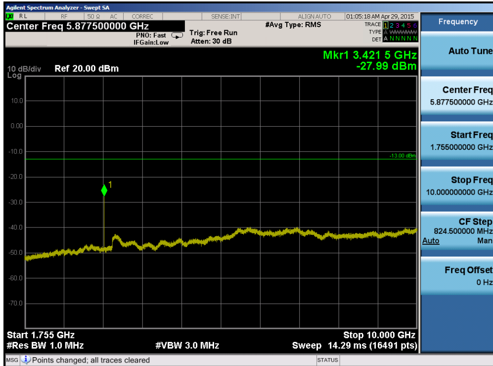
Plot 6-56. Conducted Spurious Plot (Band 4 – 5.0MHz QPSK – RB Size 1, RB Offset 0 – Low Channel)
