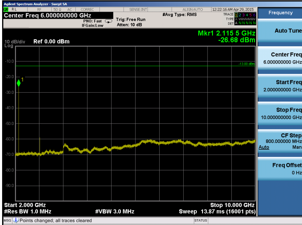
Plot 6-39. Conducted Spurious Plot (Band 17 – 5.0MHz QPSK – RB Size 1, RB Offset 0 – Low Channel)
