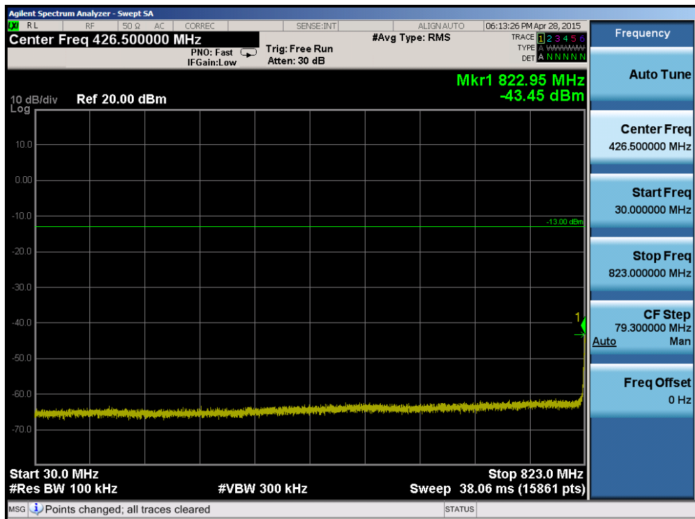
Plot 6-46. Conducted Spurious Plot (Band 5 – 1.4MHz QPSK – RB Size 1, RB Offset 0 – Low Channel)
