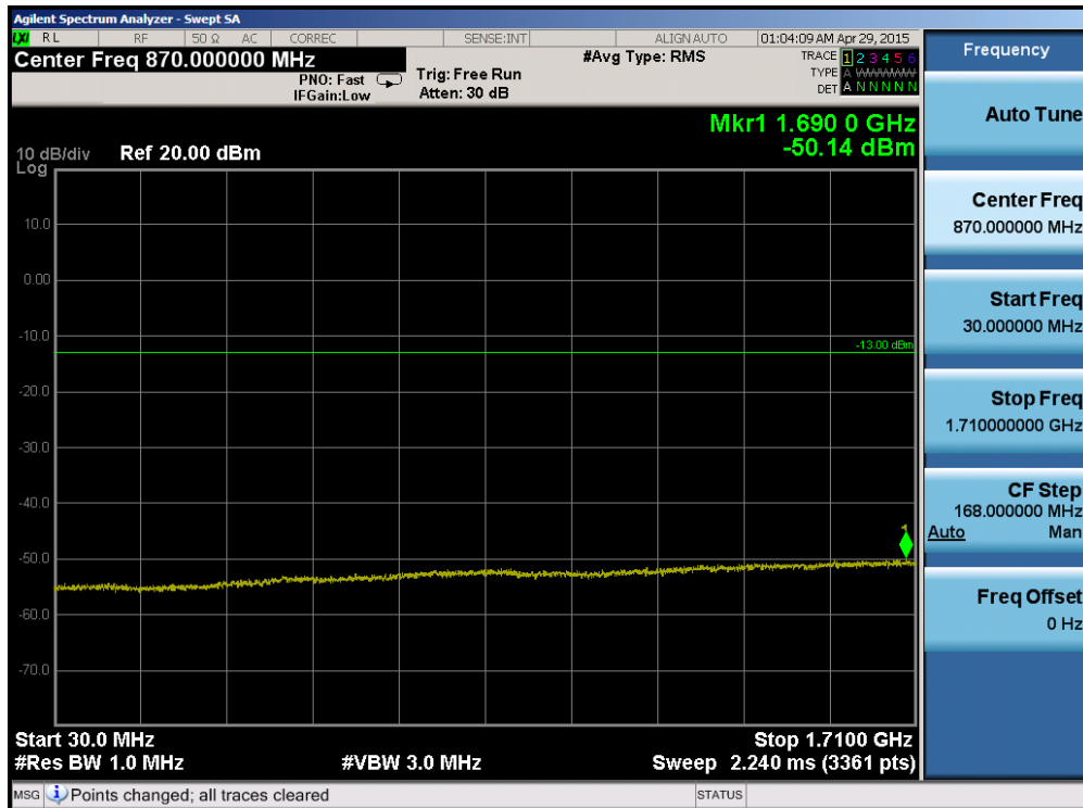
Plot 6-58. Conducted Spurious Plot (Band 4 – 5.0MHz QPSK – RB Size 1, RB Offset 0 – Mid Channel)
