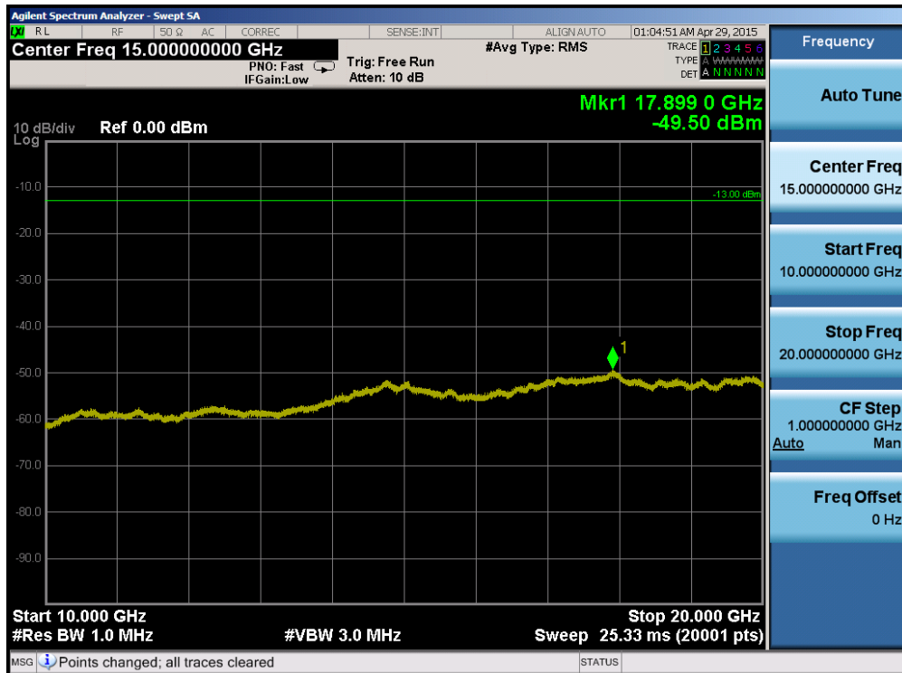
Plot 6-60. Conducted Spurious Plot (Band 4 – 5.0MHz QPSK – RB Size 1, RB Offset 0 – Mid Channel)
