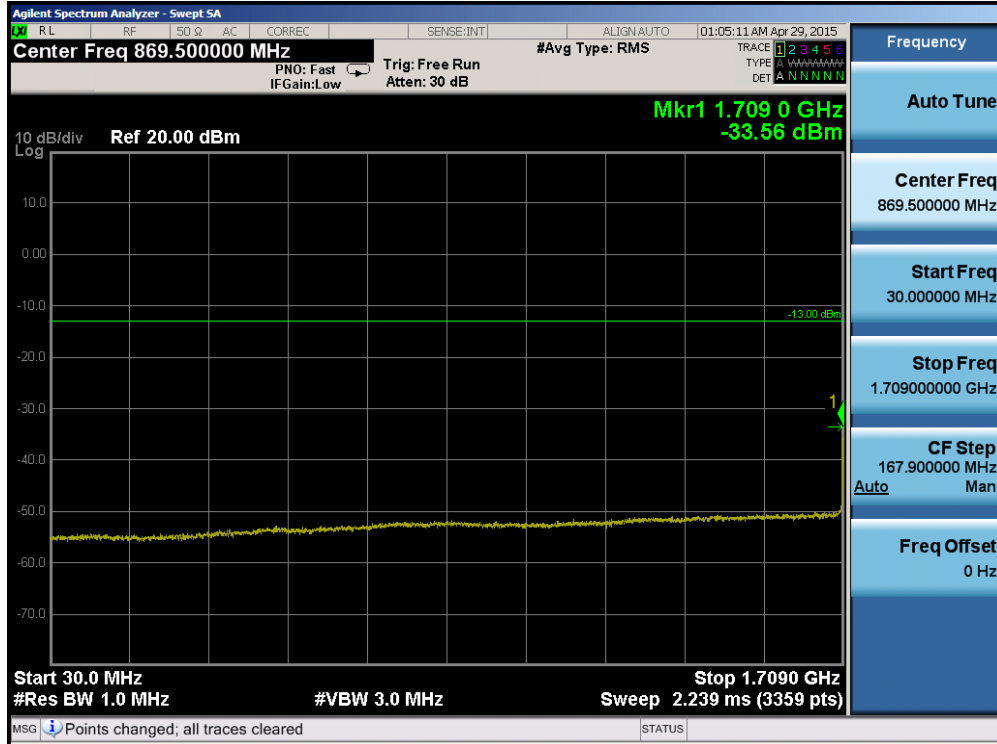
Plot 6-55. Conducted Spurious Plot (Band 4 – 5.0MHz QPSK – RB Size 1, RB Offset 0 – Low Channel)
