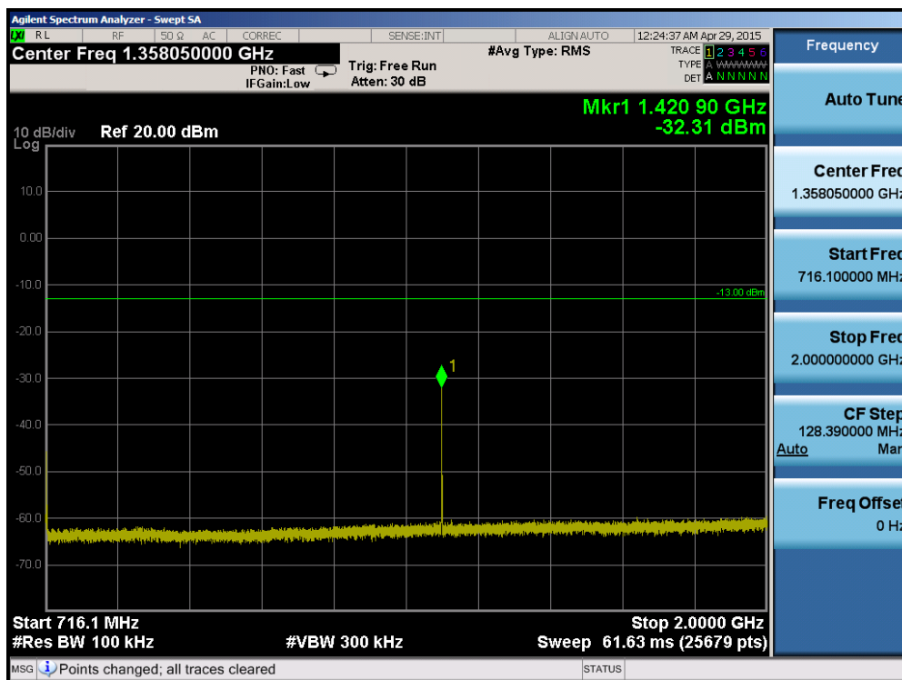
Plot 6-44. Conducted Spurious Plot (Band 17 – 5.0MHz QPSK – RB Size 1, RB Offset 0 – High Channel)
