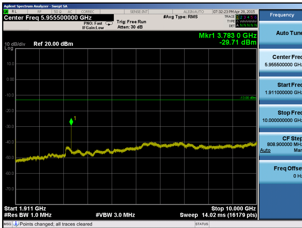
Plot 6-71. Conducted Spurious Plot (Band 2 – 20.0MHz QPSK – RB Size 1, RB Offset 0 – High Channel)
