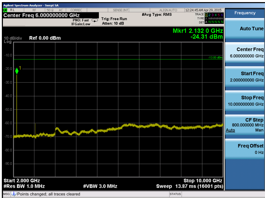
Plot 6-45. Conducted Spurious Plot (Band 17 – 5.0MHz QPSK – RB Size 1, RB Offset 0 – High Channel)
