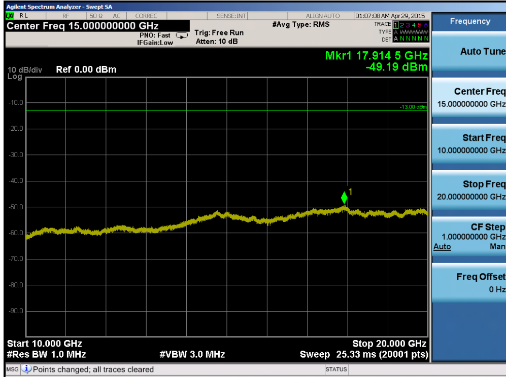
Plot 6-63. Conducted Spurious Plot (Band 4 – 5.0MHz QPSK – RB Size 1, RB Offset 0 – High Channel)
