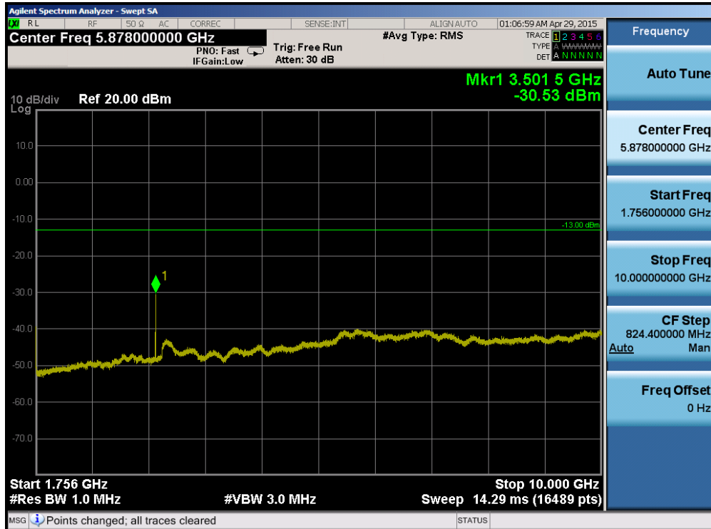
Plot 6-62. Conducted Spurious Plot (Band 4 – 5.0MHz QPSK – RB Size 1, RB Offset 0 – High Channel)
