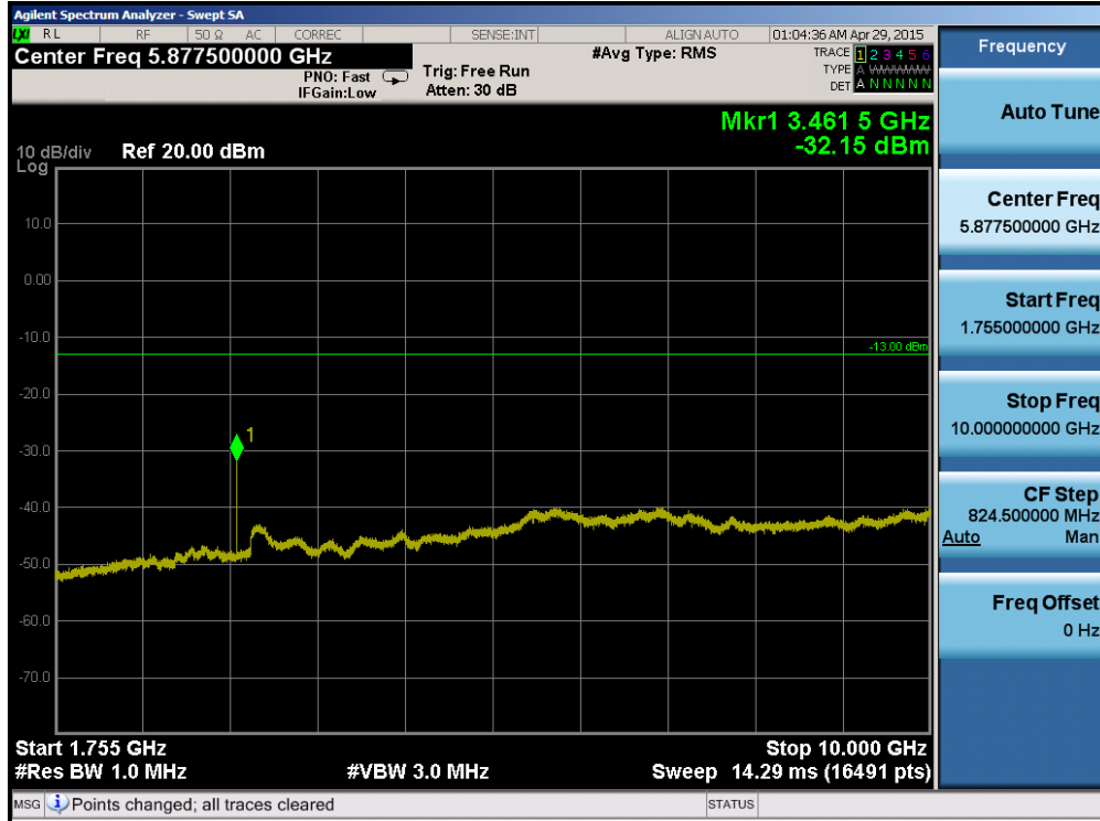
Plot 6-59. Conducted Spurious Plot (Band 4 – 5.0MHz QPSK – RB Size 1, RB Offset 0 – Mid Channel)
