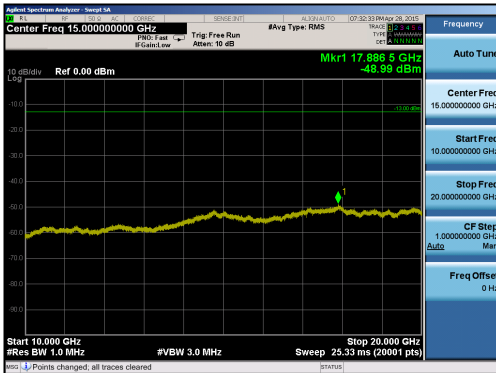
Plot 6-72. Conducted Spurious Plot (Band 2 – 20.0MHz QPSK – RB Size 1, RB Offset 0 – High Channel)
