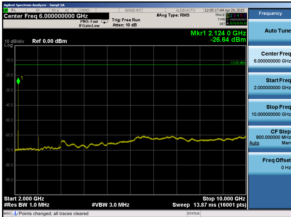
Plot 6-42. Conducted Spurious Plot (Band 17 – 5.0MHz QPSK – RB Size 1, RB Offset 0 – Mid Channel)
