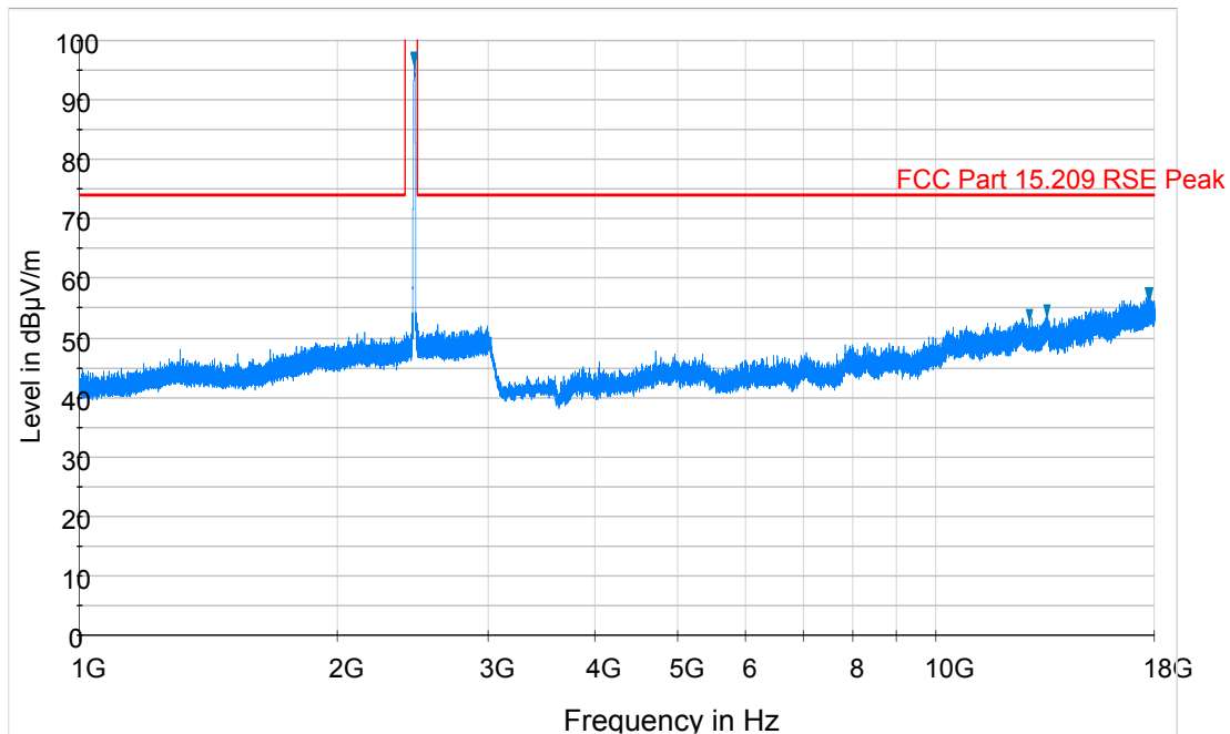
Plot 6-36. Radiated Spurious Plot above 1GHz (802.11b – Ch. 11, Ant. Pol. V)
