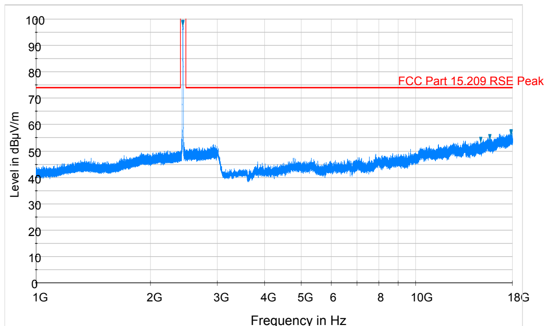
Plot 6-33. Radiated Spurious Plot above 1GHz (802.11b – Ch. 6, Ant. Pol. H)
