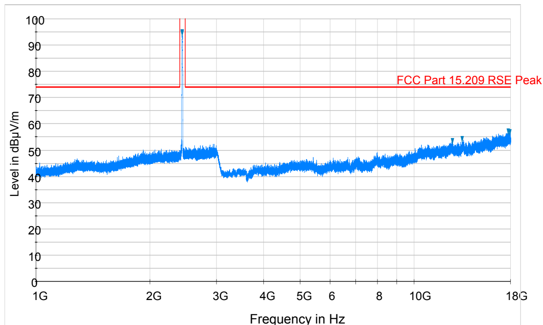
Plot 6-34. Radiated Spurious Plot above 1GHz (802.11b – Ch. 6, Ant. Pol. V)
