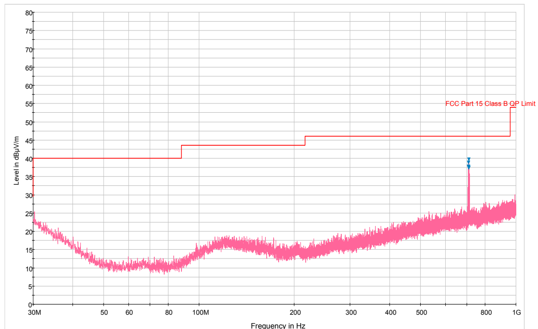
Plot 6-46. Radiated Spurious Plot below 1GHz (Pol. V)
