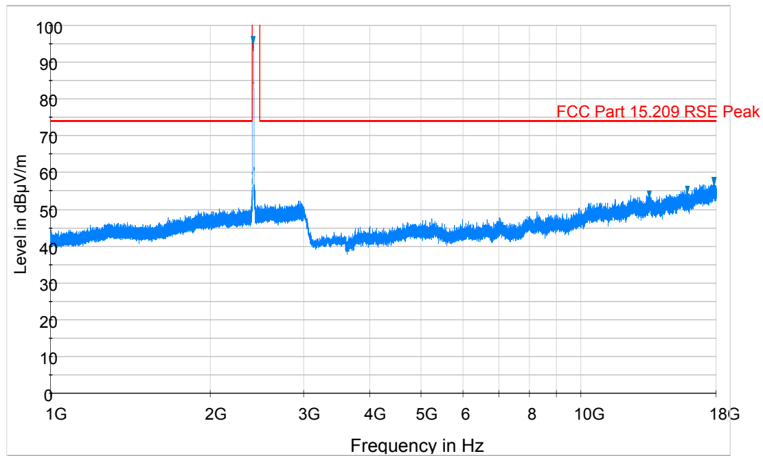
Plot 6-31. Radiated Spurious Plot above 1GHz (802.11b – Ch. 1, Ant. Pol. H)
