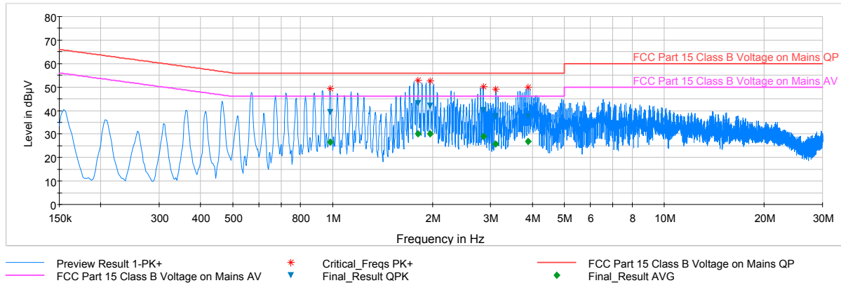
Plot 6-47. Line Conducted Plot with 802.11b (L1)
