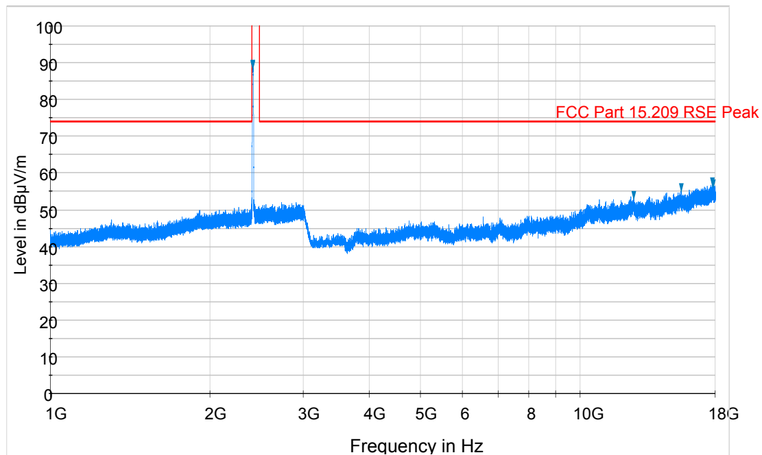
Plot 6-32. Radiated Spurious Plot above 1GHz (802.11b – Ch. 1, Ant. Pol. V)
