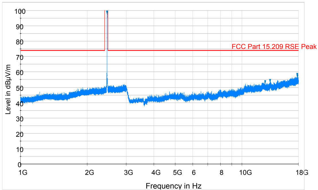
Plot 6-35. Radiated Spurious Plot above 1GHz (802.11b – Ch. 11, Ant. Pol. H)
