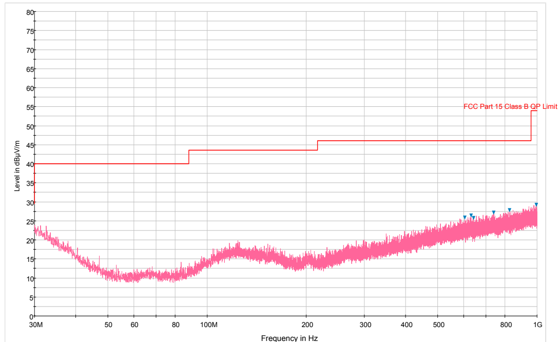
Plot 6-45. Radiated Spurious Plot below 1GHz (Pol. H)
