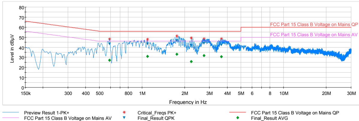
Plot 6-48. Line Conducted Plot with 802.11b (N)
