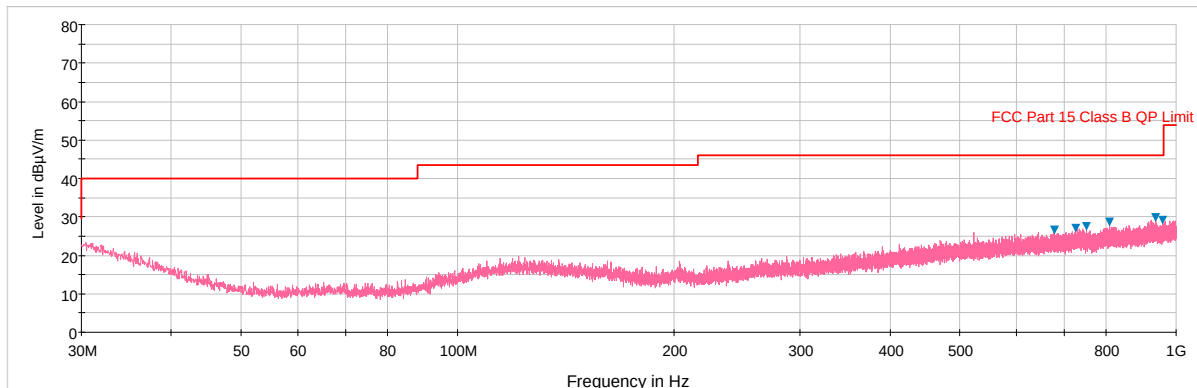
Plot 6-95. Radiated Spurious Plot below 1GHz (802.11a – U3 Ch. 157, Ant. Pol. H)
