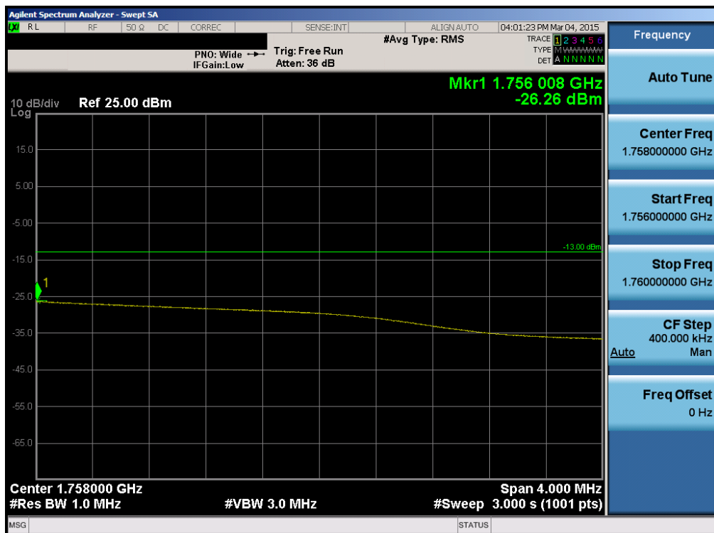
Plot 6-91. Upper Extended Band Edge Plot (Band 4 – 20.0MHz QPSK – RB Size 100)
