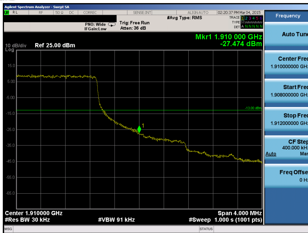
Plot 6-98. Upper Band Edge Plot (Band 2 - 3.0MHz QPSK - RB Size 15)
