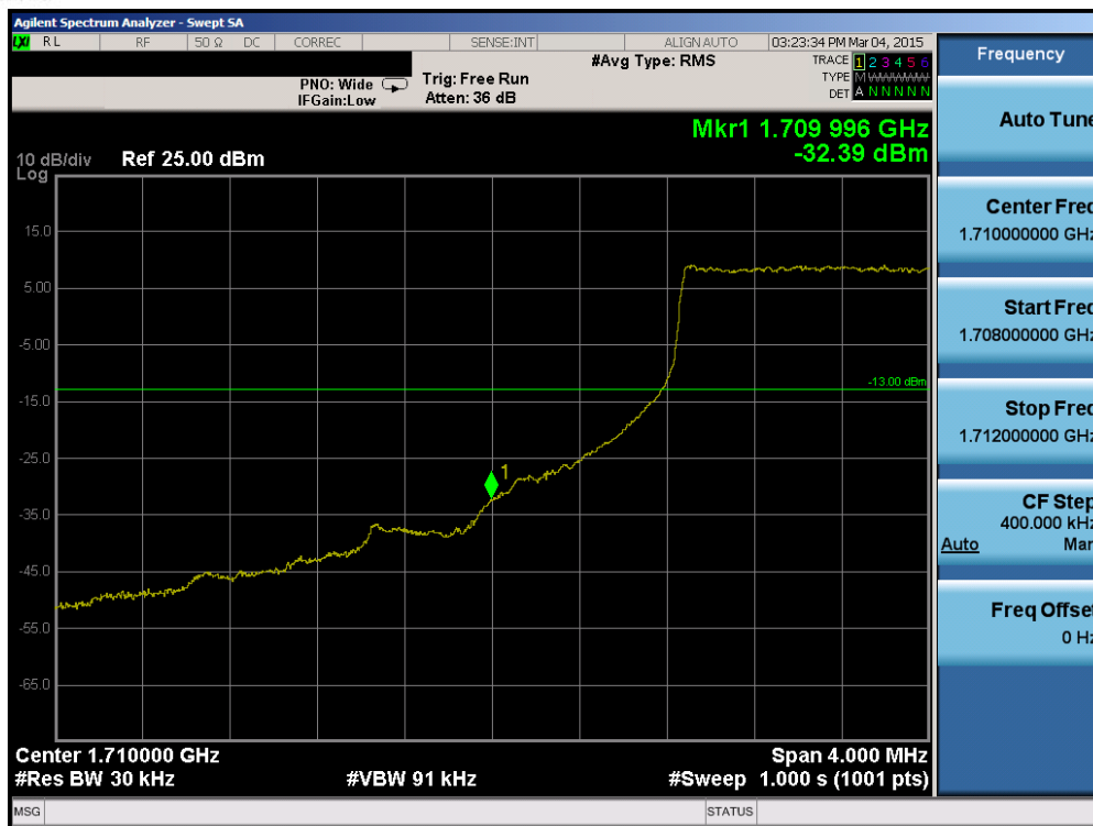
Plot 6-72. Lower Band Edge Plot (Band 4 – 3.0MHz QPSK – RB Size 15)
