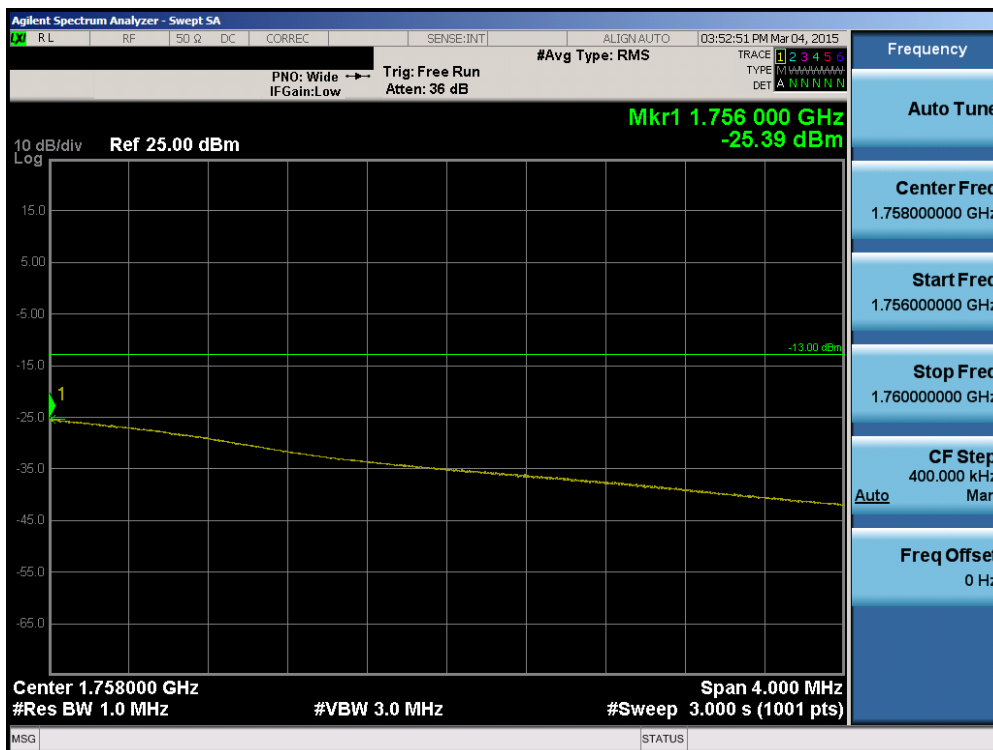
Plot 6-83. Upper Extended Band Edge Plot (Band 4 – 10.0MHz QPSK – RB Size 50)
