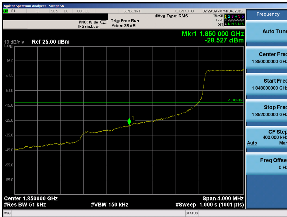
Plot 6-100. Lower Band Edge Plot (Band 2 – 5.0MHz QPSK – RB Size 25)
