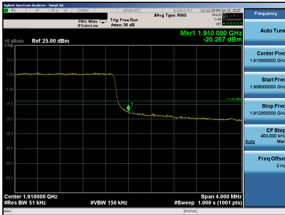
Plot 6-110. Upper Band Edge Plot (Band 2 – 5.0MHz QPSK – RB Size 25)
