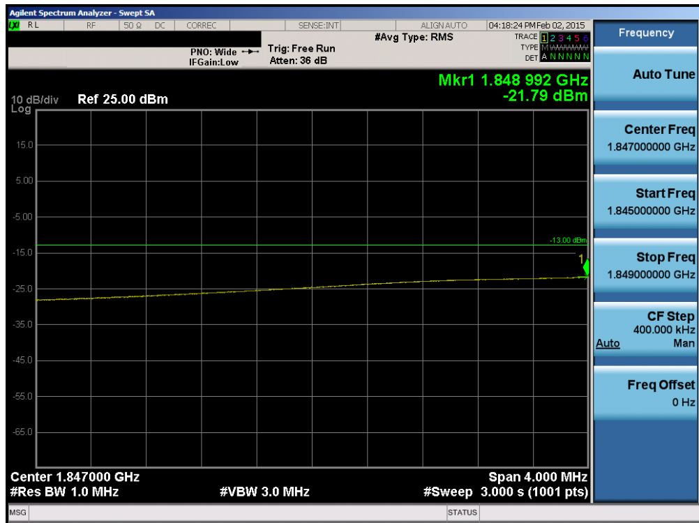
Plot 6-117. Lower Extended Band Edge Plot (Band 2 - 15.0MHz QPSK - RB Size 75)
