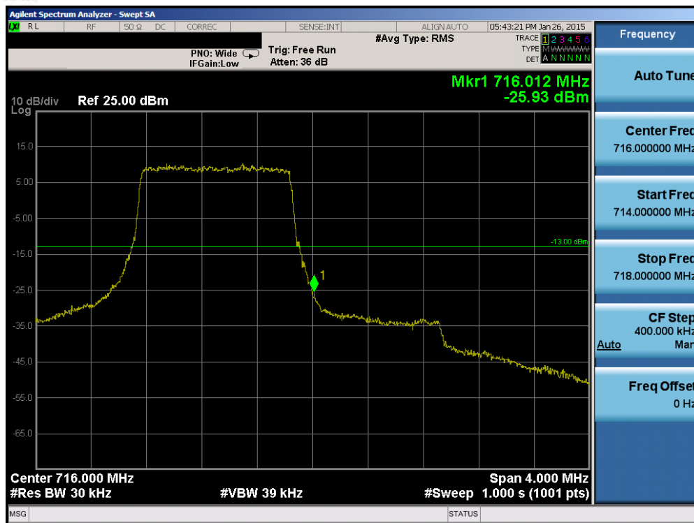
Plot 6-62. Upper Band Edge Plot (Band 12 – 1.4MHz QPSK – RB Size 6)
