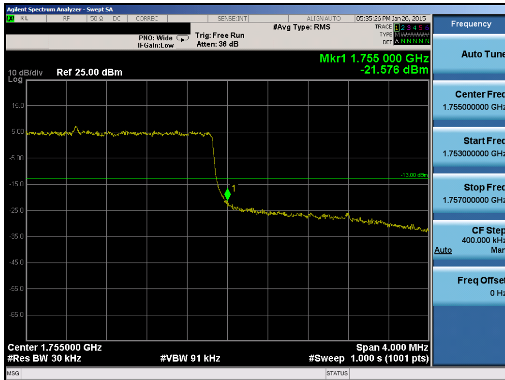
Plot 6-82. Upper Band Edge Plot (Band 4 – 3.0MHz QPSK – RB Size 15)
