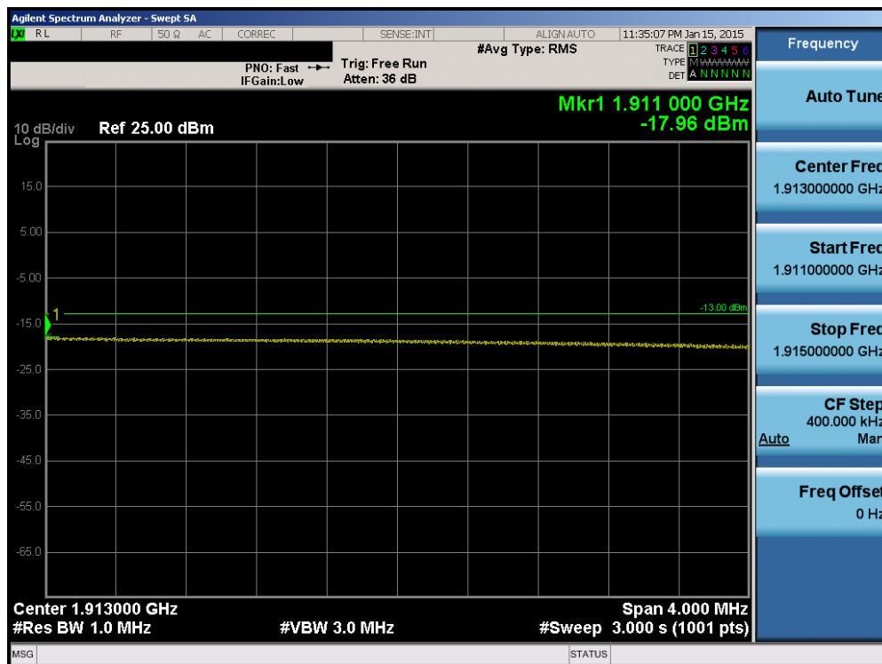
Plot 6-123. Upper Extended Band Edge Plot (Band 2 – 20.0MHz QPSK – RB Size 100)
