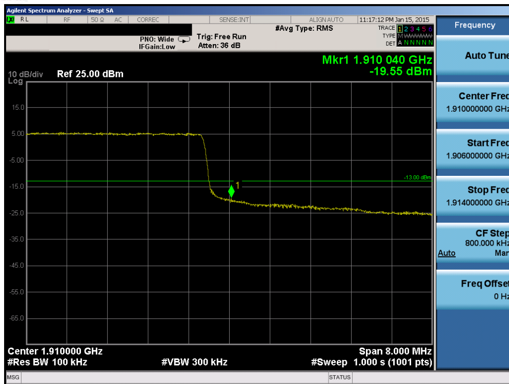
Plot 6-114. Upper Band Edge Plot (Band 2 – 10.0MHz QPSK – RB Size 50)
