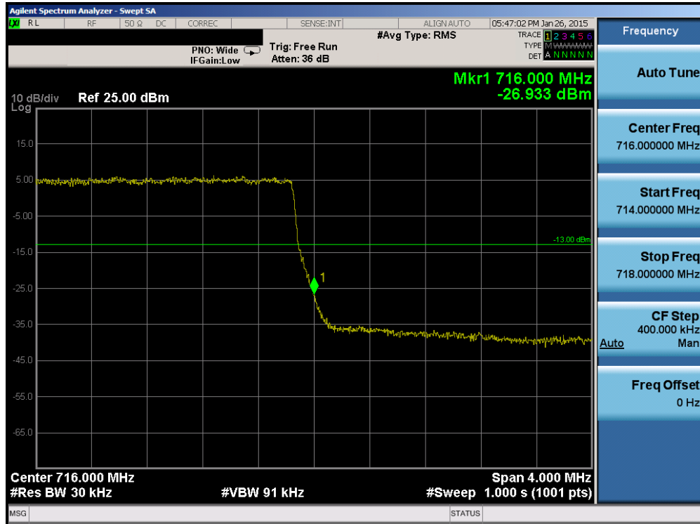
Plot 6-66. Upper Band Edge Plot (Band 12 – 3.0MHz QPSK – RB Size 15)
