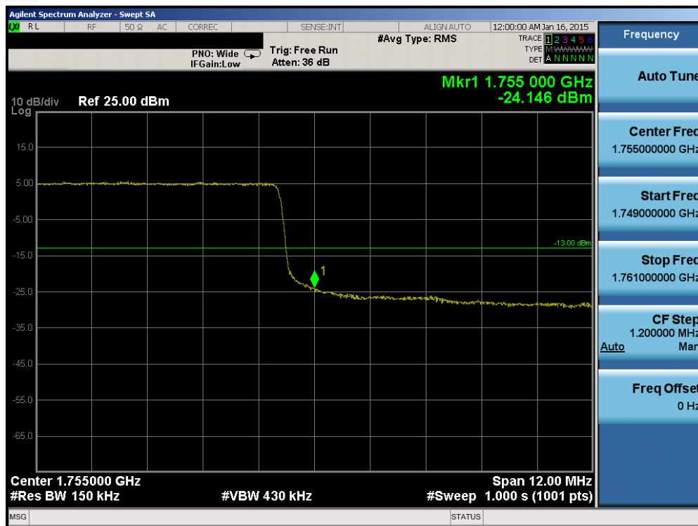
Plot 6-94. Upper Band Edge Plot (Band 4 – 15.0MHz QPSK – RB Size 75)
