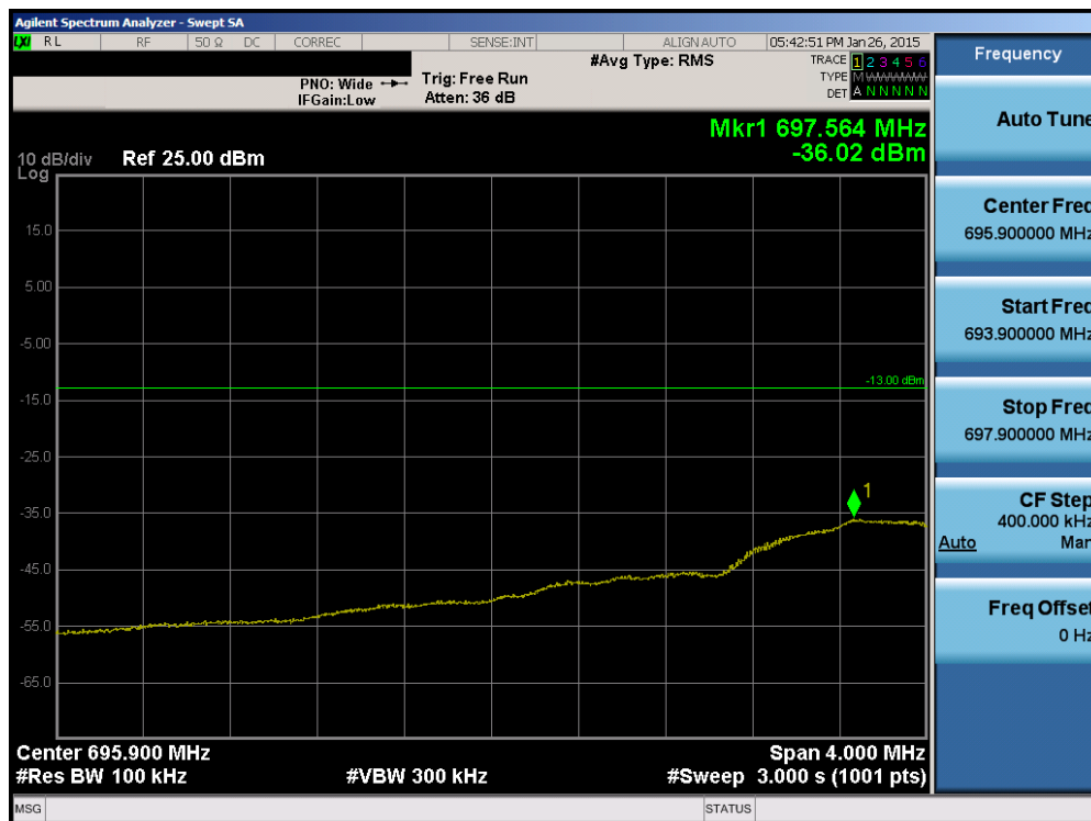
Plot 6-61. Lower Extended Band Edge Plot (Band 12 – 1.4MHz QPSK – RB Size 6)
