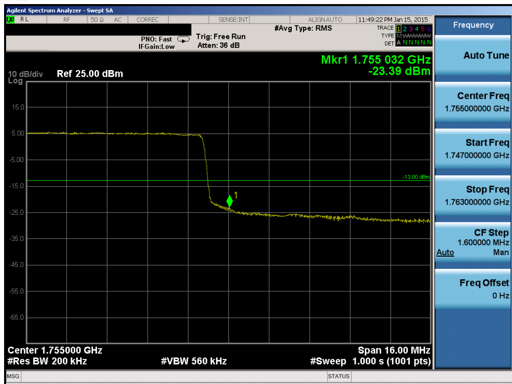
Plot 6-98. Upper Band Edge Plot (Band 4 – 20.0MHz QPSK – RB Size 100)
