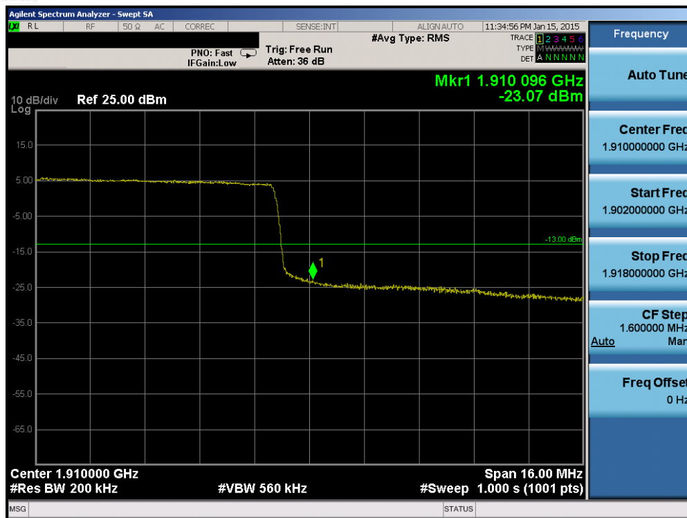
Plot 6-122. Upper Band Edge Plot (Band 2 – 20.0MHz QPSK – RB Size 100)
