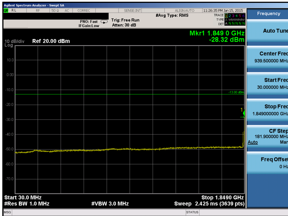
Plot 6-51. Conducted Spurious Plot (Band 2 – 20.0MHz QPSK – RB Size 1, RB Offset 0– Low Channel)
