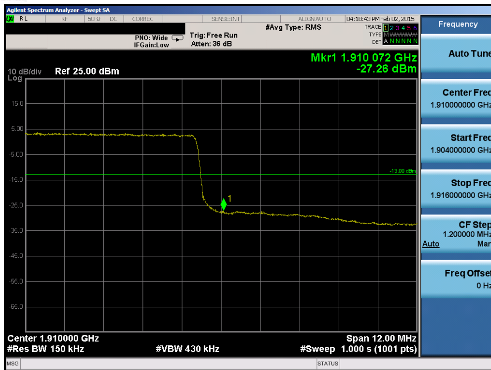
Plot 6-118. Upper Band Edge Plot (Band 2 – 15.0MHz QPSK – RB Size 75)
