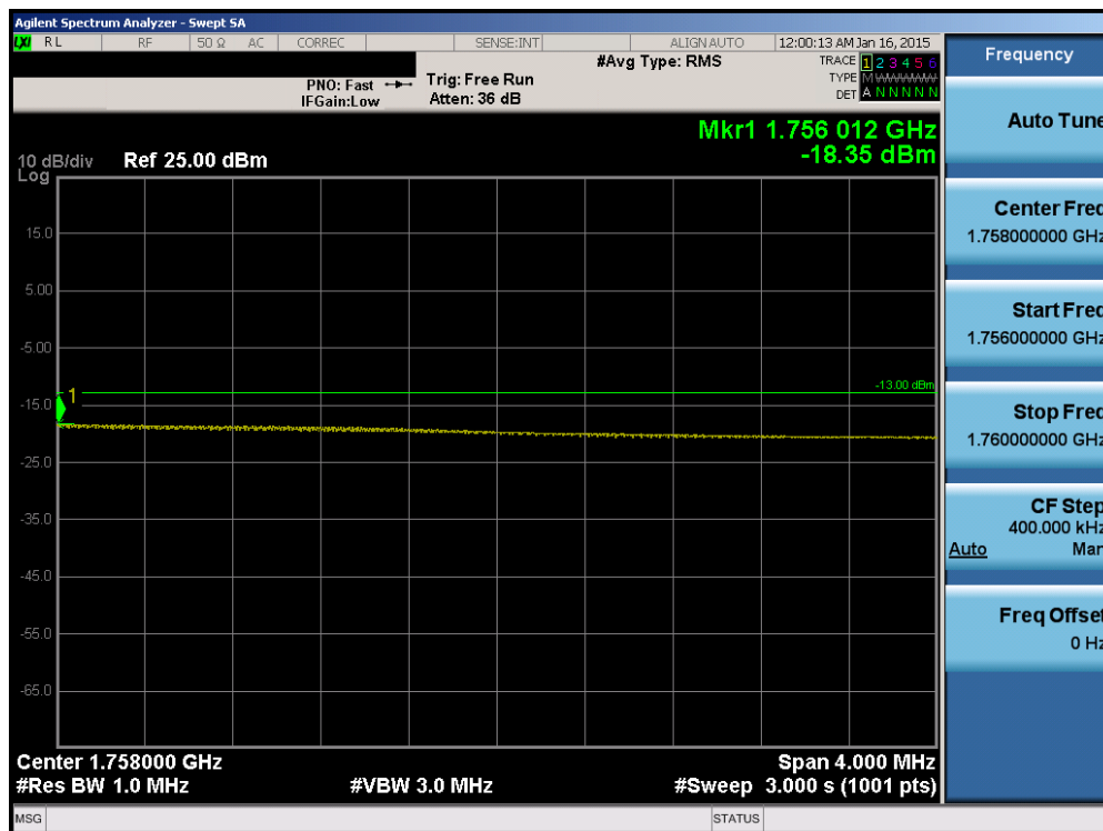
Plot 6-95. Upper Extended Band Edge Plot (Band 4 – 15.0MHz QPSK – RB Size 75)
