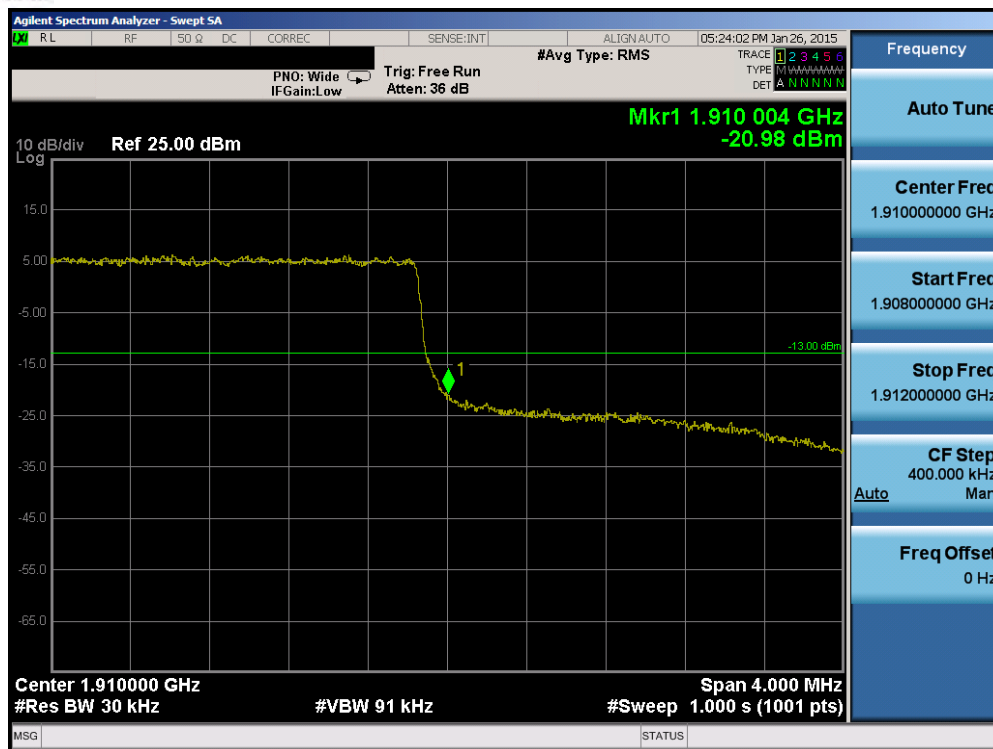
Plot 6-106. Upper Band Edge Plot (Band 2 – 3.0MHz QPSK – RB Size 15)
