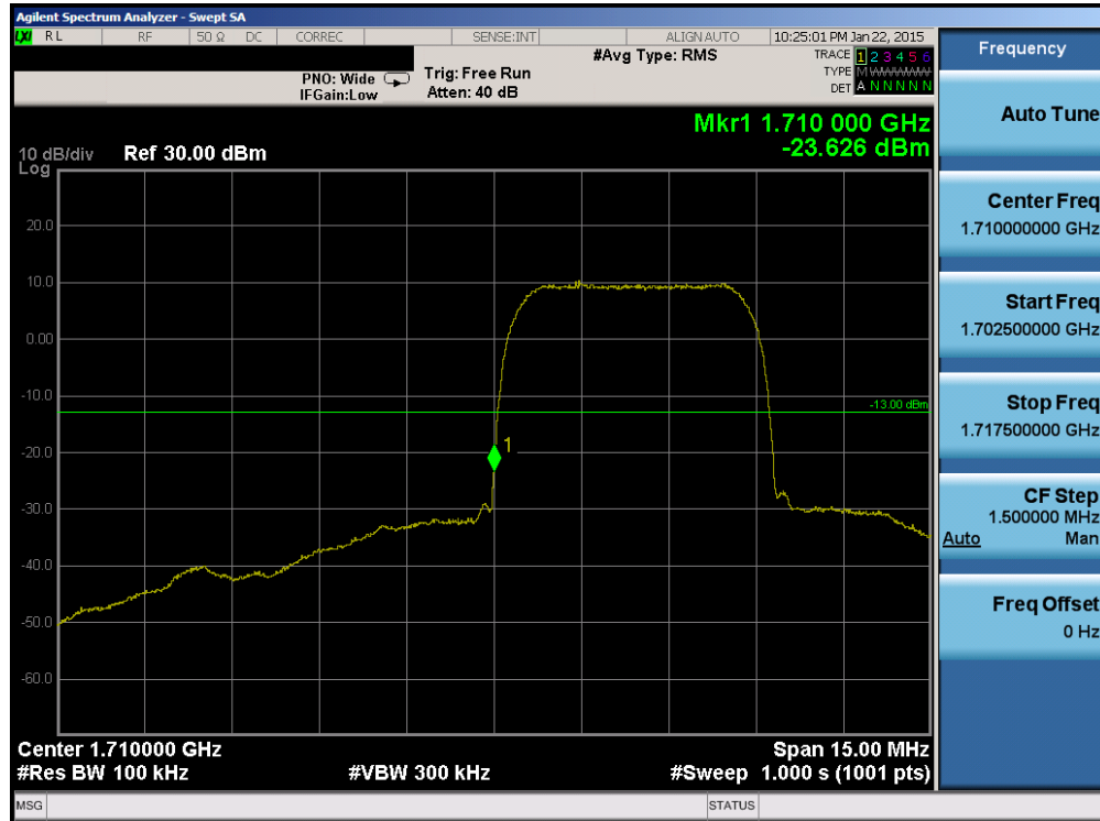
Plot 6-59. Band Edge Plot (AWS WCDMA Mode – Ch. 1312)
