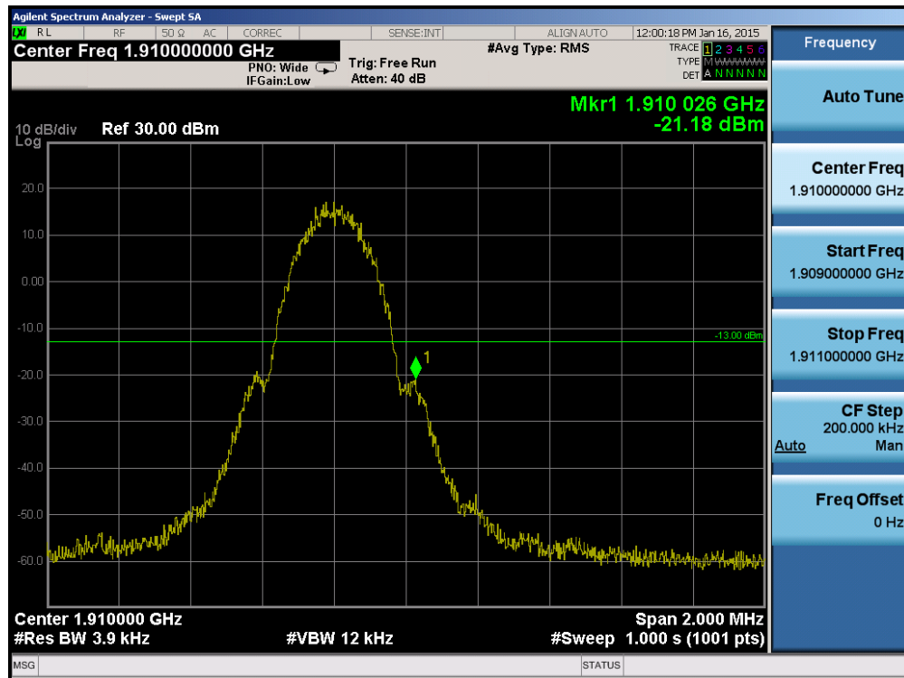
Plot 6-56. Band Edge Plot (PCS GSM Mode – Ch. 810)
