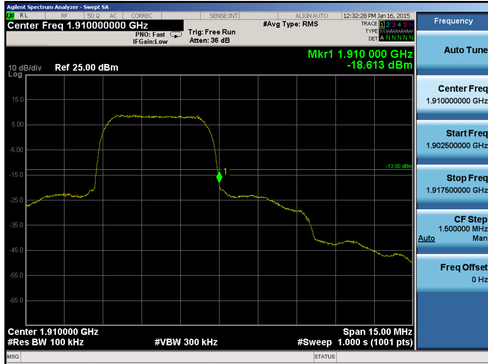
Plot 6-65. Band Edge Plot (PCS WCDMA Mode – Ch. 9538)
