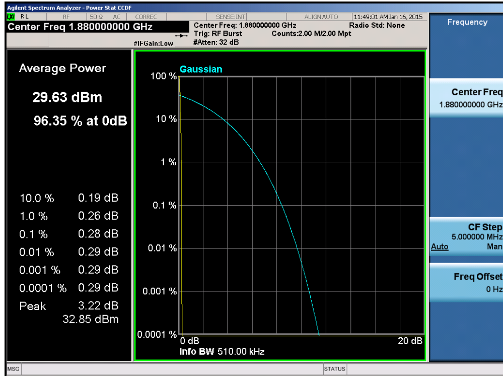
Plot 6-67. Peak-Average Ratio Plot (PCS GSM Mode – Ch. 661)
