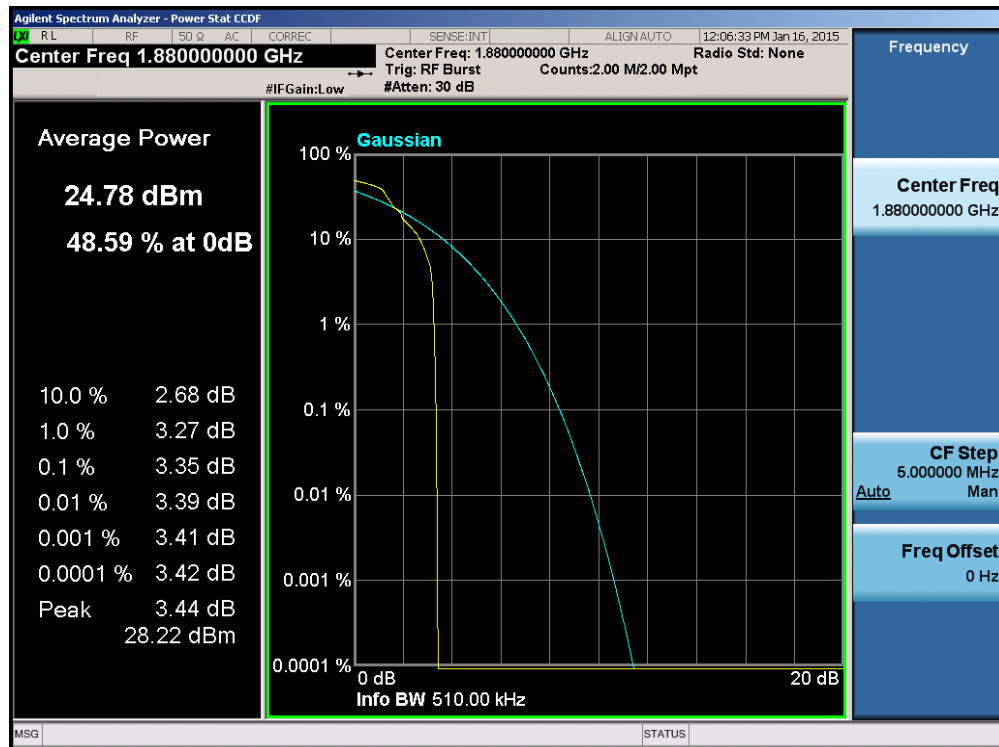
Plot 6-68. Peak-Average Ratio Plot (EDGE1900 Mode – Ch. 661)
