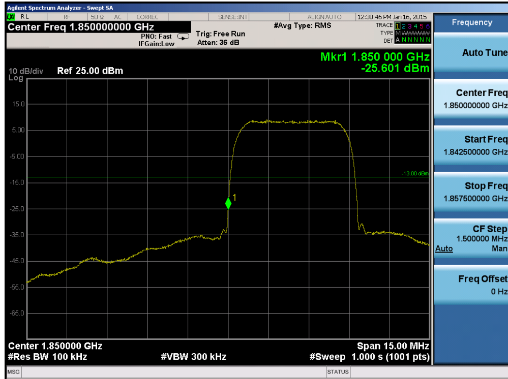
Plot 6-63. Band Edge Plot (PCS WCDMA Mode – Ch. 9262)
