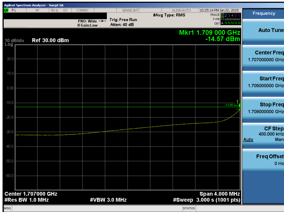
Plot 6-60. 4MHz Span Plot (AWS WCDMA Mode – Ch. 1312)
