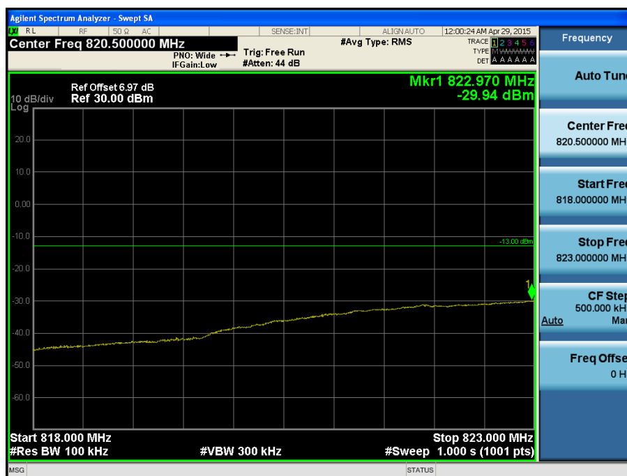
LTE Band 5 / 5MHz / 16QAM Offset/Size (25/0)
