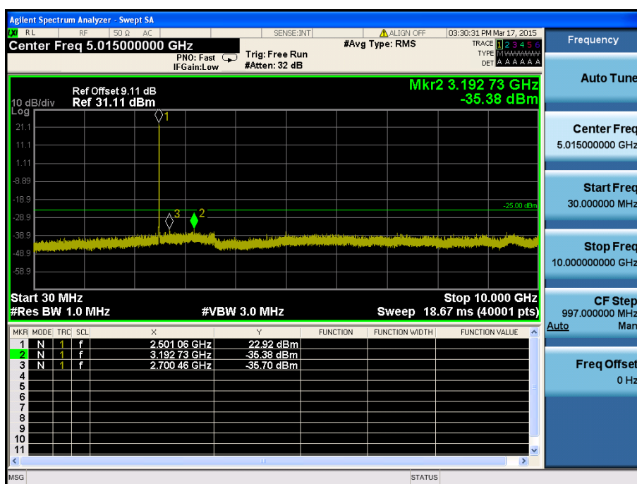
LTE Band 7 / 5MHz / QPSK - RB Size/Offset (25/0) – Low Channel
