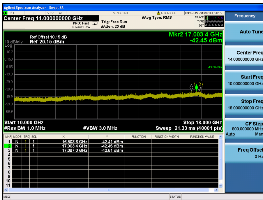
LTE Band 4 / 1.4MHz / 16QAM - RB Size/Offset (1/0) – High Channel
