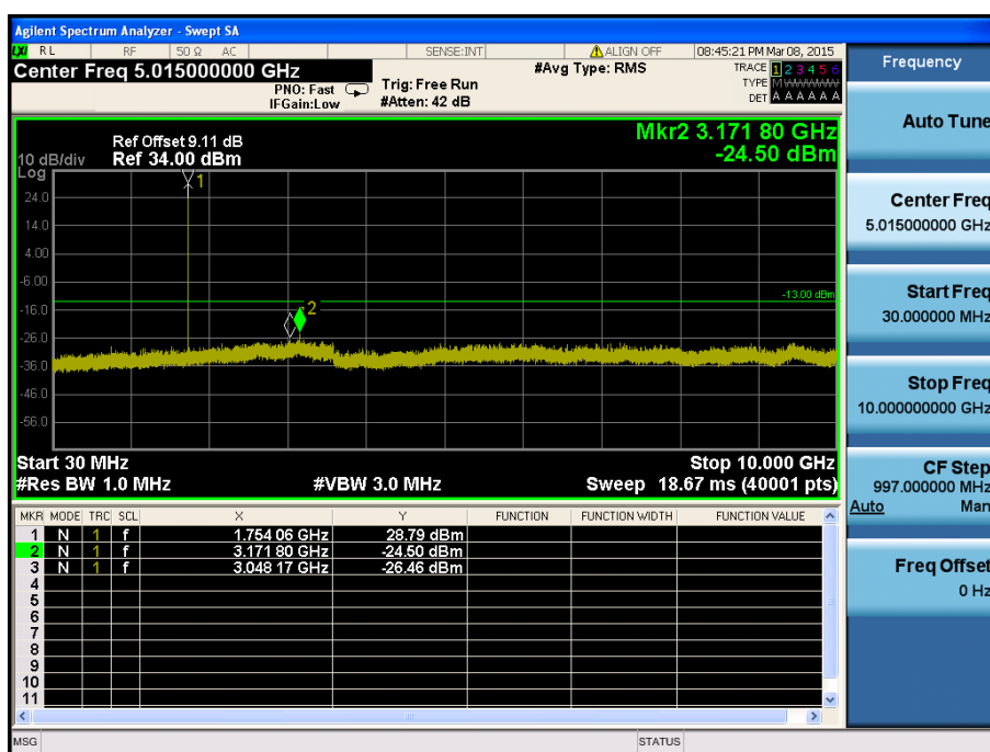
LTE Band 4 / 3MHz / QPSK - RB Size/Offset (1/7) – High Channel
