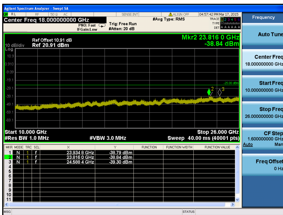
LTE Band 7 / 20MHz / QPSK - RB Size/Offset (100/0) – Low Channel
