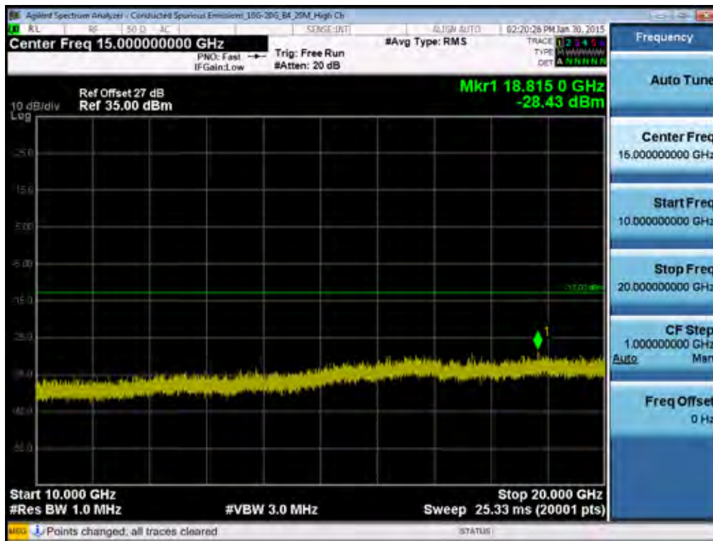
BAND 4. Conducted Spurious Plot_2 (20300ch_20MHz_QPSK_RB 1_0)
