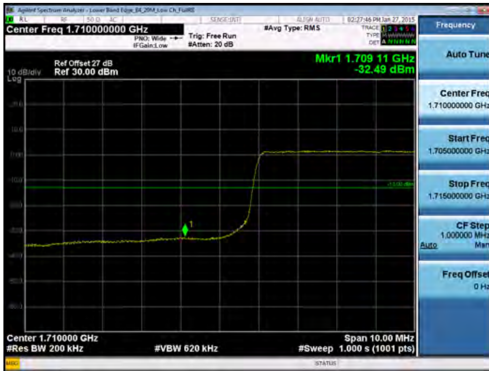
BAND 4. Lower Band Edge Plot (20M BW Ch.20050 QPSK RB 100) -2
