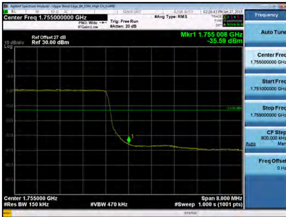
BAND 4. Upper Band Edge Plot (15M BW Ch.20325 QPSK_RB75) -2
