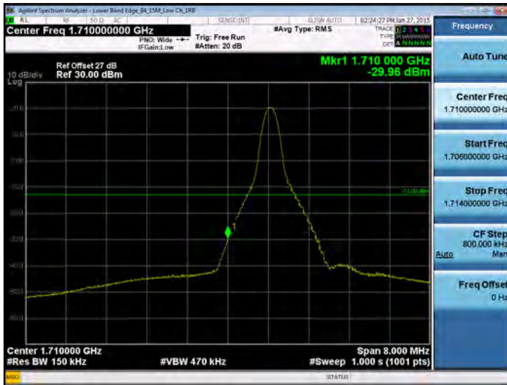
BAND 4. L Lower Band Edge Plot (15M BW Ch.20025 QPSK RB 1, Offset 0) -1
