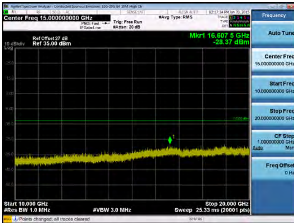
BAND 4. Conducted Spurious Plot_2 (20350ch_10MHz_QPSK_RB 1_0)
