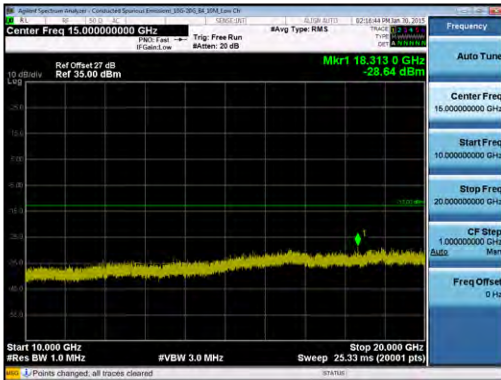
BAND 4. Conducted Spurious Plot_2 (20000ch_10MHz_QPSK_ RB 1_0)
