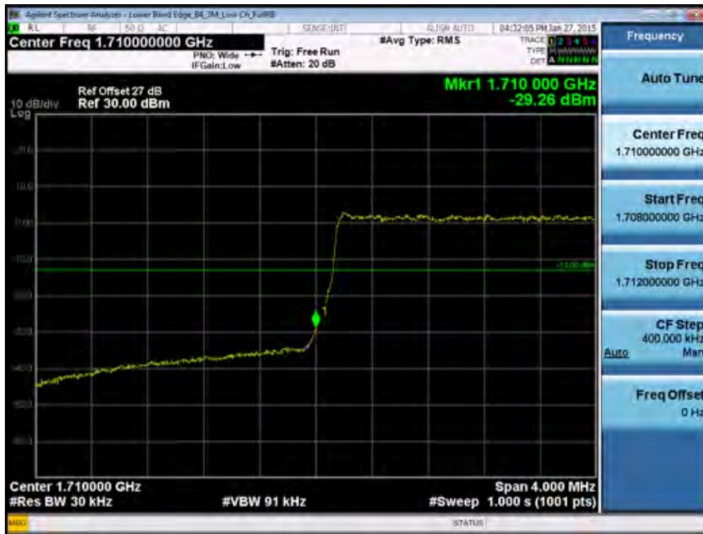
BAND 4. Lower Band Edge Plot (3M BW Ch.19965 QPSK RB 15) -2
