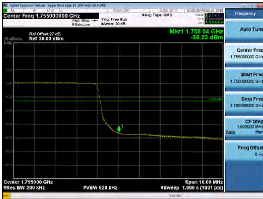
BAND 4. Upper Band Edge Plot (20M BW Ch.20300 QPSK_RB100) -2
