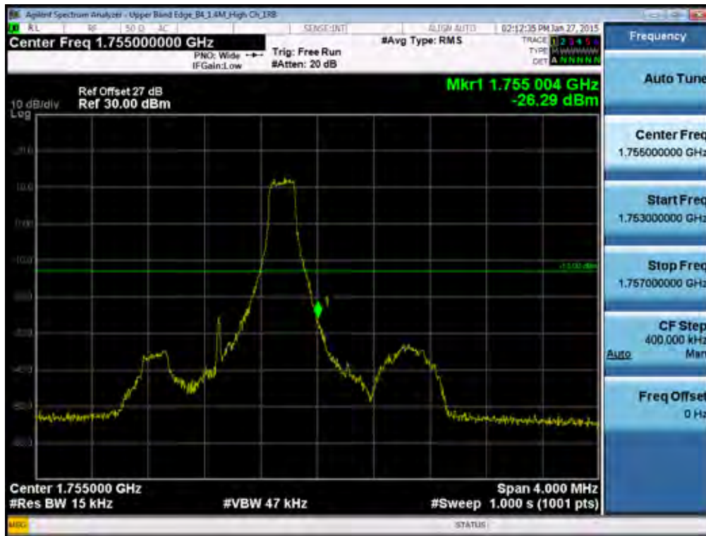
BAND 4. Upper Band Edge Plot (1.4M BW Ch.20393 QPSK_RB1_Offset) -1
