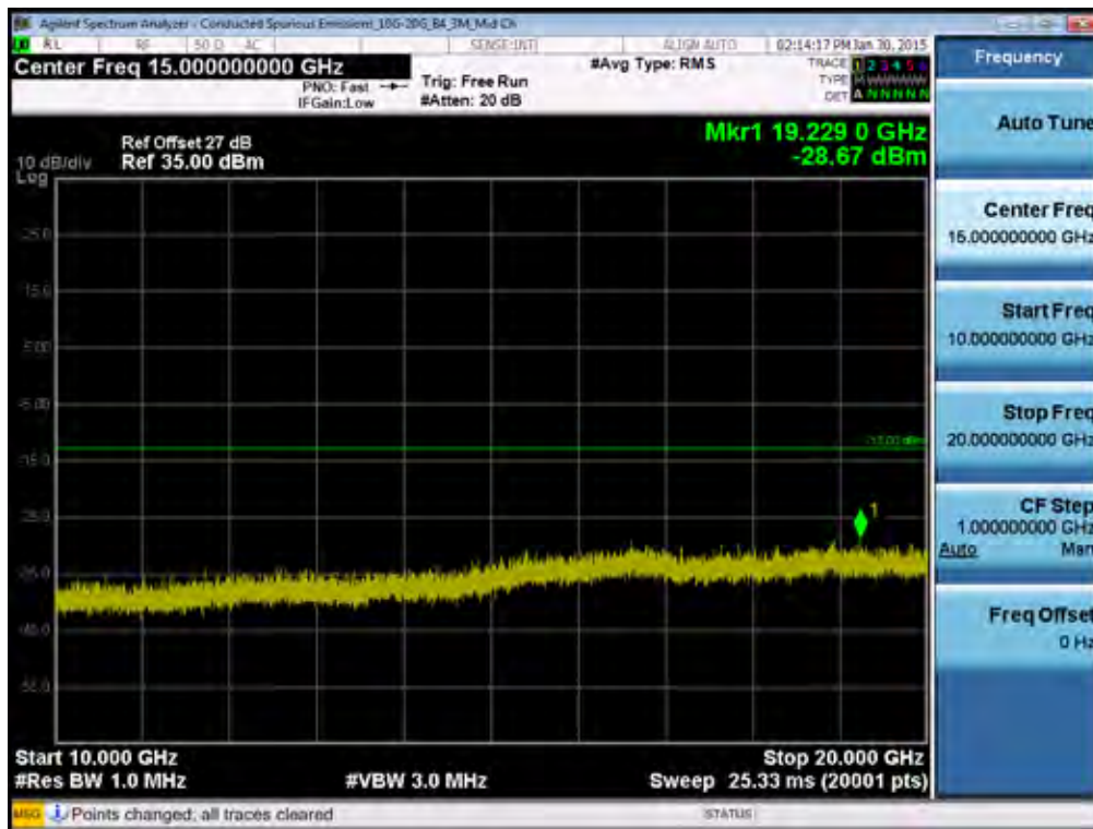
BAND 4. Conducted Spurious Plot_2 (20175ch_3MHz_QPSK_RB 1_0)
