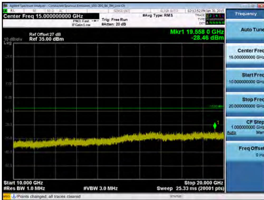
BAND 4. Conducted Spurious Plot_2 (19965ch_3MHz_QPSK_RB 1_0)
