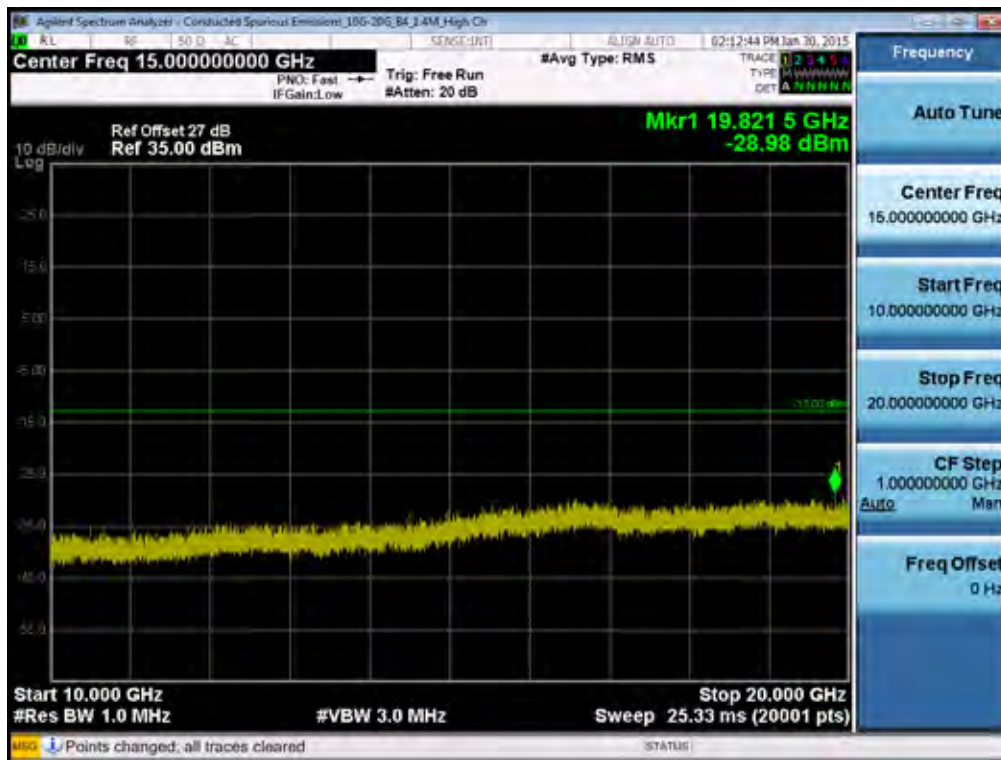
BAND 4 . Conducted Spurious Plot_2 (20393ch_1.4MHz_QPSK_RB 1_0)
