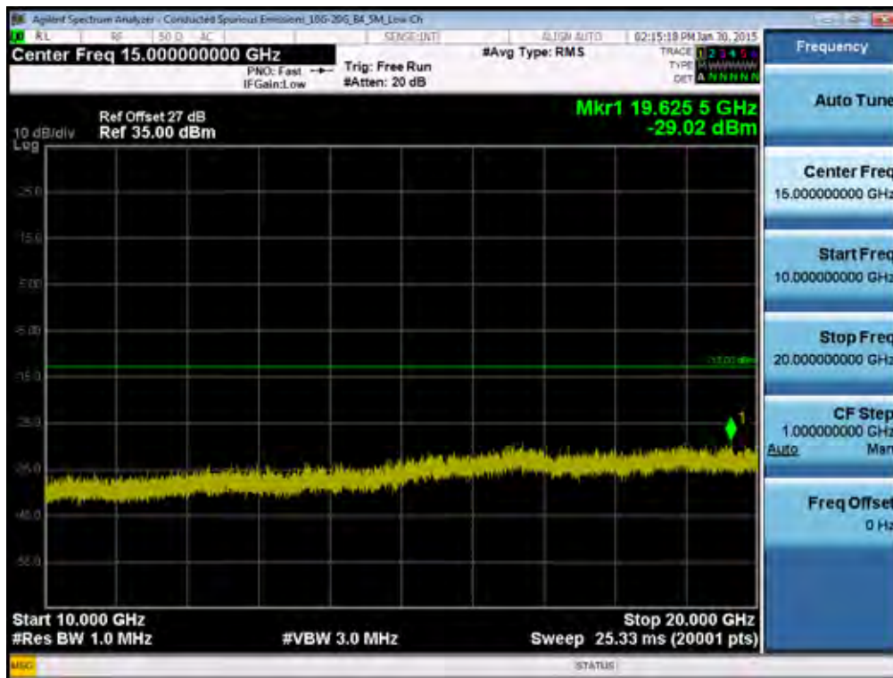
BAND 4. Conducted Spurious Plot_2 (19975ch_5MHz_QPSK_RB 1_0)
