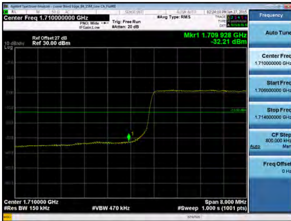
BAND 4. Lower Band Edge Plot (15M BW Ch.20025 QPSK RB 75) -2
