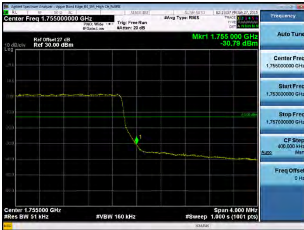
BAND 4. Upper Band Edge Plot (5M BW Ch.20375 QPSK_RB25) -2
