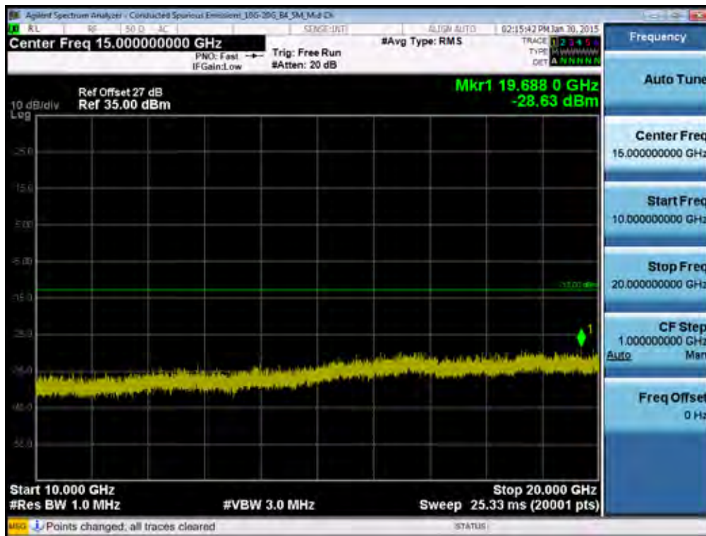
BAND 4. Conducted Spurious Plot_2 (20175ch_5MHz_QPSK_RB 1_0)
