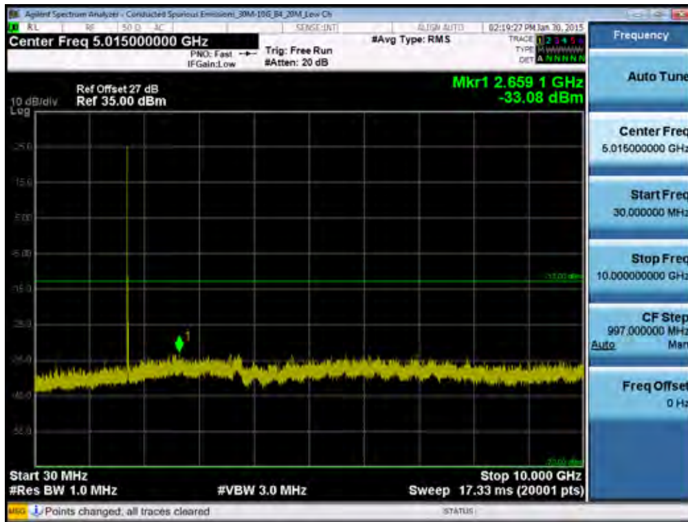
BAND 4. Conducted Spurious Plot_1 (20050ch_20MHz_QPSK_RB 1_0)
