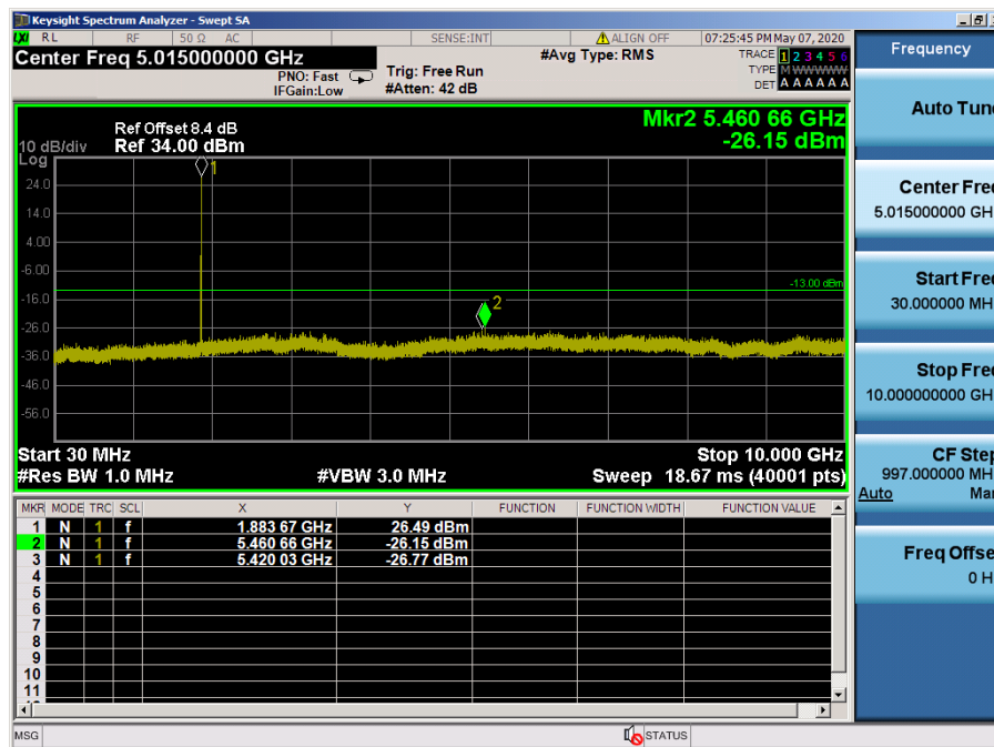
LTE Band 25, 2 / 3MHz / QPSK - RB Size/Offset (8/7) – Mid Channel
