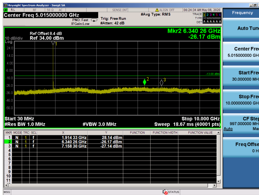
LTE Band 25, 2 / 3MHz / 64QAM - RB Size/Offset (8/7) – High Channel
