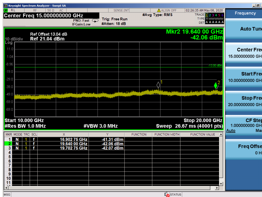
LTE Band 25, 2 / 10MHz / 16QAM - RB Size/Offset (50/0) – Low Channel
