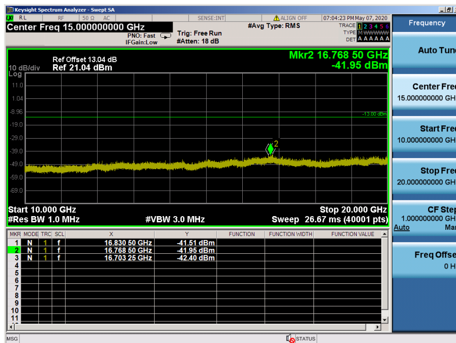
LTE Band 25, 2 / 3MHz / QPSK - RB Size/Offset (1/7) – Low Channel
