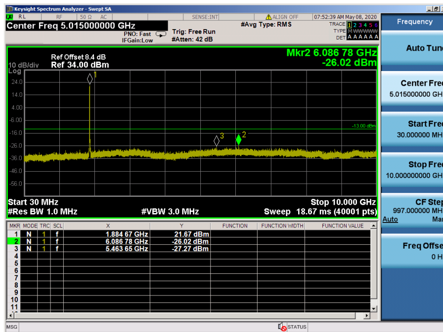
LTE Band 25, 2 / 10MHz / 64QAM - RB Size/Offset (50/0) – Mid Channel
