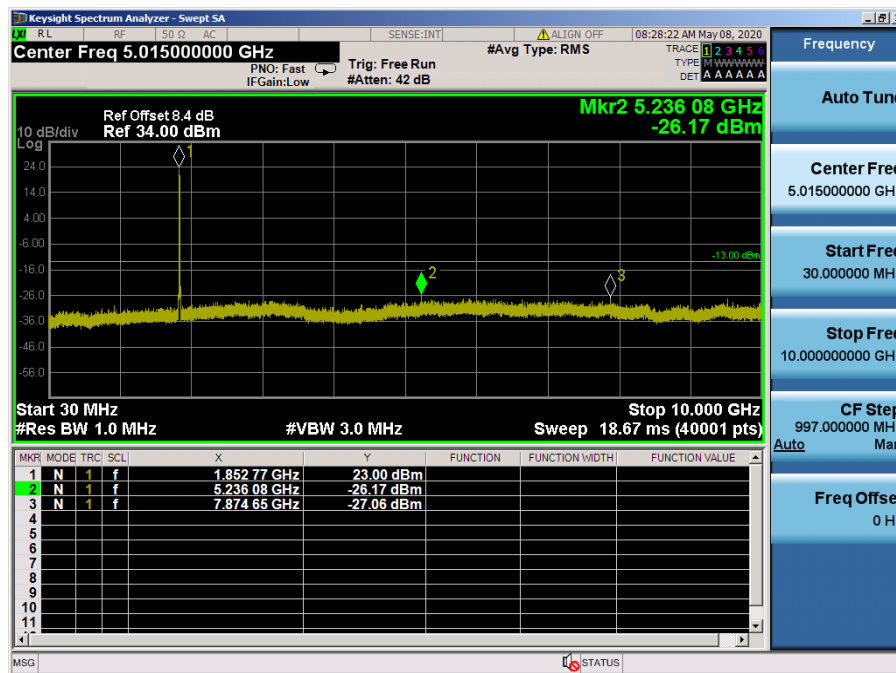
LTE Band 25, 2 / 15MHz / 64QAM - RB Size/Offset (36/0) – Low Channel
