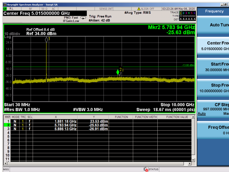
LTE Band 25, 2 / 15MHz / 16QAM - RB Size/Offset (36/18) – Mid Channel
