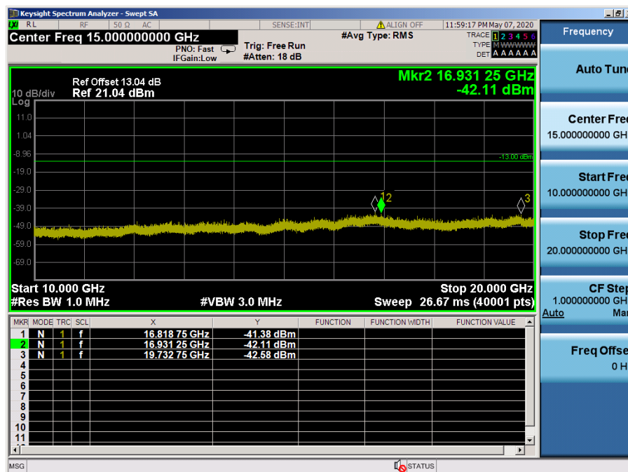
LTE Band 25, 2 / 1.4MHz / 16QAM - RB Size/Offset (1/2) – High Channel
