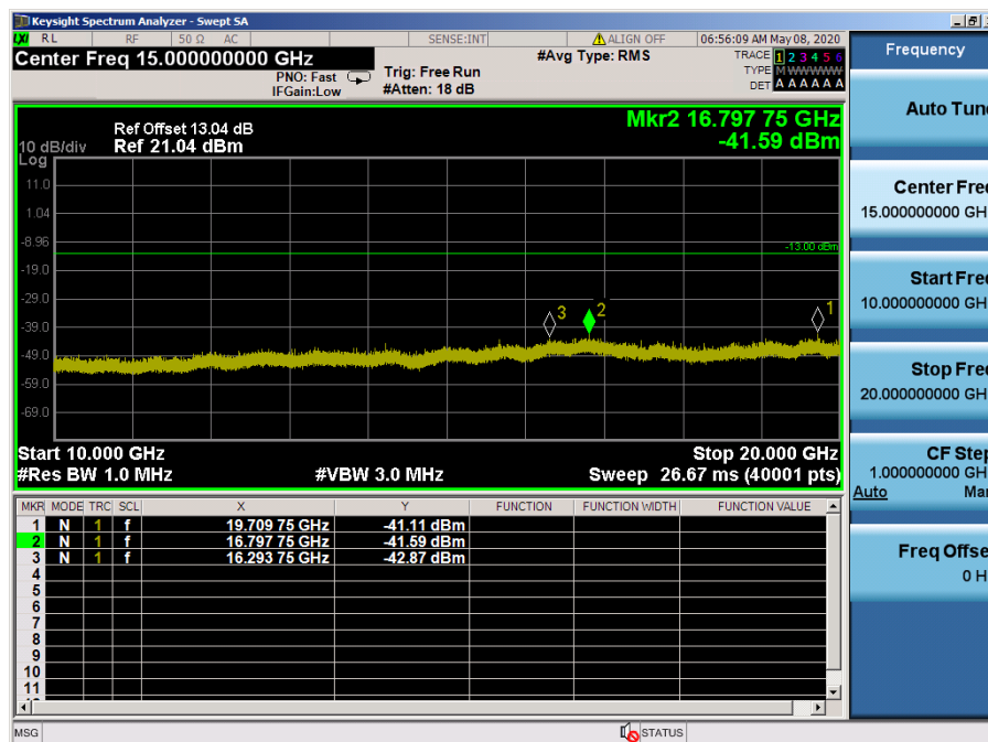
LTE Band 25, 2 / 5MHz / 64QAM - RB Size/Offset (12/0) – Mid Channel
