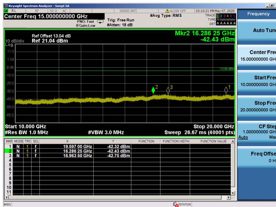
LTE Band 25, 2 / 15MHz / QPSK - RB Size/Offset (1/0) – High Channel
