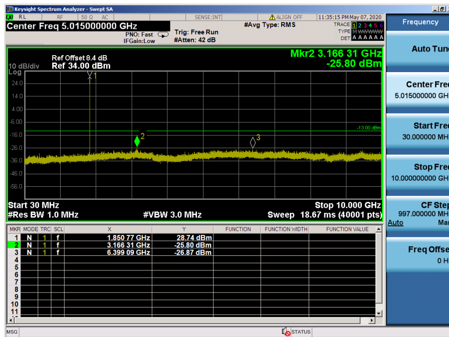
LTE Band 25, 2 / 1.4MHz / 16QAM - RB Size/Offset (3/0) – Low Channel
