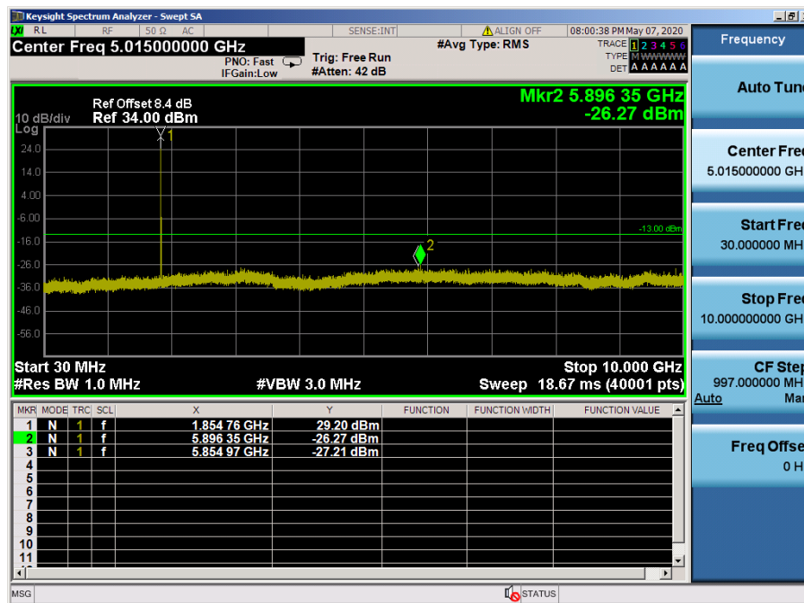
LTE Band 25, 2 / 5MHz / QPSK - RB Size/Offset (1/24) – Low Channel
