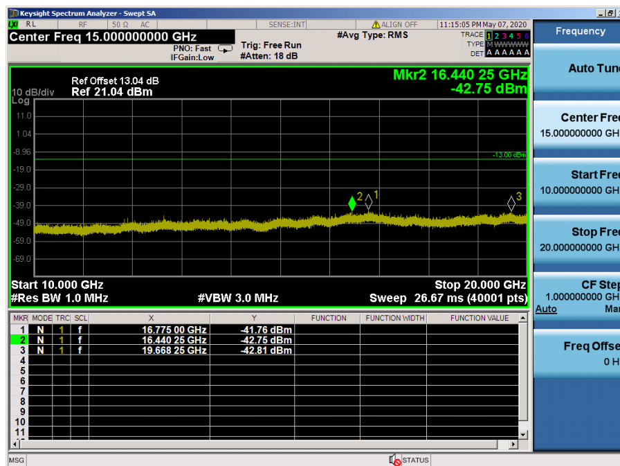
LTE Band 25, 2 / 20MHz / QPSK - RB Size/Offset (50/25) – High Channel
