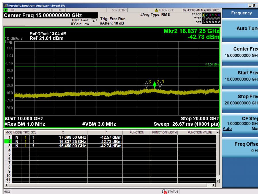
LTE Band 25, 2 / 10MHz / 16QAM - RB Size/Offset (1/49) – High Channel
