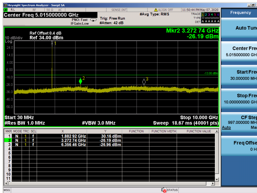
LTE Band 25, 2 / 1.4MHz / 16QAM - RB Size/Offset (3/3) – Mid Channel
