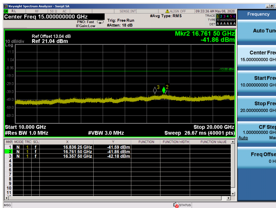
LTE Band 25, 2 / 20MHz / 64QAM - RB Size/Offset (1/0) – Mid Channel
