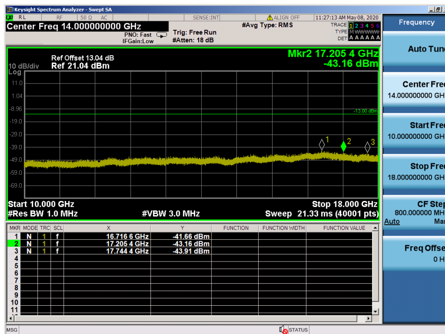
LTE Band 66, 4 / 3MHz / QPSK - RB Size/Offset (8/4) – Mid Channel
