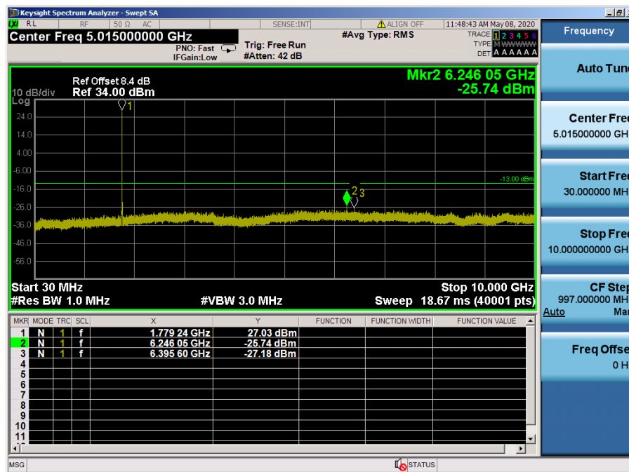
LTE Band 66, 4 / 3MHz / QPSK - RB Size/Offset (8/7) – High Channel
