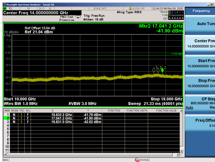
LTE Band 66, 4 / 15MHz / 64QAM - RB Size/Offset (75/0) – Mid Channel
