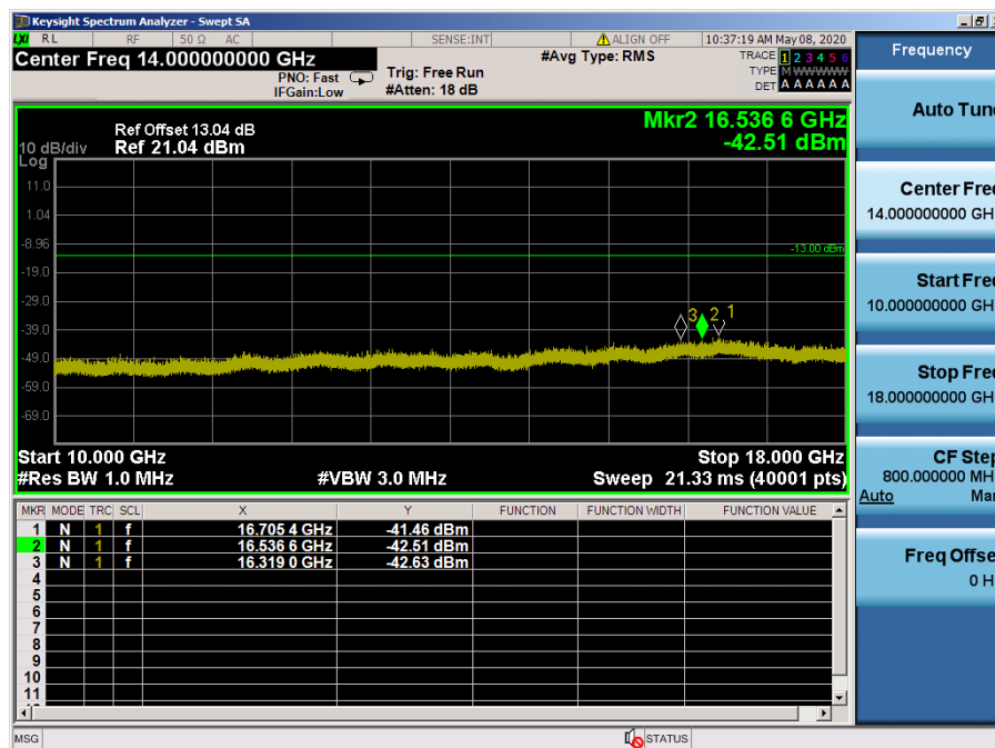
LTE Band 66, 4 / 1.4MHz / QPSK - RB Size/Offset (1/0) – High Channel
