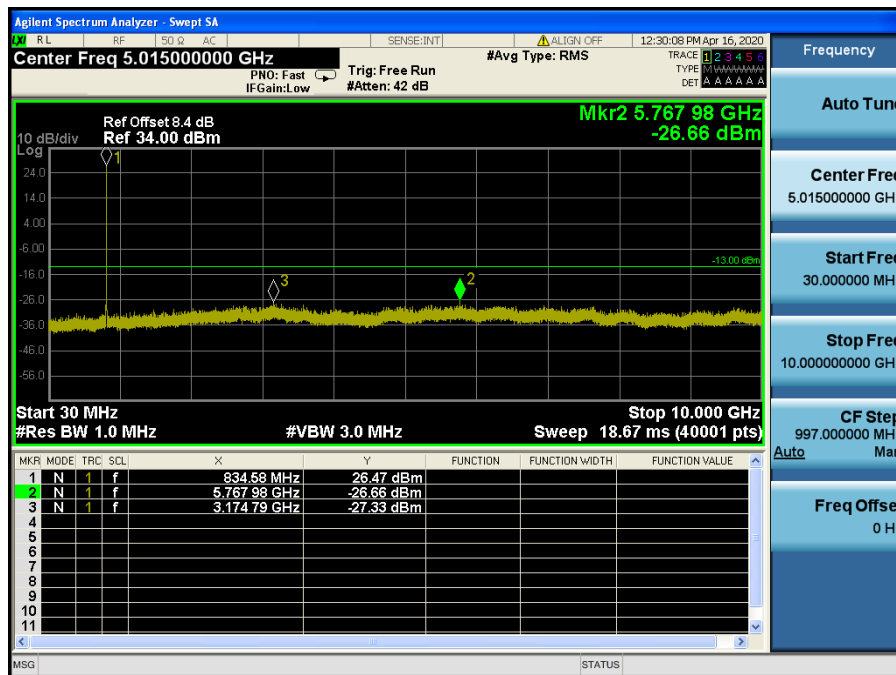
LTE Band 5, 26 / 5MHz / QPSK - RB Size/Offset (12/0) – Mid Channel
