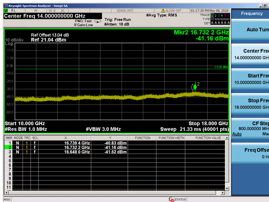
LTE Band 66, 4 / 10MHz / QPSK - RB Size/Offset (50/0) – Mid Channel
