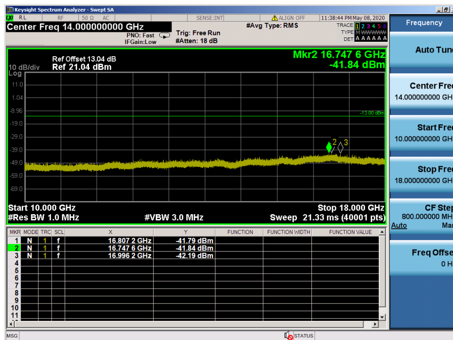
LTE Band 66, 4 / 10MHz / 64QAM - RB Size/Offset (25/12) – Low Channel
