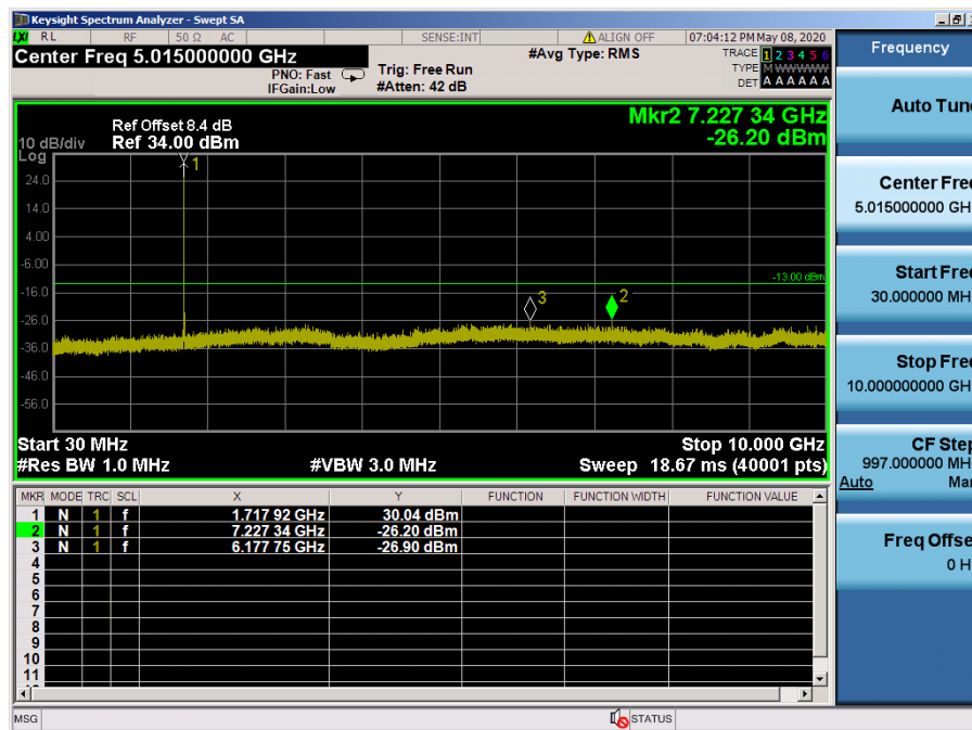
LTE Band 66, 4 / 15MHz / 16QAM - RB Size/Offset (1/36) – Low Channel
