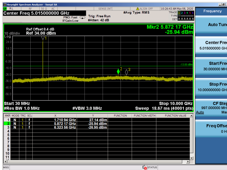
LTE Band 66, 4 / 1.4MHz / QPSK - RB Size/Offset (6/0) – Low Channel
