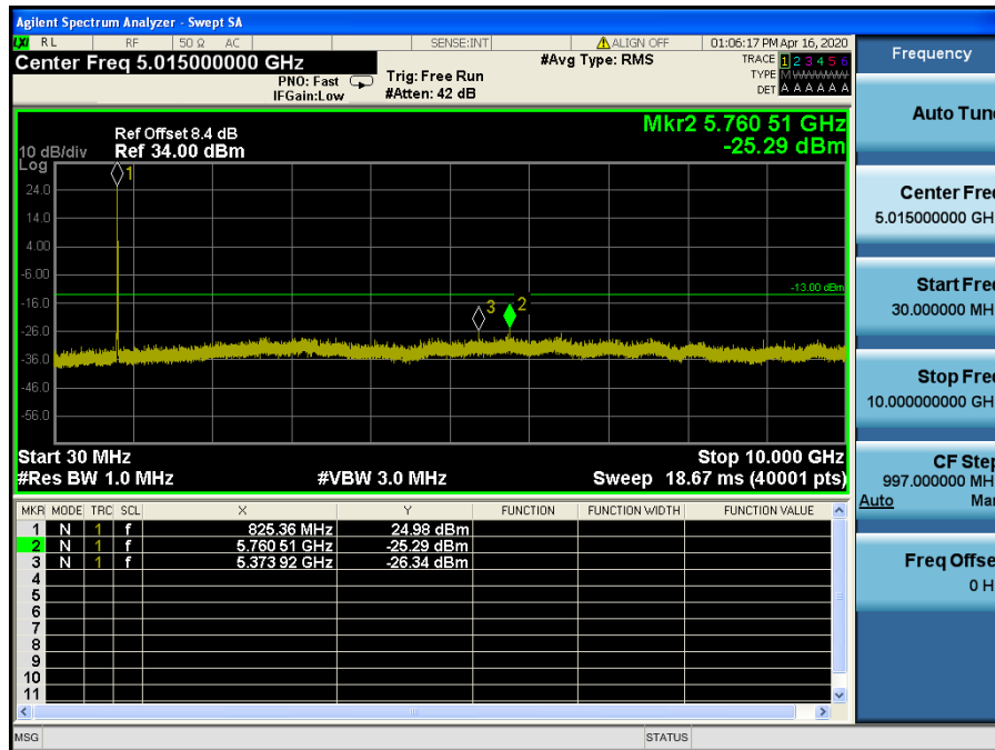
LTE Band 5, 26 / 10MHz / QPSK - RB Size/Offset (25/0) – Low Channel
