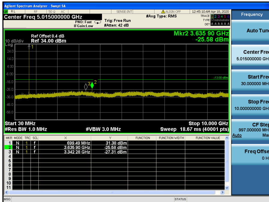
LTE Band 12 / 3MHz / 64QAM - RB Size/Offset (1/0) – Low Channel
