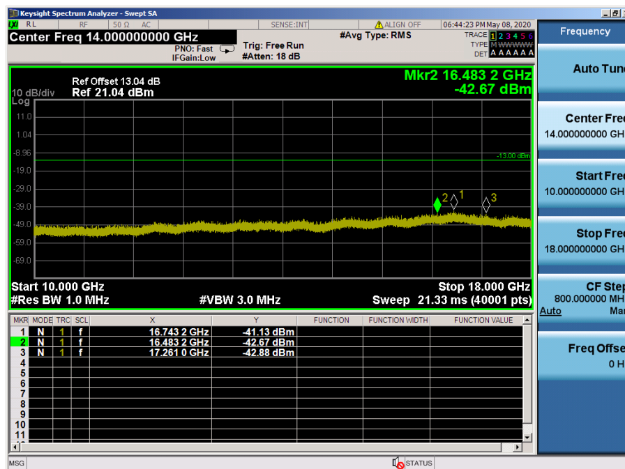
LTE Band 66, 4 / 10MHz / 16QAM - RB Size/Offset (1/49) – High Channel
