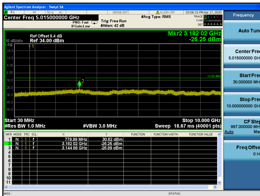
LTE Band 13 / 5MHz / 16QAM - RB Size/Offset (1/12) – Low Channel
