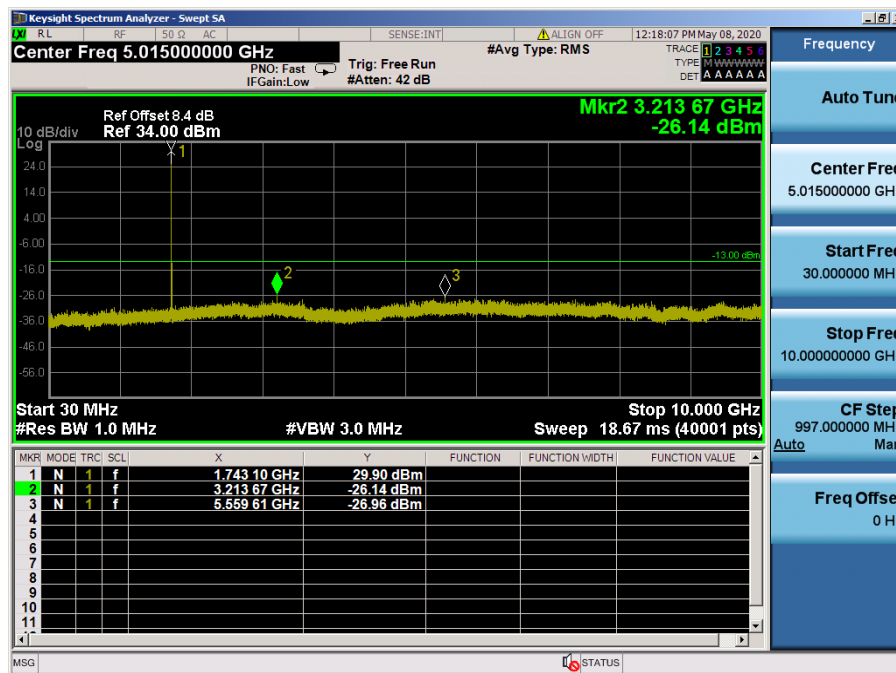
LTE Band 66, 4 / 5MHz / QPSK - RB Size/Offset (1/0) – Mid Channel
