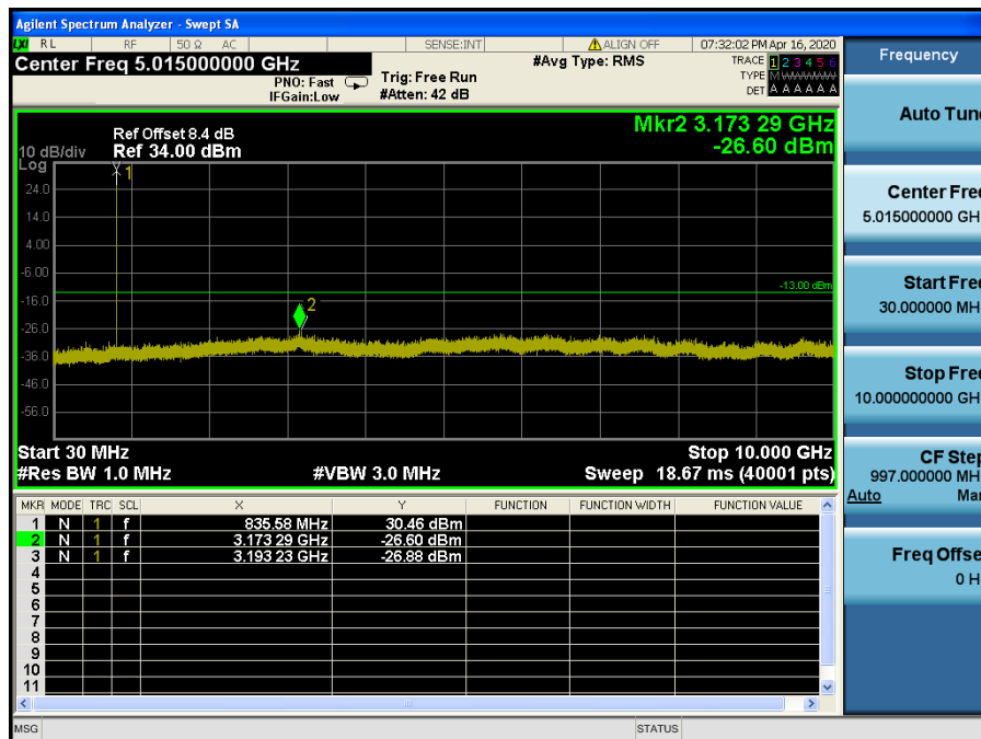
LTE Band 5, 26 / 3MHz / 64QAM - RB Size/Offset (1/0) – Mid Channel
