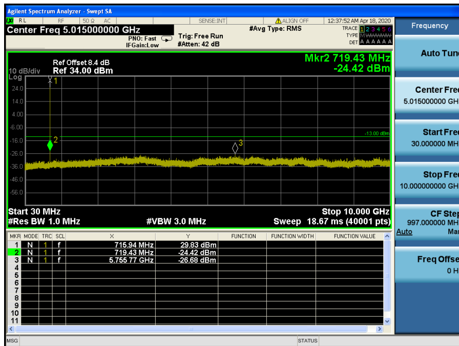
LTE Band 12 / 1.4MHz / 64QAM - RB Size/Offset (3/3) – High Channel
