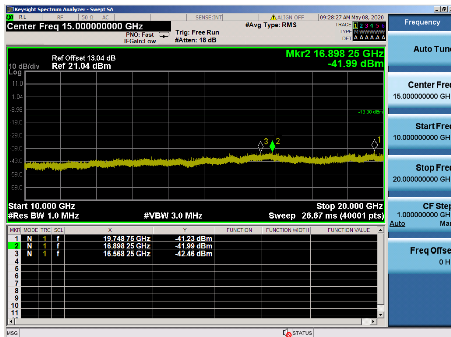
LTE Band 25, 2 / 20MHz / 64QAM - RB Size/Offset (50/50) – Low Channel
