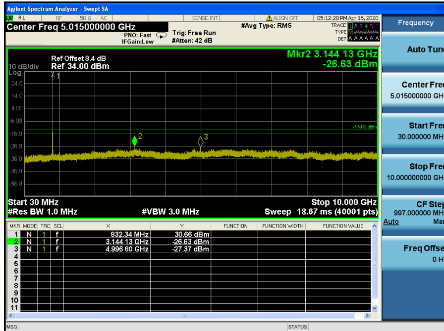
LTE Band 5, 26 / 10MHz / 16QAM - RB Size/Offset (1/0) – Mid Channel
