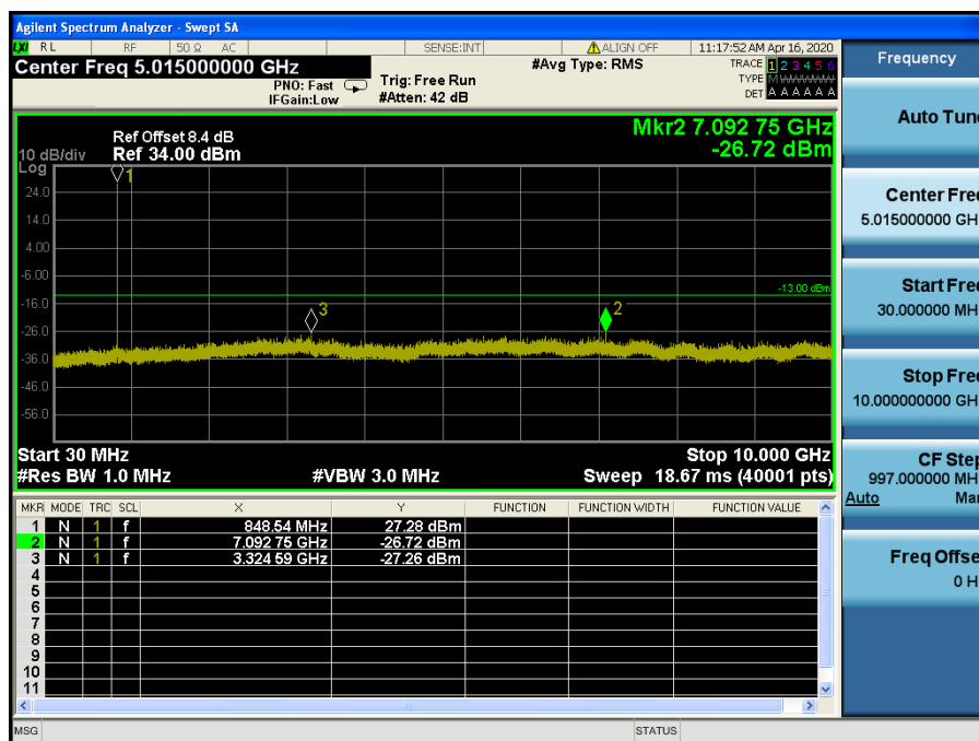
LTE Band 5, 26 / 1.4MHz / QPSK - RB Size/Offset (6/0) – High Channel
