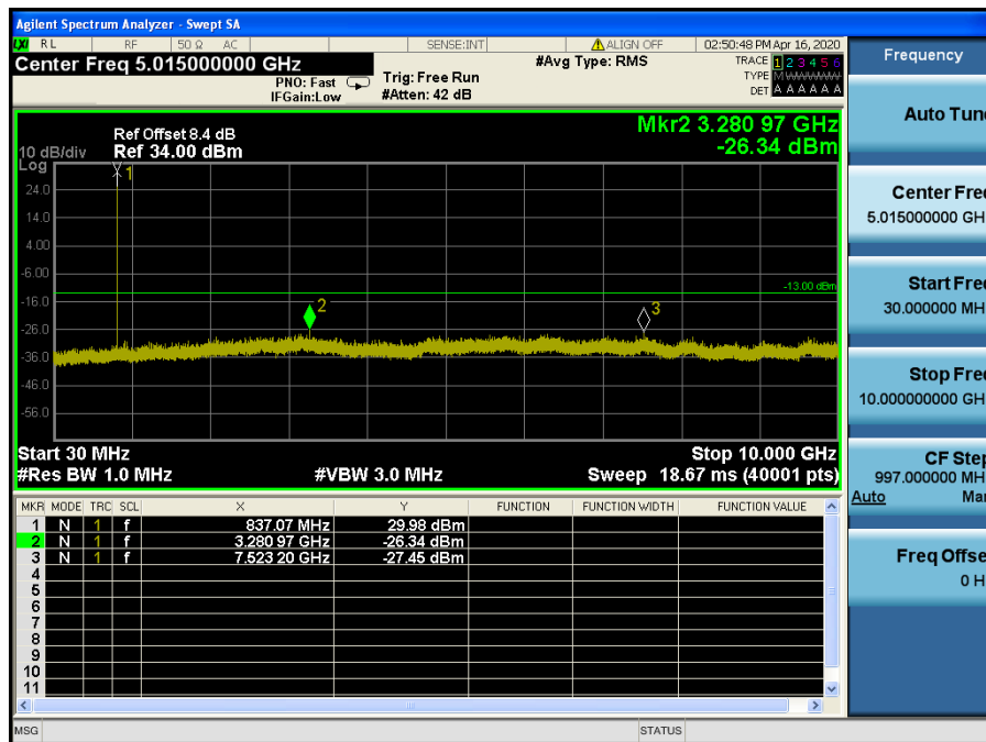
LTE Band 5, 26 / 1.4MHz / 16QAM - RB Size/Offset (3/3) – Mid Channel
