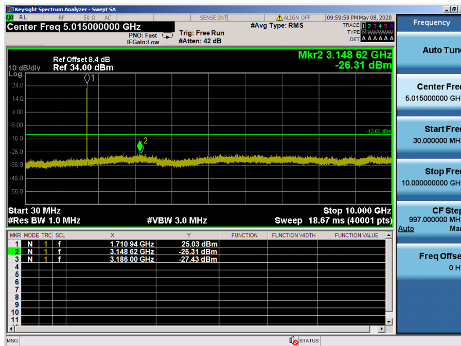
LTE Band 66, 4 / 3MHz / 64QAM - RB Size/Offset (15/0) – Low Channel
