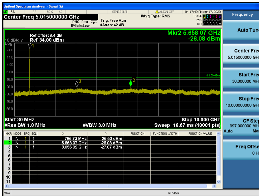
LTE Band 13 / 10MHz / 16QAM - RB Size/Offset (25/25) – Low Channel
