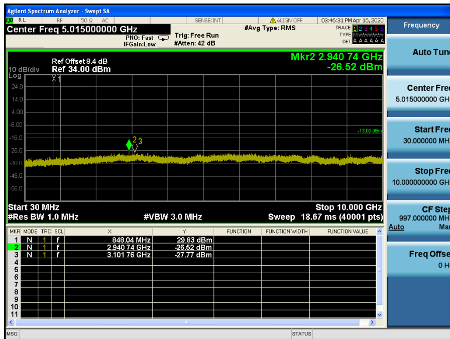
LTE Band 5, 26 / 3MHz / 16QAM - RB Size/Offset (1/7) – High Channel
