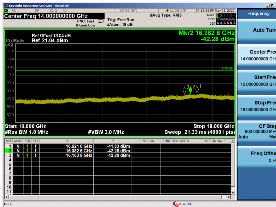
LTE Band 66, 4 / 20MHz / 16QAM - RB Size/Offset (1/0) – Low Channel
