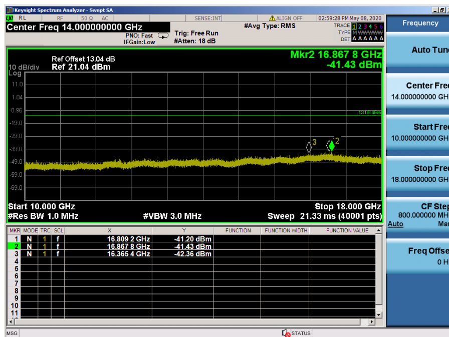
LTE Band 66, 4 / 20MHz / QPSK - RB Size/Offset (50/25) – Mid Channel
