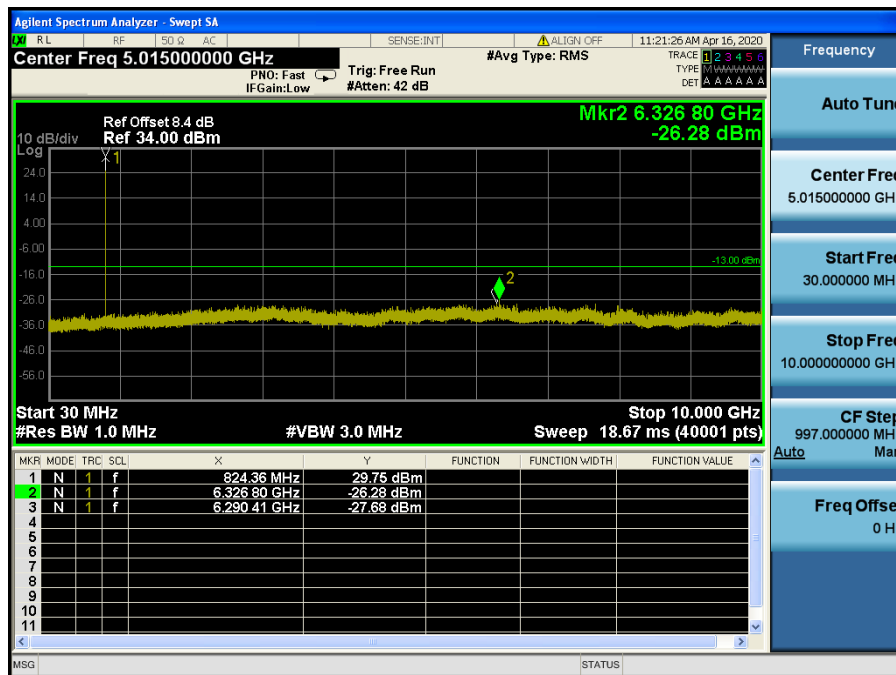
LTE Band 5, 26 / 3MHz / QPSK - RB Size/Offset (1/0) – Low Channel
