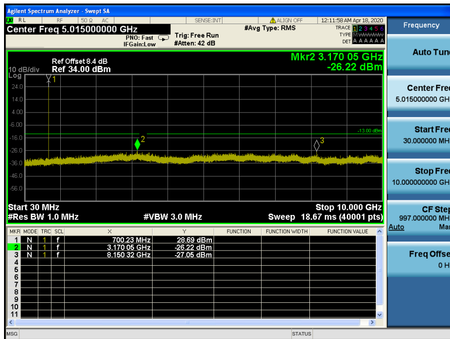
LTE Band 12 / 1.4MHz / 64QAM - RB Size/Offset (3/3) – Low Channel
