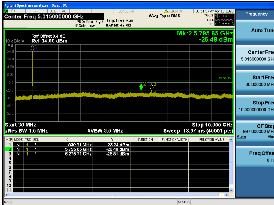
LTE Band 26 / 15MHz / 16QAM - RB Size/Offset (36/0) – High Channel
