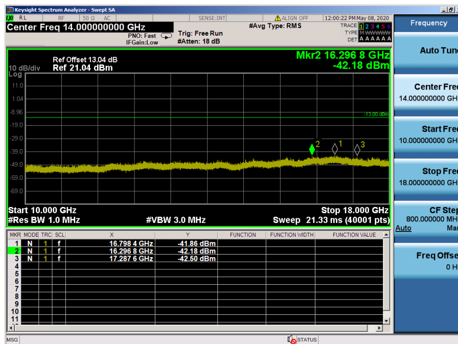
LTE Band 66, 4 / 5MHz / QPSK - RB Size/Offset (1/12) – Low Channel
