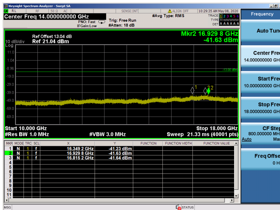
LTE Band 66, 4 / 1.4MHz / QPSK - RB Size/Offset (1/5) – Mid Channel
