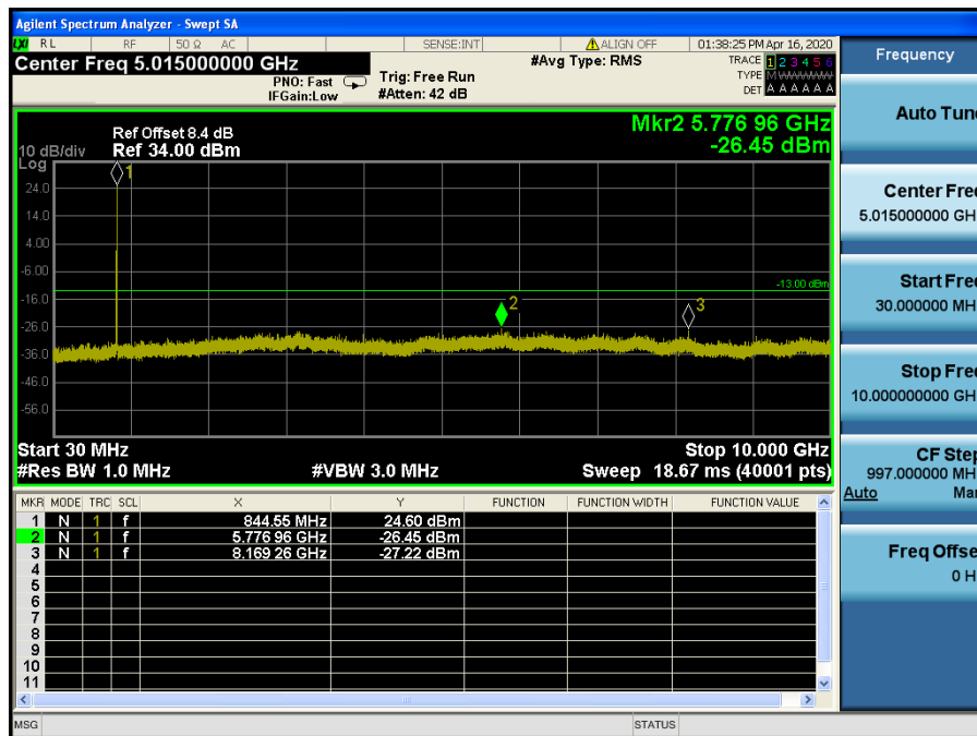
LTE Band 5, 26 / 10MHz / QPSK - RB Size/Offset (25/25) – High Channel
