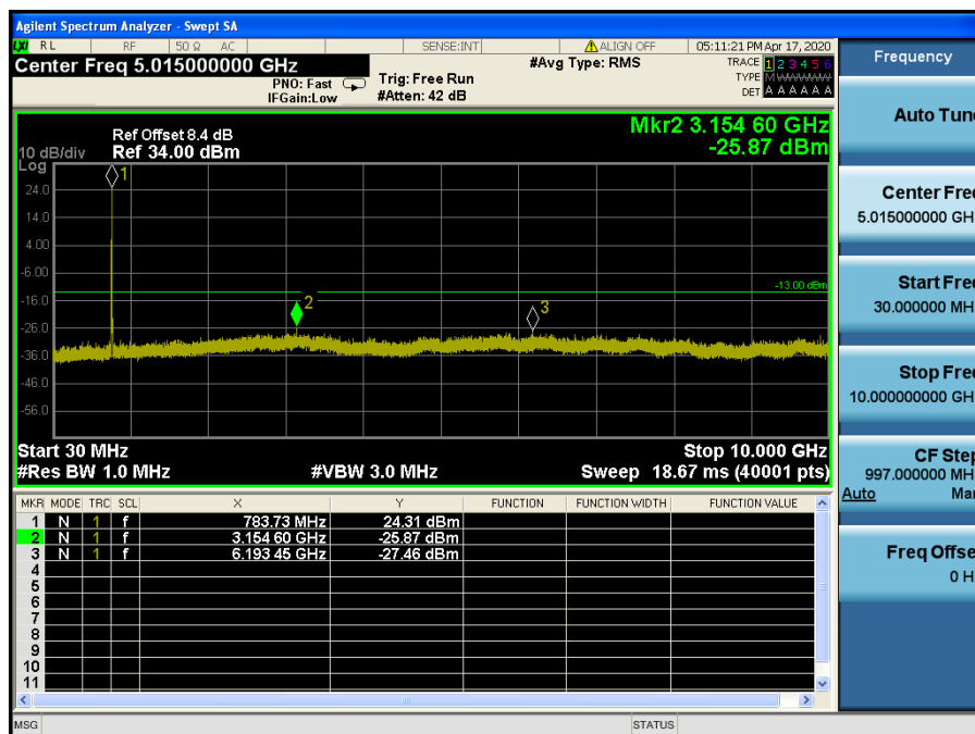
LTE Band 13 / 5MHz / 64QAM - RB Size/Offset (25/0) – High Channel
