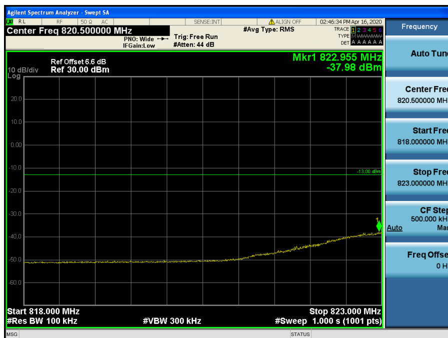
LTE Band 5, 26 / 1.4MHz / 16QAM - RB Size/Offset (6/0)
