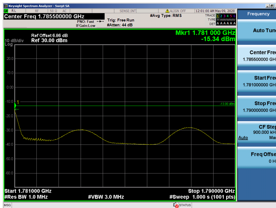
LTE Band 66, 4 / 10MHz / 64QAM - RB Size/Offset (1/49)
