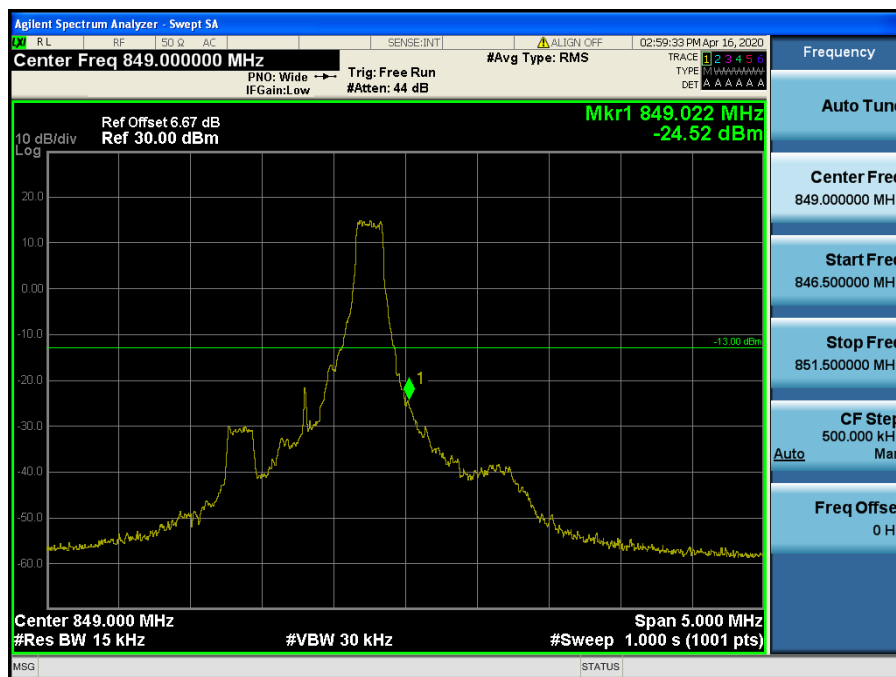
LTE Band 5, 26 / 1.4MHz / 16QAM - RB Size/Offset (1/5)
