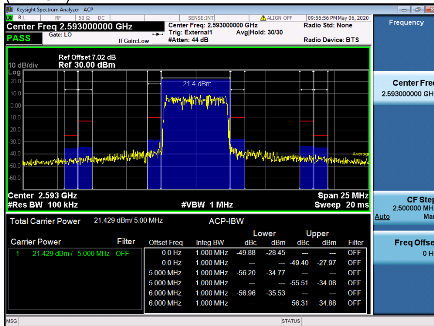
LTE Band 41 / 5MHz / 64QAM - RB Size/Offset (25/0)
