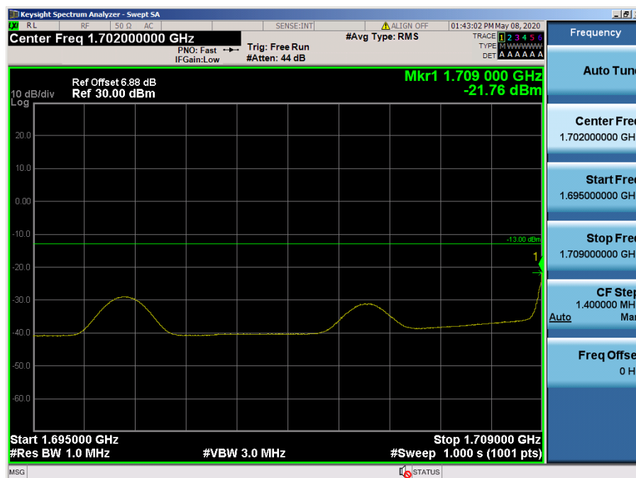
LTE Band 66, 4 / 15MHz / QPSK - RB Size/Offset (1/0)
