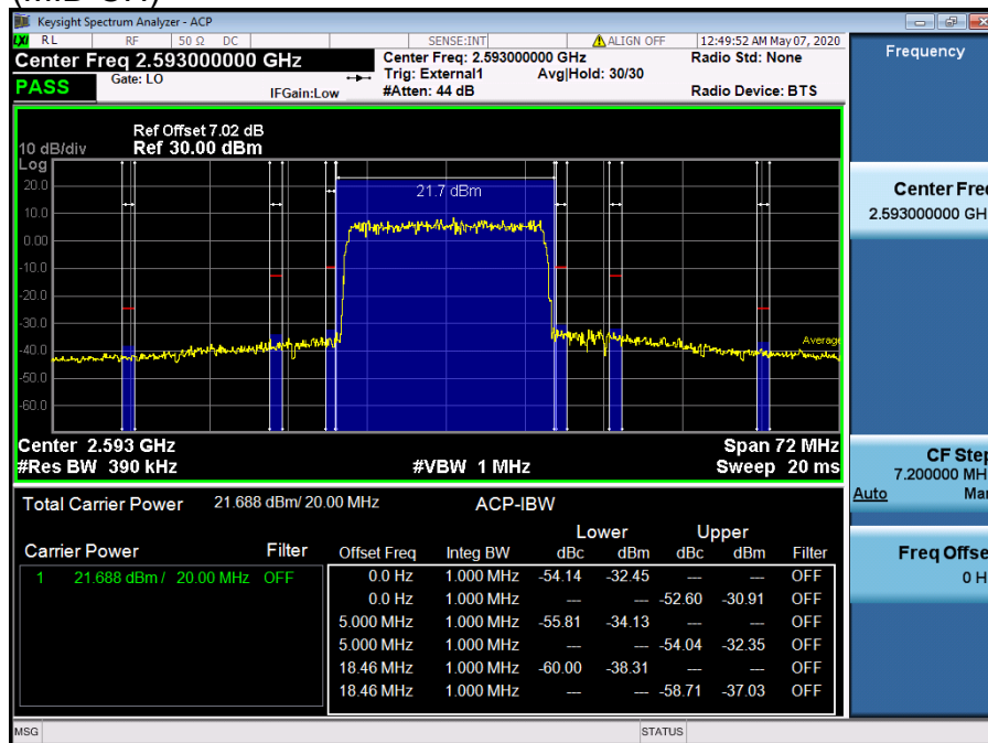
LTE Band 41 / 20MHz / 64QAM - RB Size/Offset (100/0)
