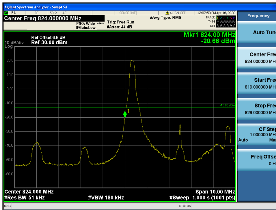
LTE Band 5, 26 / 5MHz / QPSK- RB Size/Offset (1/0)
