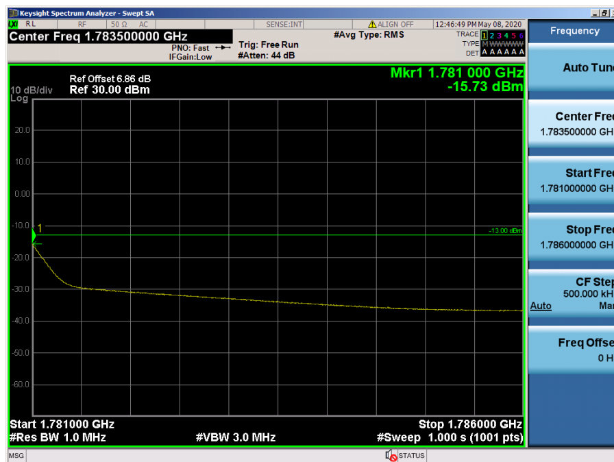
LTE Band 66, 4 / 5MHz / QPSK - RB Size/Offset (25/0)
