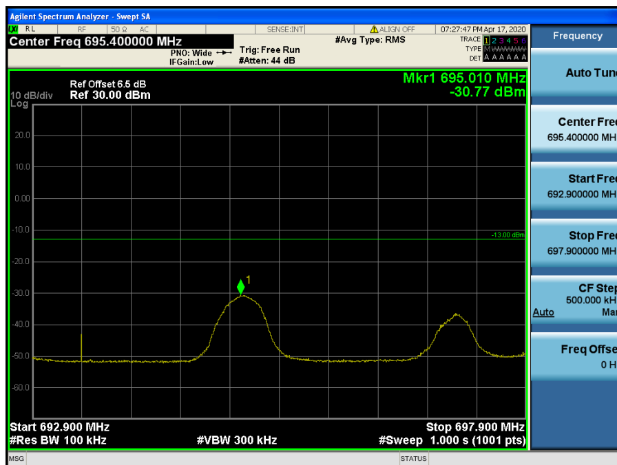
LTE Band 12, 17 / 5MHz / QPSK - RB Size/Offset (1/0)
