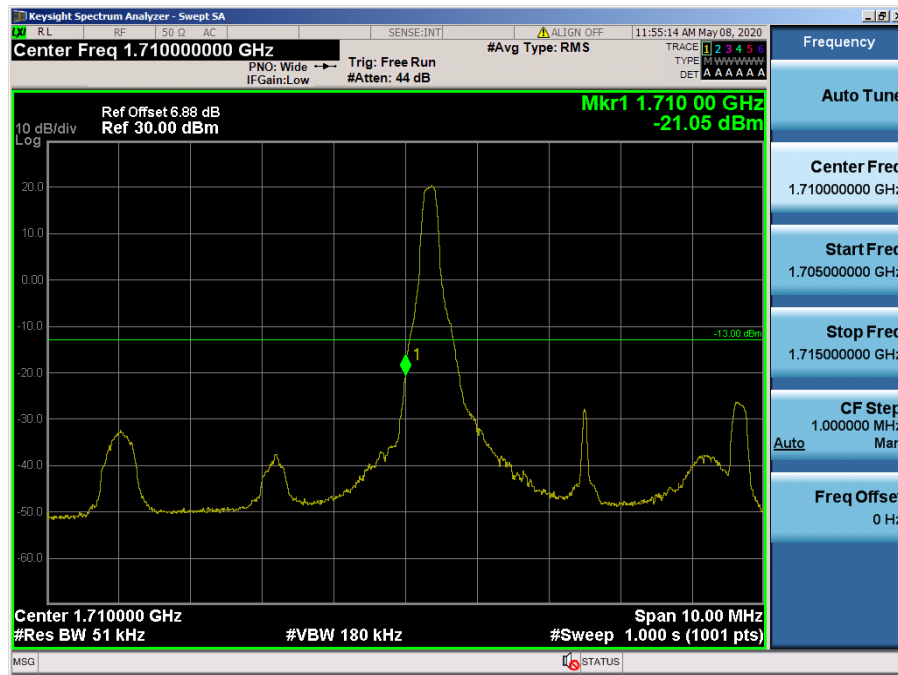
LTE Band 66, 4 / 5MHz / QPSK - RB Size/Offset (1/0)
