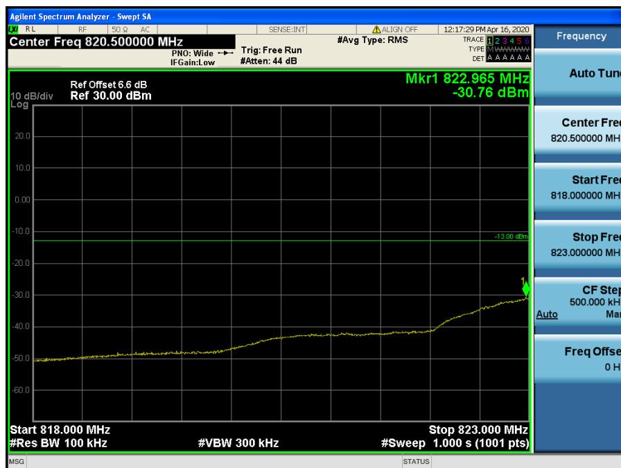
LTE Band 5, 26 / 5MHz / QPSK - RB Size/Offset (12/0)
