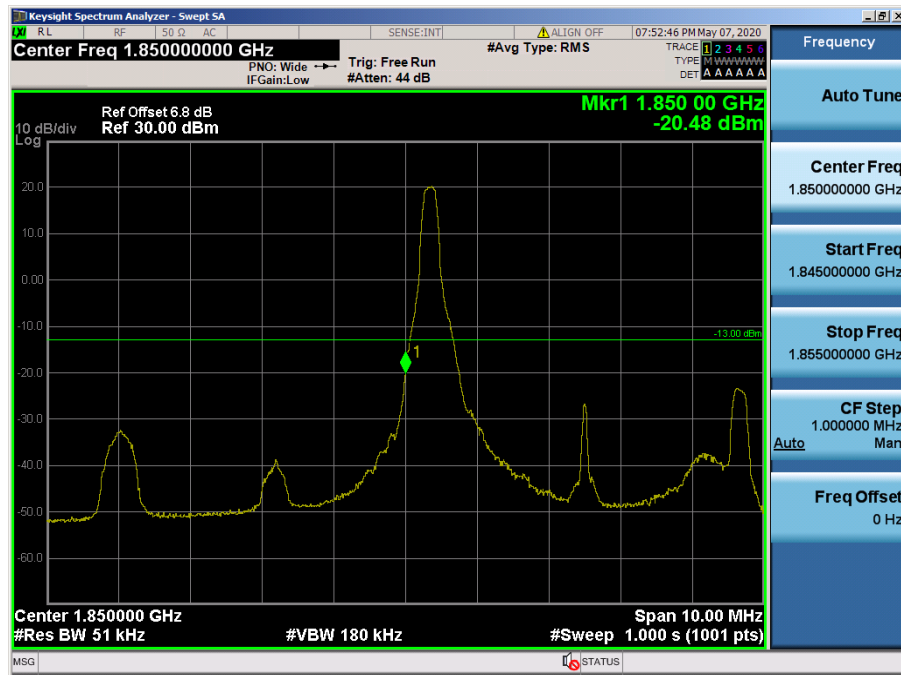
LTE Band 25, 2 / 5MHz / QPSK - RB Size/Offset (1/0)
