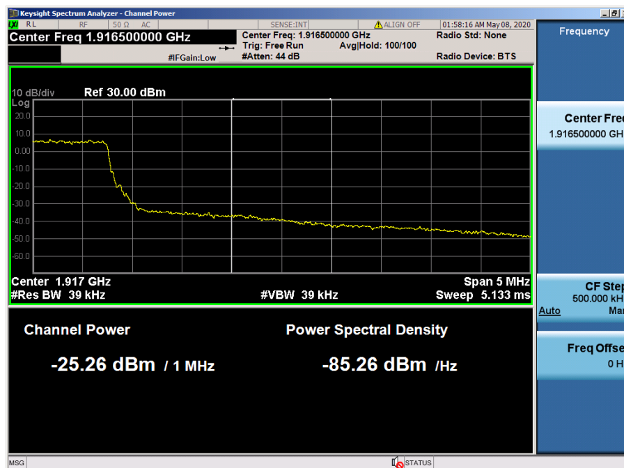
LTE Band 25, 2 / 5MHz / 16QAM - RB Size/Offset (12/13)
