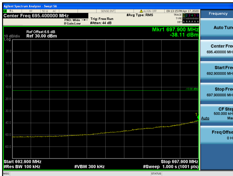
LTE Band 12 / 1.4MHz / 16QAM - RB Size/Offset (6/0)
