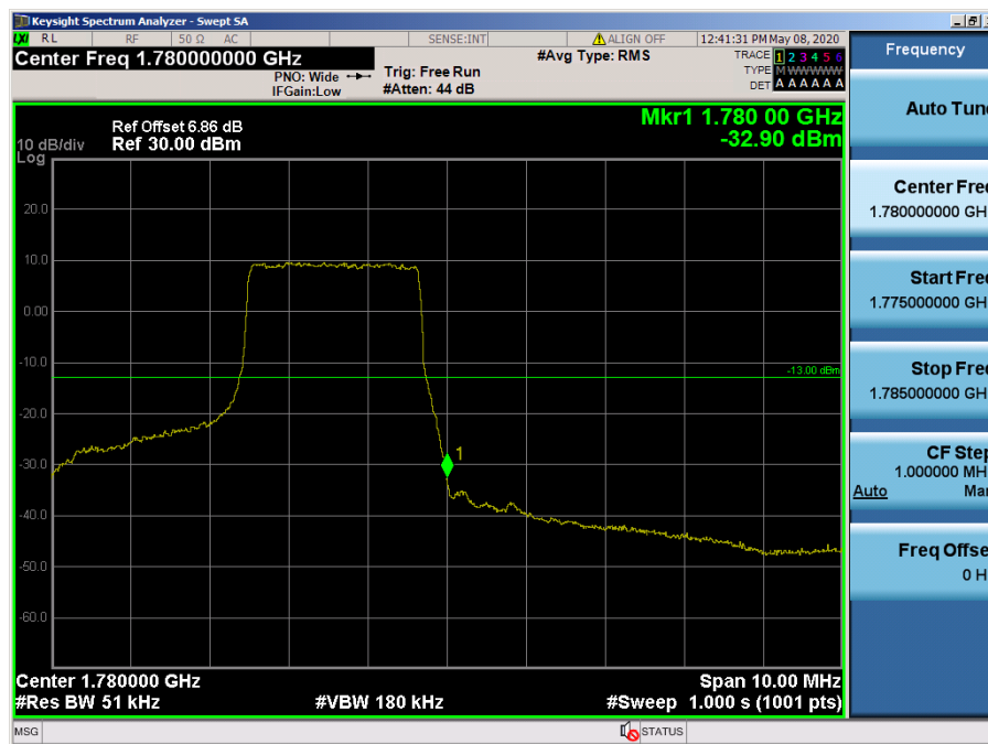
LTE Band 66, 4 / 5MHz / QPSK - RB Size/Offset (12/13)
