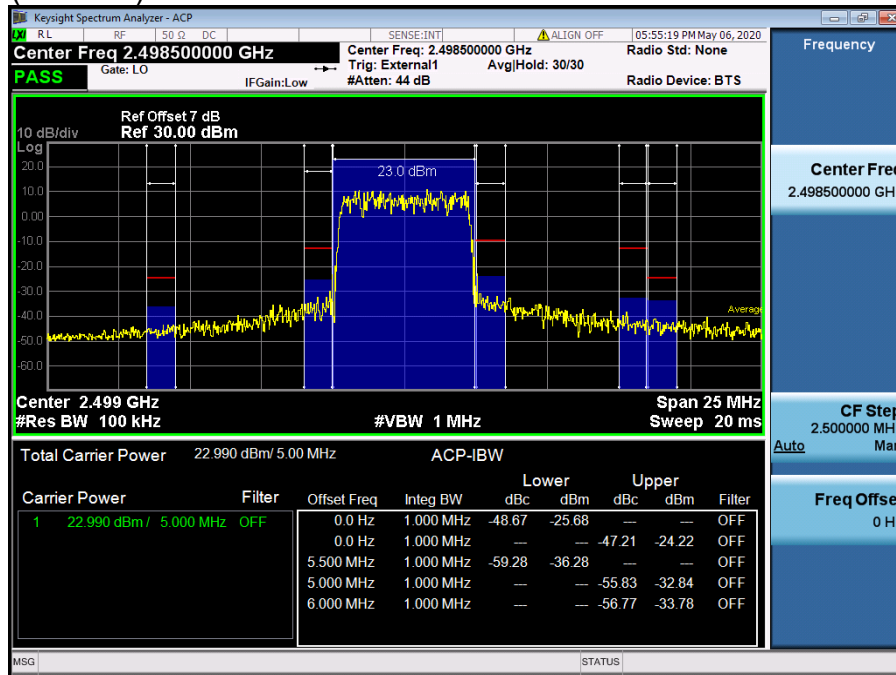
LTE Band 41 / 5MHz / 16QAM - RB Size/Offset (25/0)
