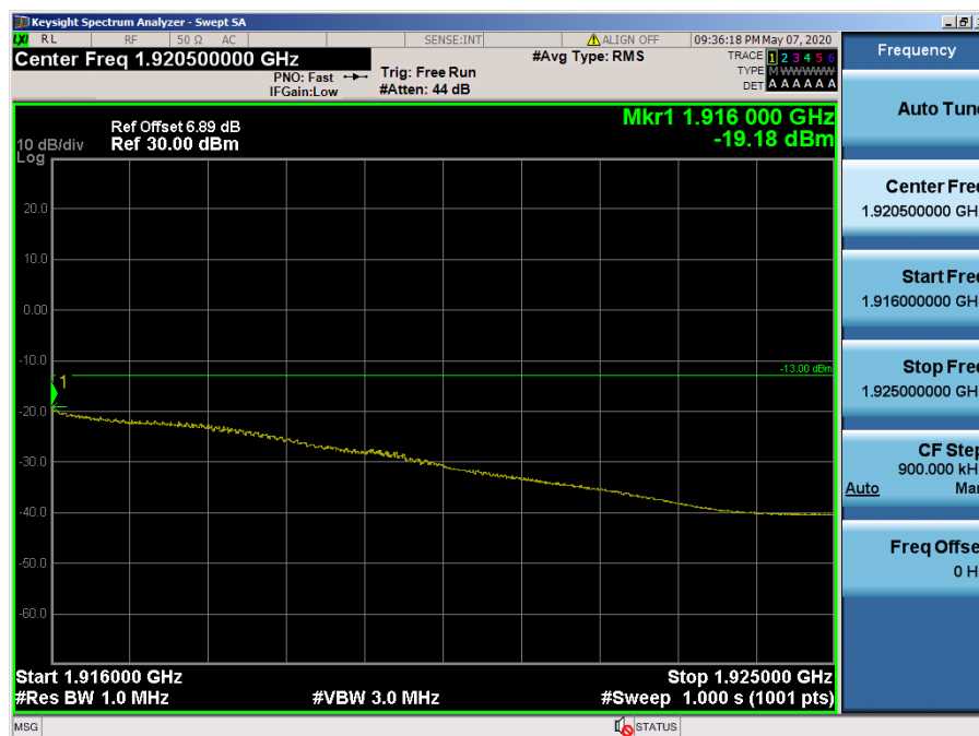
LTE Band 25, 2 / 10MHz / QPSK- RB Size/Offset (50/0)
