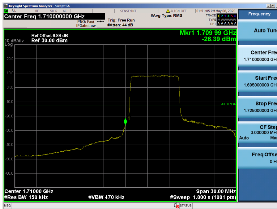
LTE Band 66, 4 / 15MHz / QPSK - RB Size/Offset (36/0)
