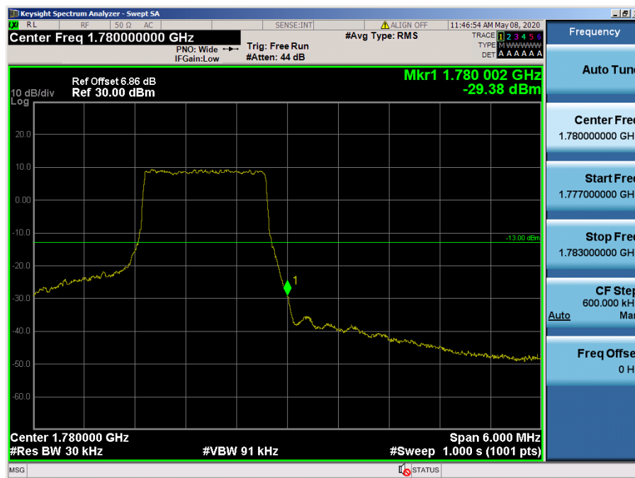
LTE Band 66, 4 / 3MHz / QPSK - RB Size/Offset (8/7)
