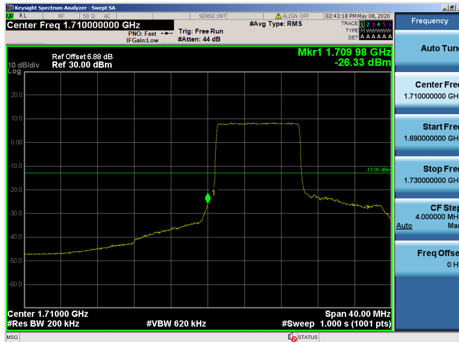
LTE Band 66, 4 / 20MHz / QPSK - RB Size/Offset (50/0)
