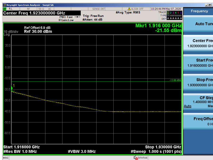
LTE Band 25, 2 / 15MHz / QPSK - RB Size/Offset (36/39)
