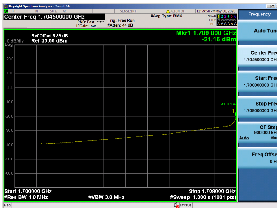
LTE Band 66, 4 / 10MHz / QPSK - RB Size/Offset (25/0)
