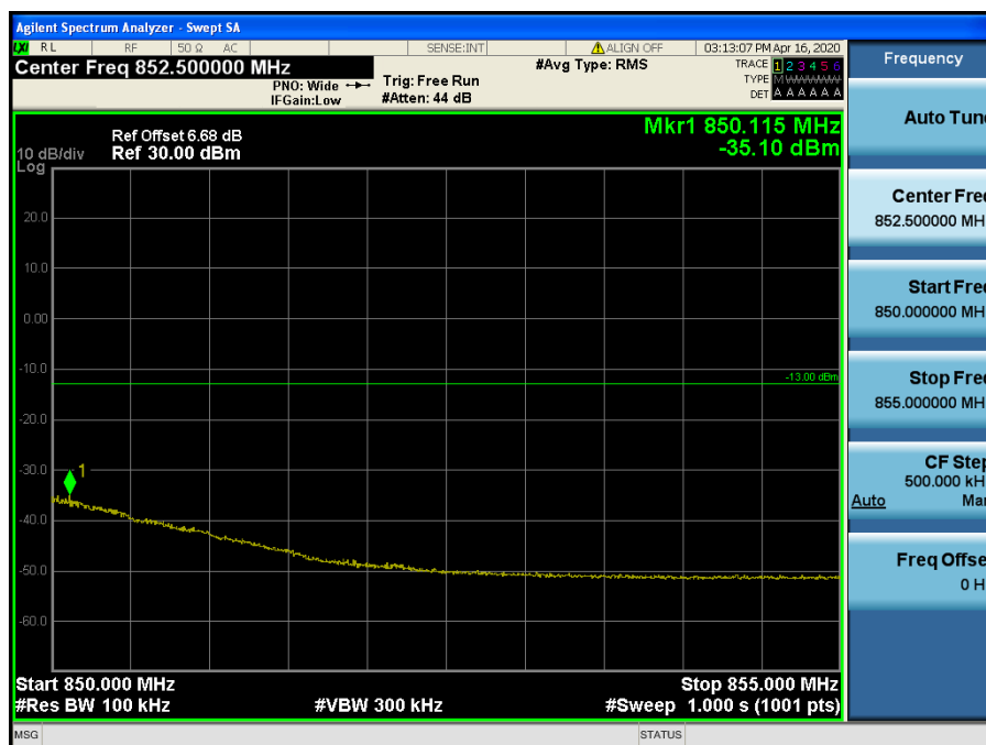
LTE Band 5, 26 / 1.4MHz / QPSK - RB Size/Offset (6/0)
