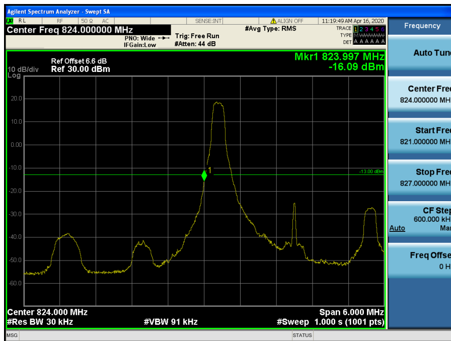
LTE Band 5, 26 / 3MHz / QPSK - RB Size/Offset (1/0)
