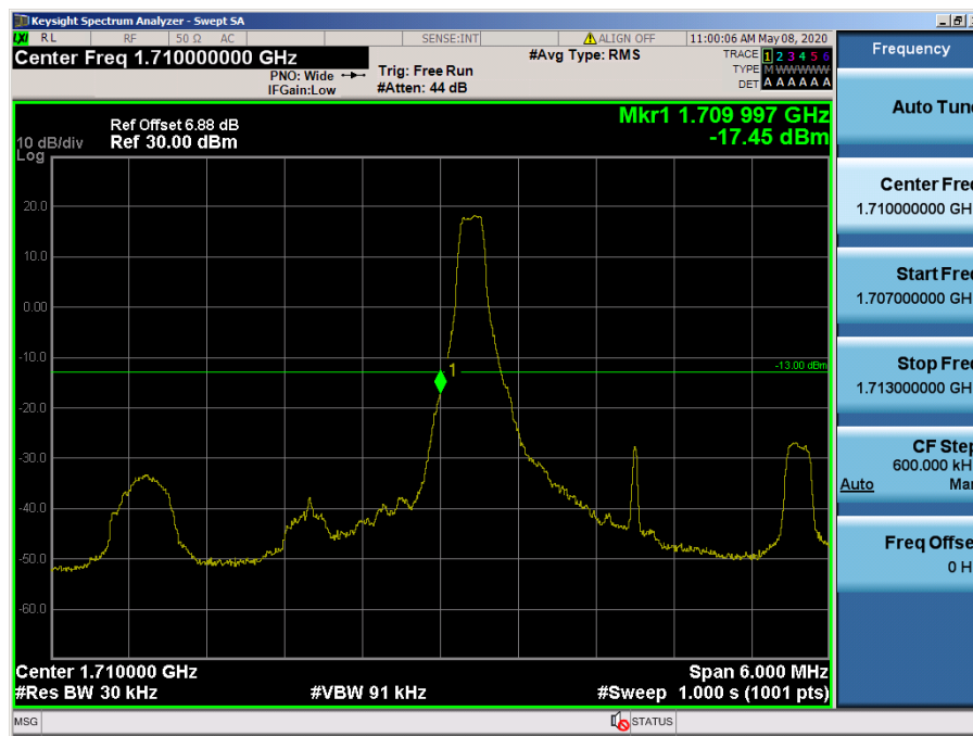
LTE Band 66, 4 / 3MHz / QPSK - RB Size/Offset (1/0)
