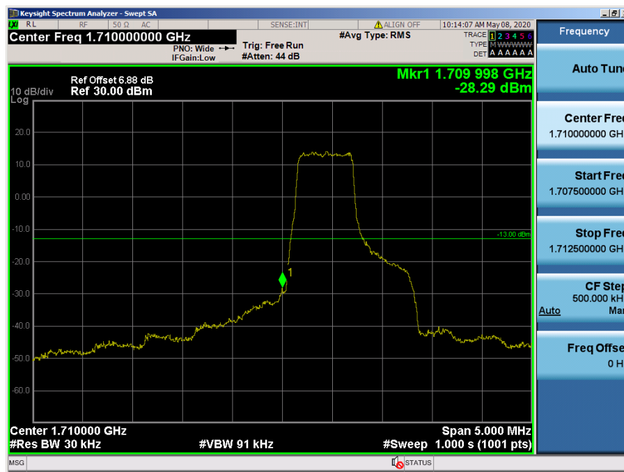
LTE Band 66, 4 / 1.4MHz / QPSK - RB Size/Offset (3/0)
