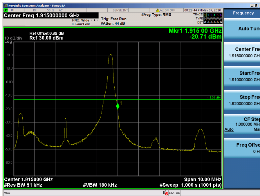
LTE Band 25, 2 / 5MHz / QPSK - RB Size/Offset (1/24)
