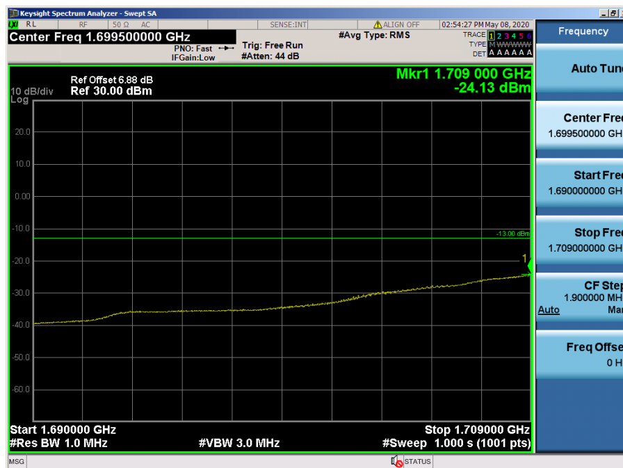
LTE Band 66, 4 / 20MHz / QPSK - RB Size/Offset (100/0)
