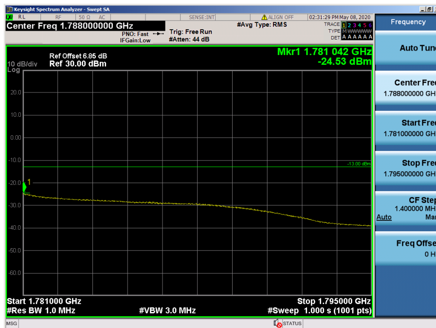
LTE Band 66, 4 / 15MHz / QPSK - RB Size/Offset (75/0)
