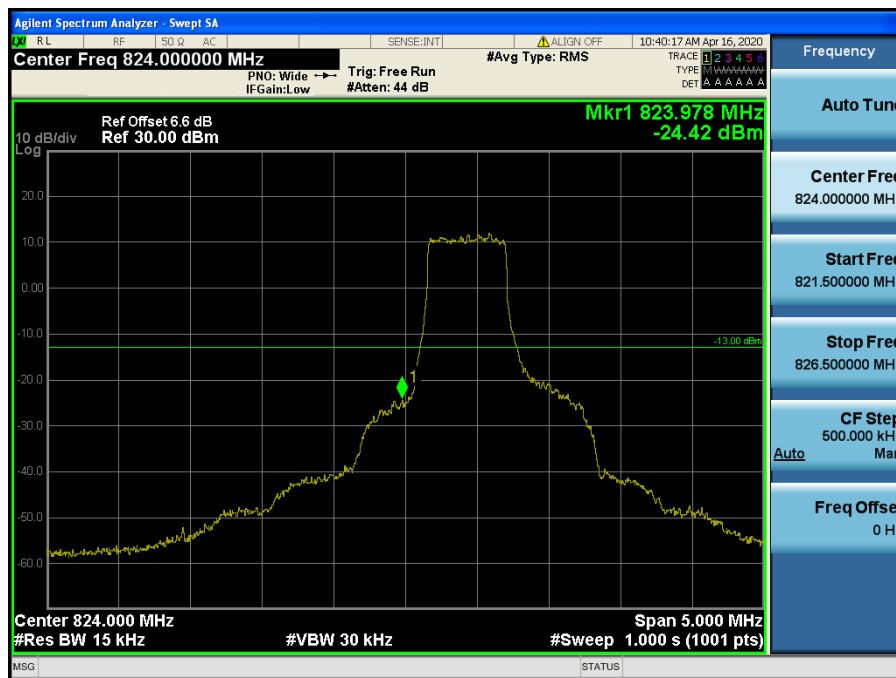
LTE Band 5, 26 / 1.4MHz / QPSK - RB Size/Offset (3/0)
