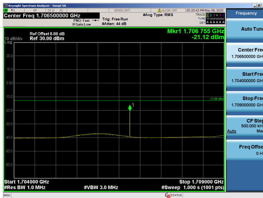
LTE Band 66, 4 / 5MHz / 16QAM - RB Size/Offset (1/24)
