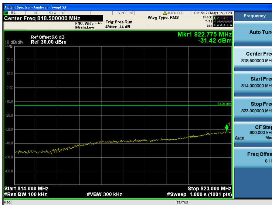
LTE Band 5, 26 / 10MHz / QPSK - RB Size/Offset (50/0)
