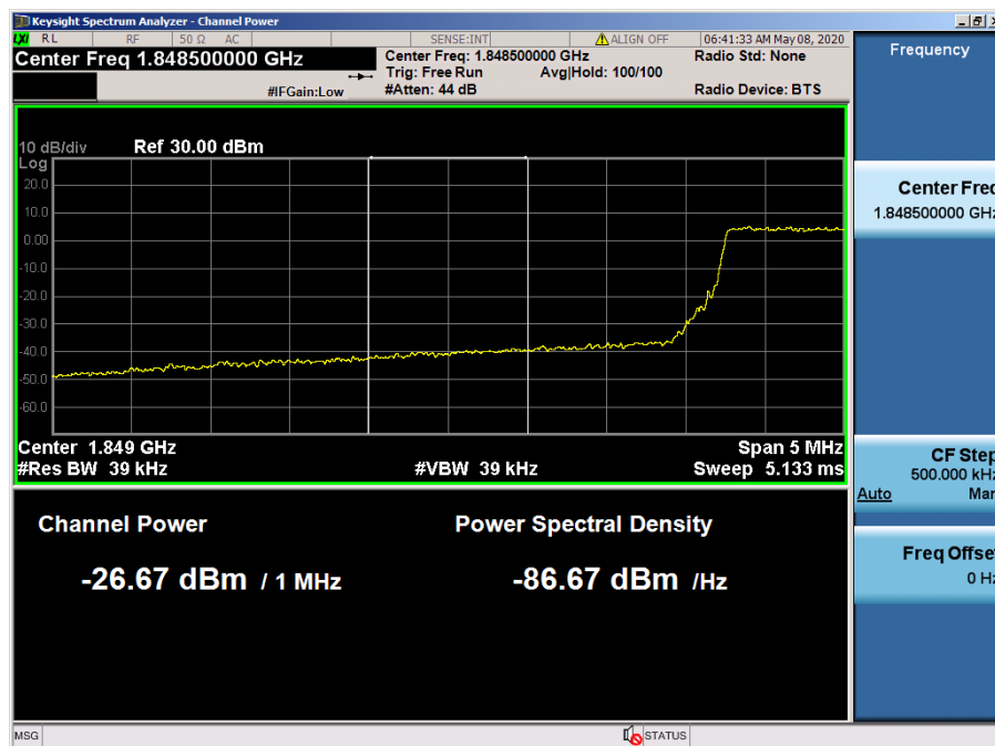
LTE Band 25, 2 / 5MHz / 64QAM - RB Size/Offset (12/0)
