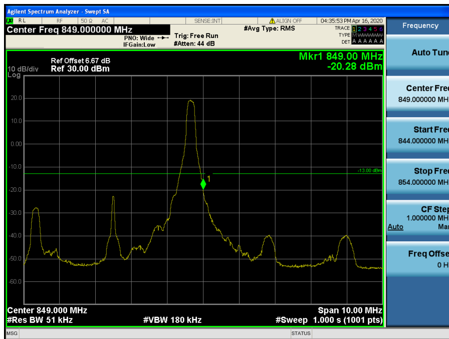
LTE Band 5, 26 / 5MHz / 16QAM - RB Size/Offset (1/24)
