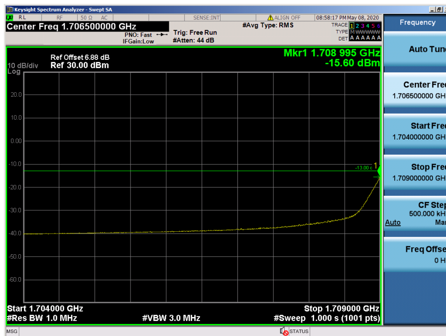
LTE Band 66, 4 / 1.4MHz / 64QAM - RB Size/Offset (3/2)
