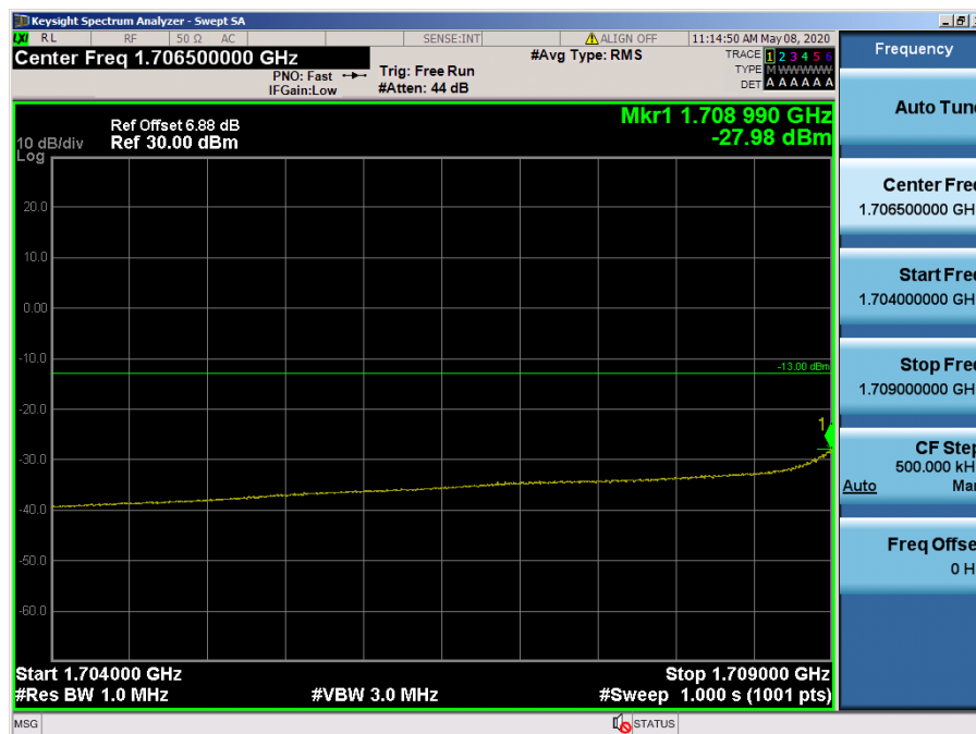
LTE Band 66, 4 / 3MHz / QPSK - RB Size/Offset (8/4)
