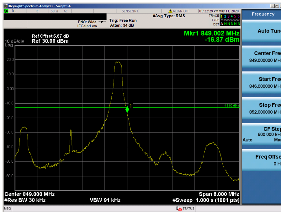
LTE Band 5, 26 / 3MHz / 16QAM - RB Size/Offset (1/14)
