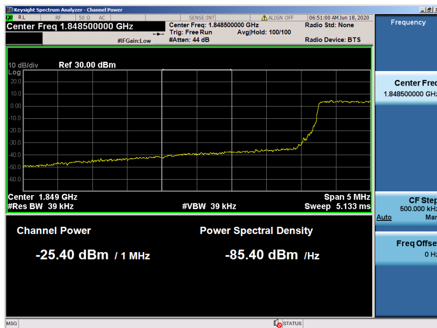
LTE Band 2 / 5 MHz / 64QAM - RB Size/Offset (12/0)
