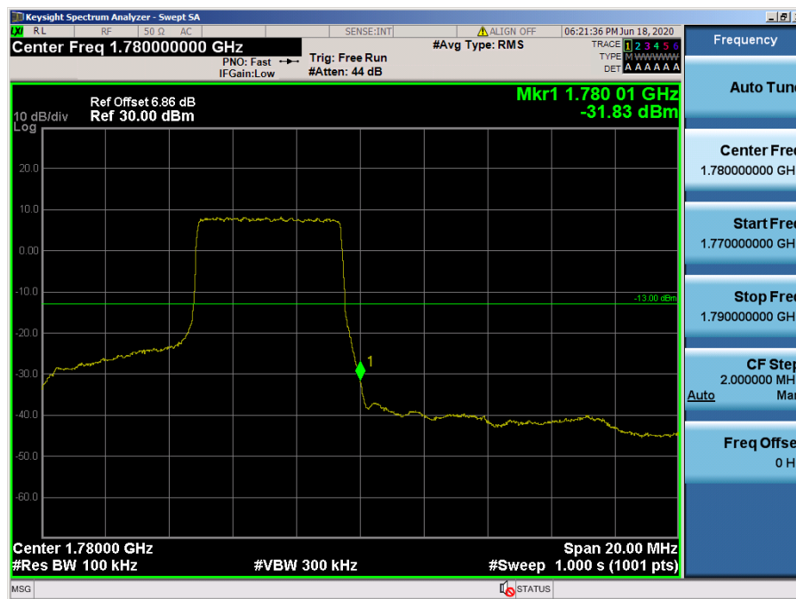
LTE Band 66, 4 / 10 MHz / QPSK - RB Size/Offset (25/25)
