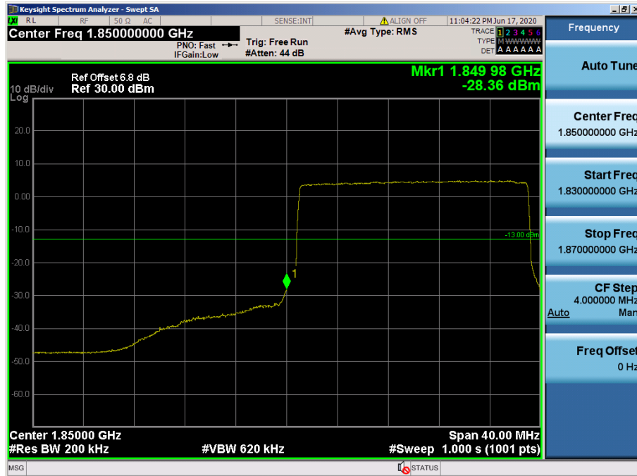
LTE Band 2 / 20 MHz / QPSK - RB Size/Offset (100/0)
