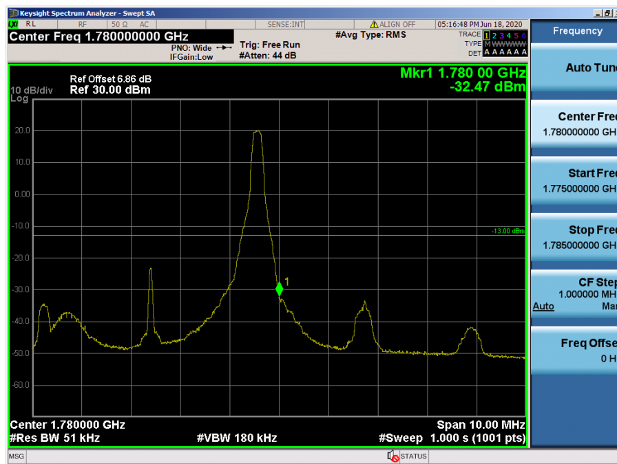
LTE Band 66, 4 / 5 MHz / QPSK - RB Size/Offset (1/24)
