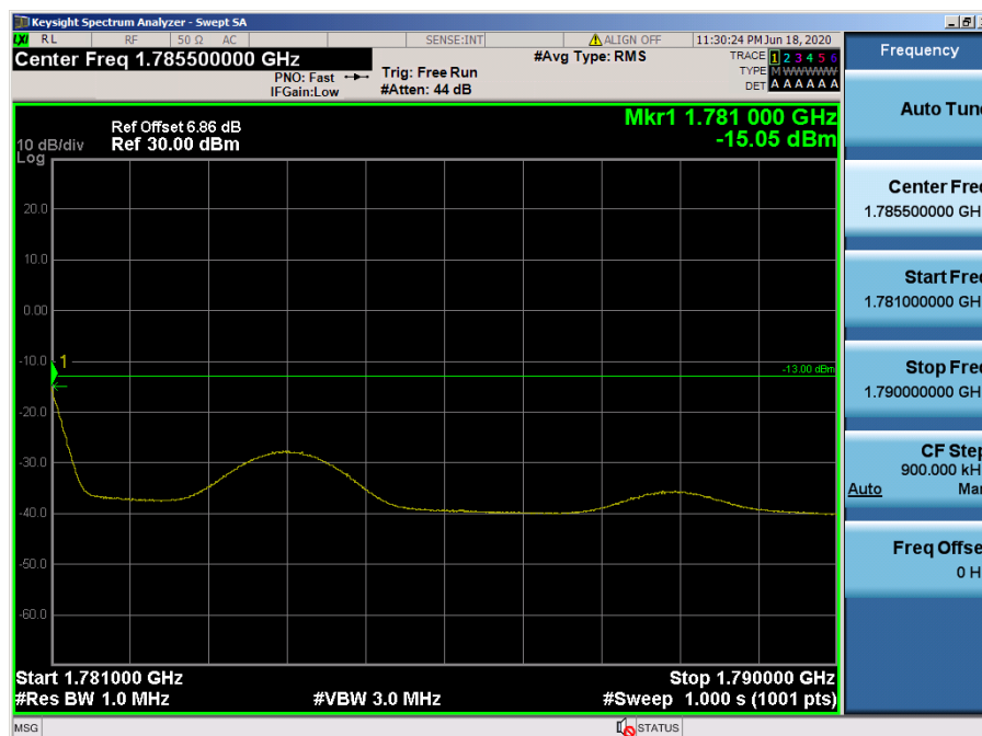
LTE Band 66, 4 / 10 MHz / 16QAM - RB Size/Offset (1/49)
