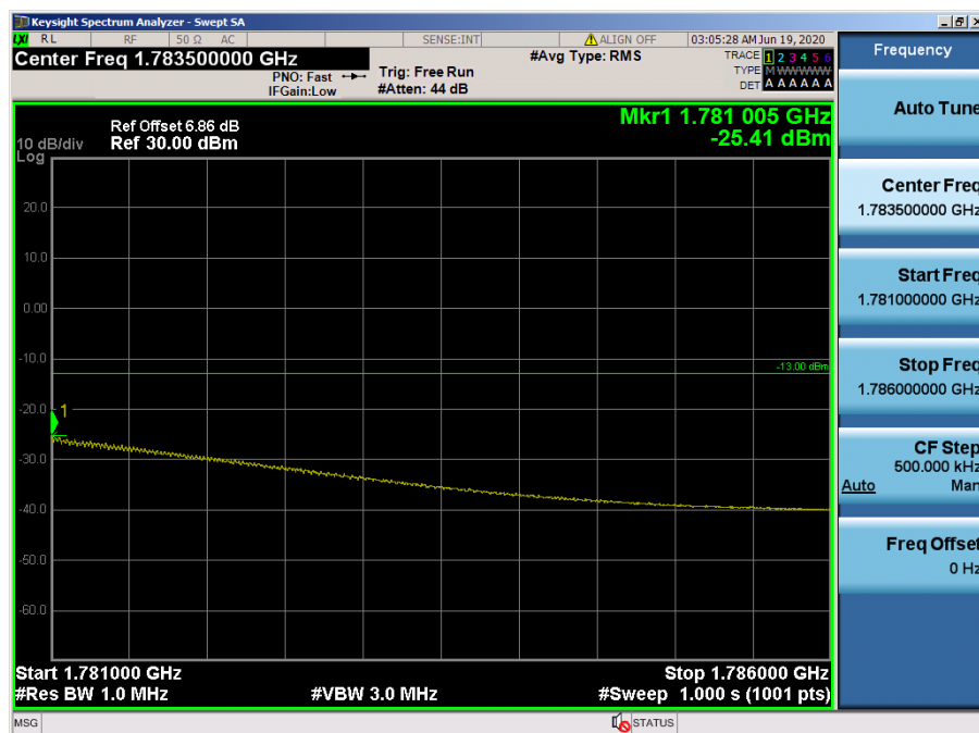
LTE Band 66, 4 / 3MHz / 64QAM - RB Size/Offset (8/4)
