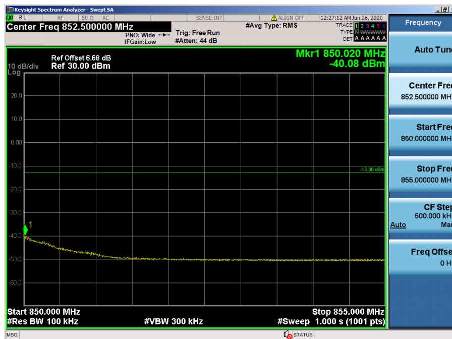
LTE Band 5 / 1.4 MHz / 16QAM - RB Size/Offset (3/3)
