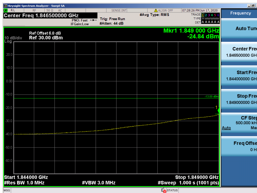
LTE Band 2 / 3MHz / QPSK - RB Size/Offset (8/4)
