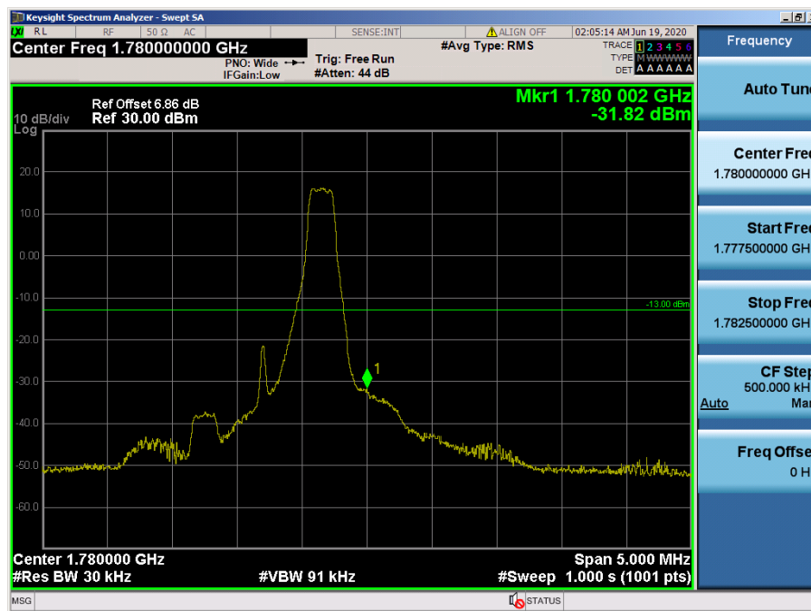
LTE Band 66, 4 / 1.4 MHz / 64QAM - RB Size/Offset (1/5)
