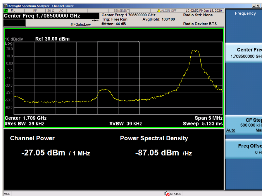
LTE Band 66, 4 / 5 MHz / 16QAM - RB Size/Offset (1/0)
