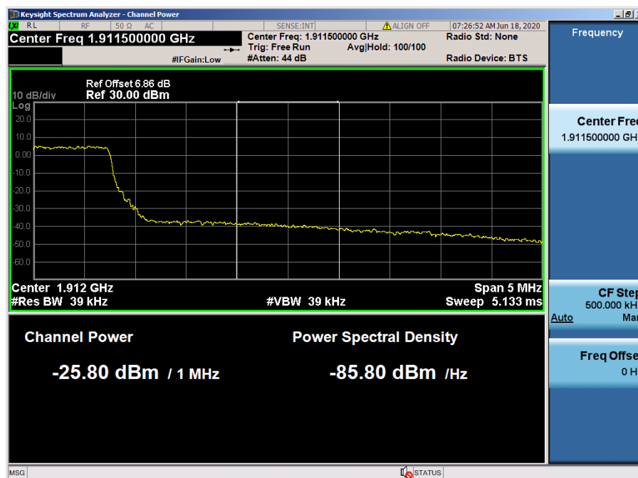
LTE Band 2 / 5 MHz / 64QAM - RB Size/Offset (12/13)
