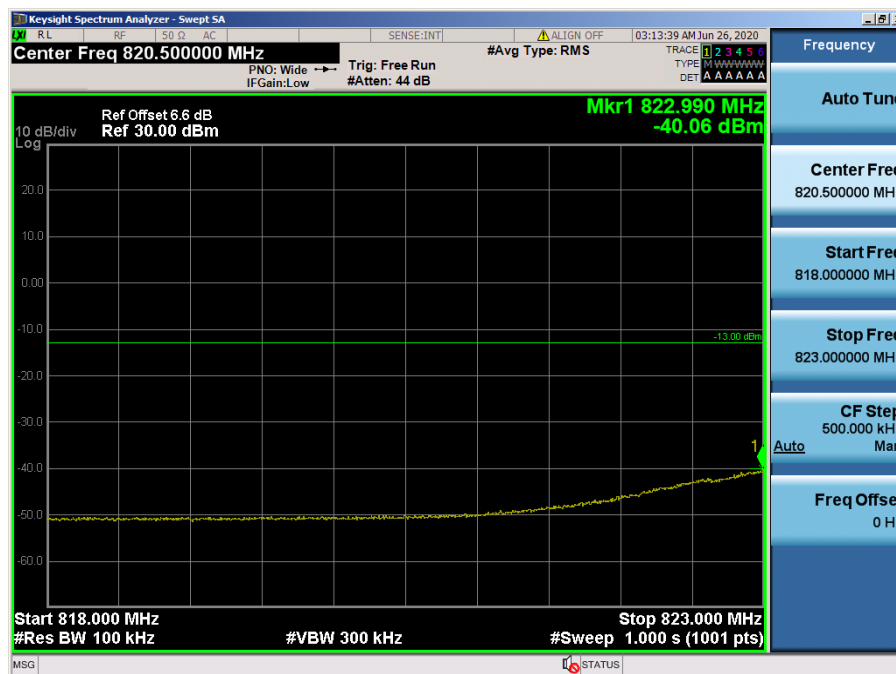
LTE Band 5 / 1.4 MHz / 64QAM - RB Size/Offset (6/0)
