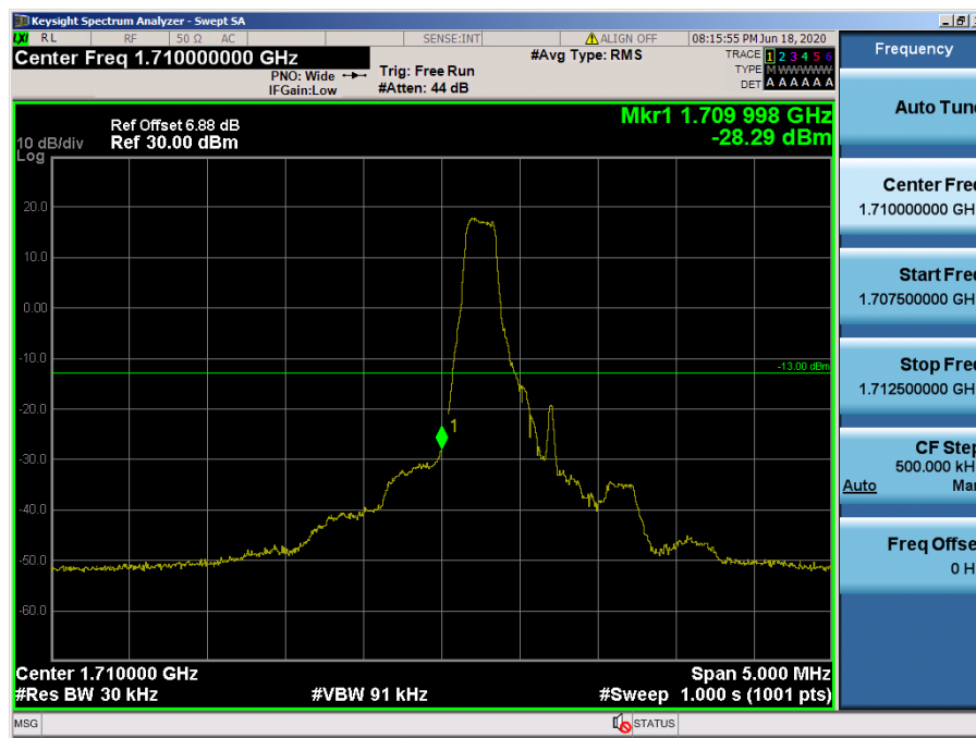
LTE Band 66, 4 / 1.4 MHz / 16QAM - RB Size/Offset (1/0)
