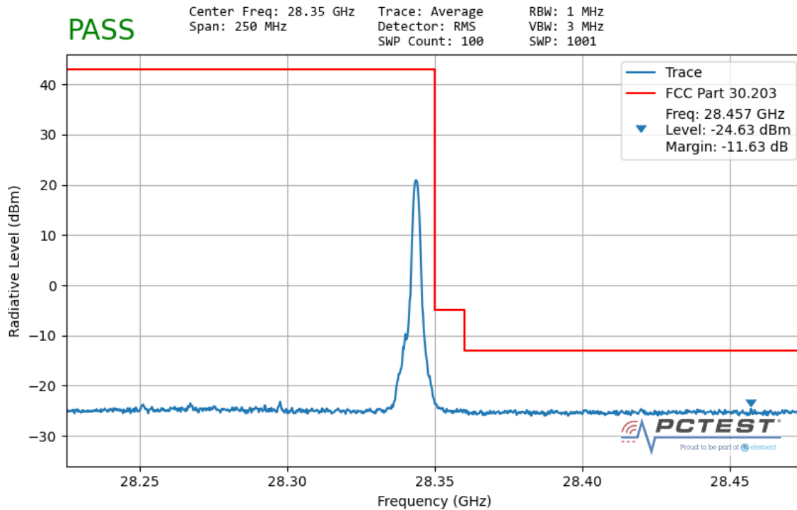
Plot 7-69. Ant 1 Upper Band Edge (100MHz-1CC – QPSK 1 RB)
