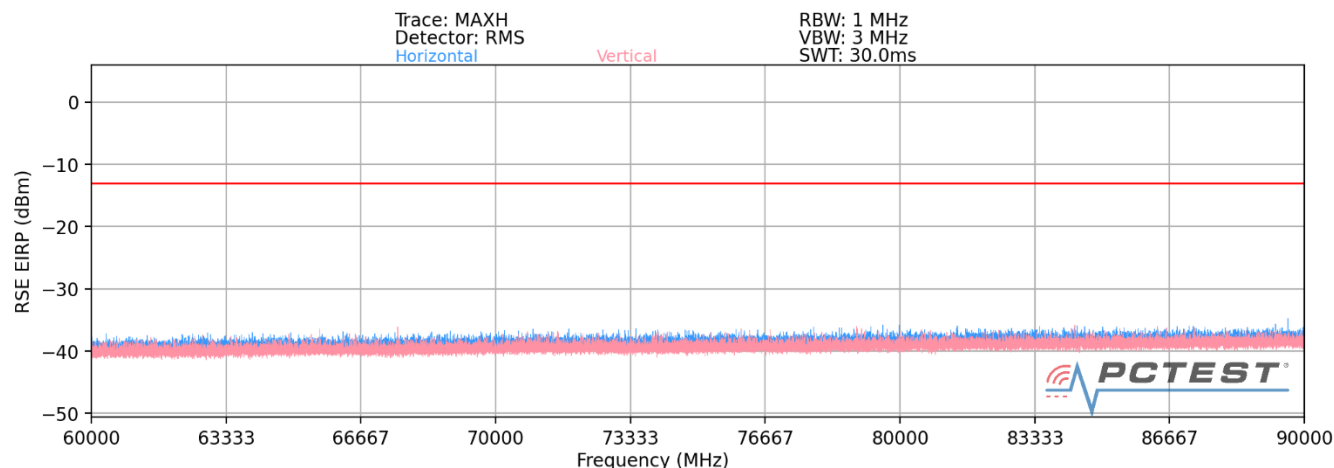
Plot 7-1. Ant 2-n260 Radiated Spurious Plot (1CC QPSK Mid Channel V Beam – ENDC Anchor Band 2)
