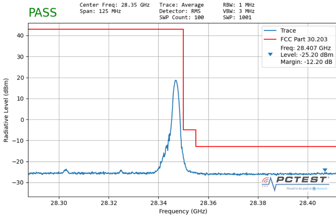
Plot 7-65. Ant 1 Upper Band Edge (50MHz-1CC – QPSK 1 RB)
