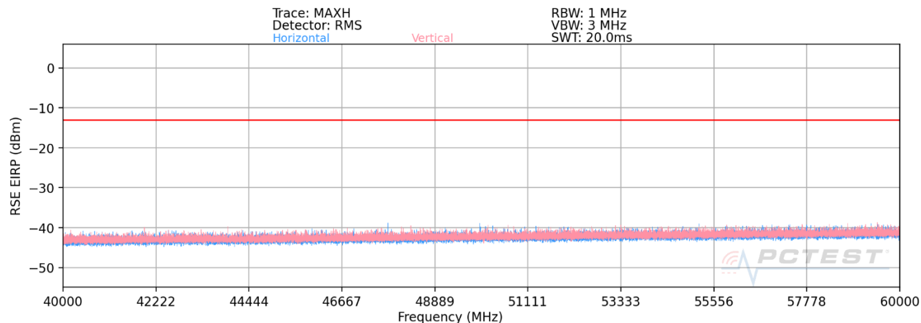
Plot 7-44. Ant 2-n261 Radiated Spurious Plot (1CC QPSK Mid Channel – ENDC Anchor B2)
